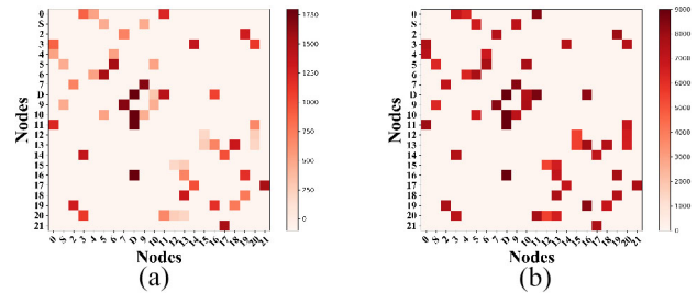
Fig. 7. R and Q matrices while training the S-Nav system.
