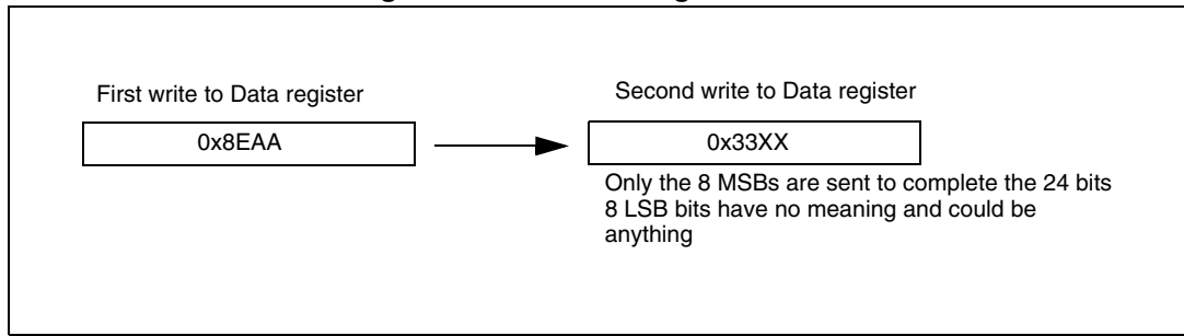
Figure 266. Transmitting 0x8EAA33
