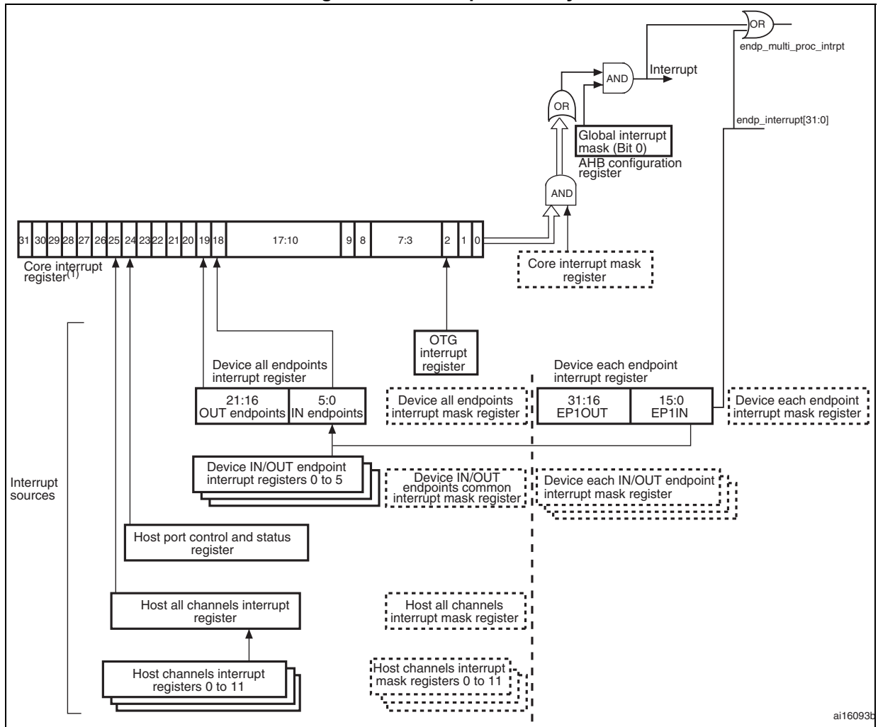
Figure 412. Interrupt hierarchy
