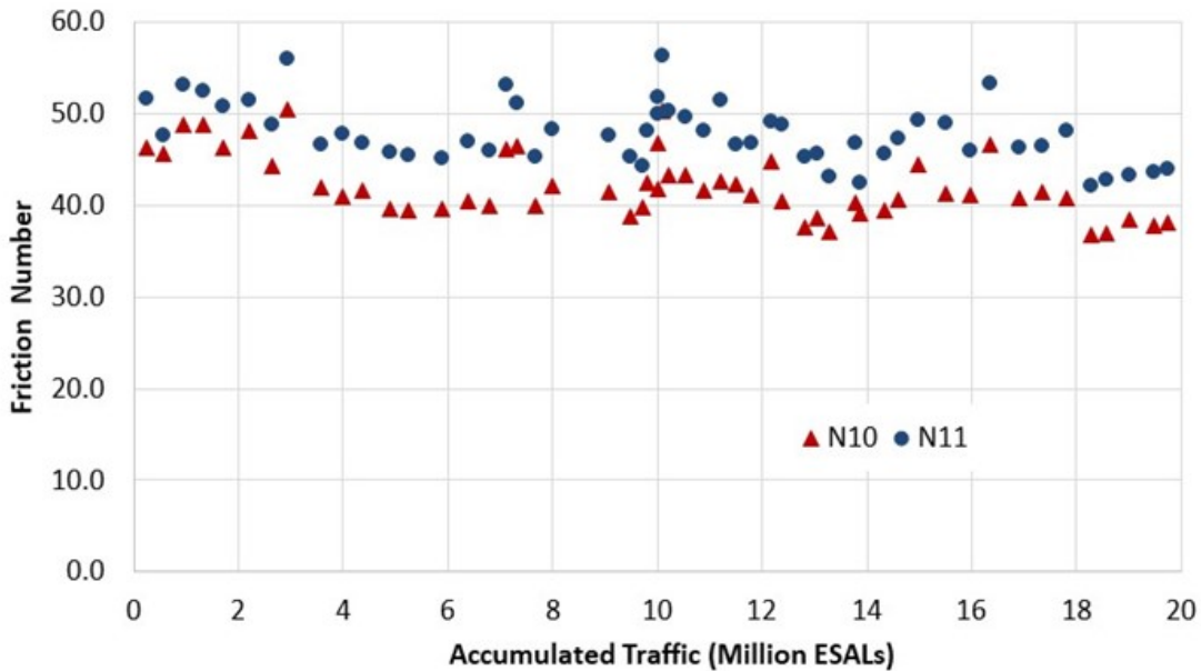
FIGURE 6 Locked-wheel friction tester data.
