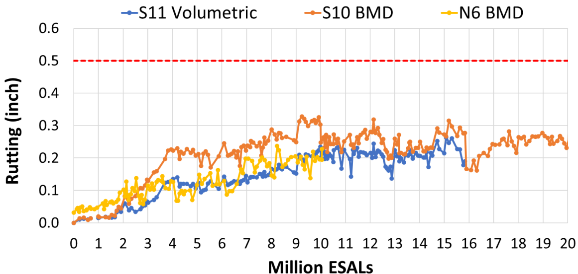
FIGURE 11. Field rutting data.
