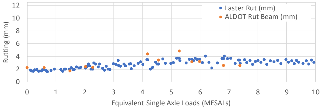
FIGURE 4 Rutting results.
