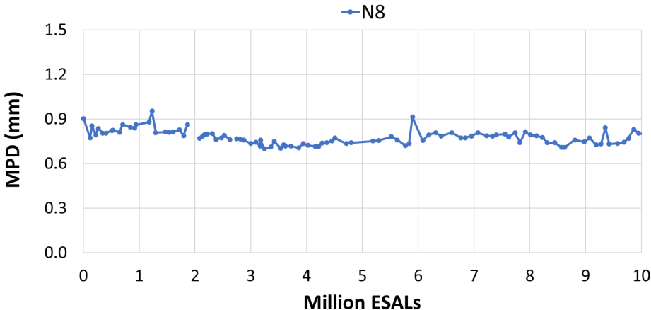
FIGURE 14 Field surface texture data of Section N8.
