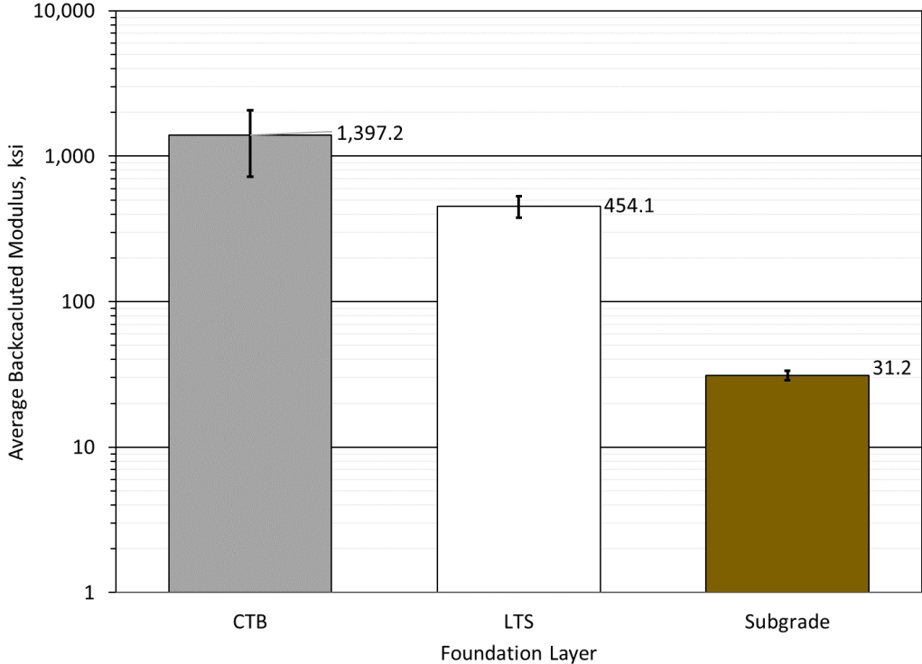
FIGURE 12 Average foundation backcalculated layer moduli in Section S2.
