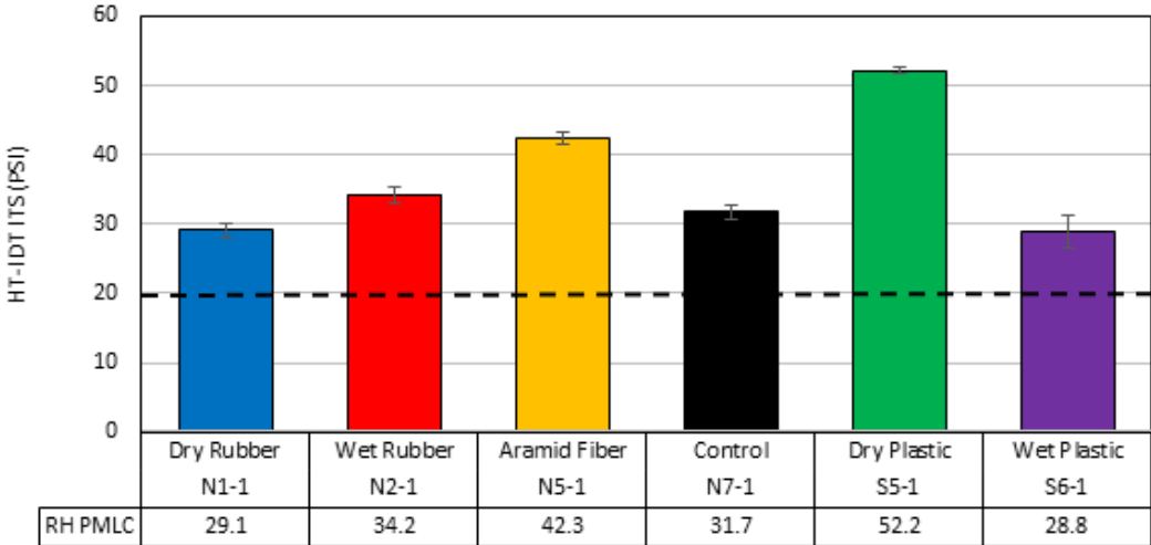
FIGURE 12 HT-IDT results for PMLC RH mixtures.
