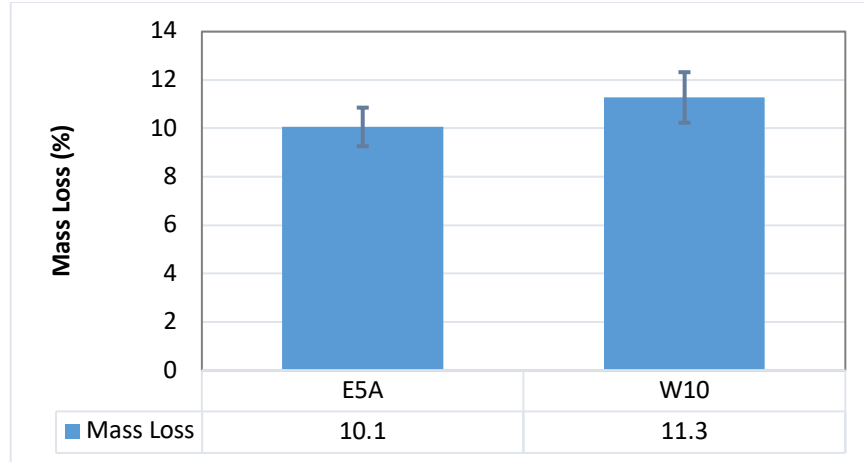
FIGURE 12 Cantabro mass loss of specimens compacted to 6.5 +/- 0.5 percent air voids.
