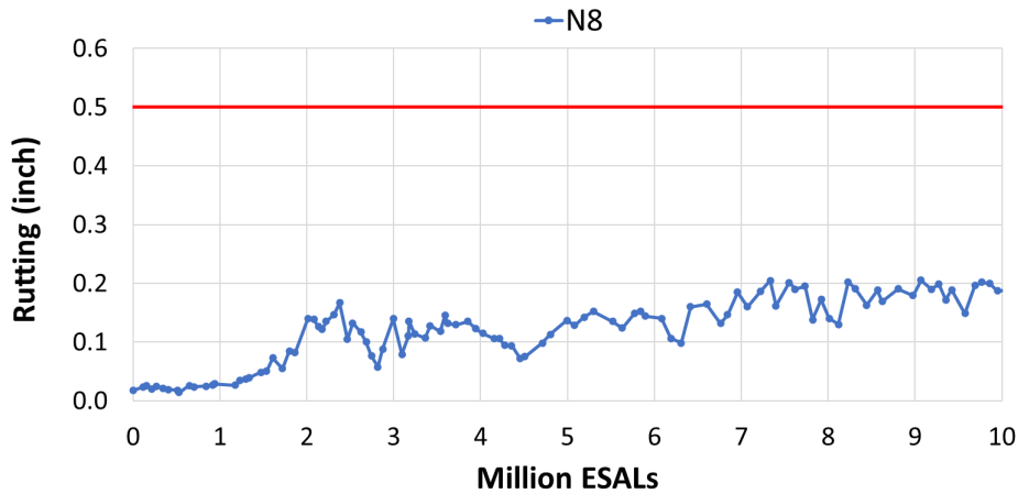
FIGURE 12 Field rutting data of Section N8.
