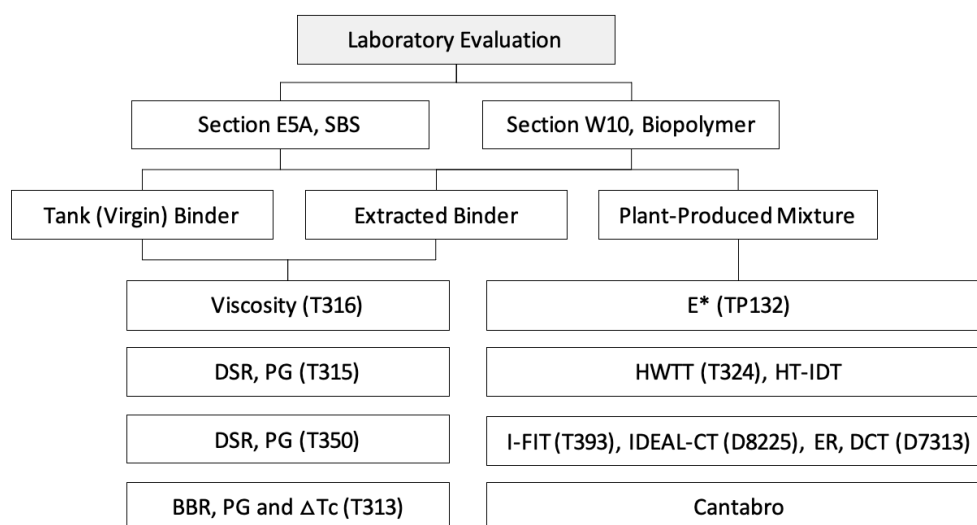
FIGURE 3 Testing plan performed for asphalt binder evaluation.
