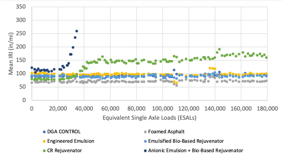
FIGURE 6 Mean IRI.
