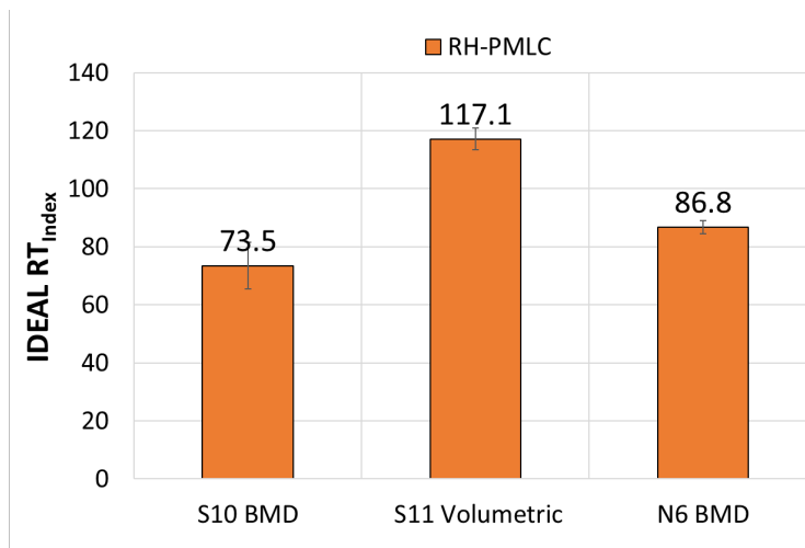
FIGURE 10. IDEAL RT_{Index} results of reheated PMLC specimens.
