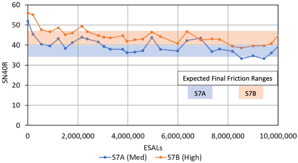
FIGURE 11 SN40R performance of S7A and S7B.
