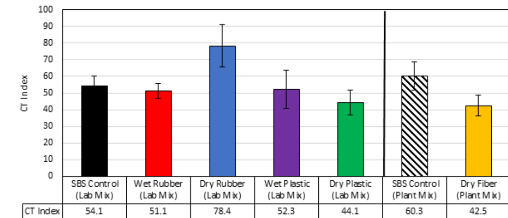
FIGURE 5 Phase I IDEAL-CT results.
