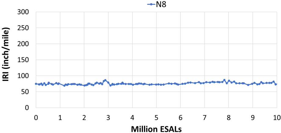
FIGURE 13 Field smoothness data of Section N8.
