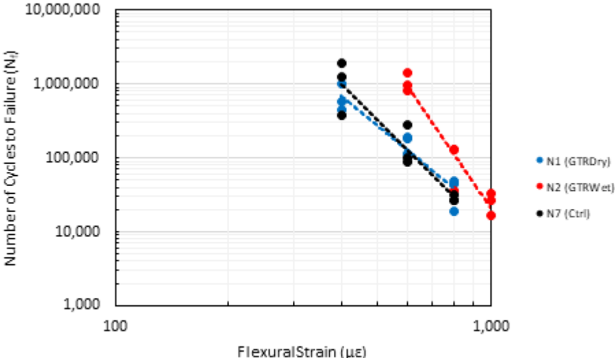
FIGURE 19 Fatigue life transfer functions (rubber-modified and control).
