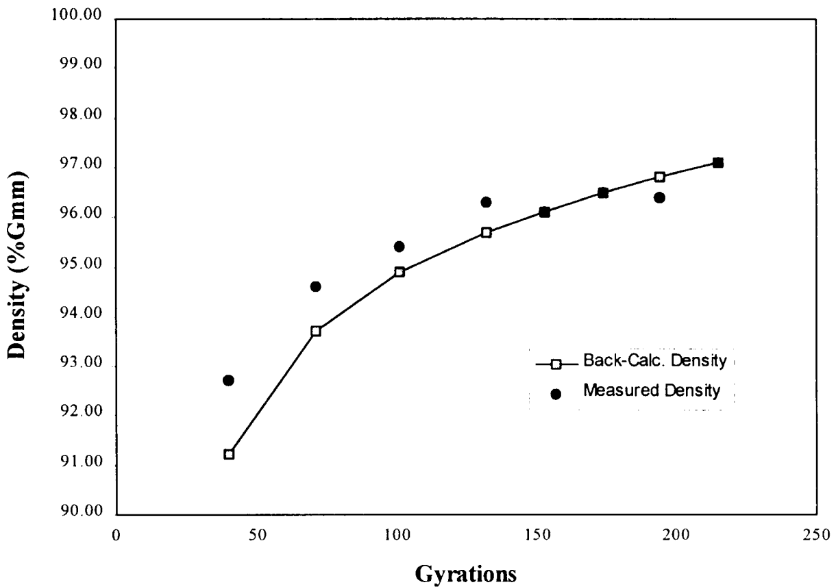
Figure 8. Density Versus Gyration Level for the SMA Mixture
