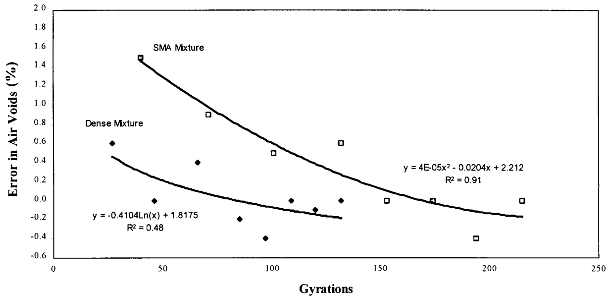
Figure 9. Error in Air Voids Calculation Versus Gyration Level
