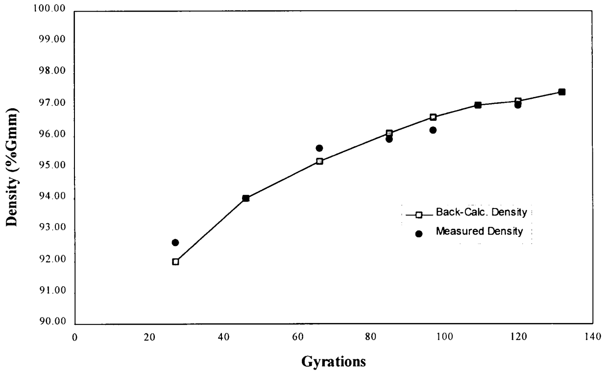
Figure 7. Density Versus Gyration Level for the Dense Mixture
