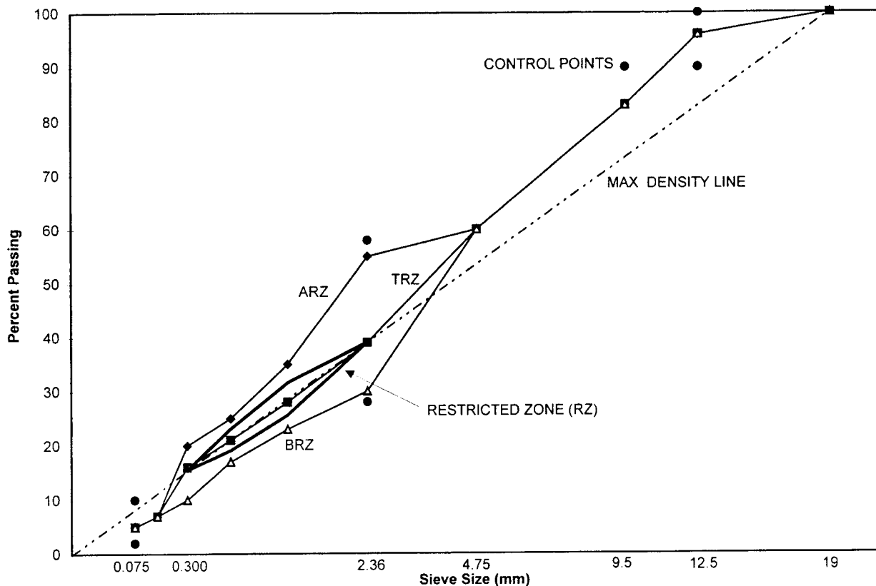
Figure 1. Gradation Criteria and Project Gradations
