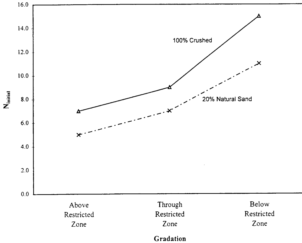
Figure 4. N_{initial} Versus Gradation
