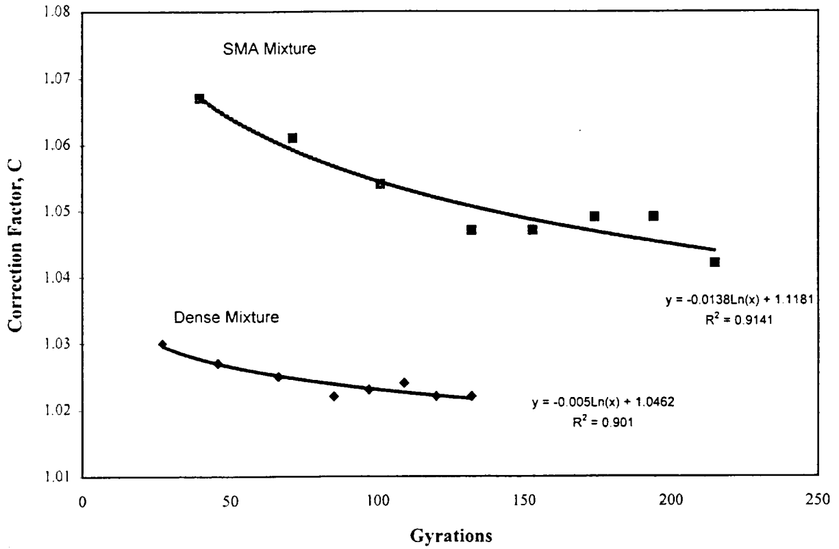
Figure 6. Correction Factor Versus Gyration Level
