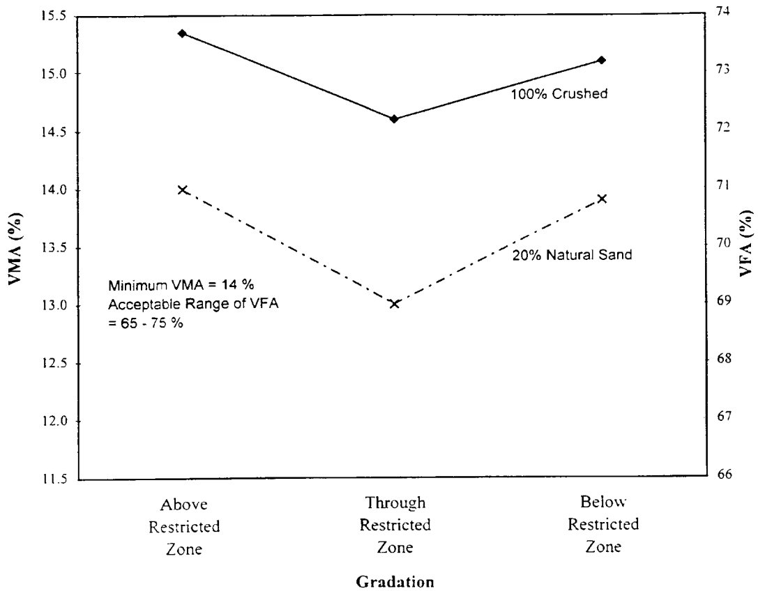
Figure 3. Voids in Mineral Aggregate and Voids Filled with Asphalt Versus Gradation
