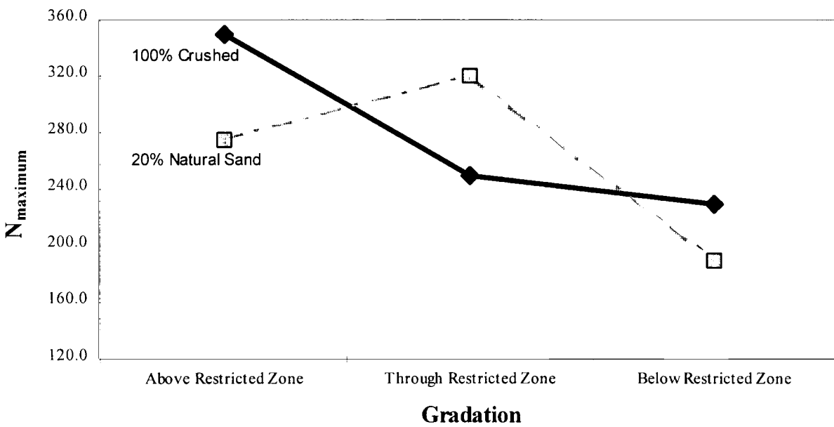
Figure 5. N_{maximum} Versus Gradation
