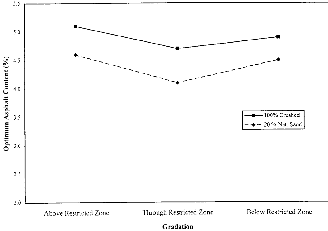
Figure 2. Optimum Asphalt Contents Versus Gradation
