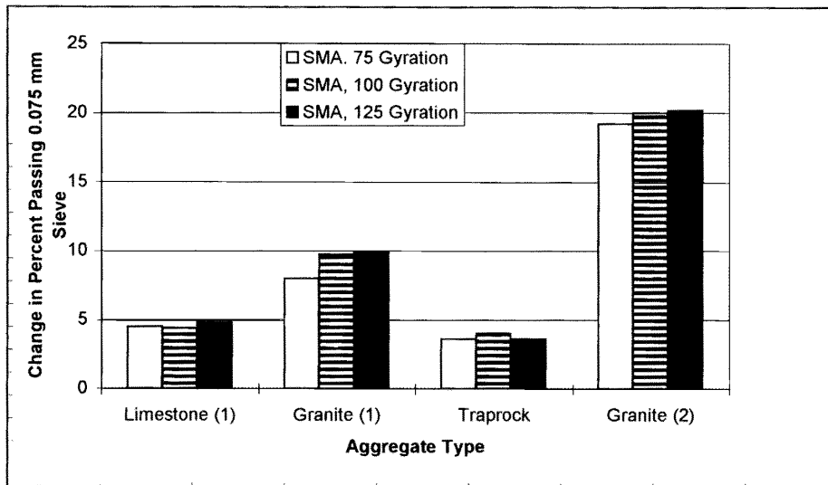
Figure 16. Aggregate Type Versus Change in Percent Passing 0.075 mm Sieve at Different Compaction Levels (Mixes Compacted with SGC)
