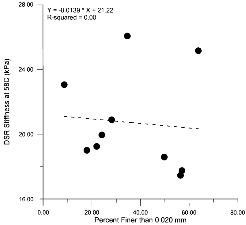
Figure 6. Percent Finer Than 0.020 mm versus DSR Stiffness at 58°C
