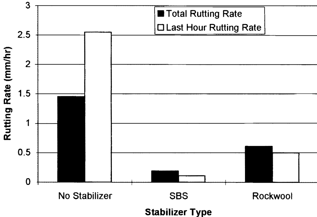
Figure 18. Stabilizer Type versus Rutting Rate
