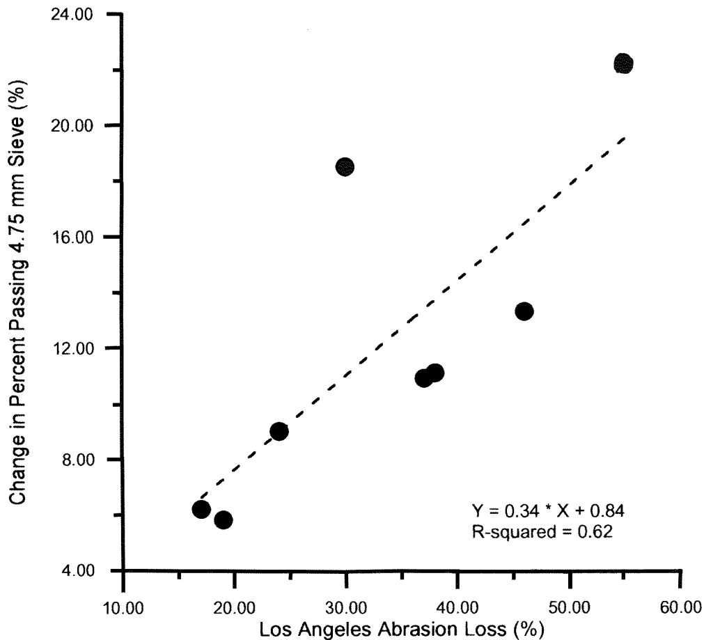
Figure 1. Los Angeles Abrasion Loss Versus Change in Percent Passing 4.75 mm Sieve (50 Blow Marshall Compaction)
