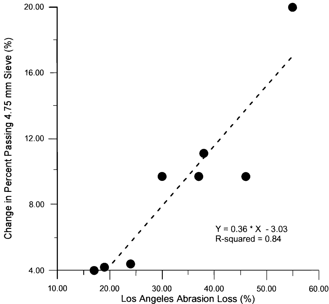
Figure 2. Los Angeles Abrasion Loss Versus Change in Percent Passing 4.75 mm Sieve (Compaction with 100 Revolutions of SGC)
