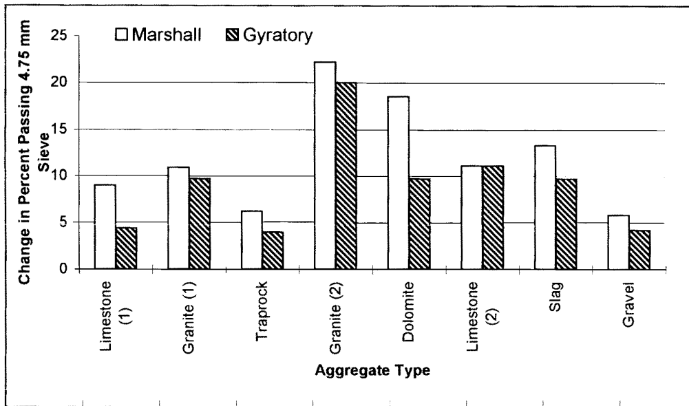
Figure 11. Aggregate Type Versus Change in Percent Passing 4.75 mm Sieve
