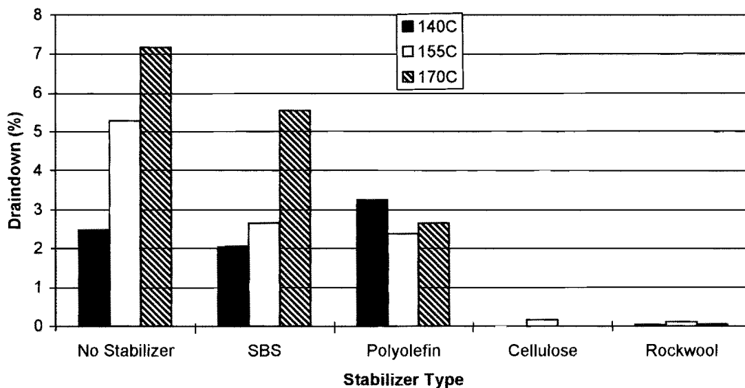
Figure 17. Stabilizer Type versus Draindown
