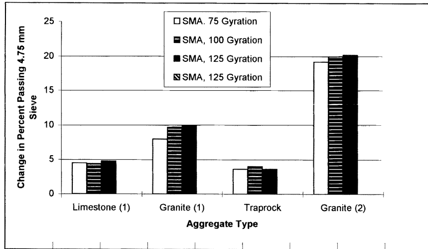
Figure 15. Aggregate Type Versus Change in Percent Passing 4.75 mm Sieve at Different Compaction Levels (Mixes Compacted with SGC)
