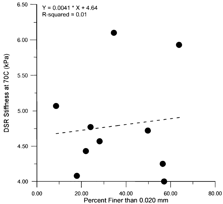
Figure 7. Percent Finer Than 0.020 mm versus DSR Stiffness at 70°C
