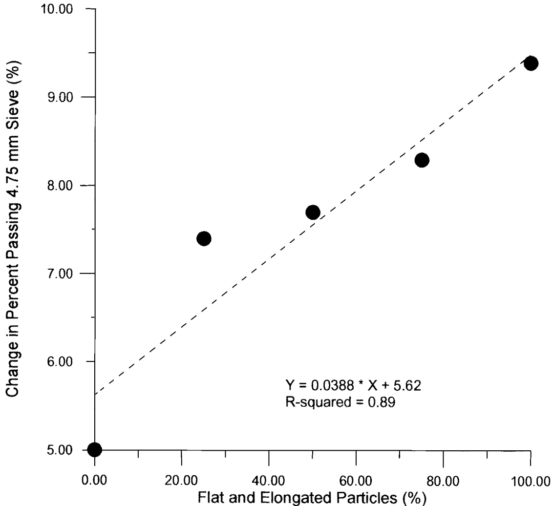
Figure 3. Flat and Elongated Particle Content Versus Change in Percent Passing 4.75 mm Sieve (50-Blow Marshall Compaction)
