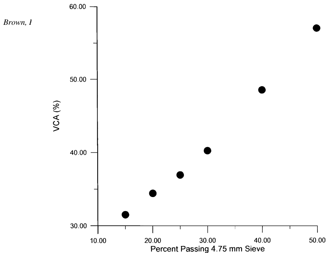
Figure 5. Percent Passing 4.75 mm Sieve Versus VCA (Gravel Mixes, 50-Blow Marshall Compaction)
