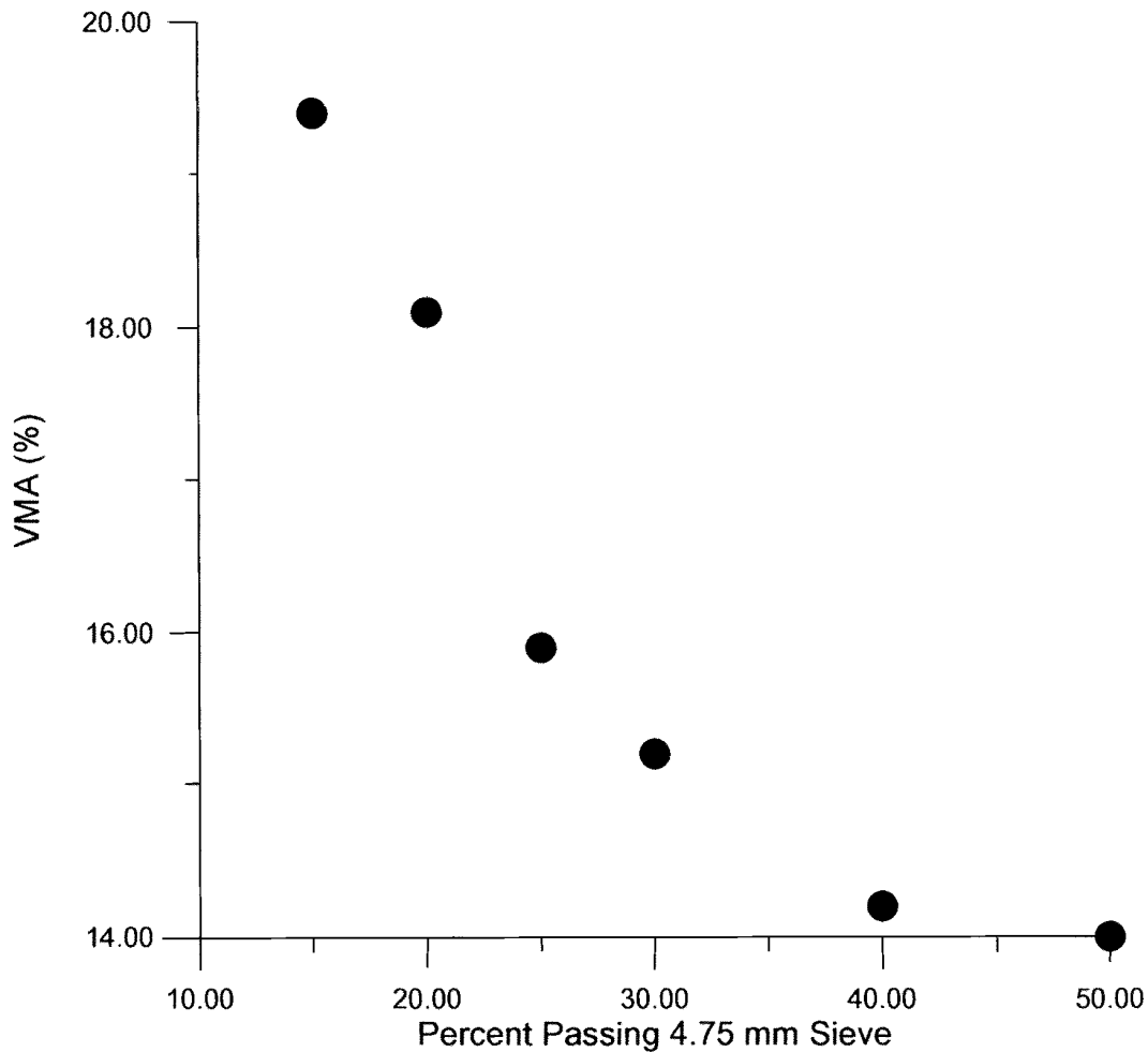
Figure 4. Percent Passing 4.75 mm Sieve Versus VMA (Gravel Mixes, 50-Blow Marshall Compaction)
