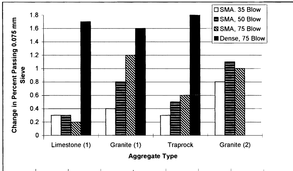
Figure 14. Aggregate Type Versus Change in Percent Passing 0.075 mm Sieve at Different Compaction Levels (Mixes Compacted with Marshall Hammer)
