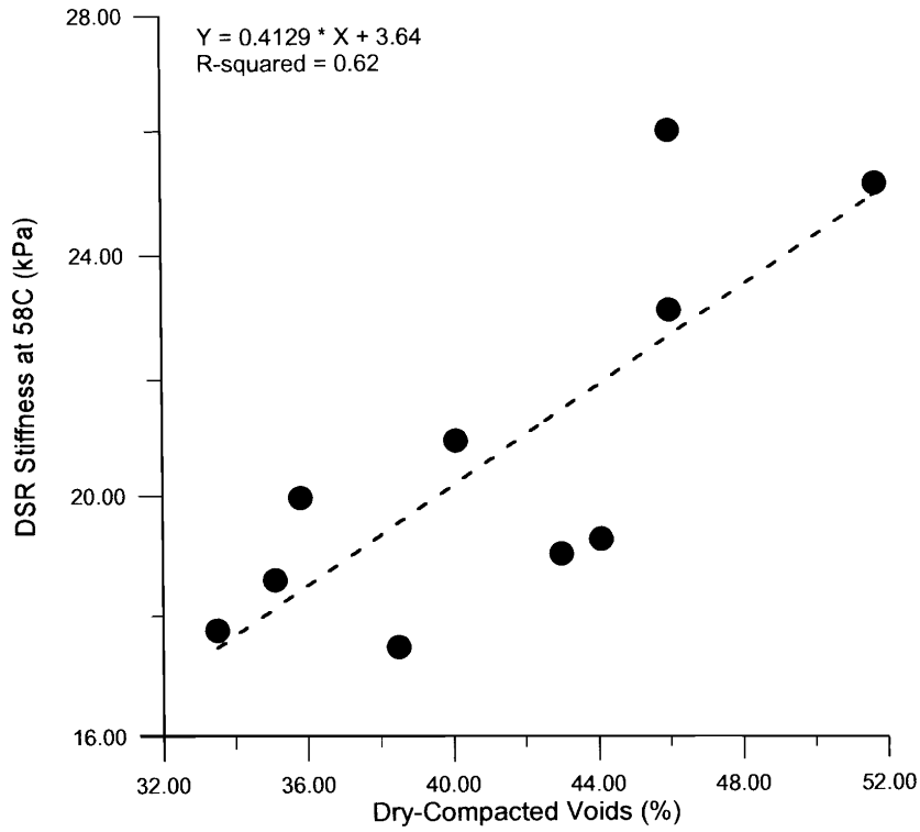
Figure 8. Dry-Compacted Voids versus DSR Stiffness at 58°C
