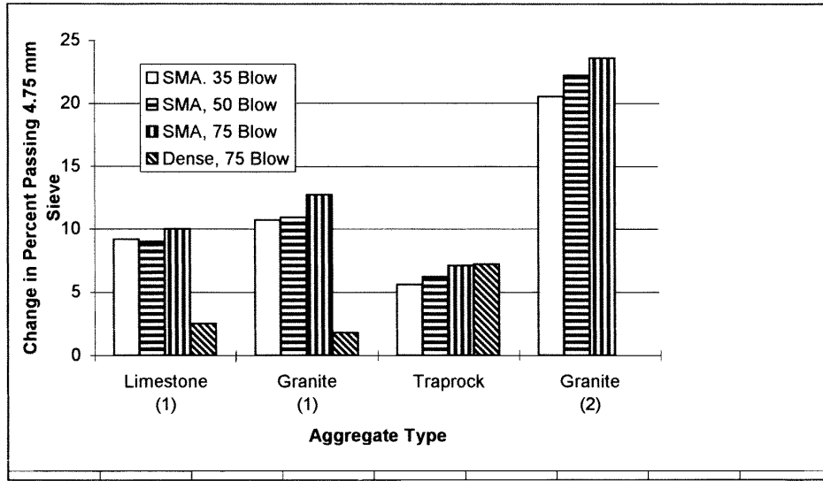
Figure 13. Aggregate Type Versus Change in Percent Passing 4.75 mm Sieve at Different Compaction Levels (Mixes Compacted with Marshall Hammer)
