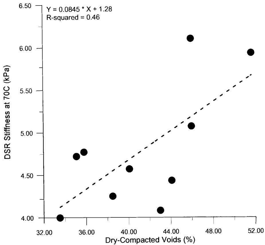
Figure 9. Dry-Compacted Voids versus DSR Stiffness at 70°C
