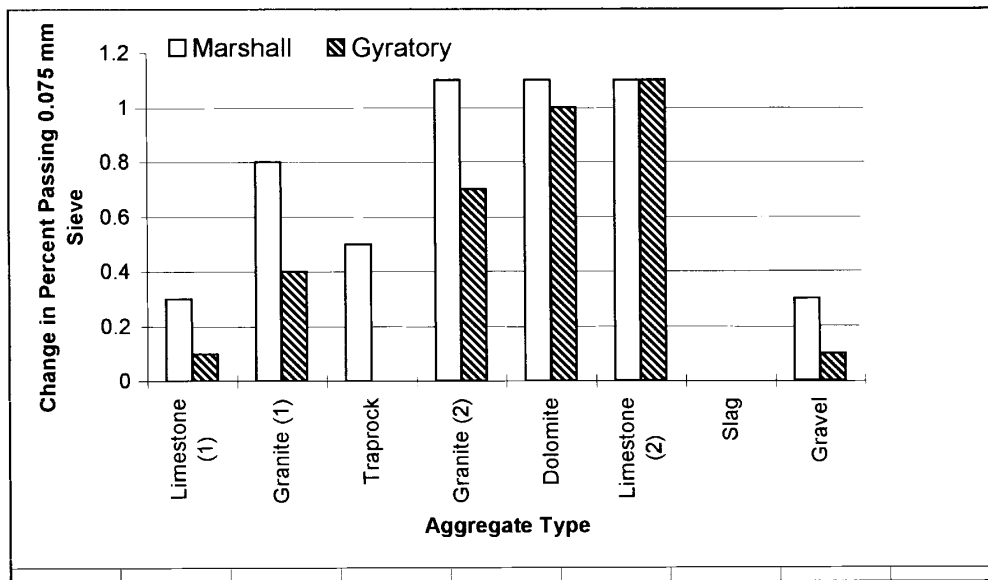
Figure 12. Aggregate Type Versus Change in Percent Passing 0.075 M Sieve
