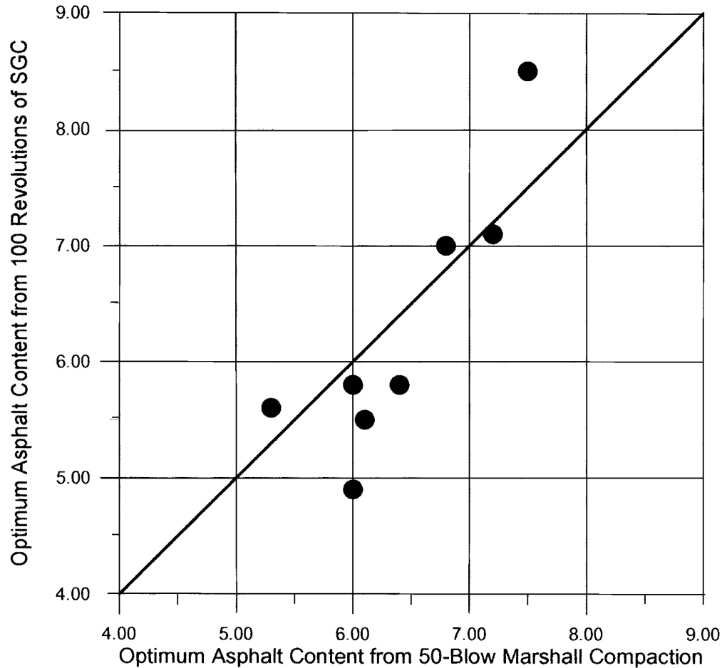
Figure 10. Optimum Asphalt Content from Marshall Compaction Versus Optimum Asphalt Content from SGC Compaction
