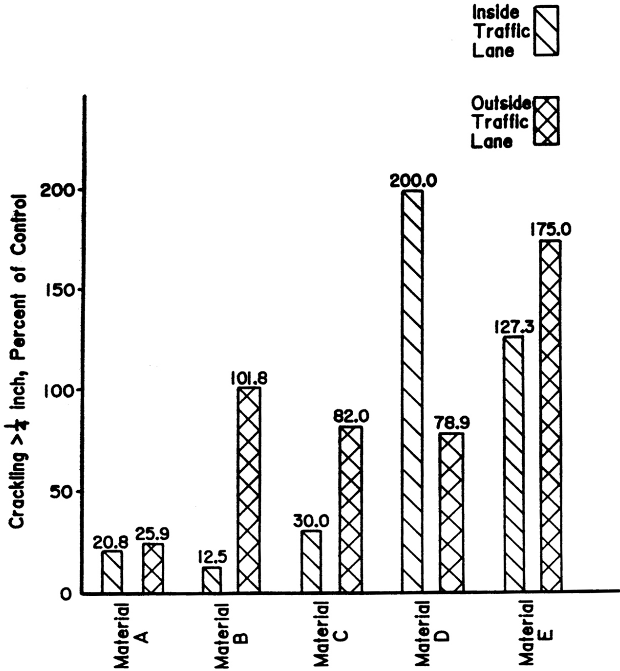
Figure 5. Relationship Between Material Type and Cracking Wider Than 1/4 Inch
