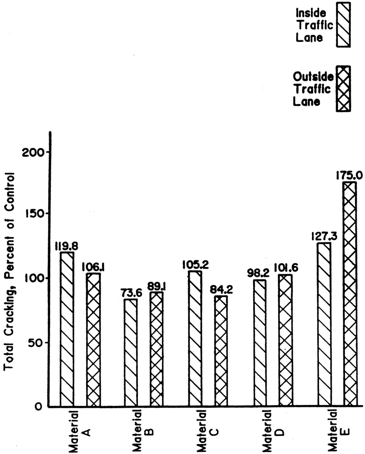
Figure 4. Relationship Between Material Type and Total Cracking
