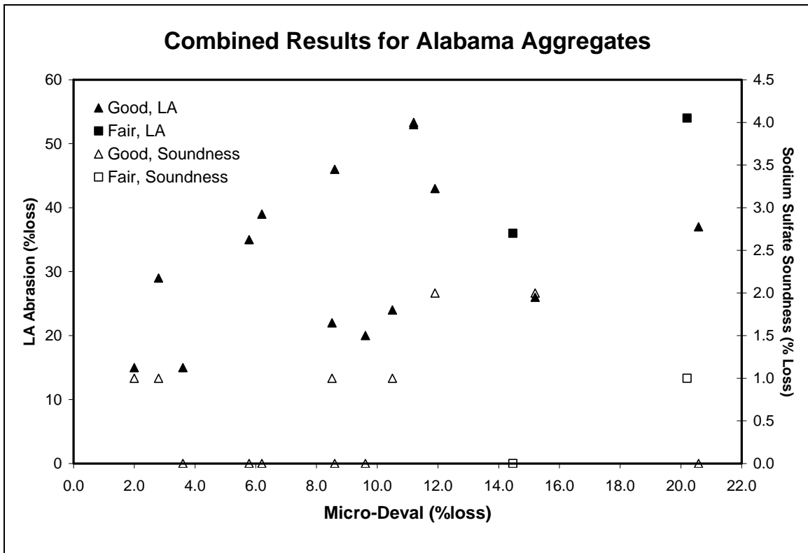
Figure 1. Test Results for Alabama Aggregates by Performance Ranking
