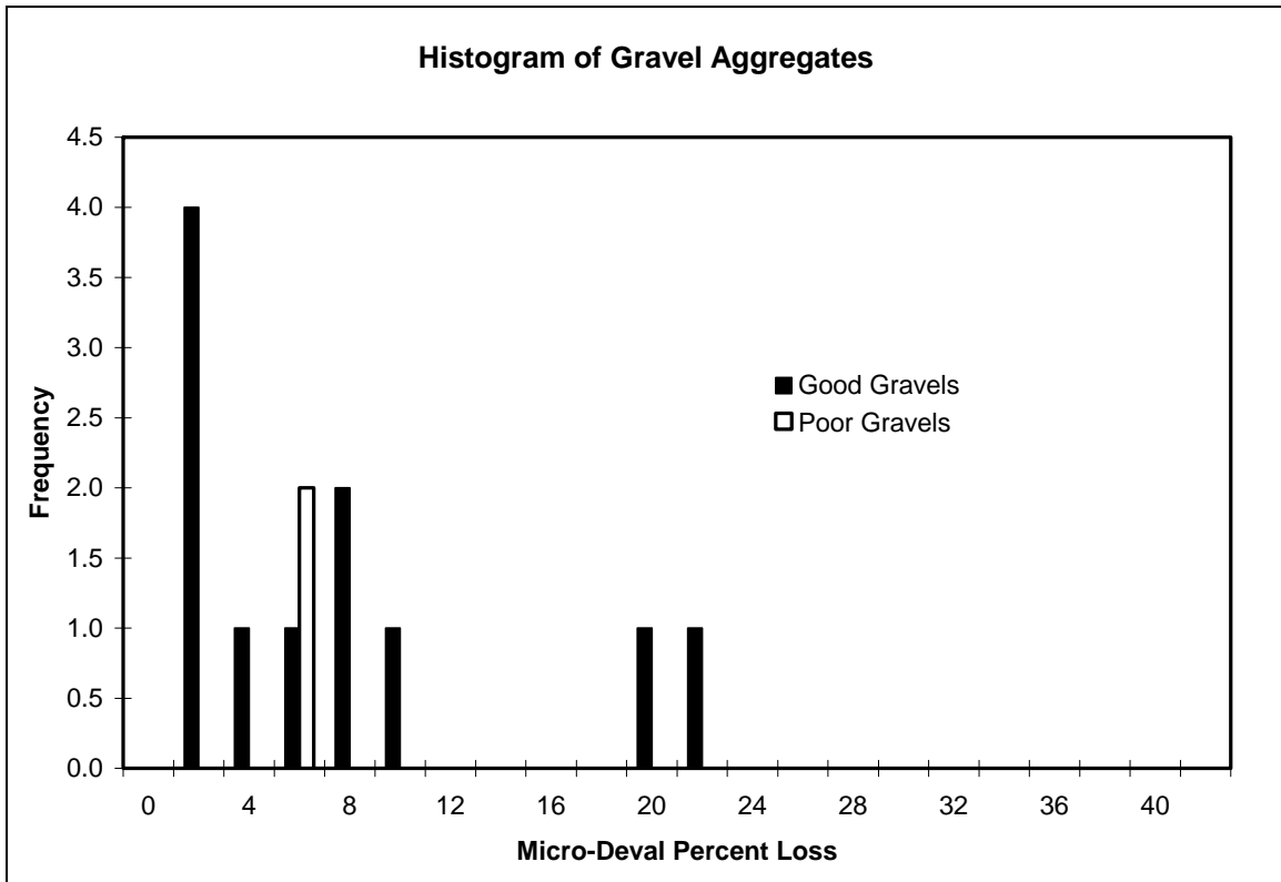
Figure 19. Histogram of Micro-Deval Results for Gravel Aggregates By Performance Category
