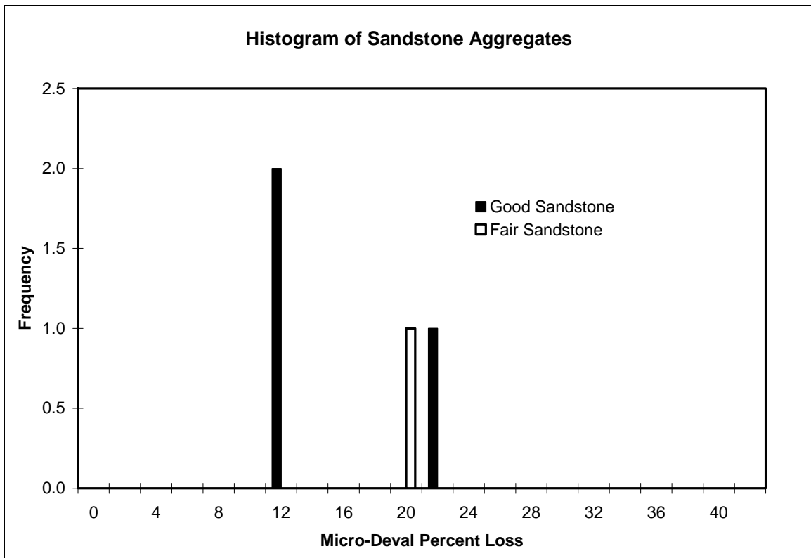
Figure 20. Histogram of Micro-Deval Results for Sandstone Aggregates By Performance Category
