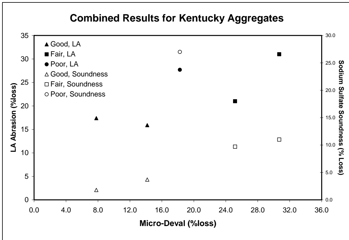
Figure 4. Test Results for Kentucky Aggregates by Performance Ranking
