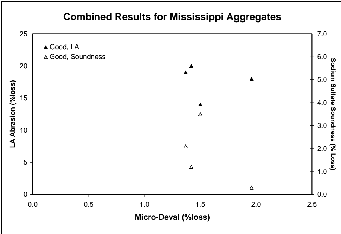
Figure 5. Test Results for Mississippi Aggregates by Performance Ranking
