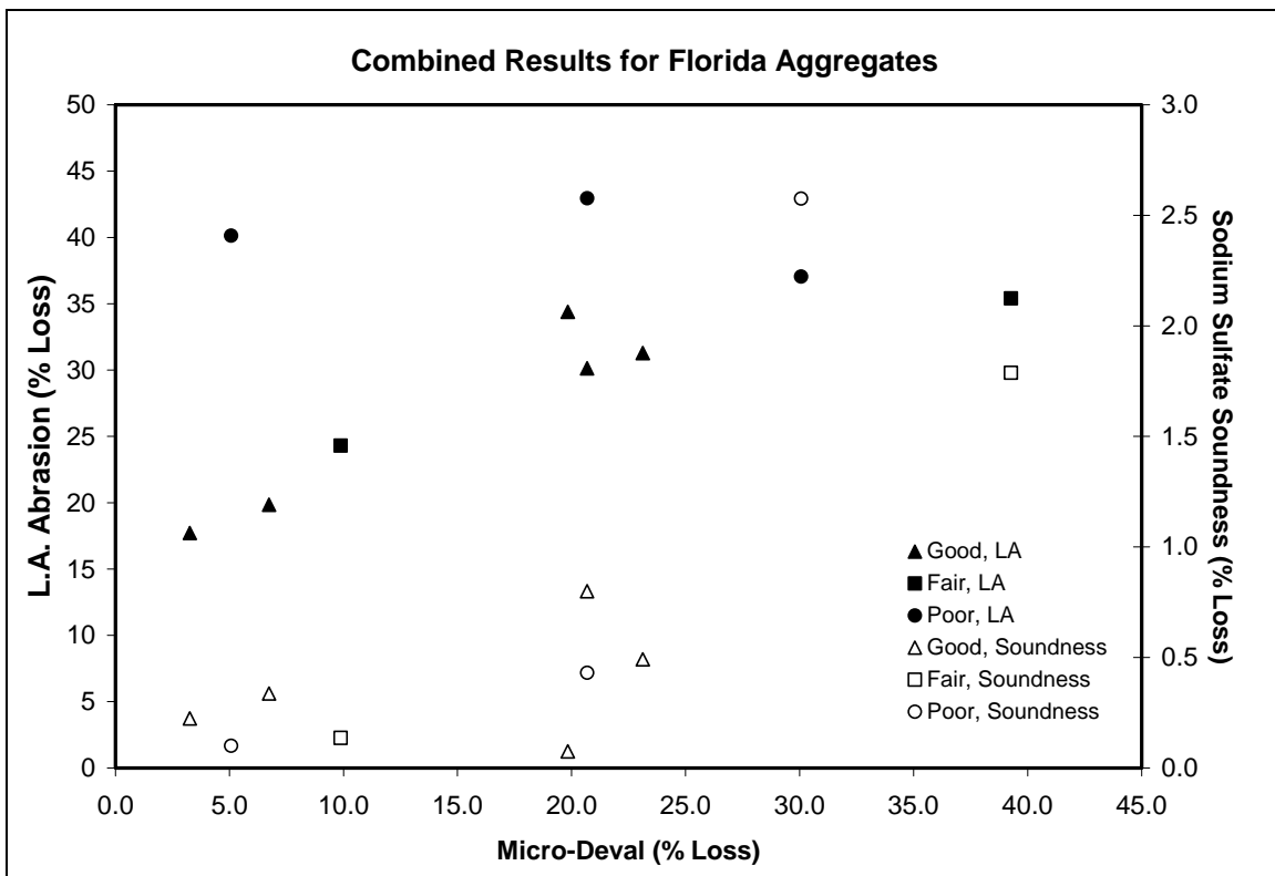
Figure 2. Test Results for Florida Aggregates by Performance Ranking
