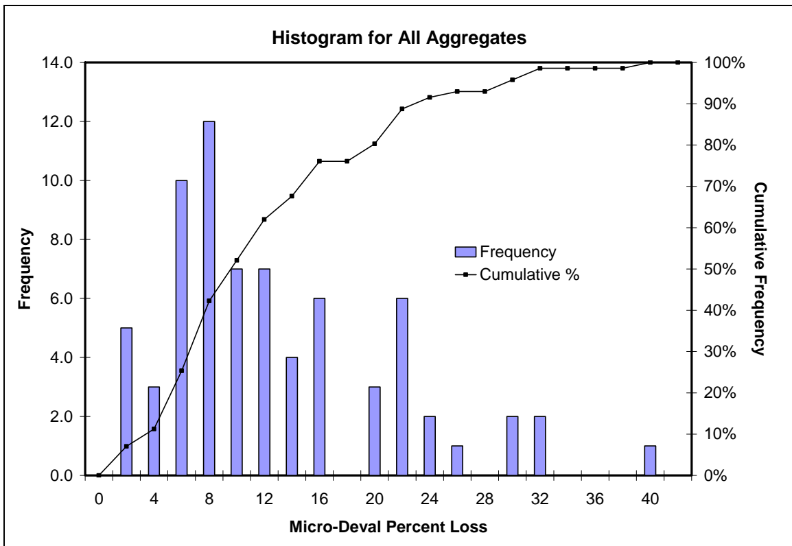
Figure 9. Histogram of All Micro-Deval Test Results
