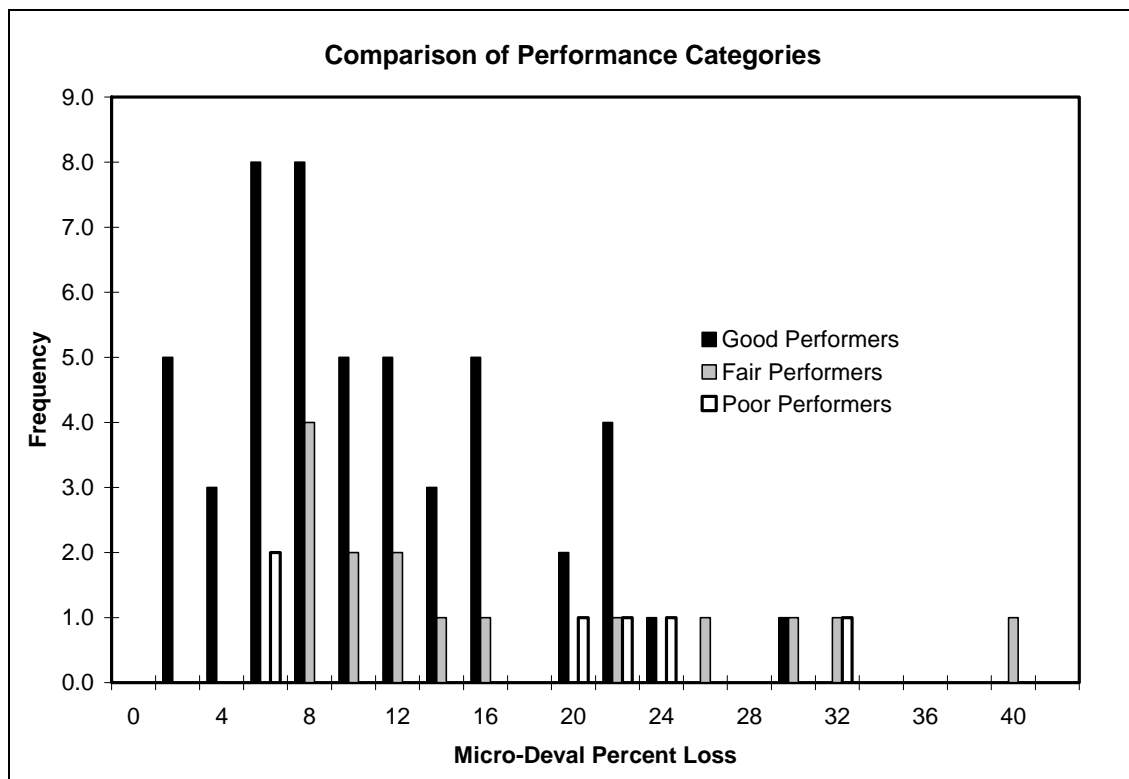
Figure 12. Comparison of Micro-Deval Test Results by Performance Category
