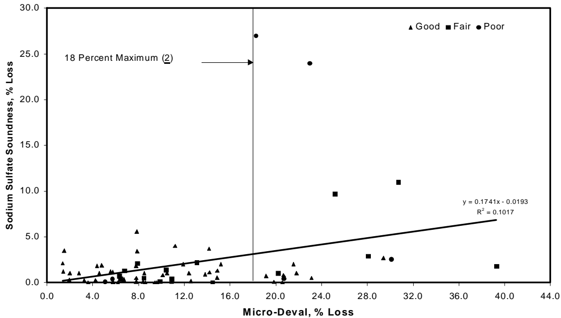
Figure 16. Comparison of Sodium Sulfate Soundness and Micro-Deval Test Results
