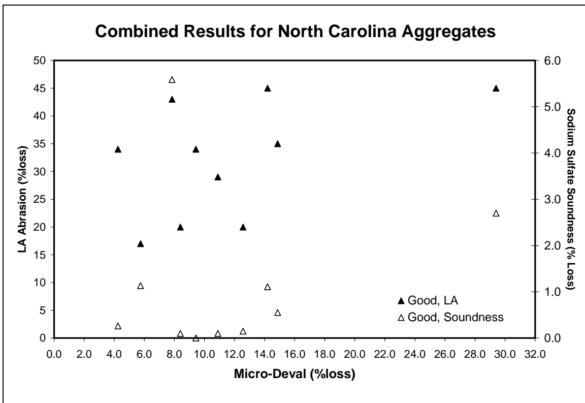
Figure 6. Test Results of Testing on North Carolina Aggregates by Performance Ranking
