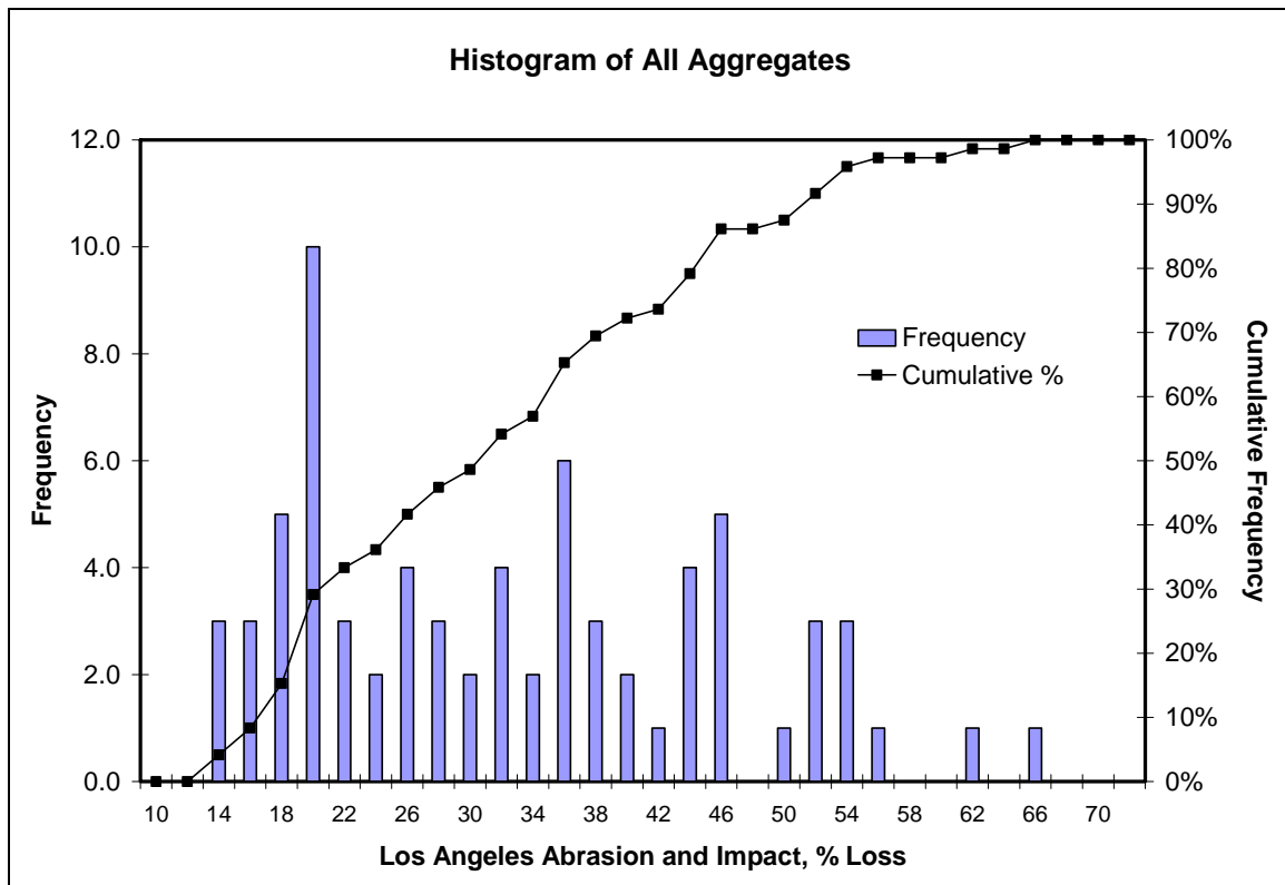
Figure 10. Histogram of All L.A. Abrasion and Impact Test Results
