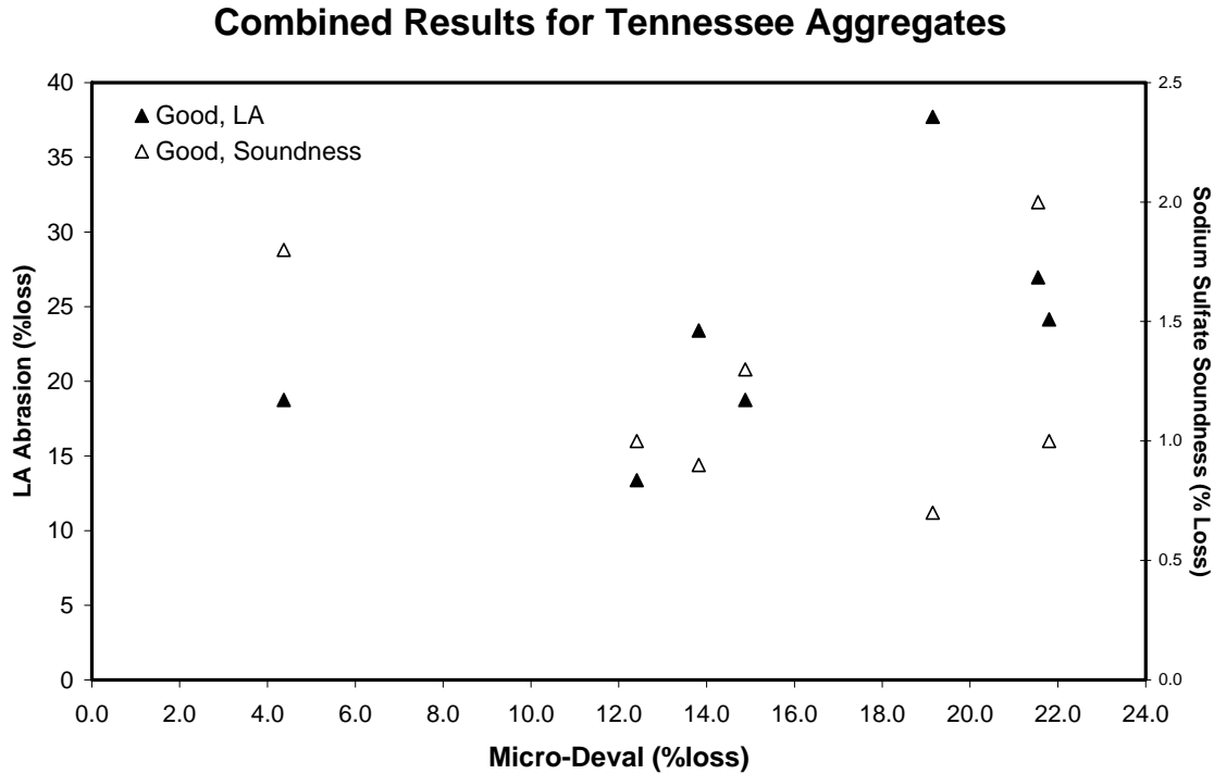
Figure 8. Test Results for Tennessee Aggregates by Performance Ranking
