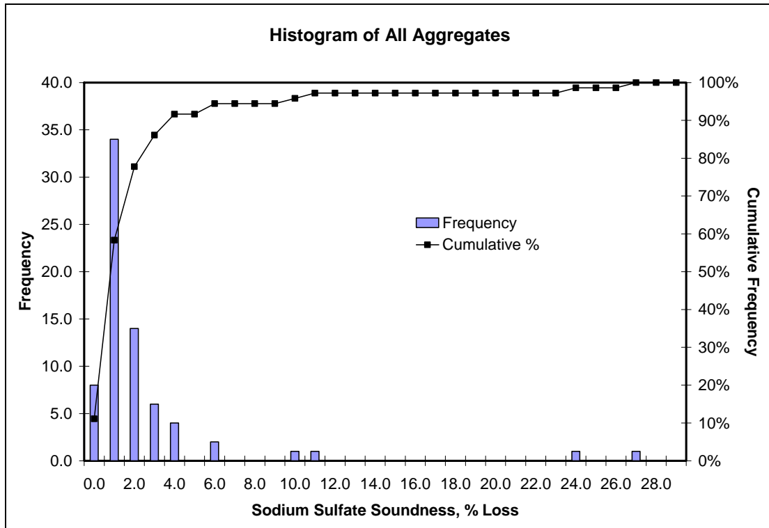
Figure 11. Histogram of All Sodium Sulfate Soundness Test Results
