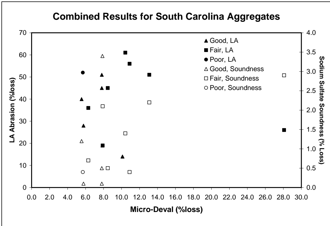
Figure 7. Test Results for South Carolina Aggregates by Performance Ranking
