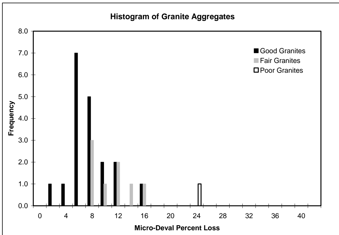
Figure 17. Histogram of Micro-Deval Results for Granite Aggregates By Performance Category
