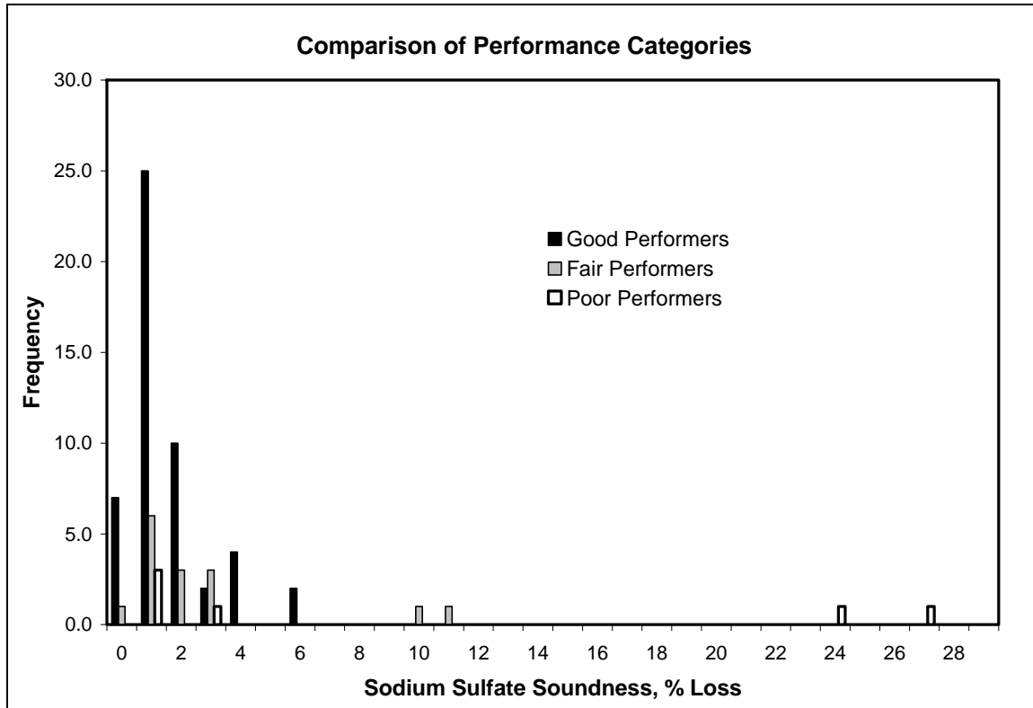
Figure 14: Comparison of Sodium Sulfate Soundness Test Results by Performance Category
