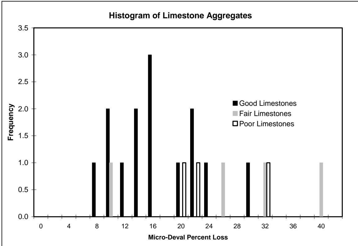
Figure 18. Histogram of Micro-Deval Results for Limestone Aggregates By Performance Category
