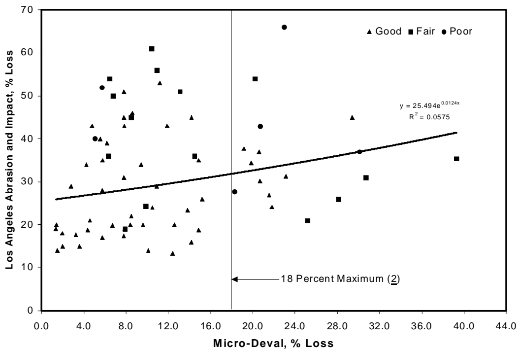
Figure 15. Comparison of L. A. Abrasion and Micro-Deval Test Results
