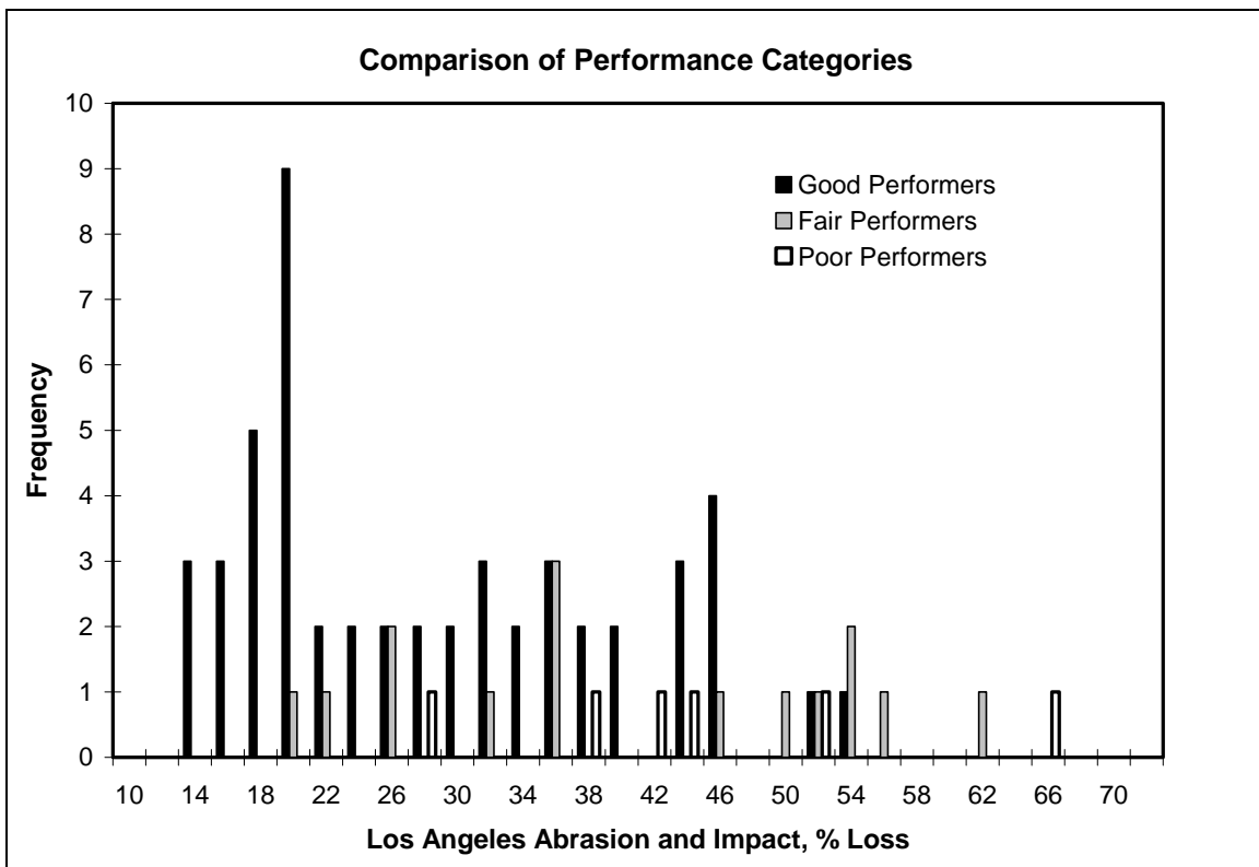
Figure 13. Comparison of L.A. Abrasion and Impact Test Results by Performance Category
