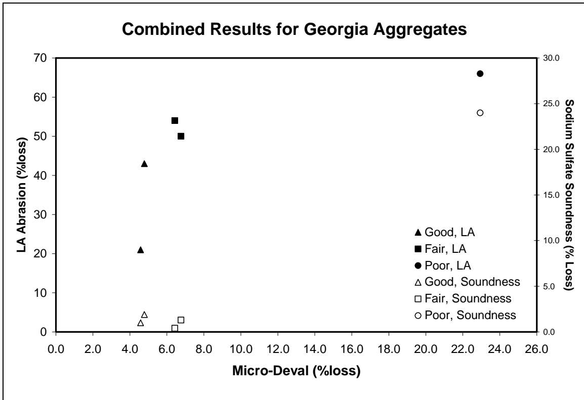
Figure 3. Test Results for Georgia Aggregates by Performance Ranking
