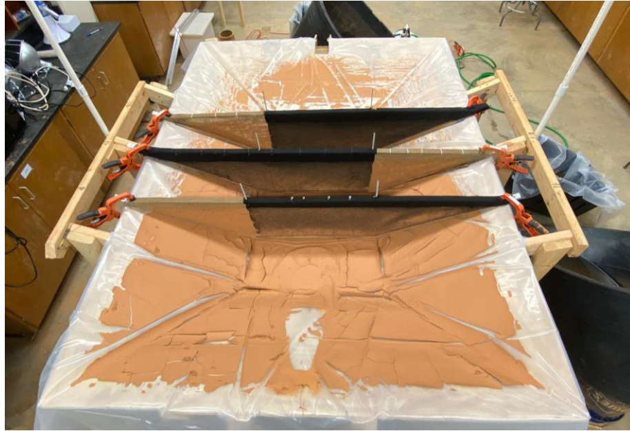
Figure 3.15: Standard Basin: Labyrinth Flow Path.
