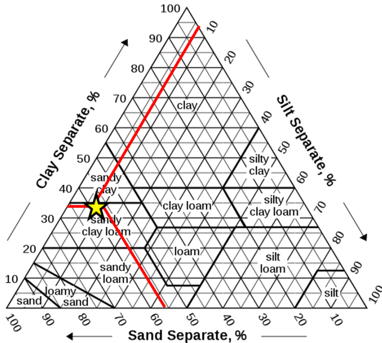
Figure 3.10: AU-SRF Soil Triangle.
