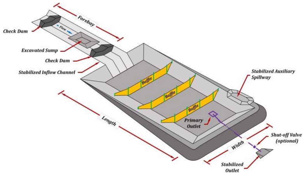
Figure 2.1: IECA Sediment Basin Standard Drawing (IECA 2021).
