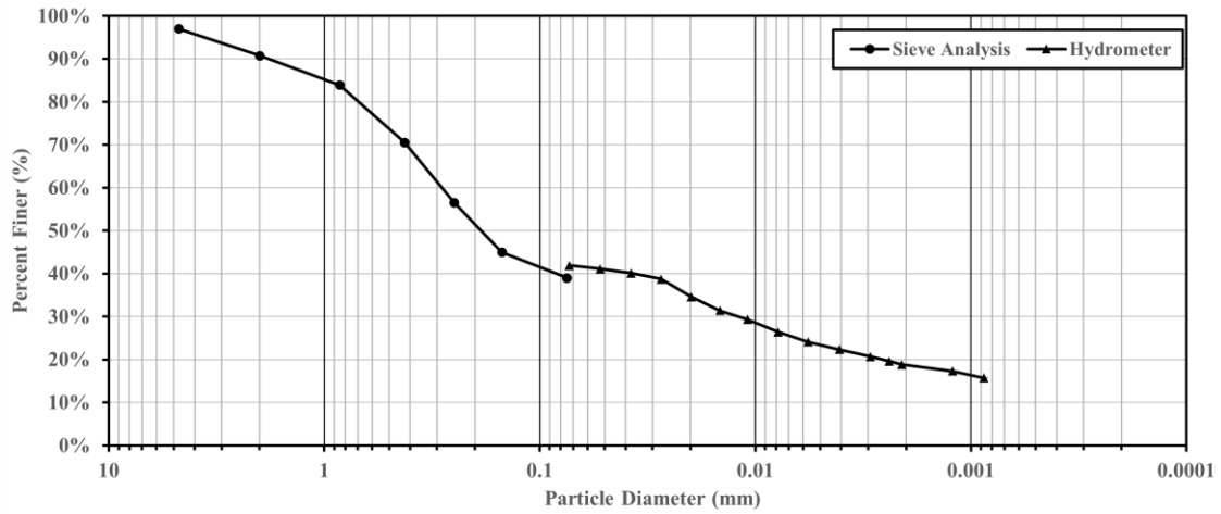
Figure 3.9 AU-SRF Soil Gradation Curve (Kazaz et al. 2021).
