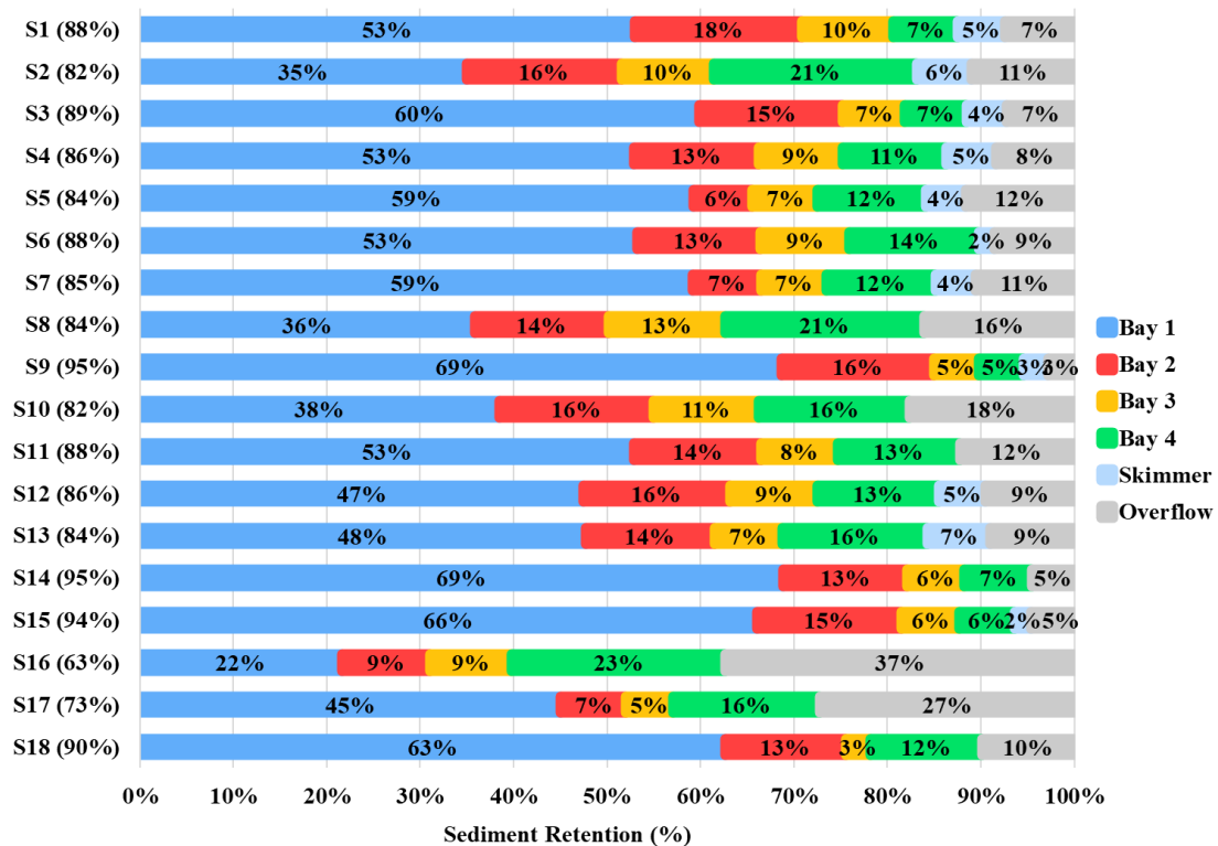
Figure 4.13 Sediment Retention by Location for All Configurations.
