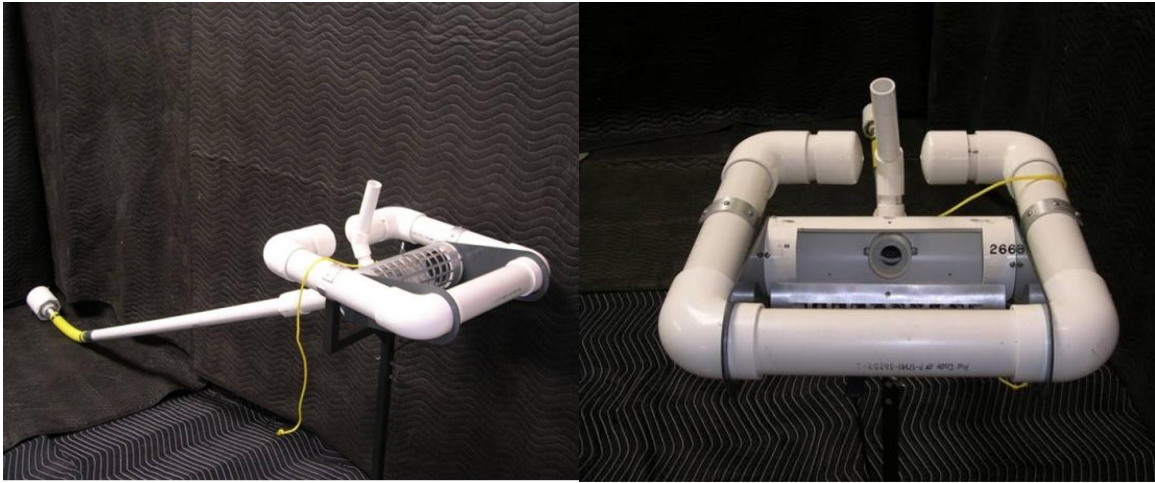
Figure 2.7: Faircloth Skimmer ® (Faircloth 2007).
