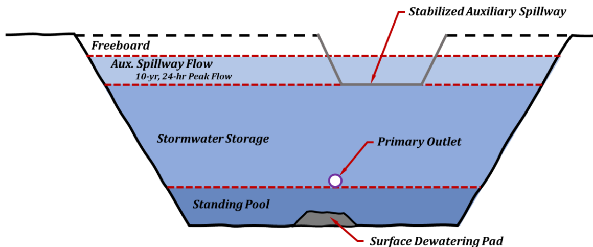
Figure 2.3 :Sediment Basin Cross-Section (IECA 2021).
