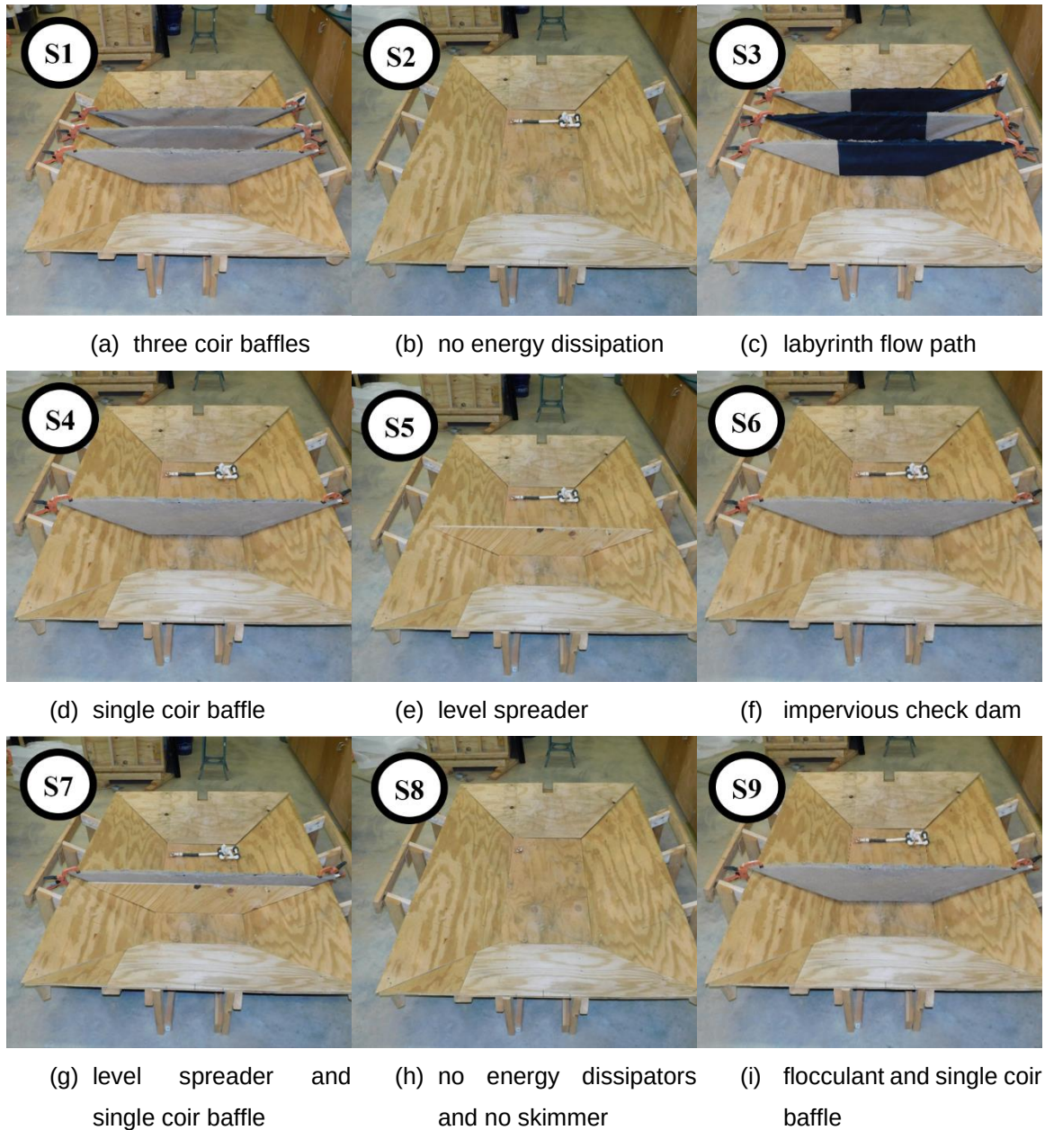
Figure 3.12: Nine Energy Dissipation Arrangements in the Standard Basin.
