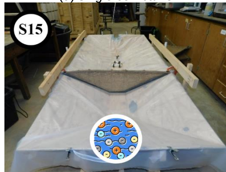
(f) flocculant with a single coir baffle.
