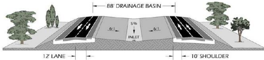
(a) cross-section view
