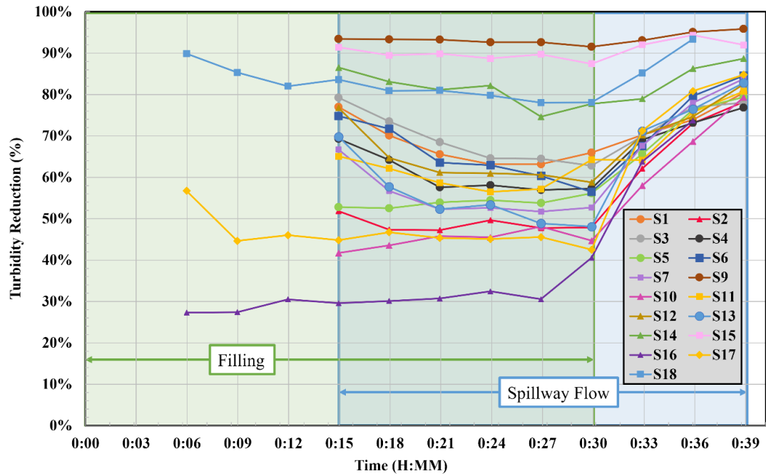
(a) inflow to skimmer
