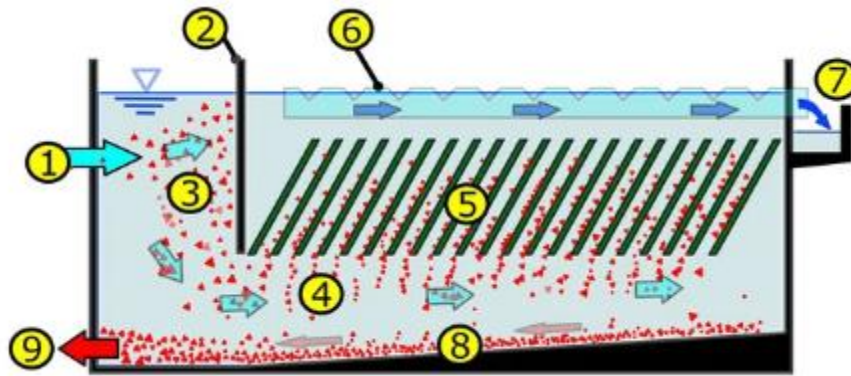
Figure 2.6: Lamella Settling Tank (Hewitech 2023).
