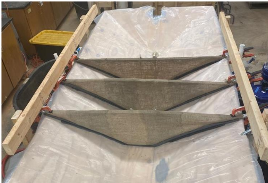
Figure 3.25: In-Channel Basin: Three Coir Baffles.
