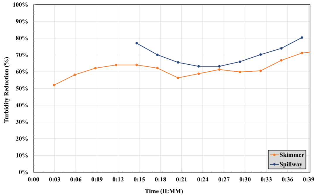
Figure 4.3 ALDOT Standard Turbidity Reduction.
