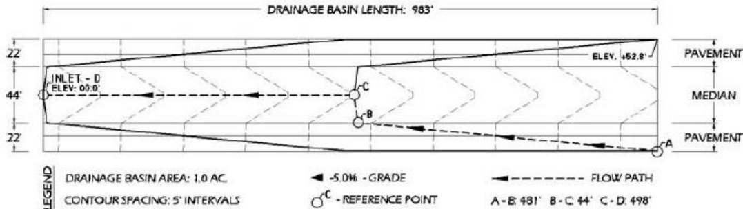
(b) plan view
