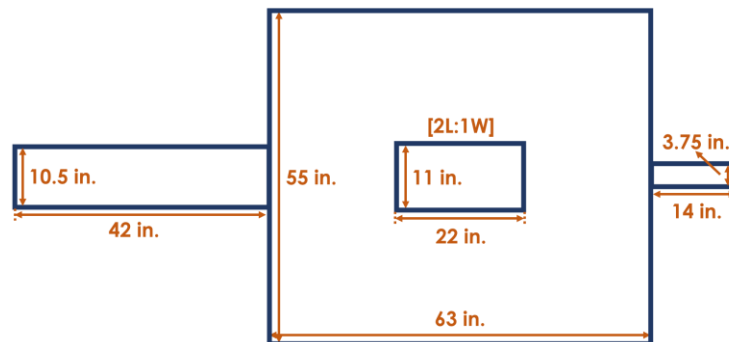
(c) undersized basin dimensions
