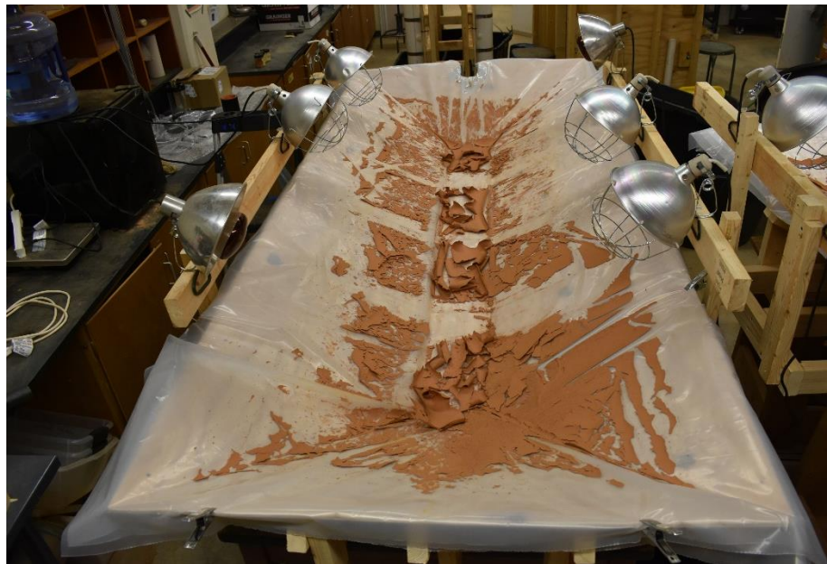
Figure 3.38: Dried Sediment Split by Bays.
