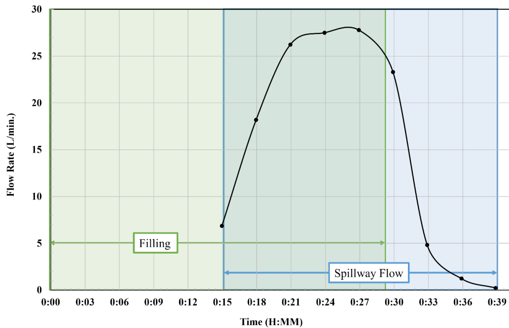
(b) spillway flow rate versus time
