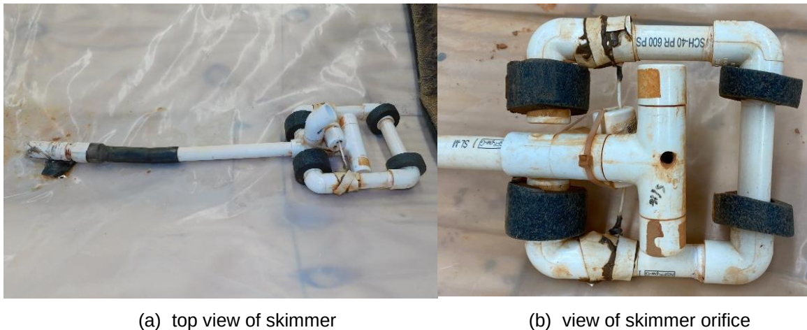
Figure 3.5: Skimmer Components.
