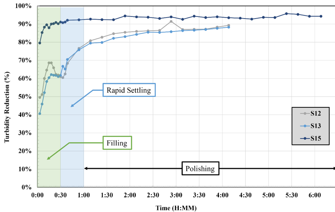
(b) full testing duration
