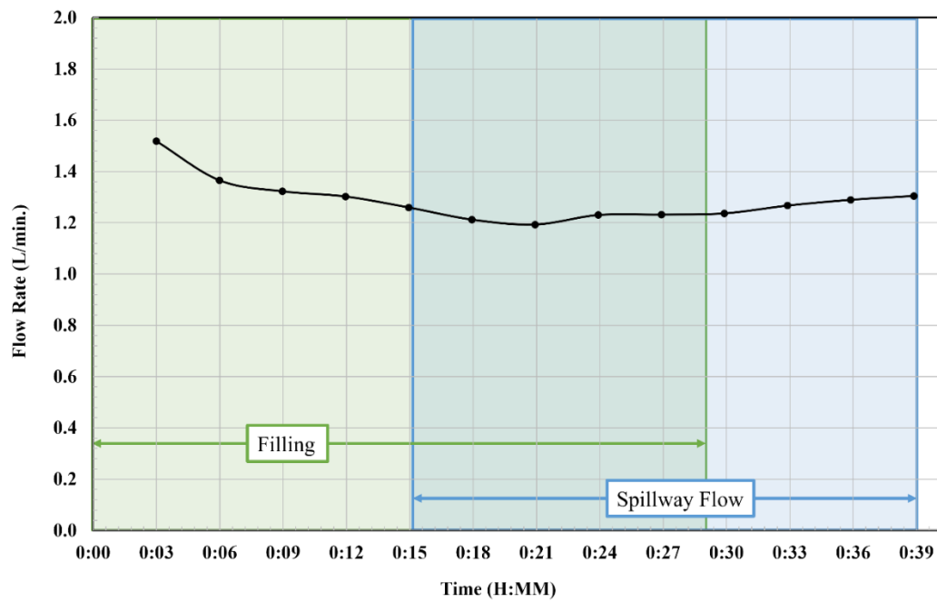
(a) skimmer flow rate versus time
