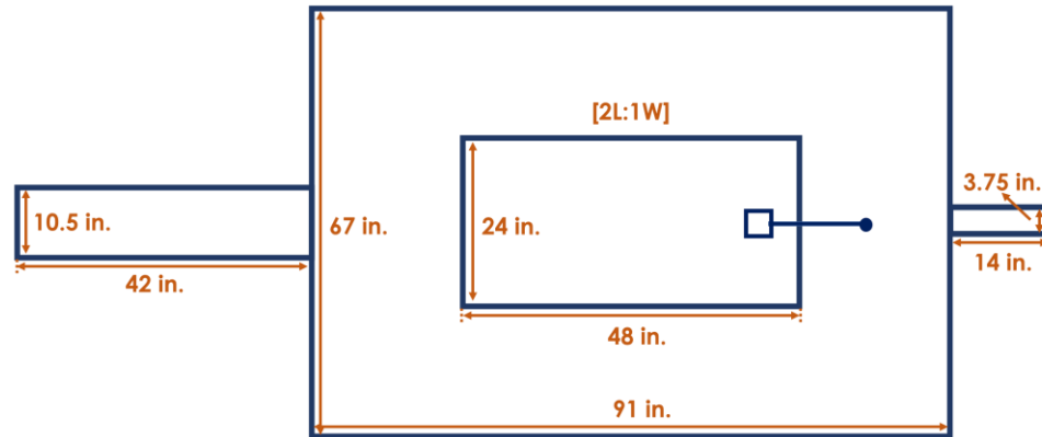
(a) standard basin dimensions
