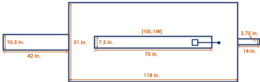
(b) in-channel basin dimensions
