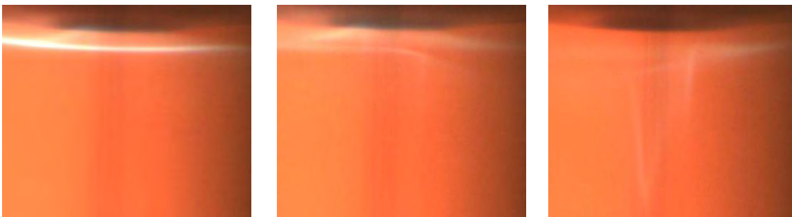
Figure 2-6: Images of 99% hexadecane droplets undergoing combustion in air at 800 °C
