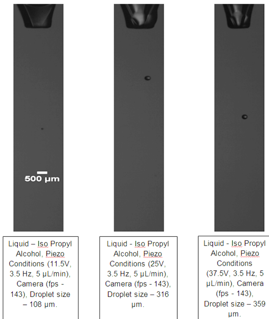
Figure 2-25: Isopropyl Alcohol microdroplet generation at different voltages
