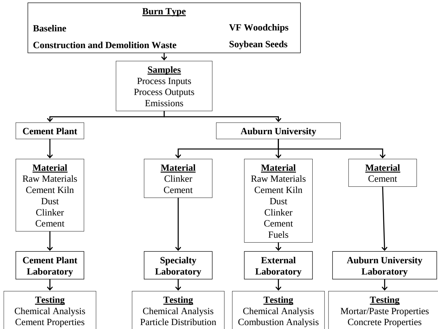
Figure 5-1: Analysis Plan
