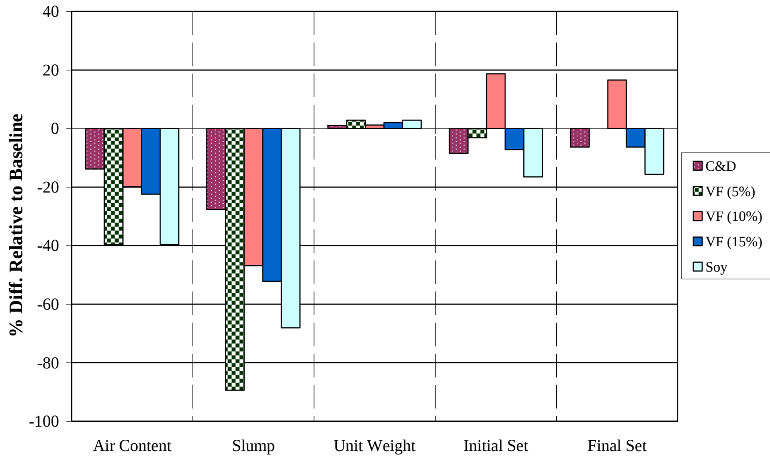
Figure 5-20: AUR – Percent Difference in Physical Properties Relative to Baseline for Mix 0.37 Concrete for Trial Burn
