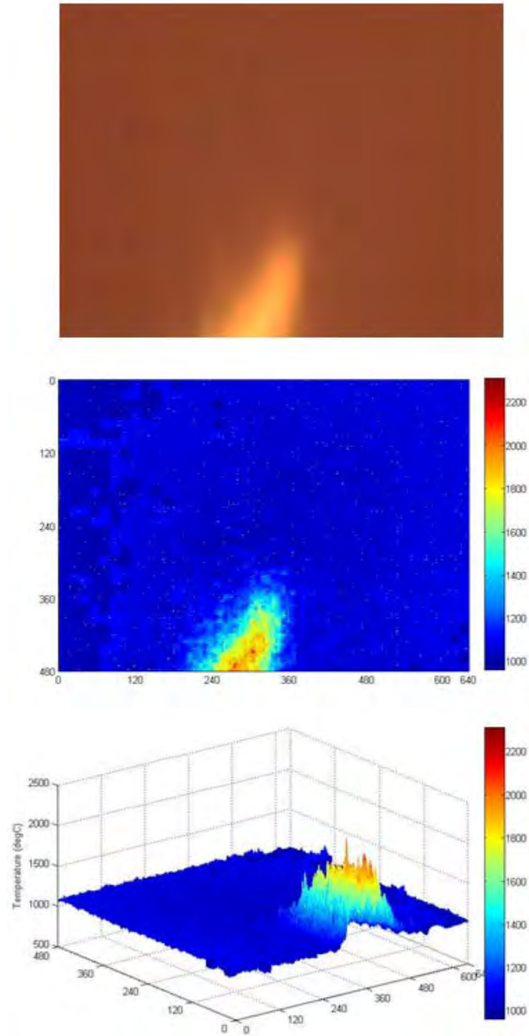
Figure 2-10: Wood combustion image and surface temperature estimates at 900 °C in air
