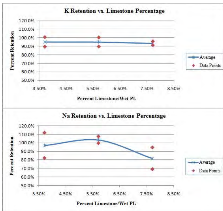
Figure 10-33: Alkali Retention vs. Limestone Percentage
