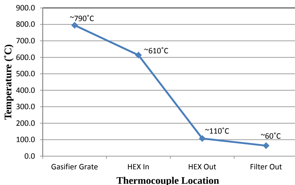
Figure 9-7: Average temperature of the syngas at different locations in the system starting at gasifier exit, proceeding through the heat exchanger (HEX), and finally after the filter
