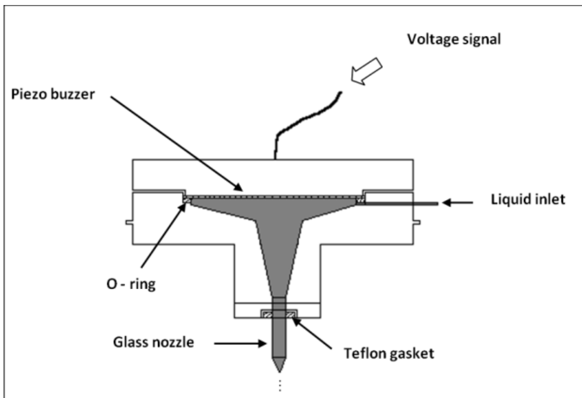
Figure 2-19: Detailed view of piezoelectric droplet generator
