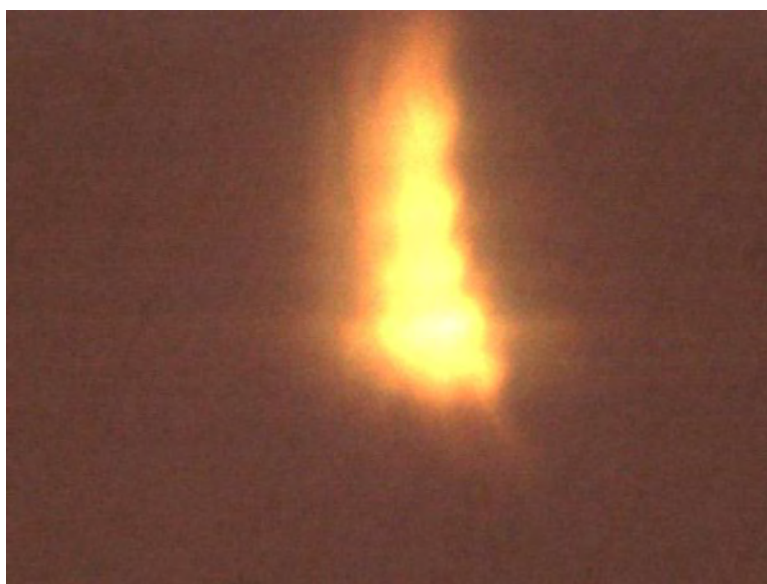
Figure 2-3: Wood at 900 °C in air (100 micrometer nominal particle)
