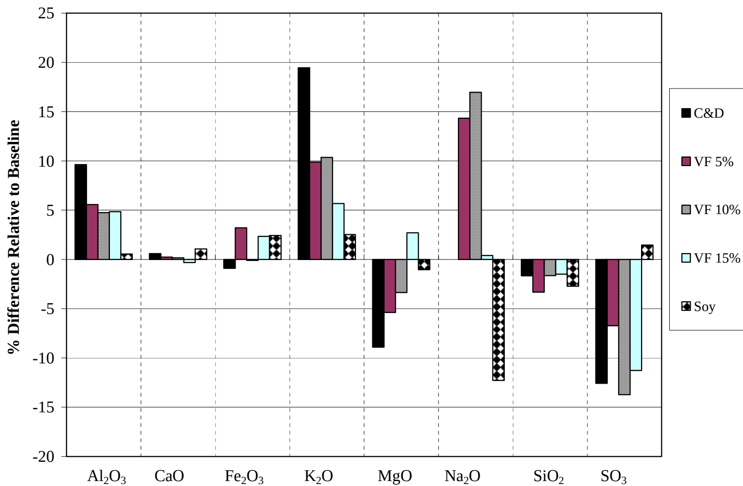
Figure 5-9: CPR – Percent Difference of Cement Composition Relative to Baseline
