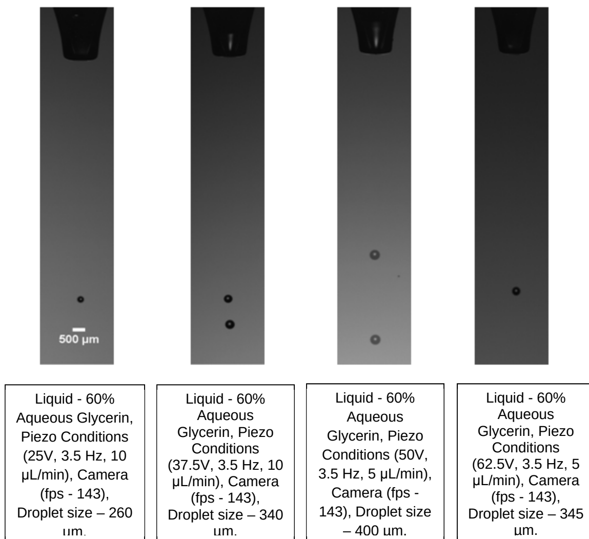
Figure 2-23: 60% aqueous glycerin microdroplet generation at different voltages
