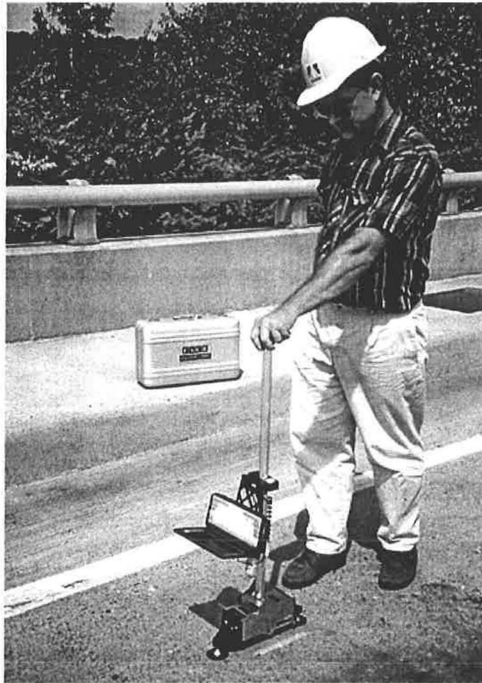
Figure 2.5 - Face Technologies Rolling Dipstick
