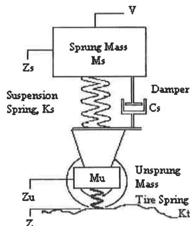
Figure 2.1 - Quarter-car Model
