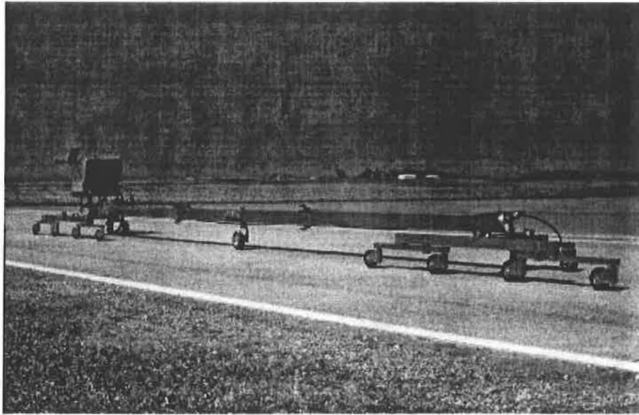
Figure 2.3 - Ames Model 4000 Profilograph
