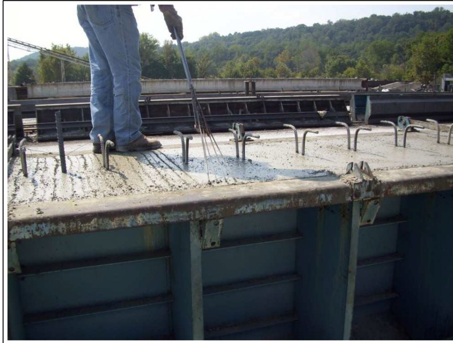
Figure 3.10: Application of transverse, top-surface roughening with a metal rake
