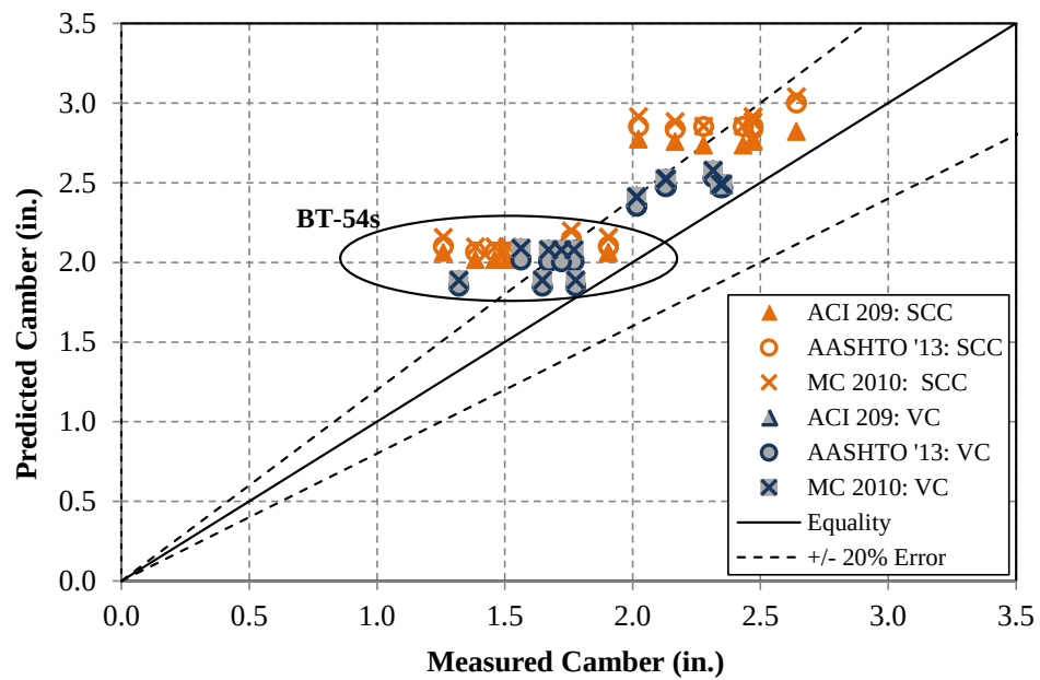
Figure 6.16: Comparison of measured and predicted cambers at fifty-six days
