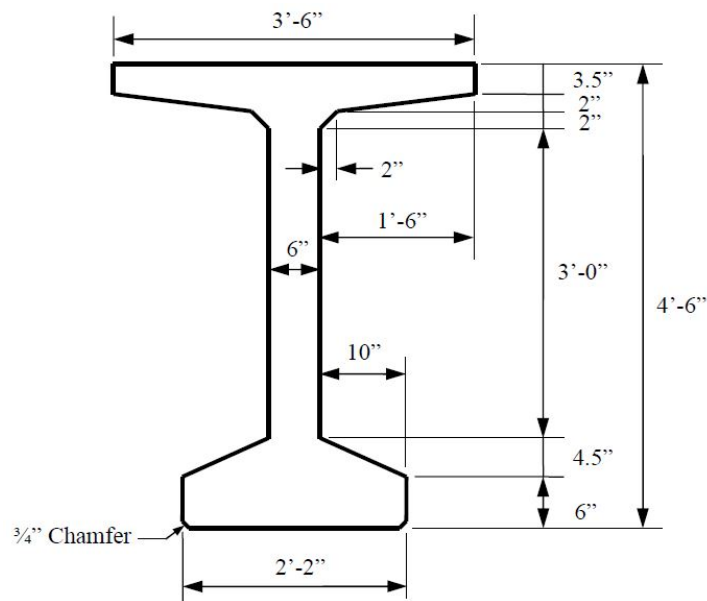
Figure 3.3: Typical BT-54 girder cross-sectional dimensions
