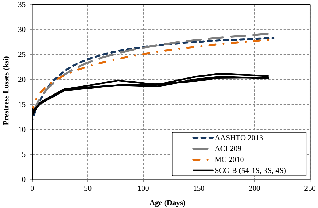
Figure 6.12: Sample comparison of predicted prestress losses in SCC BT-54s
