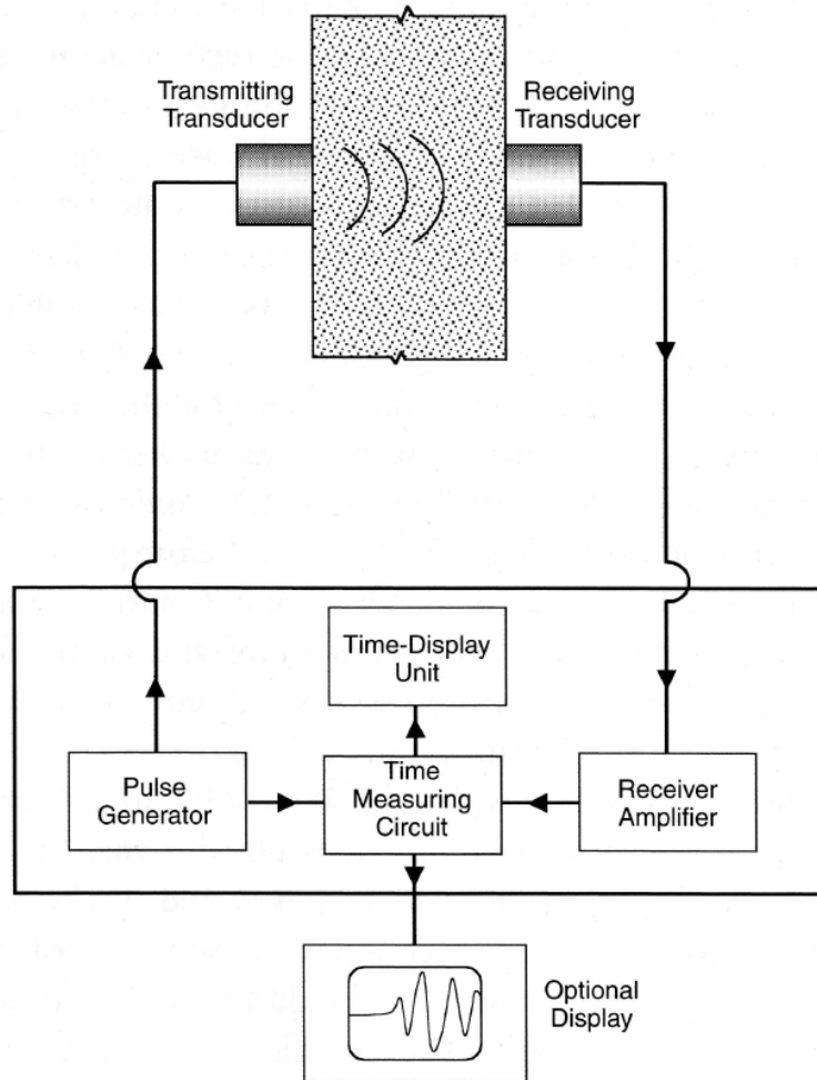
Figure 2.9: Ultrasonic pulse velocity testing equipment (Naik et al. 2004)
