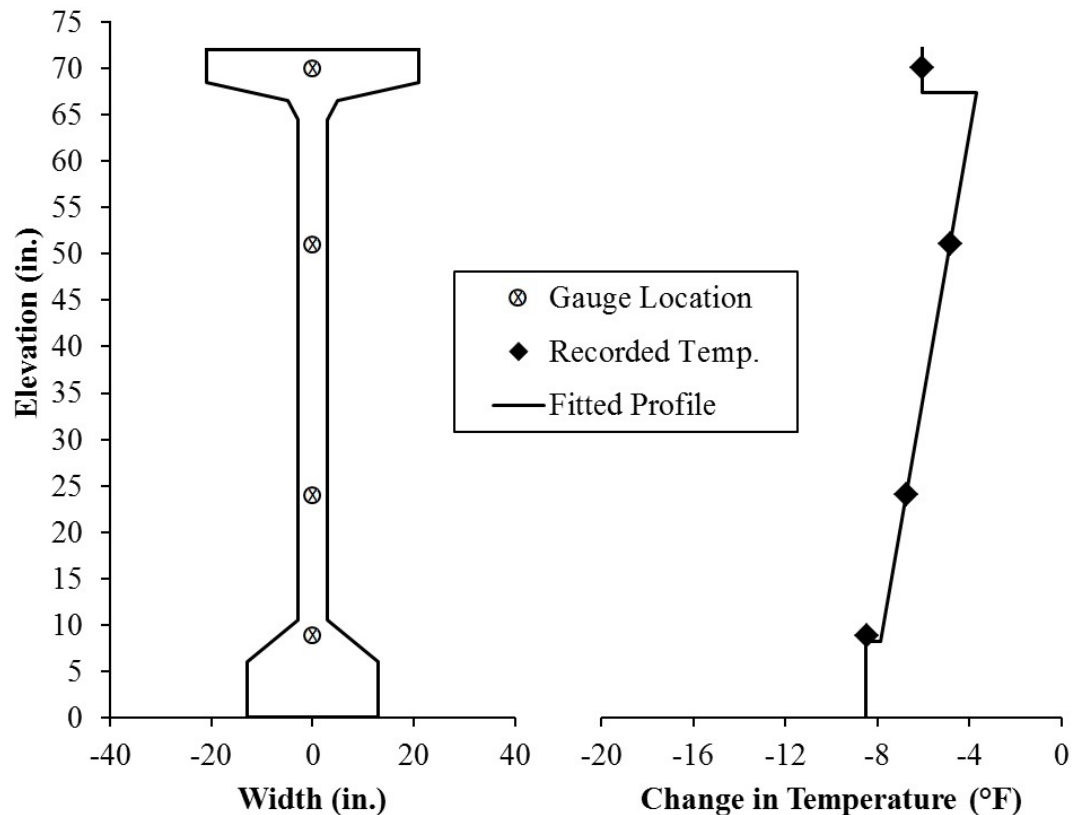
Figure 6.4: Example of idealized thermal gradient profile in BT-72
