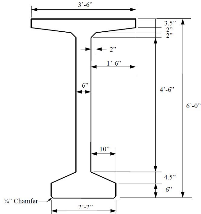
Figure 3.4: Typical BT-72 girder cross-sectional dimensions
