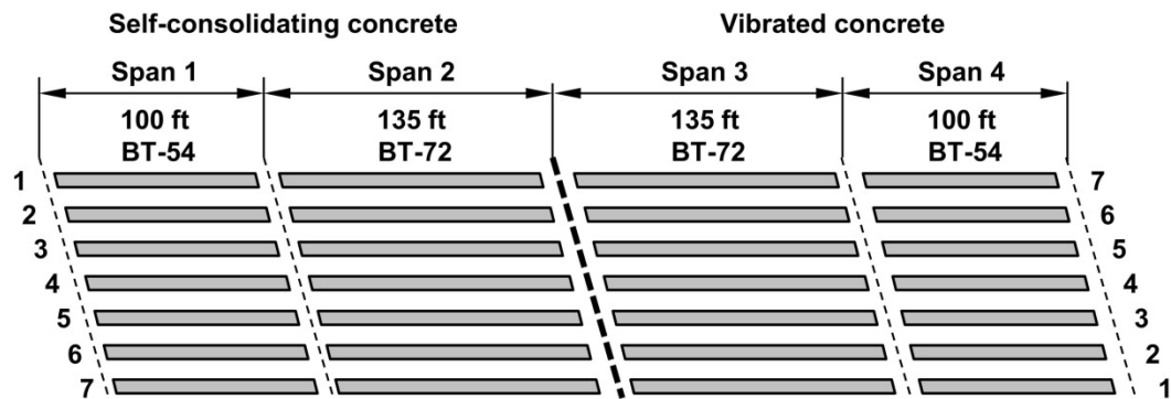
Figure 3.2: SCC and VC girders placed in the bridge over Hillabee Creek
