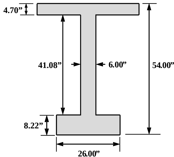
Figure 6.2: Simplified BT-54 composite section
