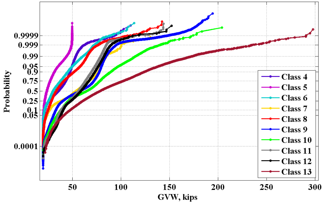
Figure 25: CDF's of GVW for vehicle classes 4-13 for 965 (Shorter)
