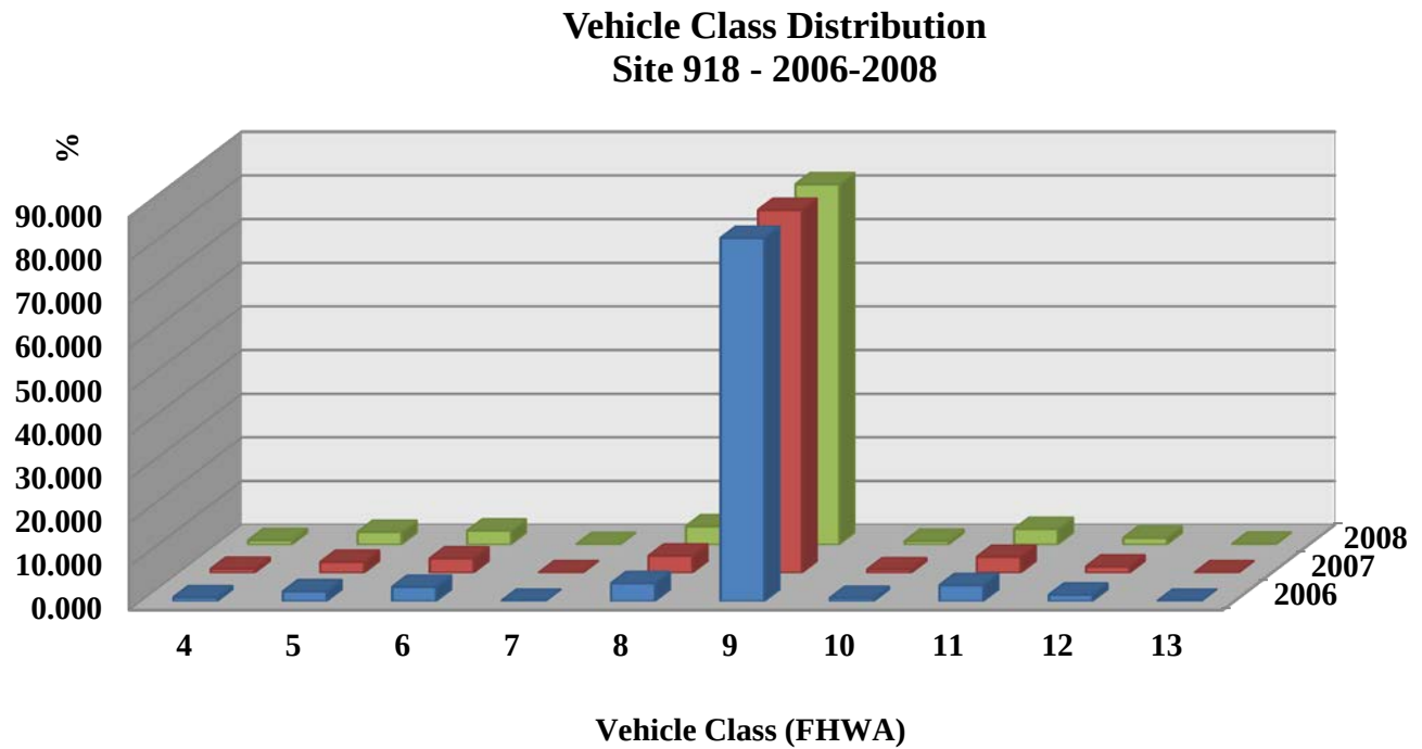
Figure 6: Percentage of vehicles in each class for location 918(Bucksville)
