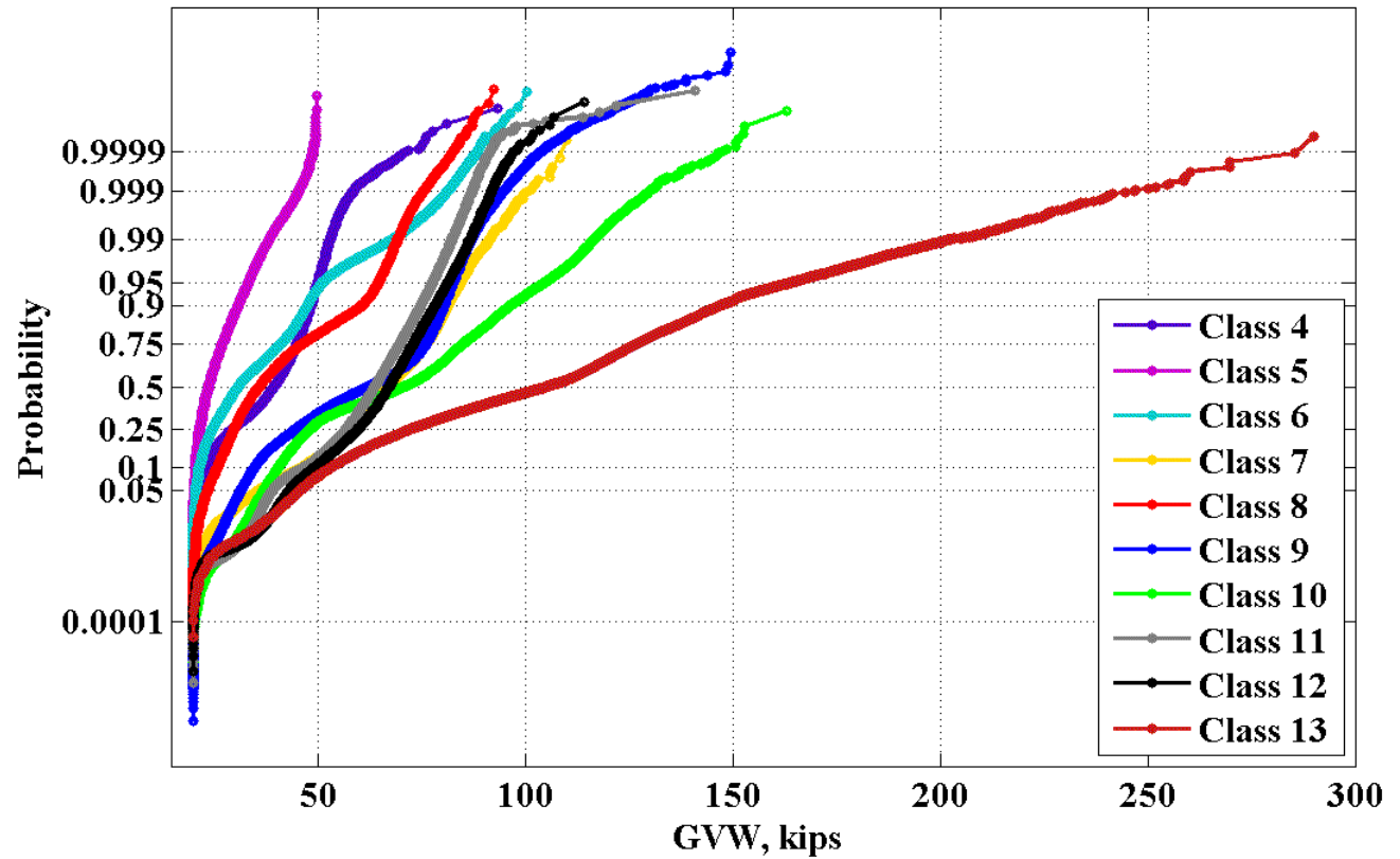
Figure 7: CDF's of GVW for vehicle classes 4-13 for 918 (Bucksville)
