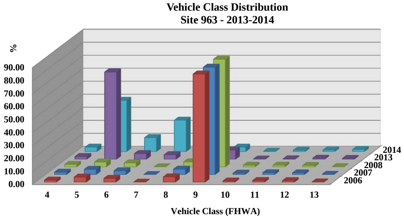
Figure 20: Percentage of vehicles in each class for location 963(Grand Bay)
