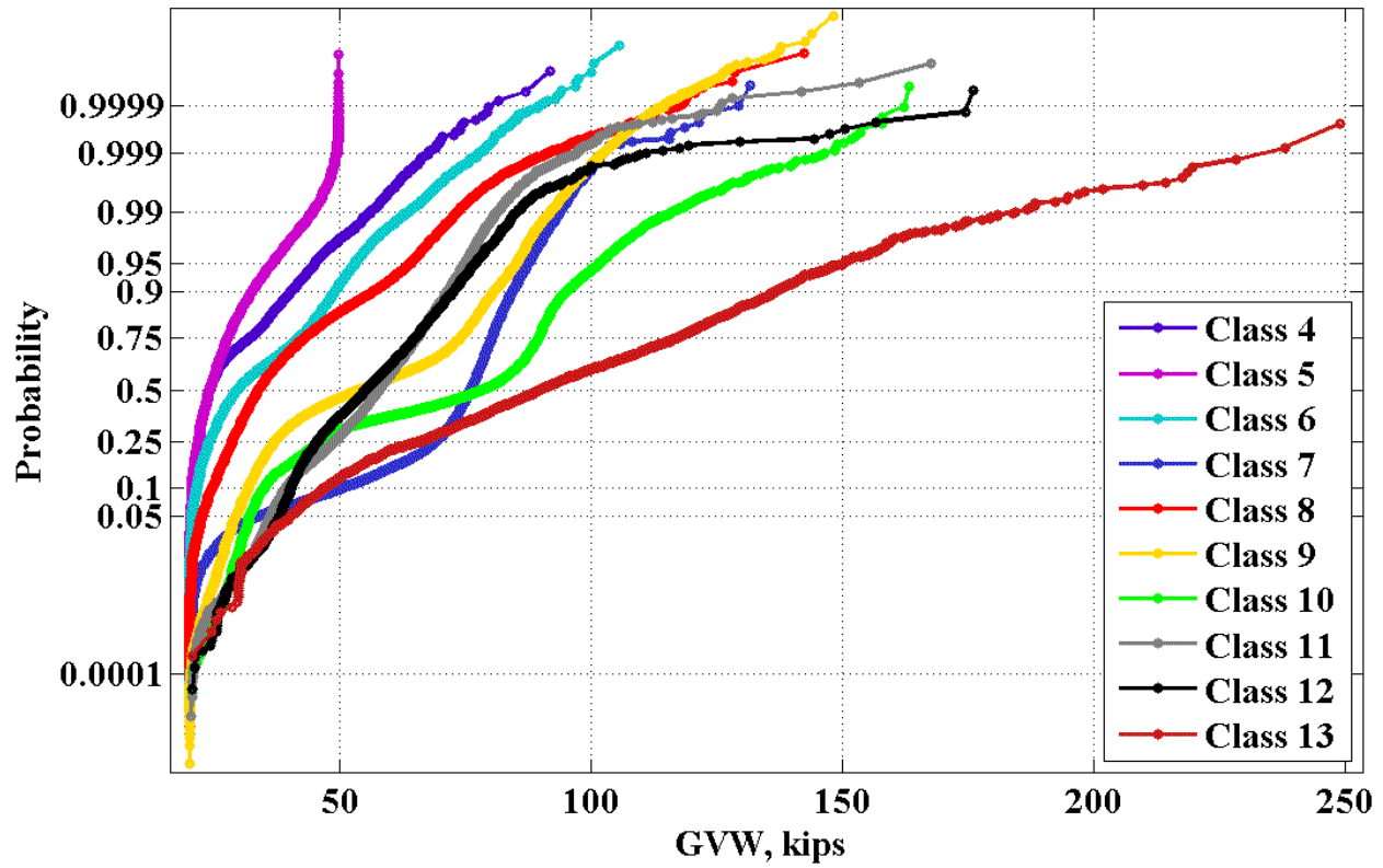
Figure 3: CDF's of GVW for vehicle classes 4-13 for 911 (Alex City)
