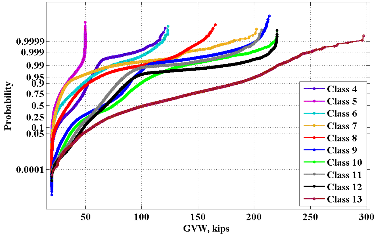
Figure 21: CDF's of GVW for vehicle classes 4-13 for 963(Grand Bay)
