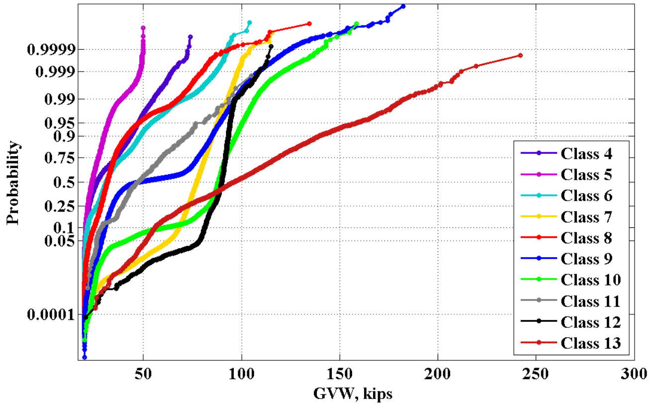
Figure 5: CDF's of GVW for vehicle classes 4-13 for 915 (Sunflower)
