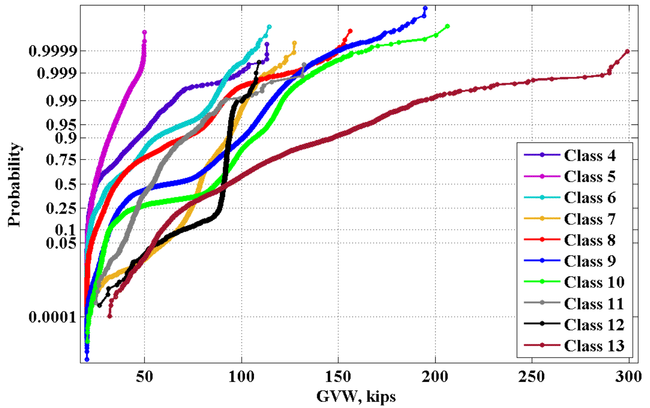
Figure 17: CDF's of GVW for vehicle classes 4-13 for 960(Whatley)
