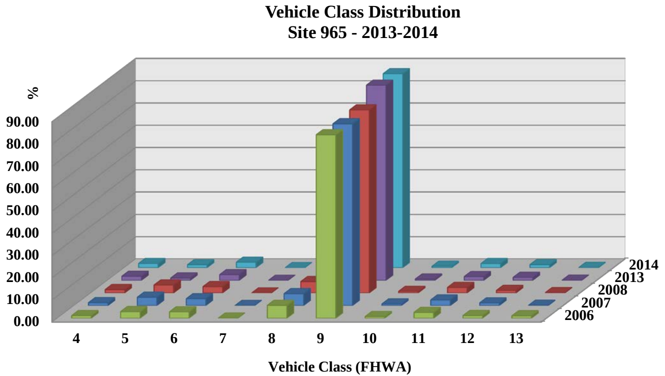
Figure 24: Percentage of vehicles in each class for location 965 (Shorter)
