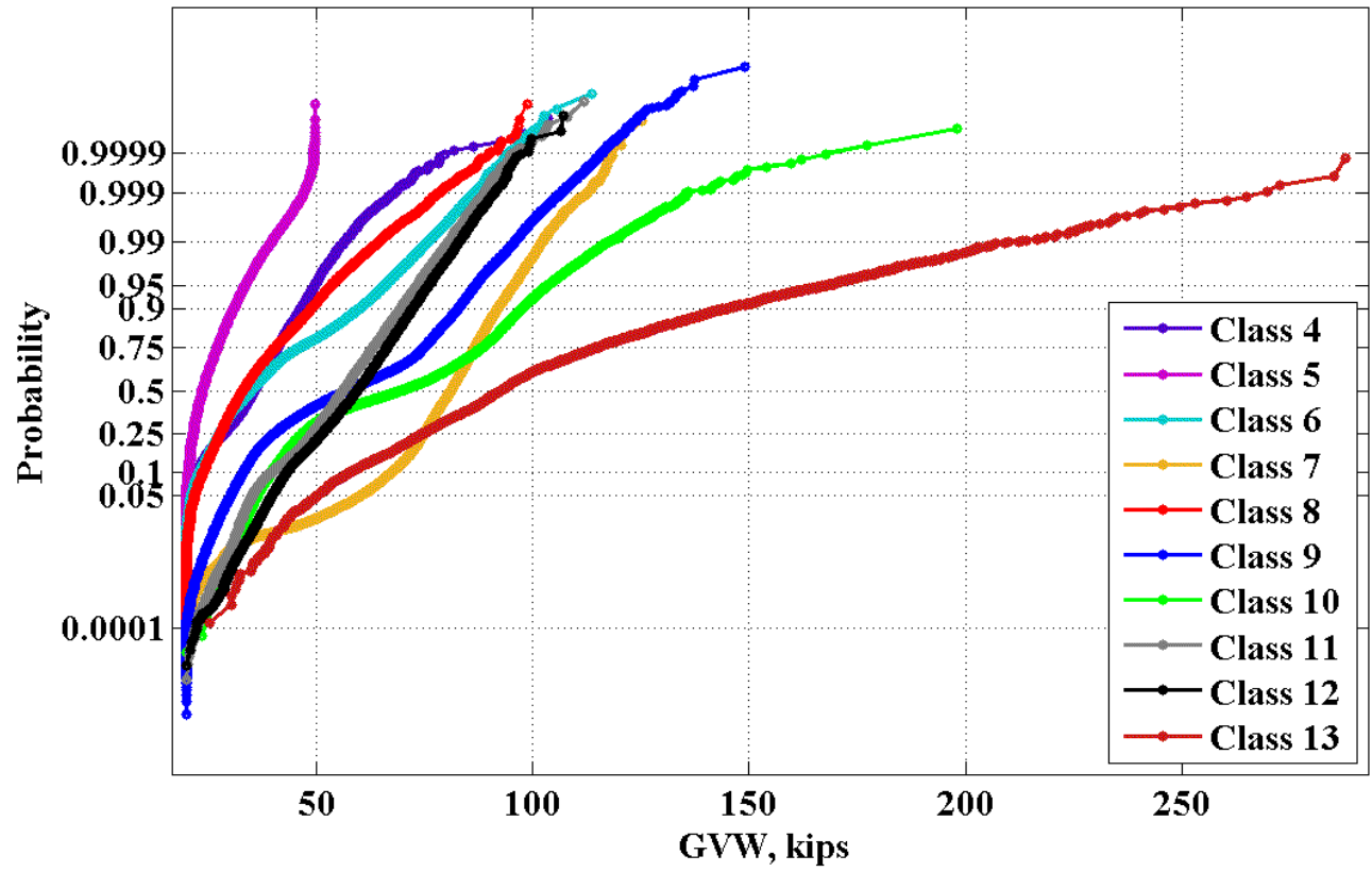
Figure 13: CDF's of GVW for vehicle classes 4-13 for 934(Sumiton)
