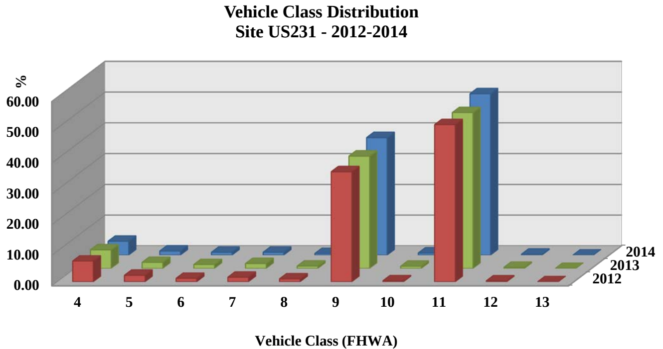
Figure 26: Percentage of vehicles in each class for location US-231
