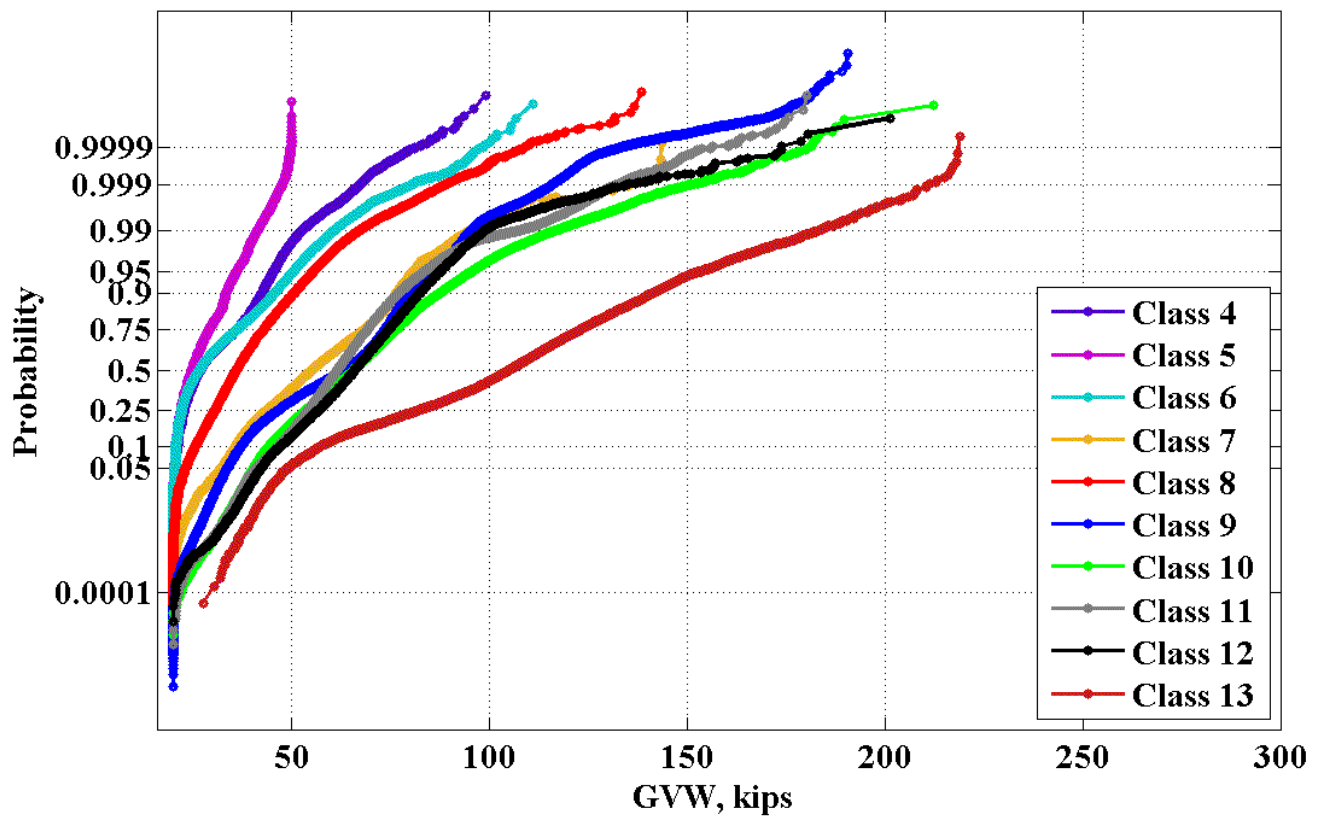
Figure 9: CDF's of GVW for vehicle classes 4-13 for 931 (Athens)
