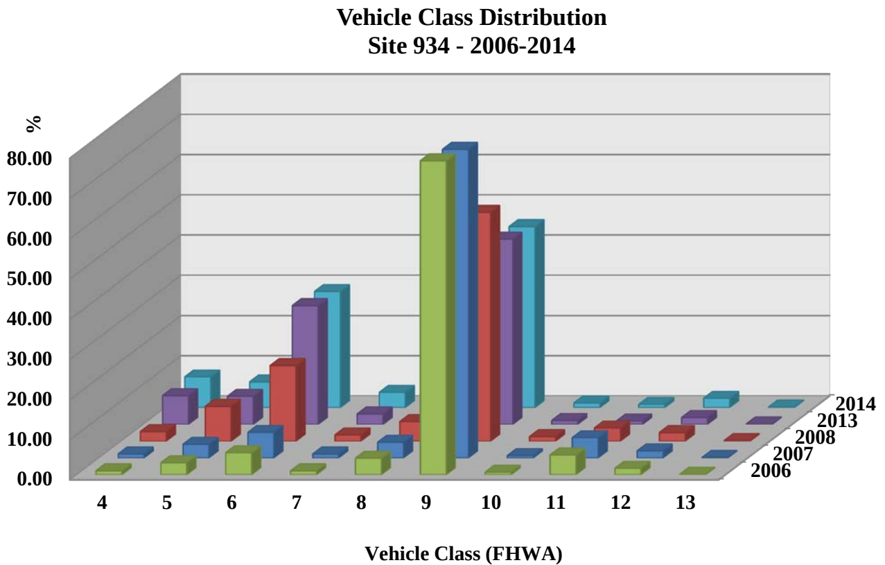
Figure 12 : Percentage of vehicles in each class for location 934(Sumiton)
