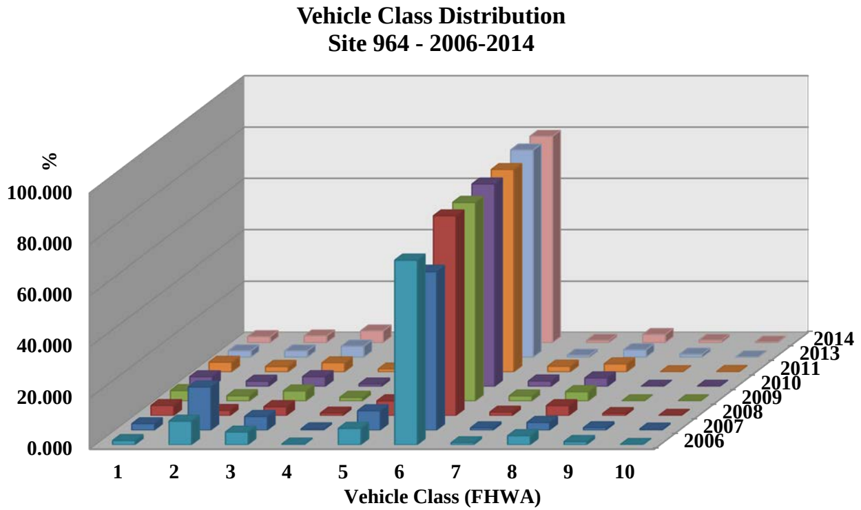
Figure 22: Percentage of vehicles in each class for location 964(Ozark)
