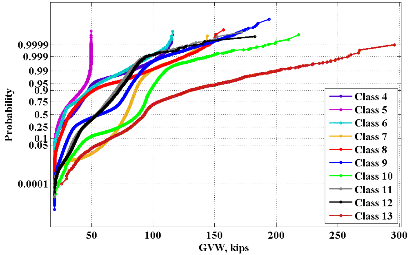
Figure 15: CDF's of GVW for vehicle classes 4-13 for 942(Pine Level)
