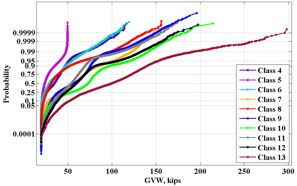
Figure 19: CDF's of GVW for vehicle classes 4-13 for 961(Mobile)
