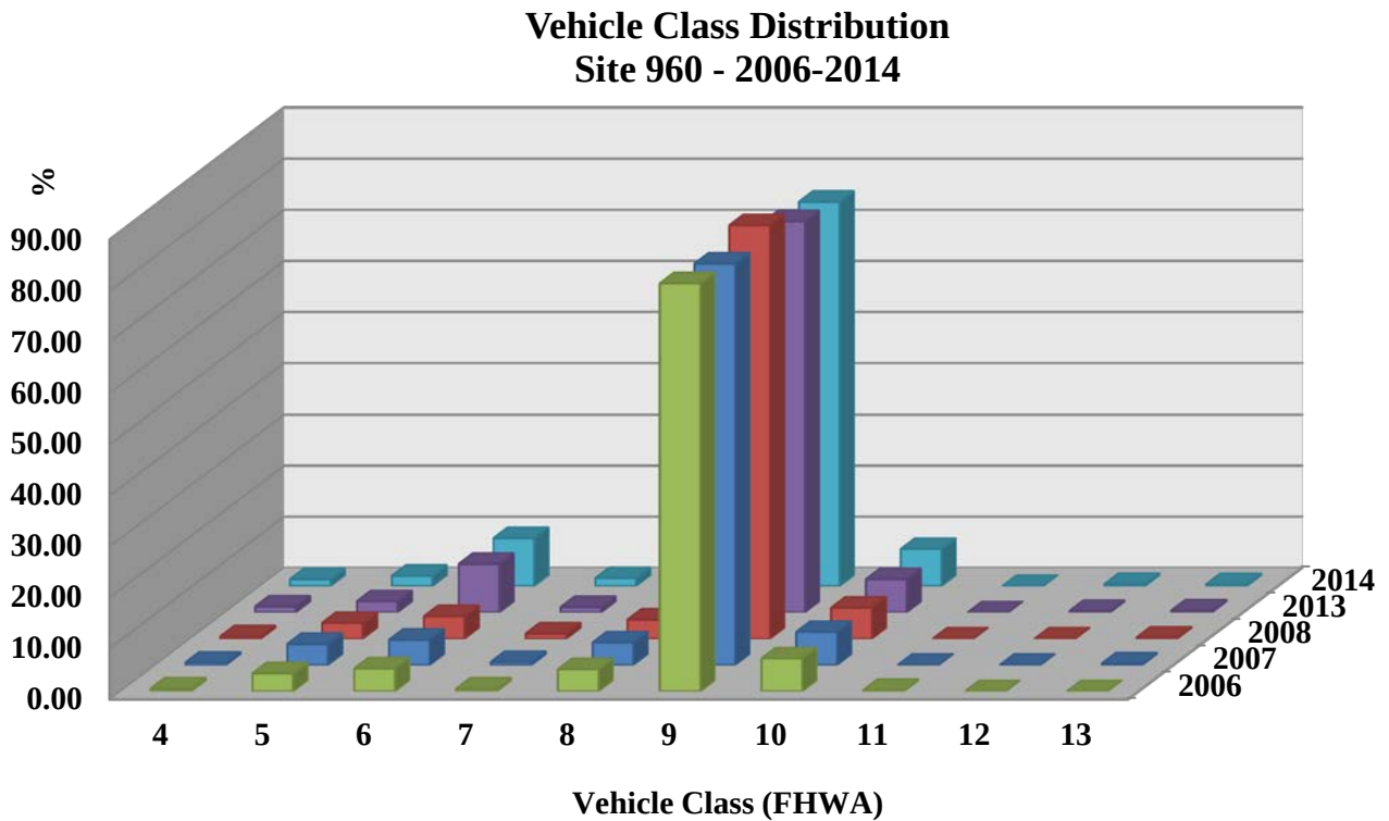
Figure 16: Percentage of vehicles in each class for location 960(Whatley)
