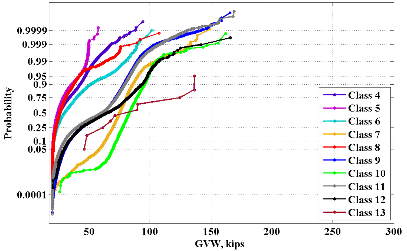
Figure 27: CDF's of GVW for vehicle classes 4-13 for 965 (Shorter)
