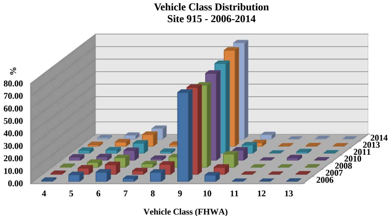
Figure 4: Percentage of each vehicle class for location 915(Sunflower)
