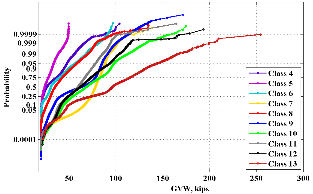
Figure 23: CDF's of GVW for vehicle classes 4-13 for 964(Ozark)
