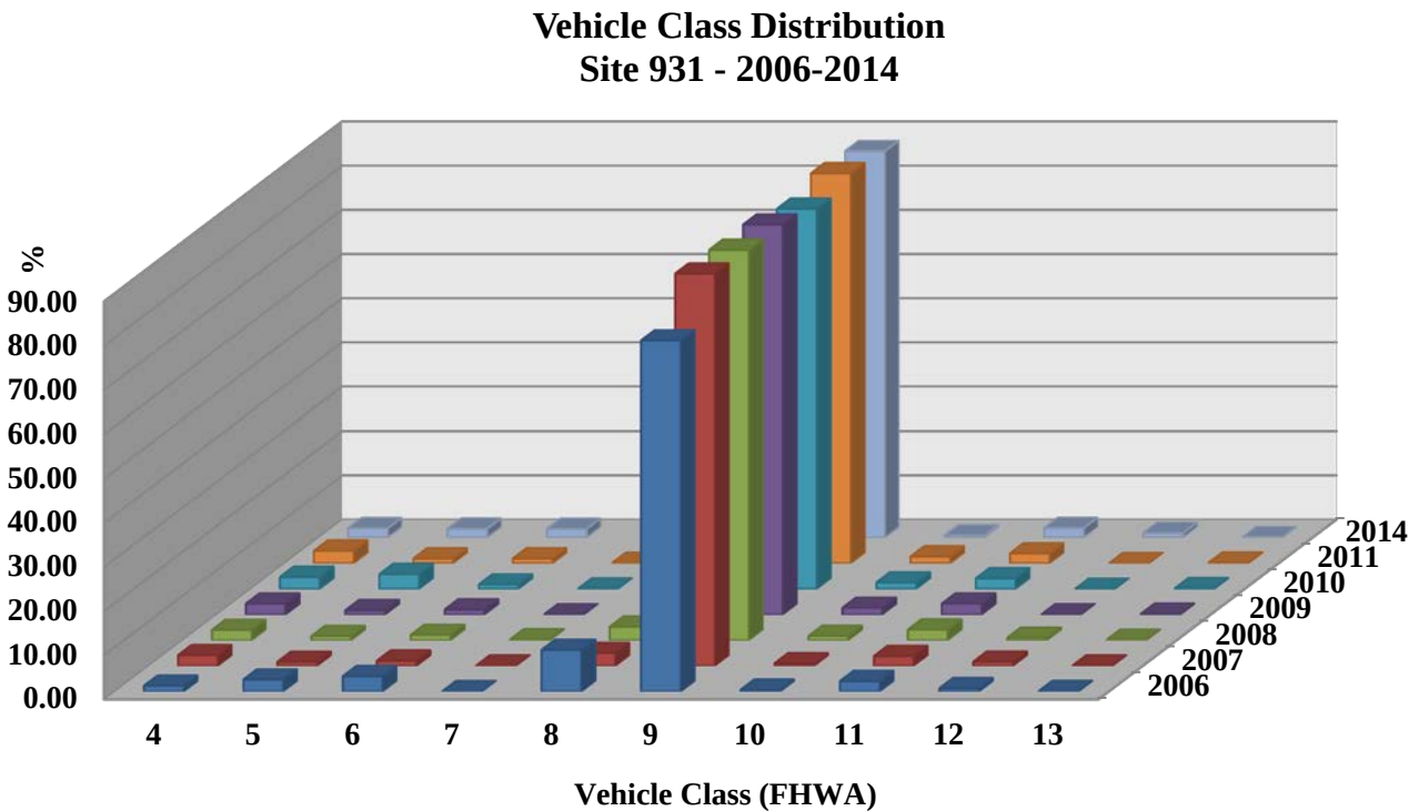
Figure 8: Percentage of vehicles in each class for location 931(Athens)
