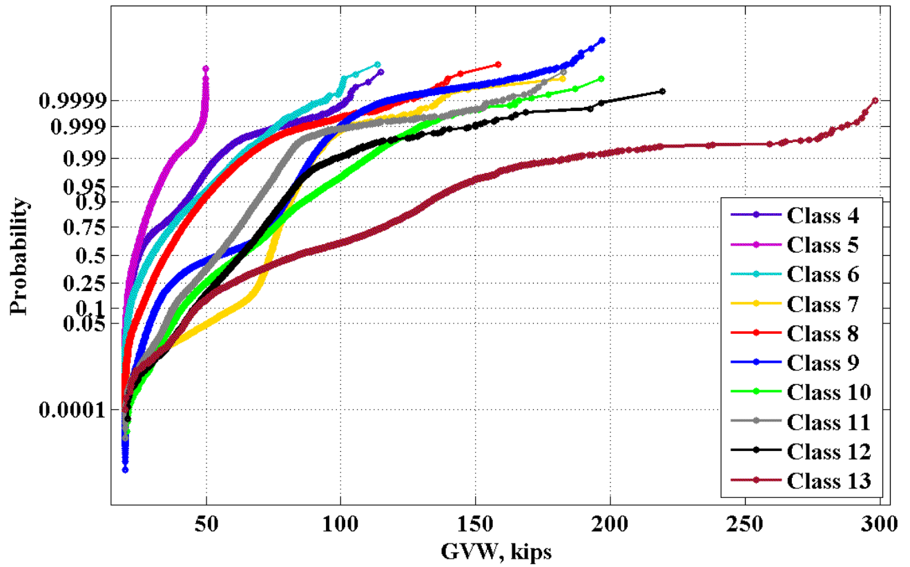
Figure 11: CDF's of GVW for vehicle classes 4-13 for 933 (Muscle Shoals)
