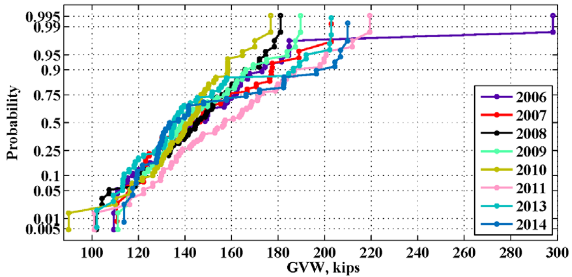
Figure 45: Maximum weekly GVW for the location 933(Muscle Shoals) – 2006-2014
