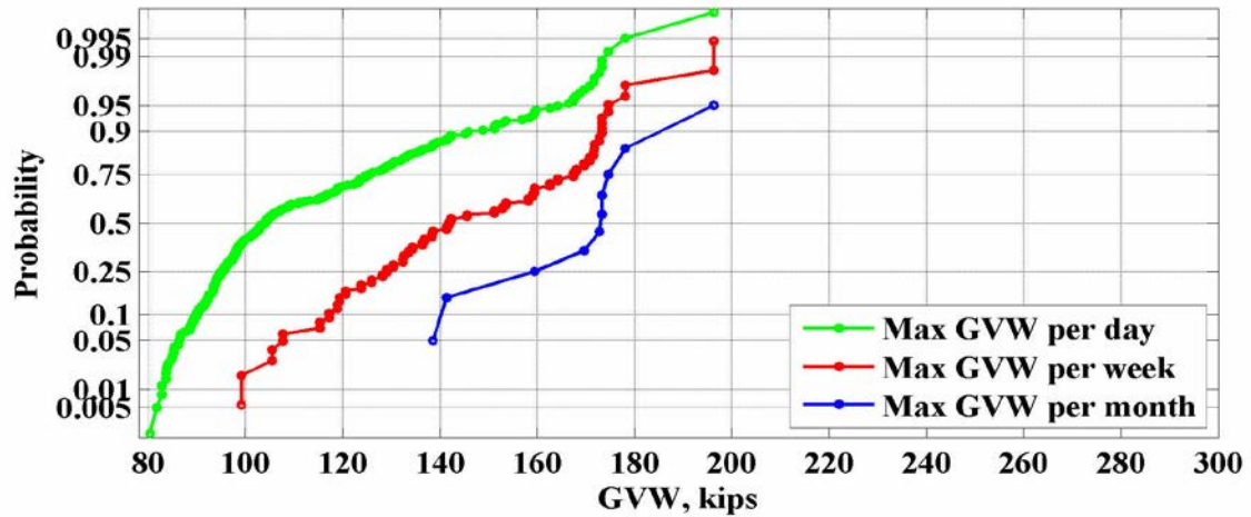
Figure 58: Maximum values of GVW for the location 942(Pine Level) – 2013
