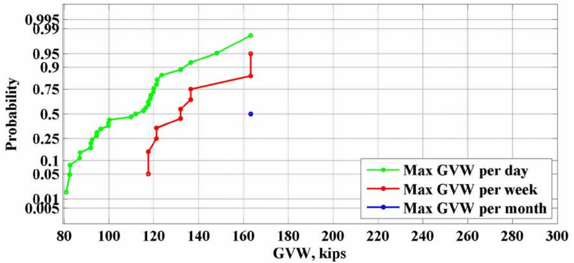
Figure 101: Maximum values of GVW for the location 965(Shorter) – 2013
