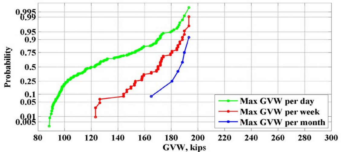
Figure 67: Maximum values of GVW for the location 960(Whatley) – 2014
