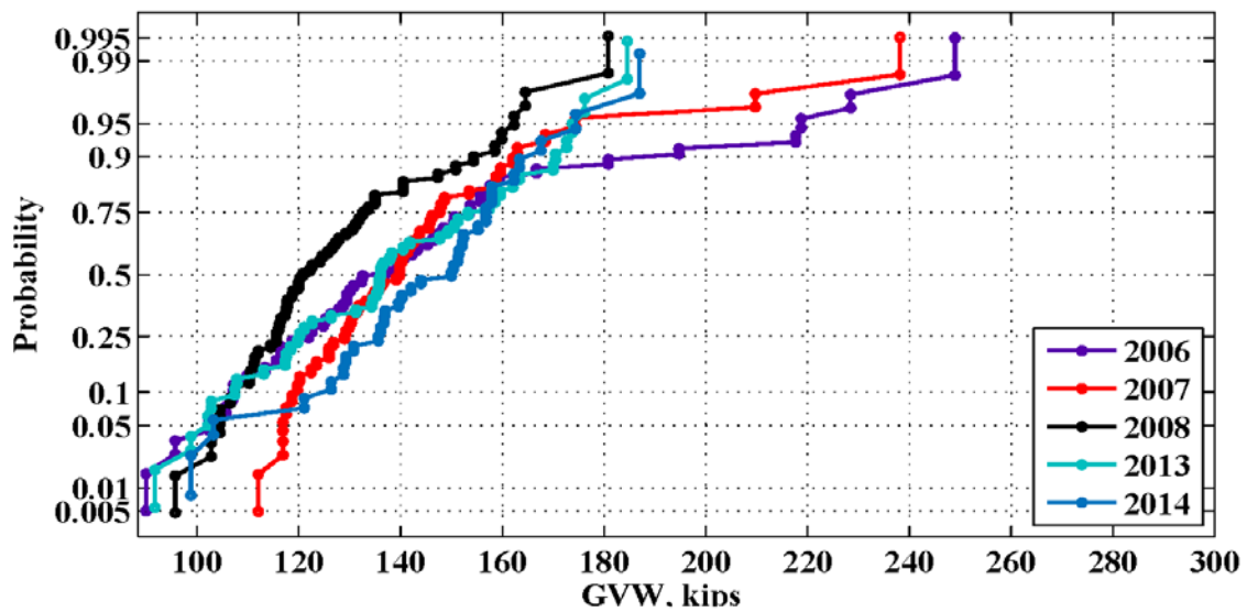
Figure 7: Maximum weekly GVW for the location 911(Alex City) – 2006-2014
