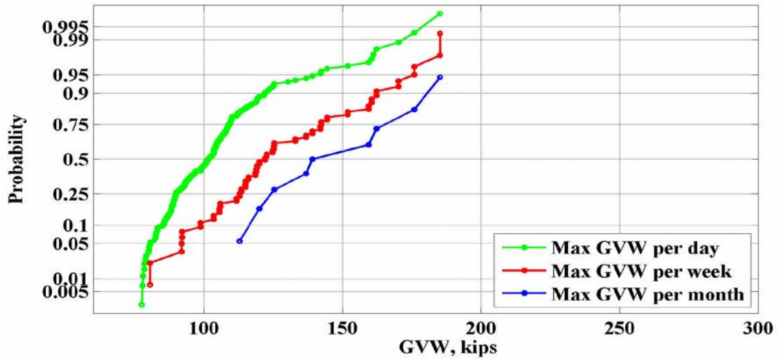
Figure 50: Maximum values of GVW for the location 934(Sumiton) – 2013
