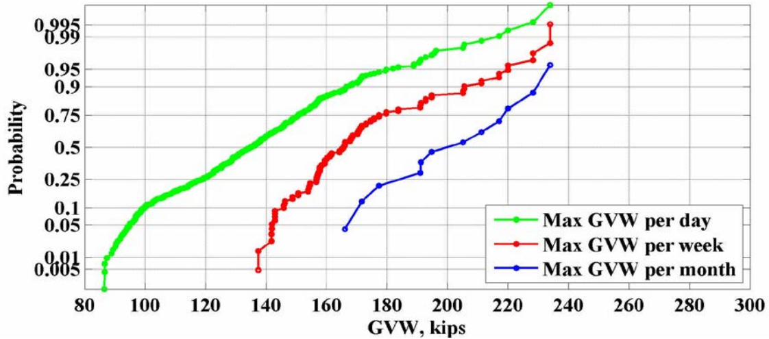
Figure 98: Maximum values of GVW for the location 965(Shorter) – 2006
