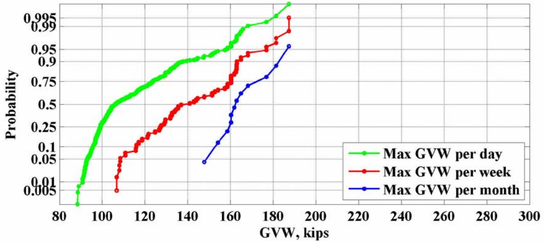
Figure 90: Maximum values of GVW for the location 964(Ozark) – 2009
