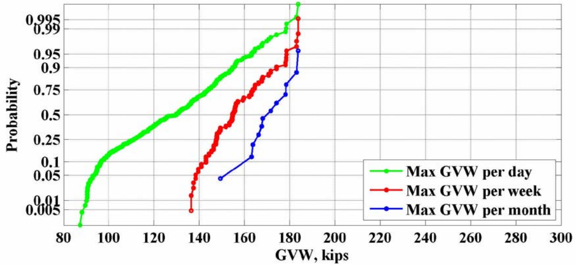
Figure 29: Maximum values of GVW for the location 931(Athens) – 2009
