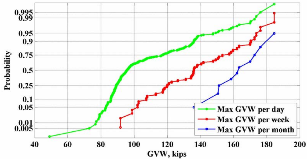
Figure 4: Maximum values of GVW for the location 911(Alex City) – 2013
