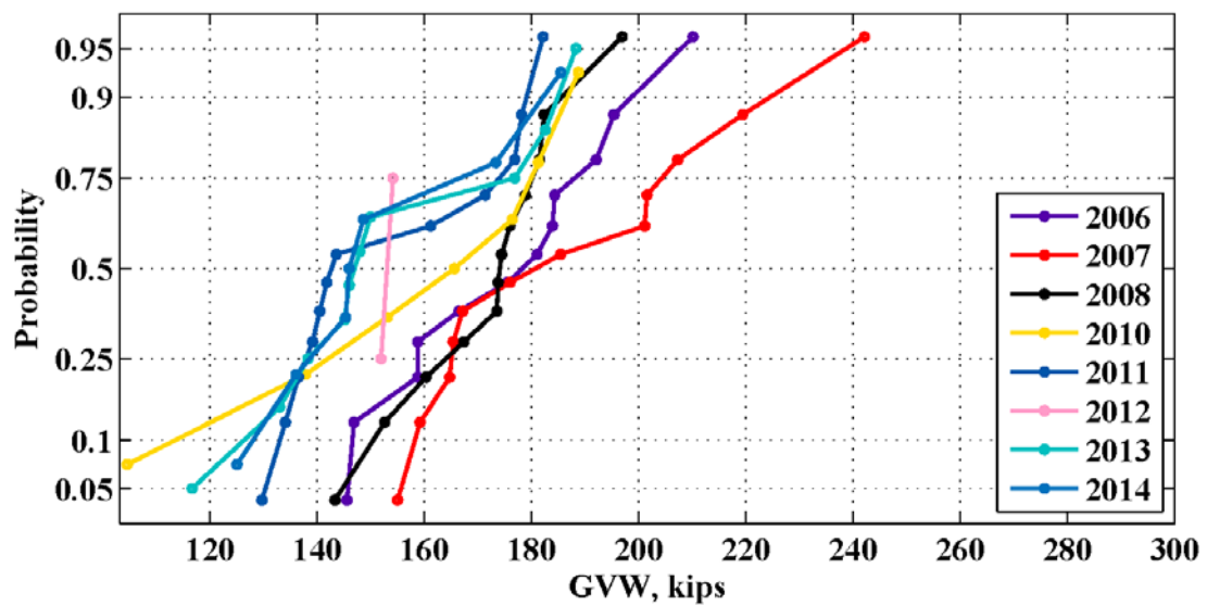
Figure 19: Maximum monthly GVW for the location 915(Sunflower) – 2006-2014
