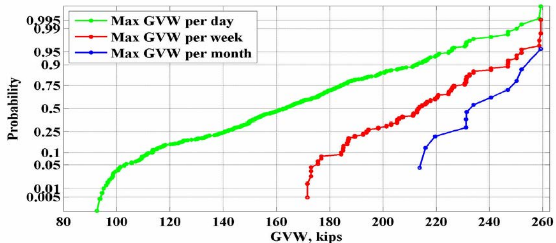
Figure 22: Maximum values of GVW for the location 918(Bucksville) – 2008
