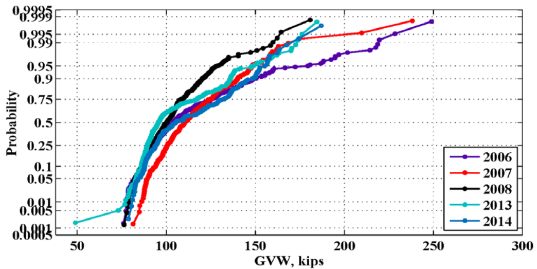
Figure 6: Maximum daily GVW for the location 911(Alex City) – 2006-2014
