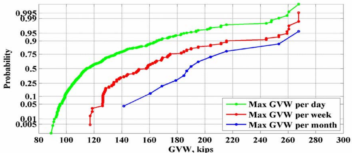
Figure 56: Maximum values of GVW for the location 942(Pine Level) – 2007
