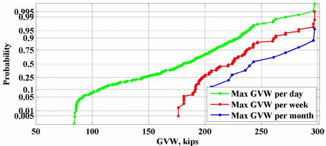
Figure 80: Maximum values of GVW for the location 963(Grand Bay) – 2007
