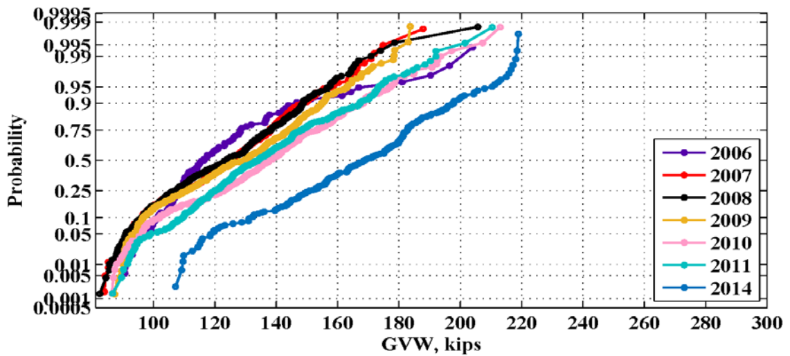
Figure 33: Maximum daily GVW for the location 931(Athens) – 2006-2014
