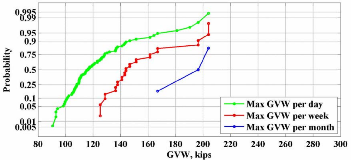
Figure 26: Maximum values of GVW for the location 931(Athens) – 2006
