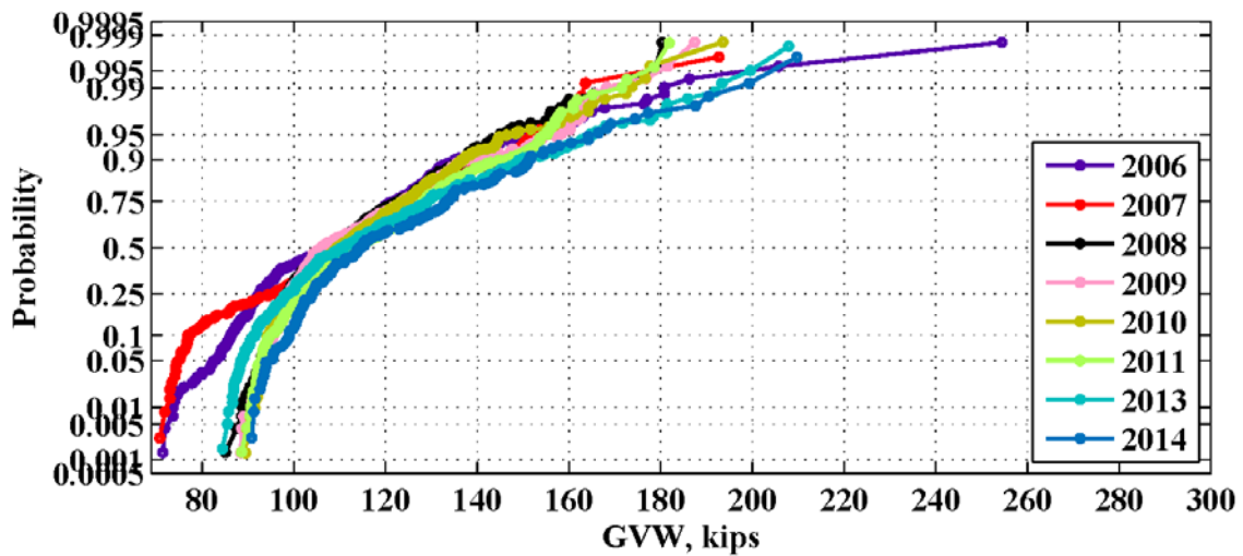
Figure 95: Maximum daily GVW for the location 964(Ozark) – 2006-2014
