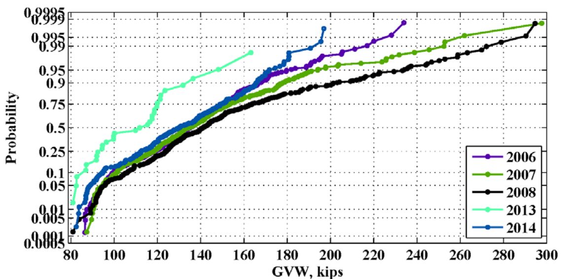
Figure 103: Maximum daily GVW for the location 965(Shorter) – 2006-2014
