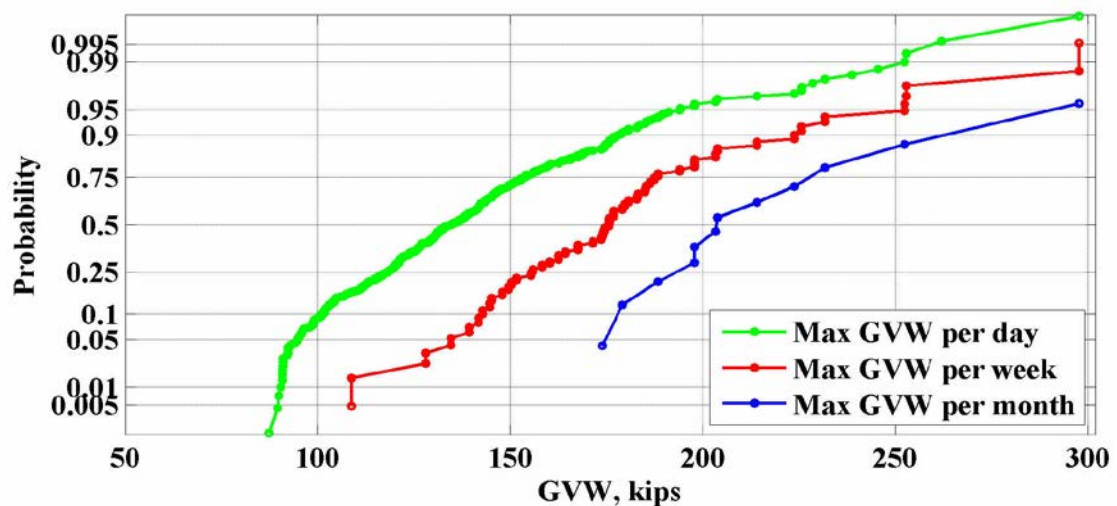
Figure 99: Maximum values of GVW for the location 965(Shorter) – 2007
