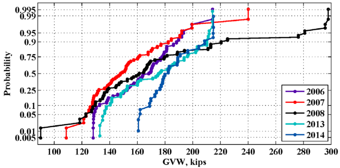
Figure 77: Maximum weekly GVW for the location 961(Mobile) – 2006-2014
