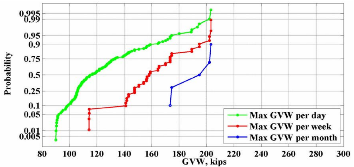
Figure 59: Maximum values of GVW for the location 942(Pine Level) – 2014
