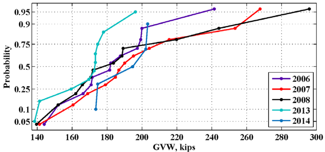
Figure 62: Maximum monthly GVW for the location 942(Pine Level) – 2006-2014
