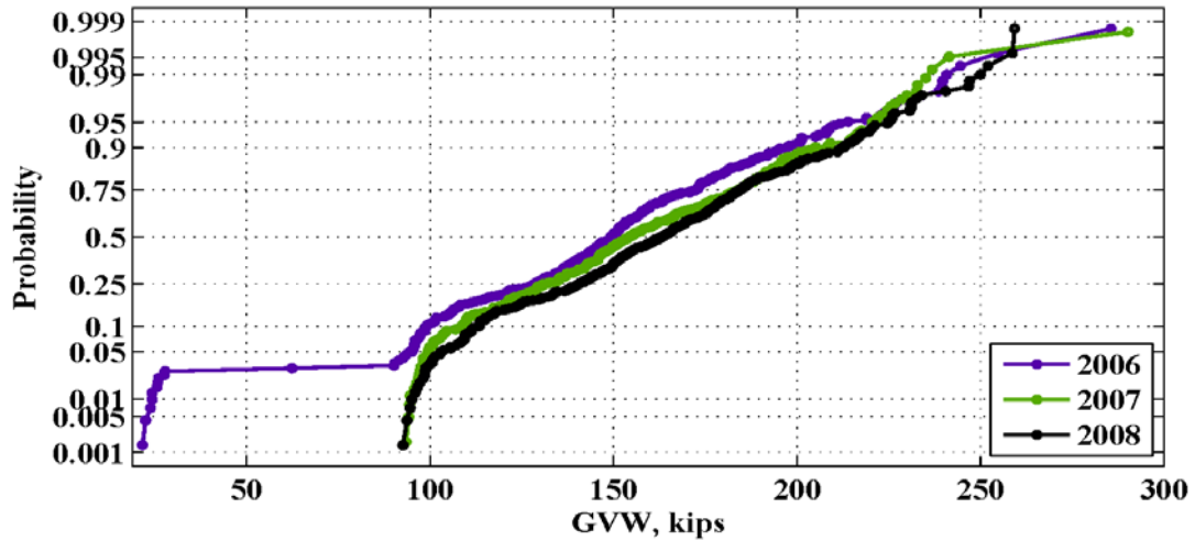
Figure 23: Maximum daily GVW for the location 915(Sunflower) – 2006-2014
