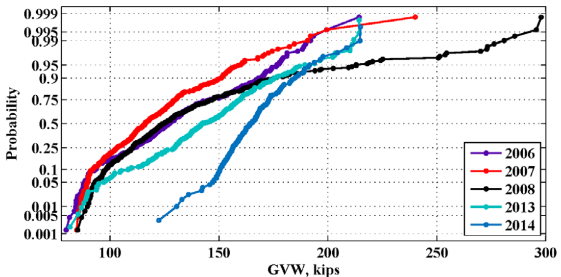
Figure 76: Maximum daily GVW for the location 961(Mobile) – 2006-2014
