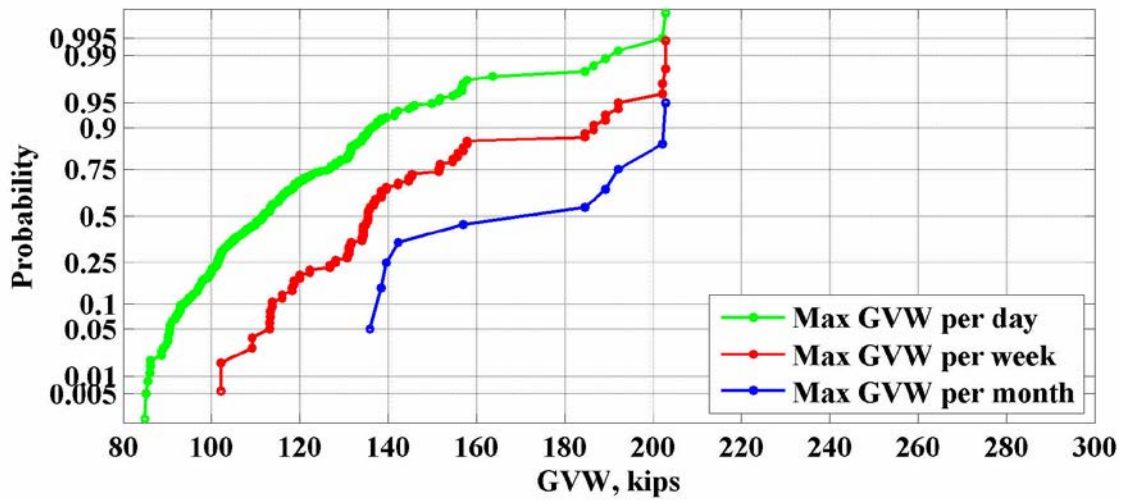
Figure 42: Maximum values of GVW for the location 933(Muscle Shoals)– 2013
