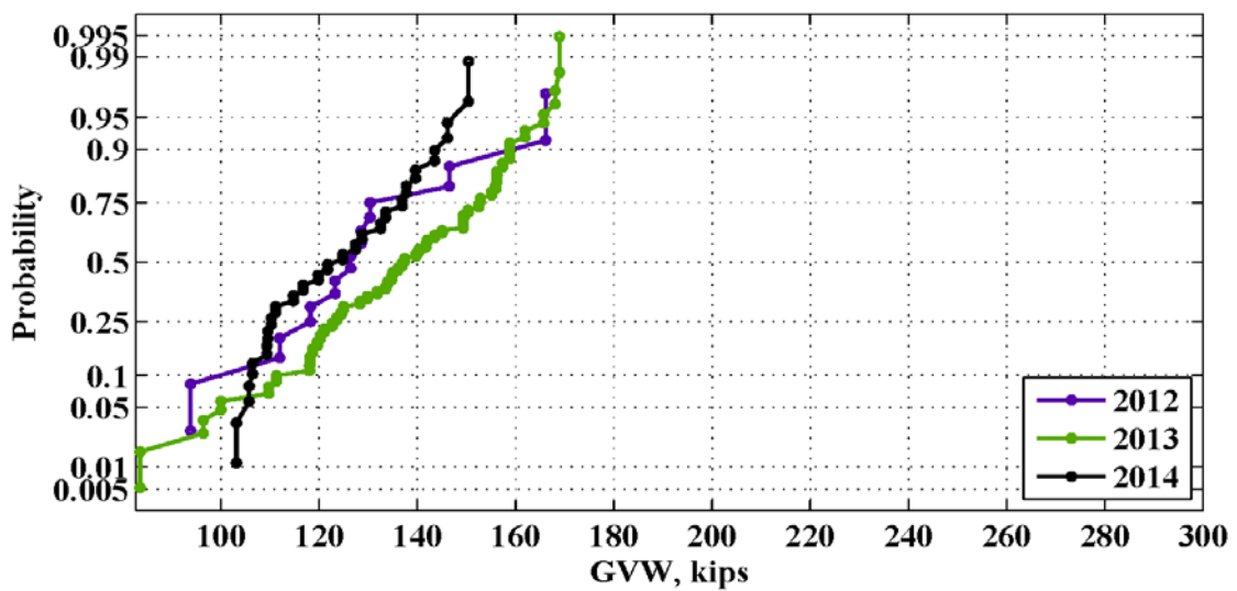
Figure 110: Maximum weekly GVW for the location US-231 – 2012-2014
