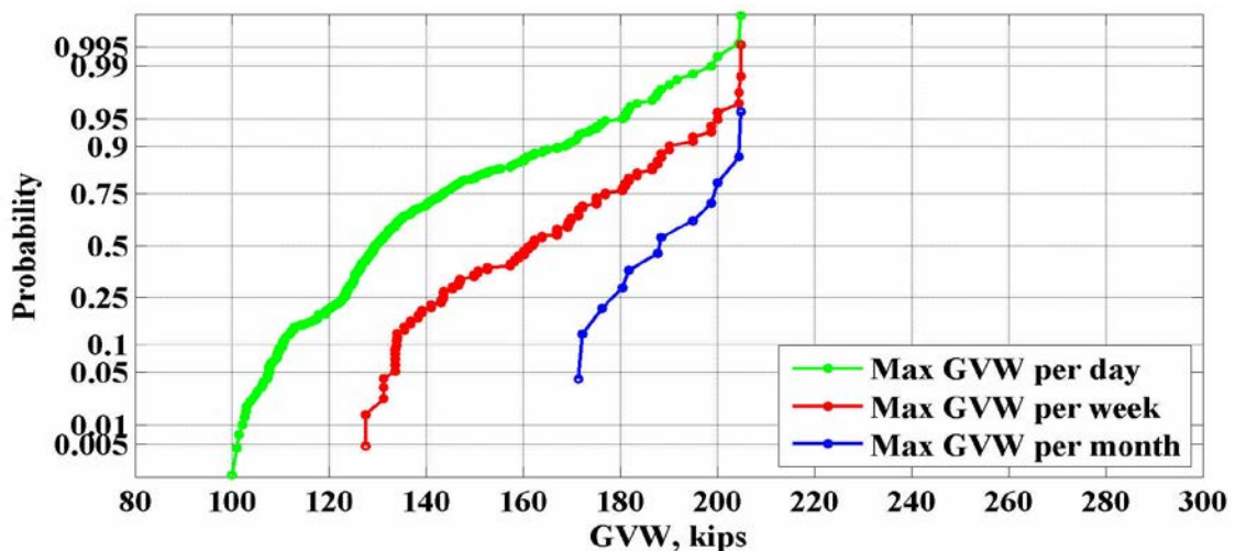
Figure 64: Maximum values of GVW for the location 960(Whatley) – 2007
