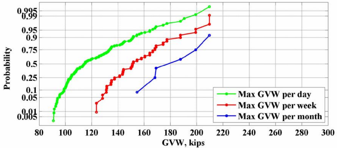
Figure 94: Maximum values of GVW for the location 964(Ozark) – 2014
