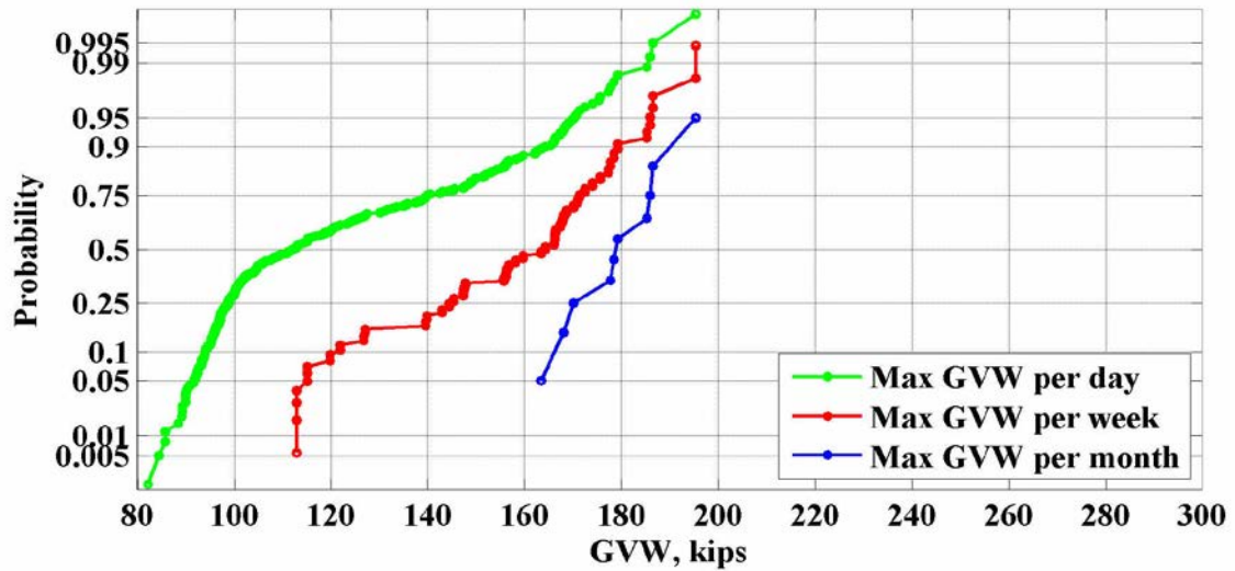
Figure 66: Maximum values of GVW for the location 960(Whatley) – 2013
