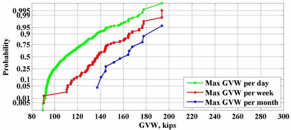
Figure 91: Maximum values of GVW for the location 964(Ozark) – 2010
