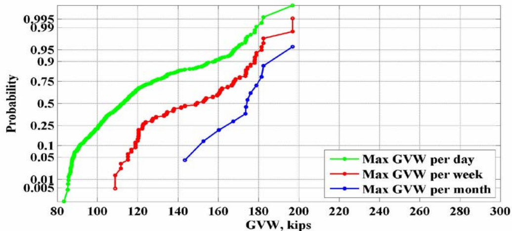
Figure 11: Maximum values of GVW for the location 915(Sunflower) – 2008
