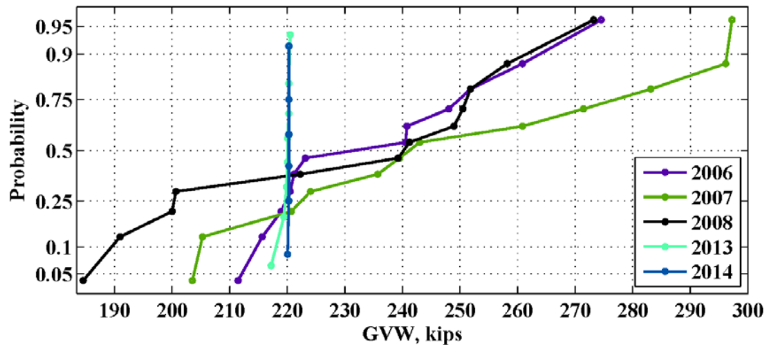
Figure 86: Maximum monthly GVW for the location 963(Grand Bay) – 2006-2014
