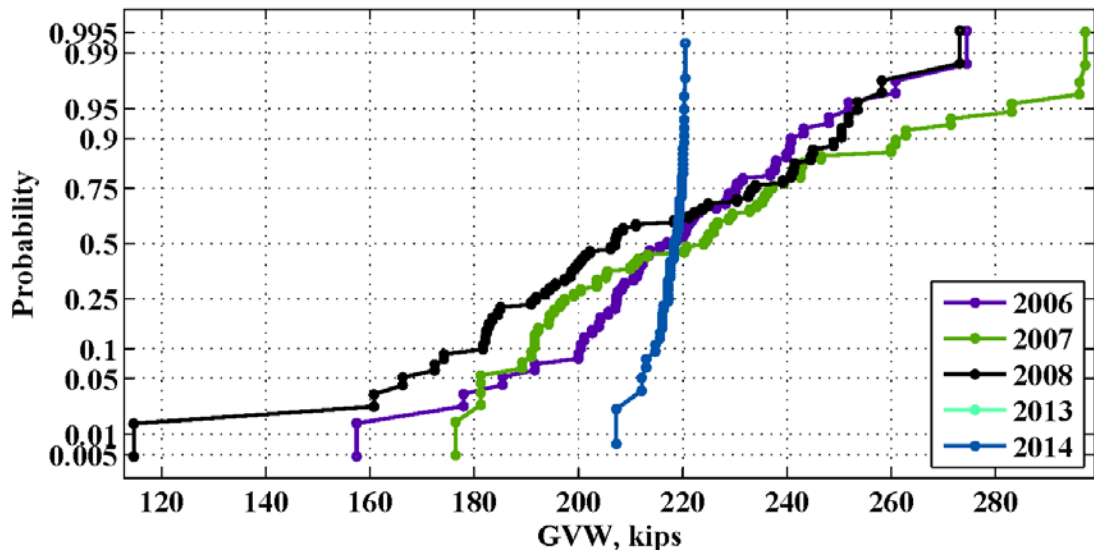
Figure 85: Maximum weekly GVW for the location 963(Grand Bay) – 2006-2014
