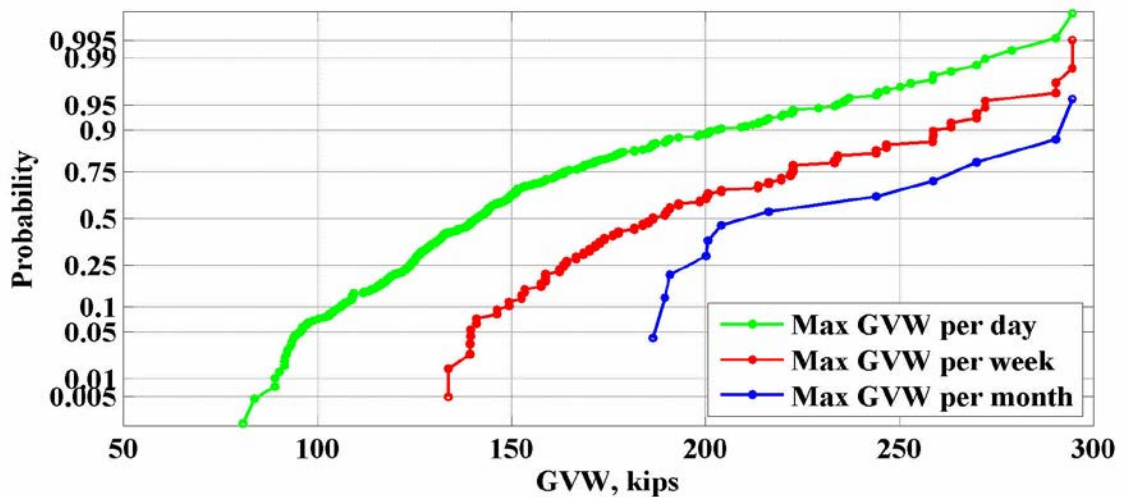
Figure 100: Maximum values of GVW for the location 965(Shorter) – 2008
