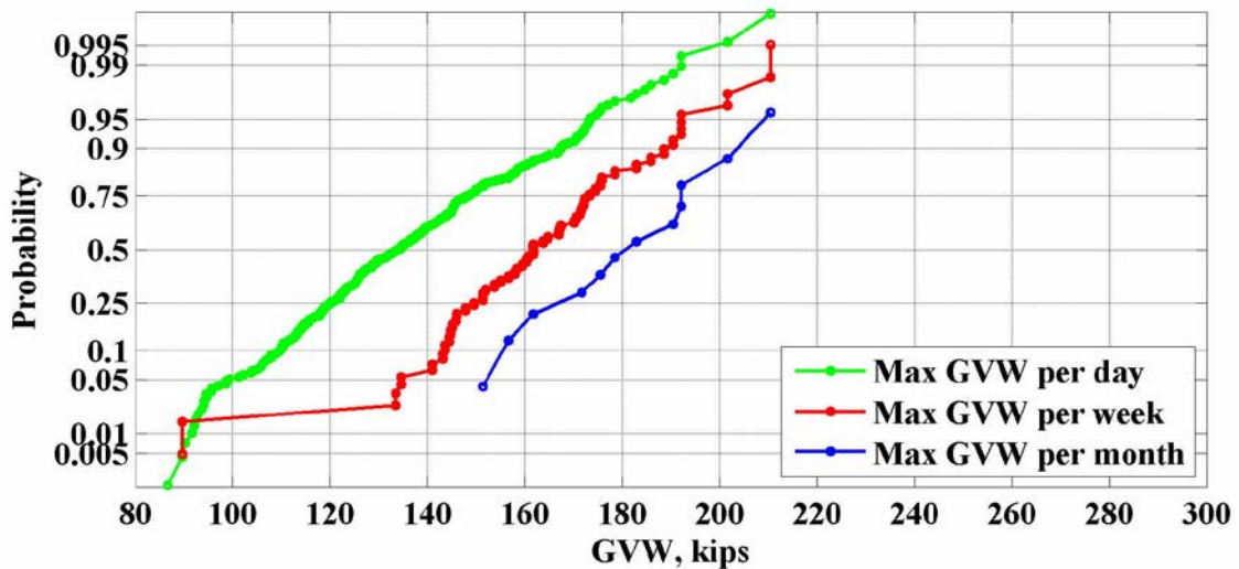
Figure 31: Maximum values of GVW for the location 931(Athens) – 2011
