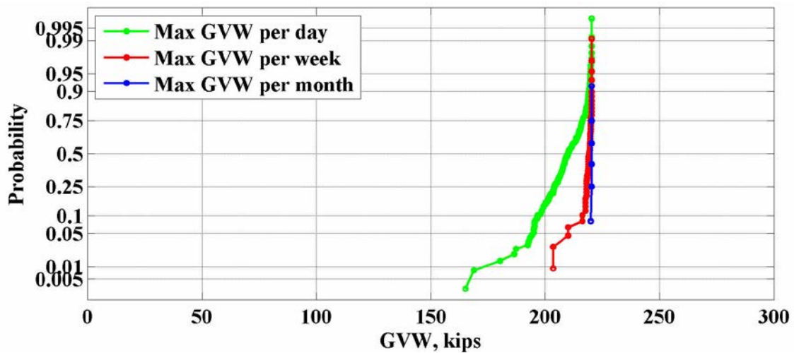
Figure 83: Maximum values of GVW for the location 963(Grand Bay) – 2014
