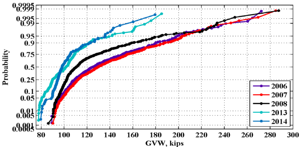
Figure 52: Maximum daily GVW for the location 934(Sumiton) – 2006-2014
