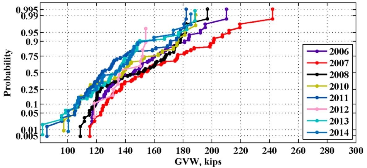
Figure 18: Maximum weekly GVW for the location 915(Sunflower) – 2006-2014
