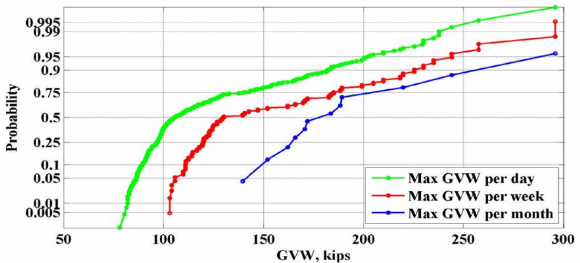
Figure 57: Maximum values of GVW for the location 942(Pine Level) – 2008
