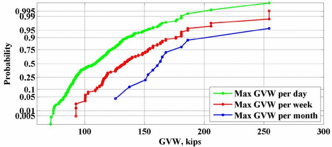
Figure 87: Maximum values of GVW for the location 964(Ozark) – 2006
