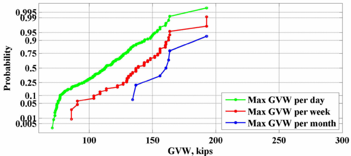
Figure 88: Maximum values of GVW for the location 964(Ozark) – 2007
