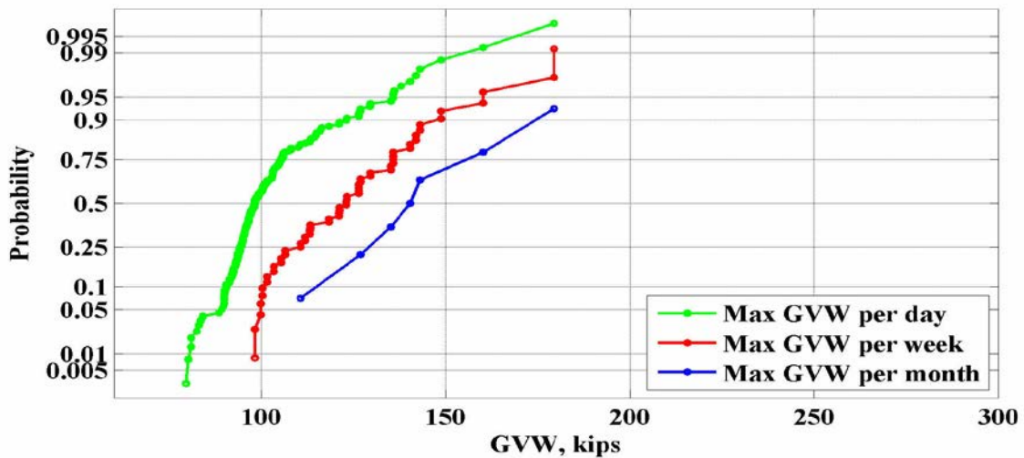
Figure 51: Maximum values of GVW for the location 934(Sumiton) – 2014
