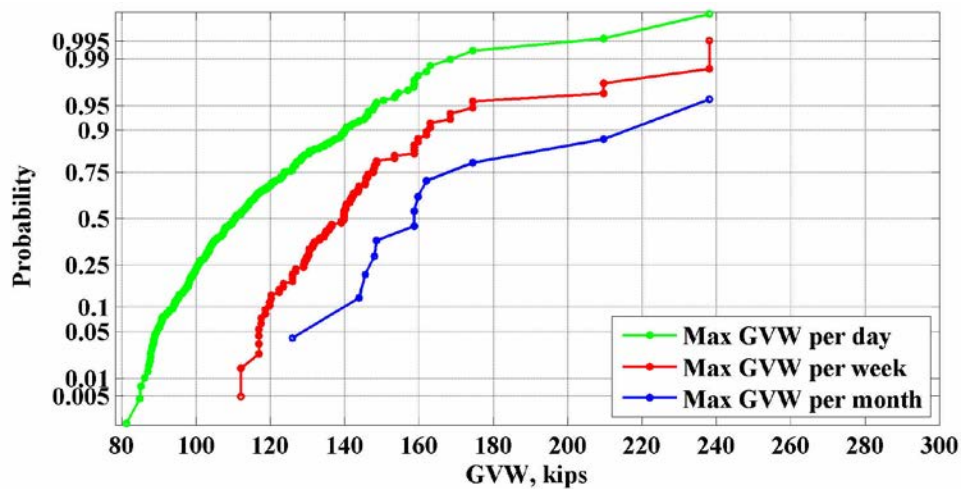
Figure 2: Maximum values of GVW for the location 911(Alex City) – 2007
