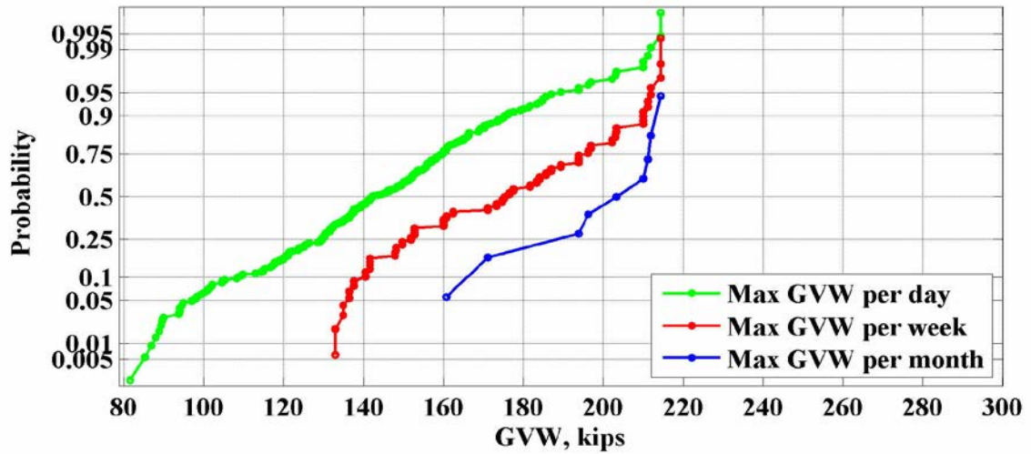
Figure 74: Maximum values of GVW for the location 961(Mobile) – 2013
