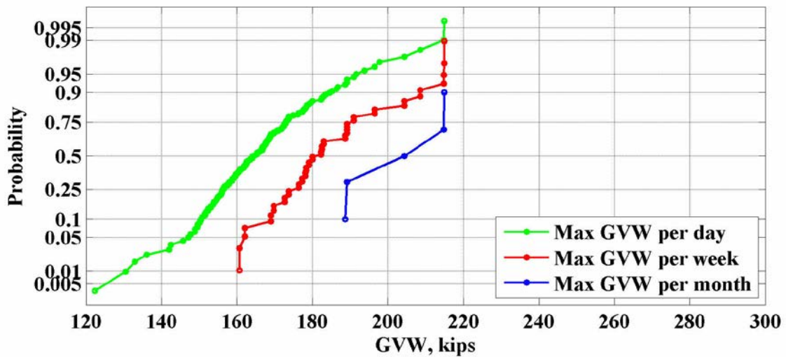
Figure 75: Maximum values of GVW for the location 961(Mobile) – 2014
