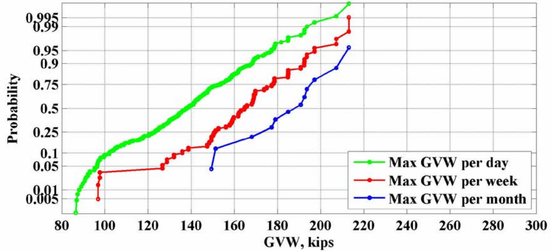
Figure 30: Maximum values of GVW for the location 931(Athens) – 2010
