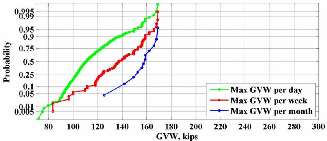
Figure 107: Maximum values of GVW for the location US231 – 2013
