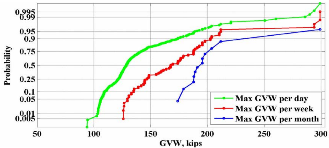
Figure 63: Maximum values of GVW for the location 960(Whatley) – 2006
