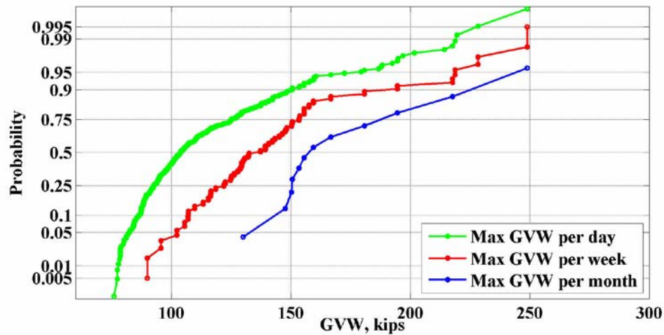
Figure 1: Maximum values of GVW for the location 911(Alex City) – 2006
