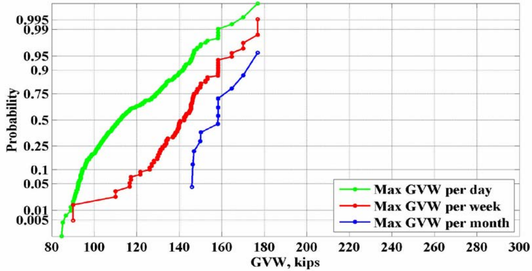
Figure 40: Maximum values of GVW for the location 933(Muscle Shoals) – 2010
