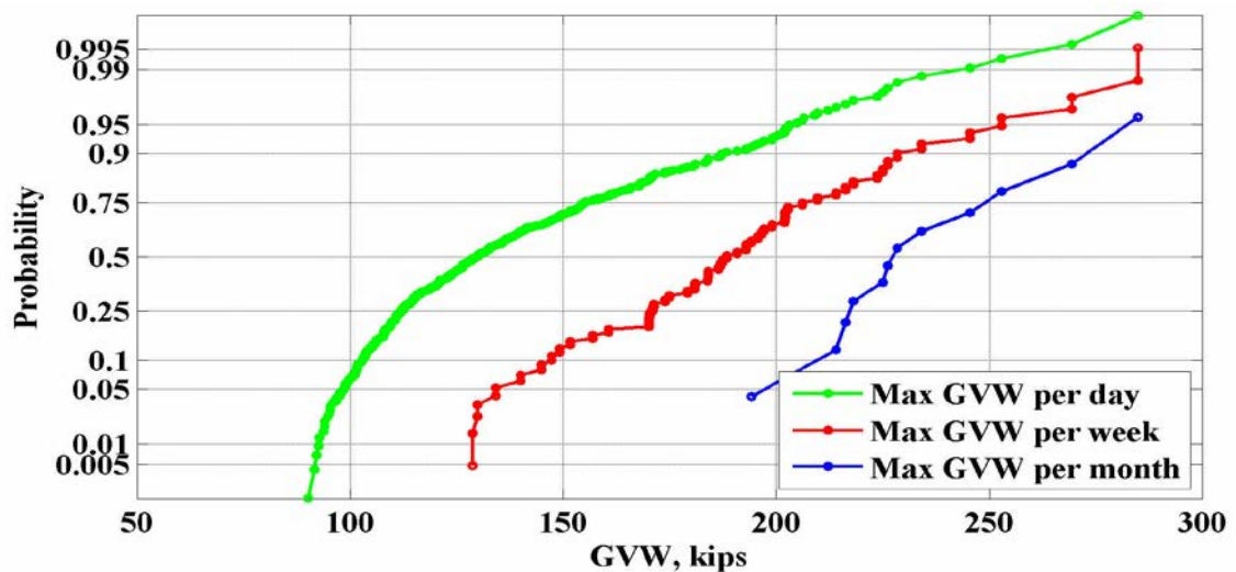
Figure 48: Maximum values of GVW for the location 934(Sumiton) – 2007
