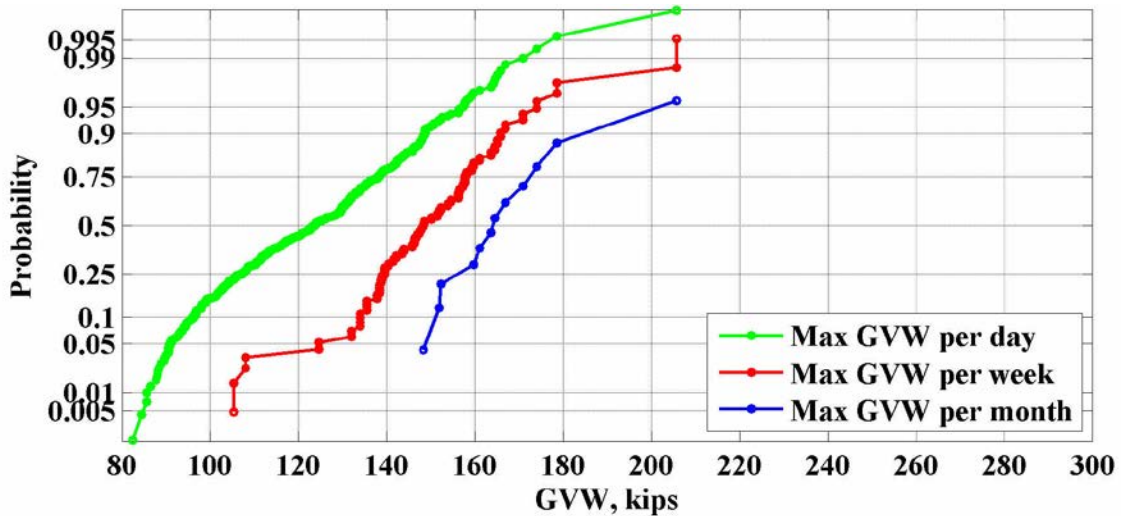
Figure 28: Maximum values of GVW for the location 931(Athens) – 2008
