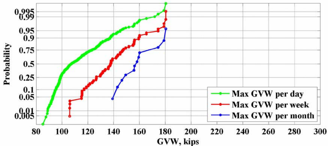
Figure 89: Maximum values of GVW for the location 964(Ozark) – 2008
