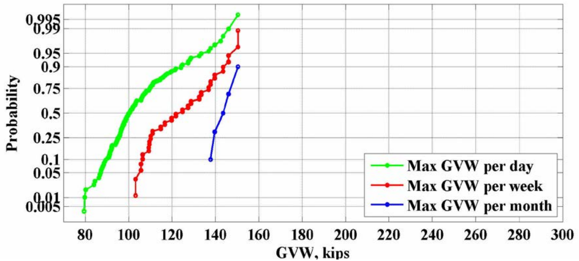
Figure 108: Maximum values of GVW for the location US231 – 2014
