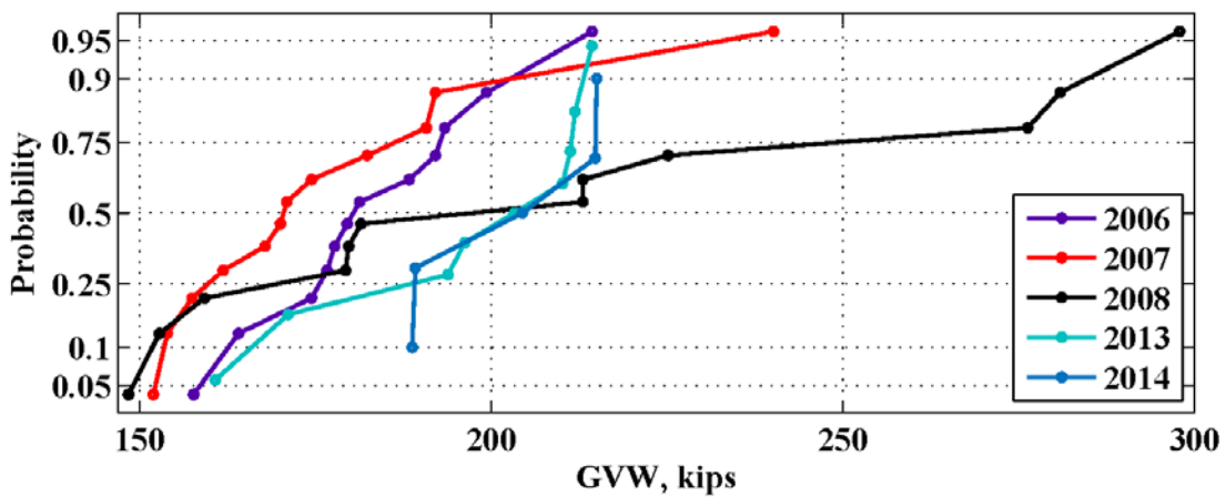
Figure 78: Maximum monthly GVW for the location 961(Mobile) – 2006-2014
