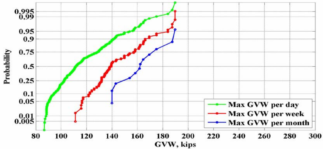
Figure 39: Maximum values of GVW for the location 933(Muscle Shoals) – 2009
