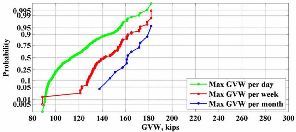
Figure 92: Maximum values of GVW for the location 964(Ozark) – 2011
