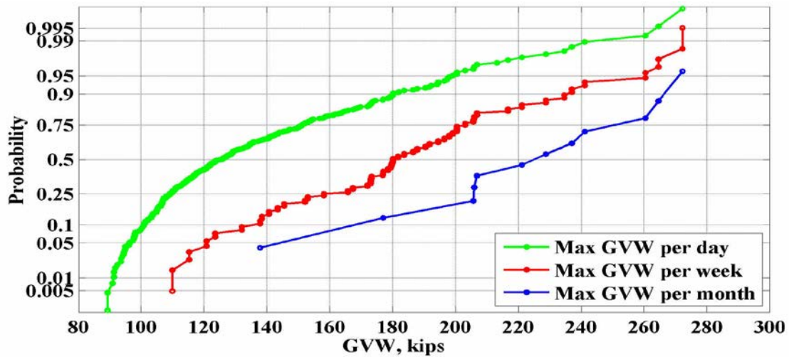
Figure 47: Maximum values of GVW for the location 934(Sumiton) – 2006
