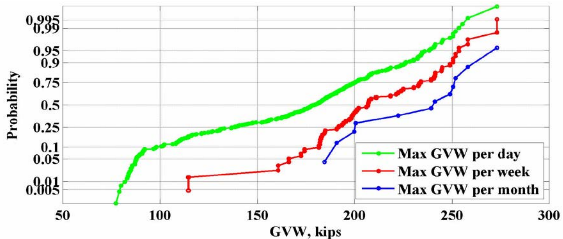
Figure 81: Maximum values of GVW for the location 963(Grand Bay) – 2008
