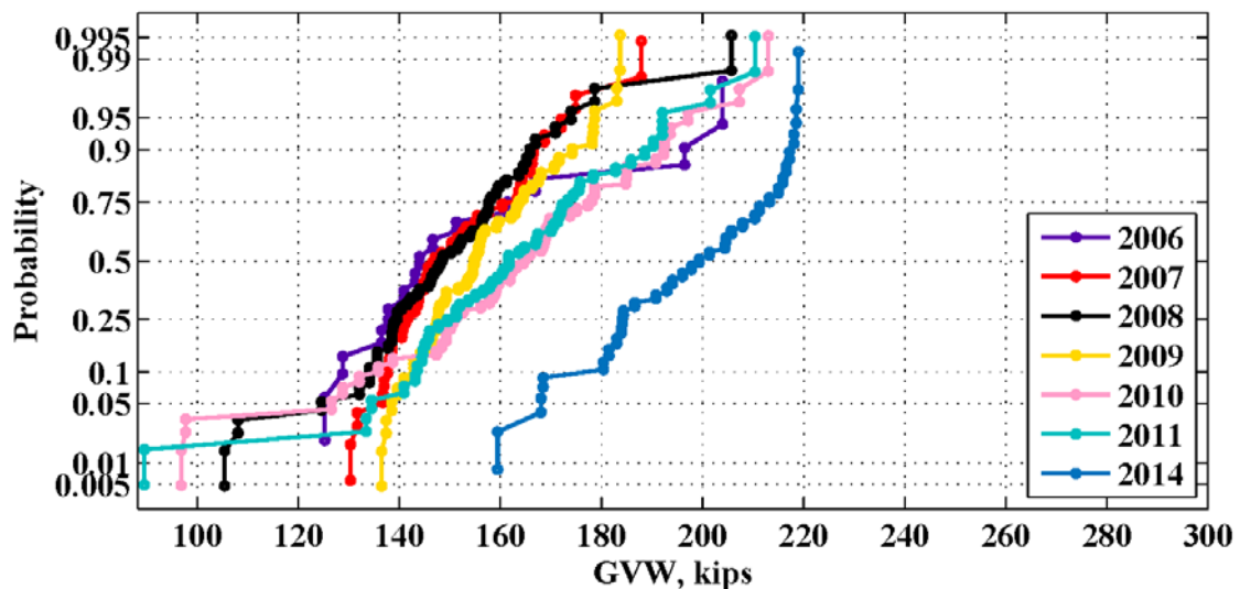
Figure 34: Maximum weekly GVW for the location 931(Athens) – 2006-2014
