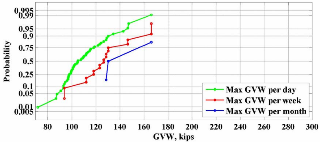
Figure 106: Maximum values of GVW for the location US231 – 2012
