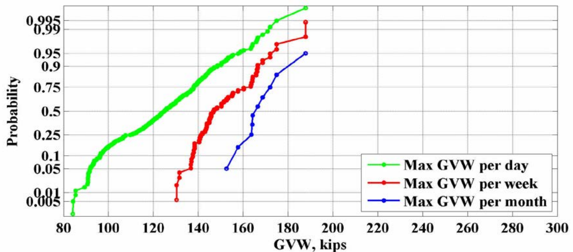
Figure 27: Maximum values of GVW for the location 931(Athens) – 2007
