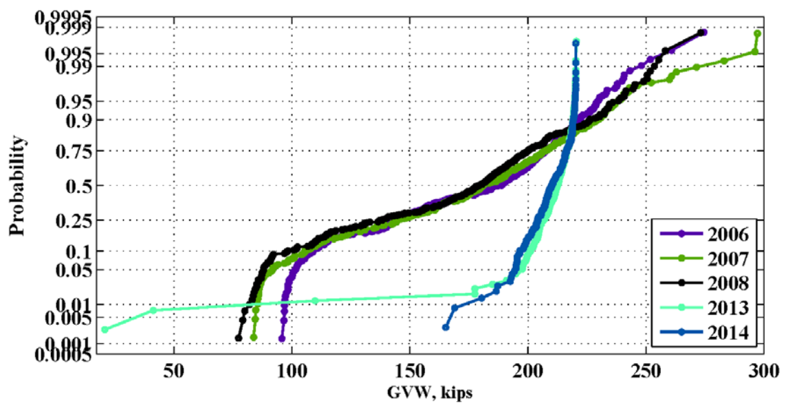
Figure 84: Maximum daily GVW for the location 963(Grand Bay) – 2006-2014
