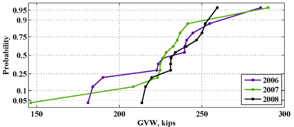
Figure 25: Maximum monthly GVW for the location 915(Sunflower) – 2006-2014
