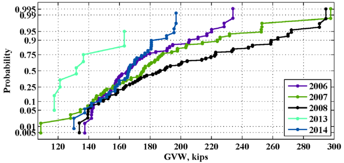
Figure 104: Maximum weekly GVW for the location 965(Shorter)– 2006-2014
