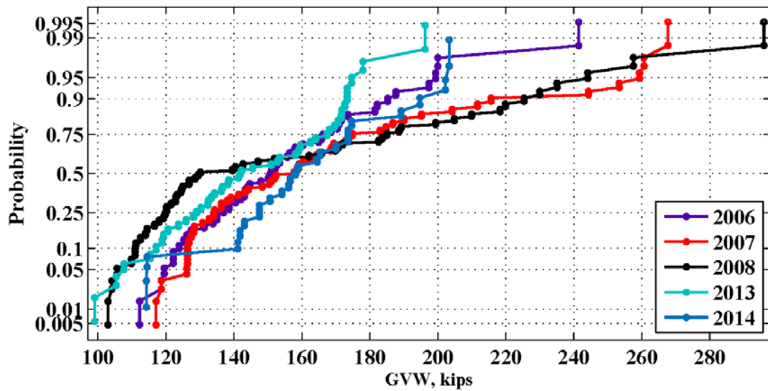
Figure 61: Maximum weekly GVW for the location 942(Pine Level) – 2006-2014
