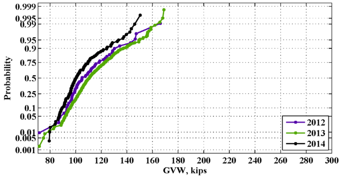
Figure 109: Maximum daily GVW for the location US-231 – 2012-2014
