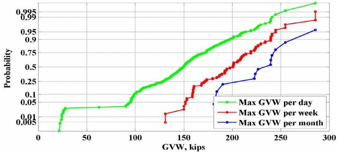
Figure 20: Maximum values of GVW for the location 918(Bucksville) – 2006
