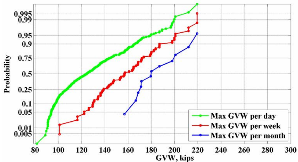
Figure 41: Maximum values of GVW for the location 933(Muscle Shoals) – 2011
