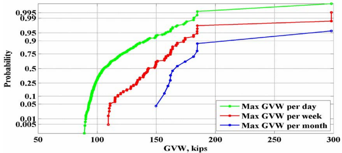
Figure 36: Maximum values of GVW for the location 933(Muscle Shoals) – 2006
