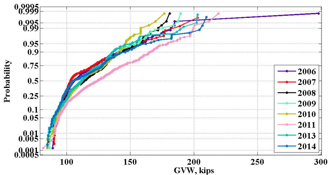
Figure 44: Maximum daily GVW for the location 933(Muscle Shoals) – 2006-2014
