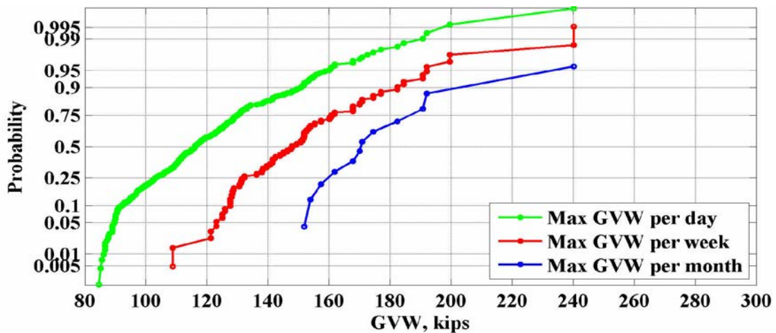
Figure 72: Maximum values of GVW for the location 961(Mobile) – 2007
