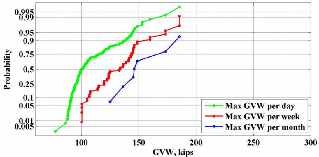
Figure 16: Maximum values of GVW for the location 915(Sunflower) – 2014
