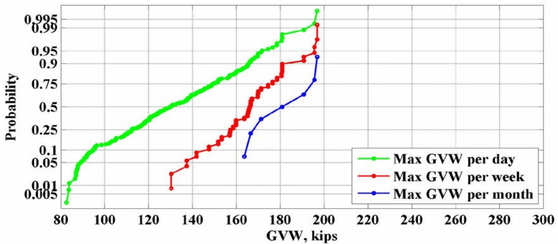
Figure 102: Maximum values of GVW for the location 965(Shorter) – 2014
