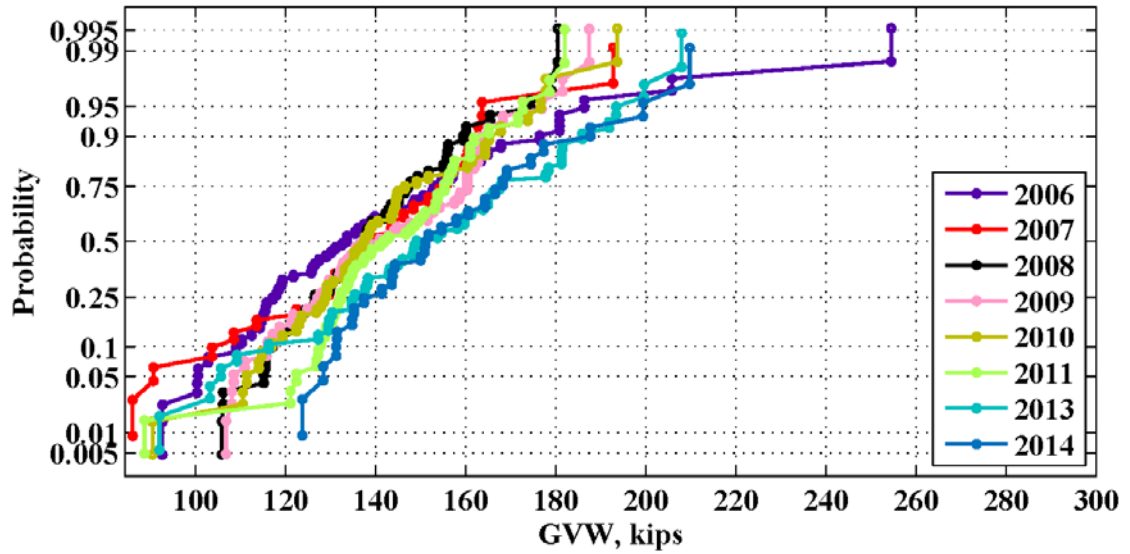
Figure 96: Maximum weekly GVW for the location 964(Ozark) – 2006-2014
