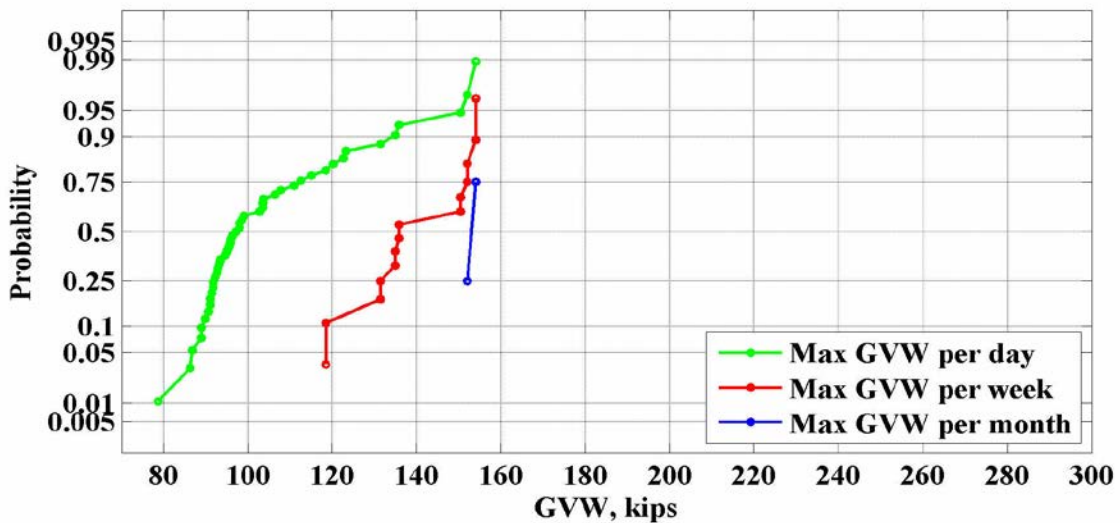
Figure 14: Maximum values of GVW for the location 915(Sunflower) – 2012
