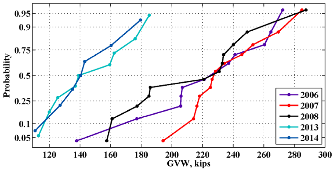
Figure 54: Maximum monthly GVW for the location 934(Sumiton) – 2006-2014
