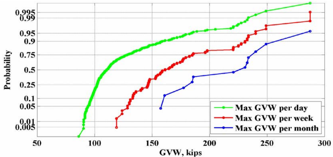
Figure 49: Maximum values of GVW for the location 934(Sumiton) – 2008
