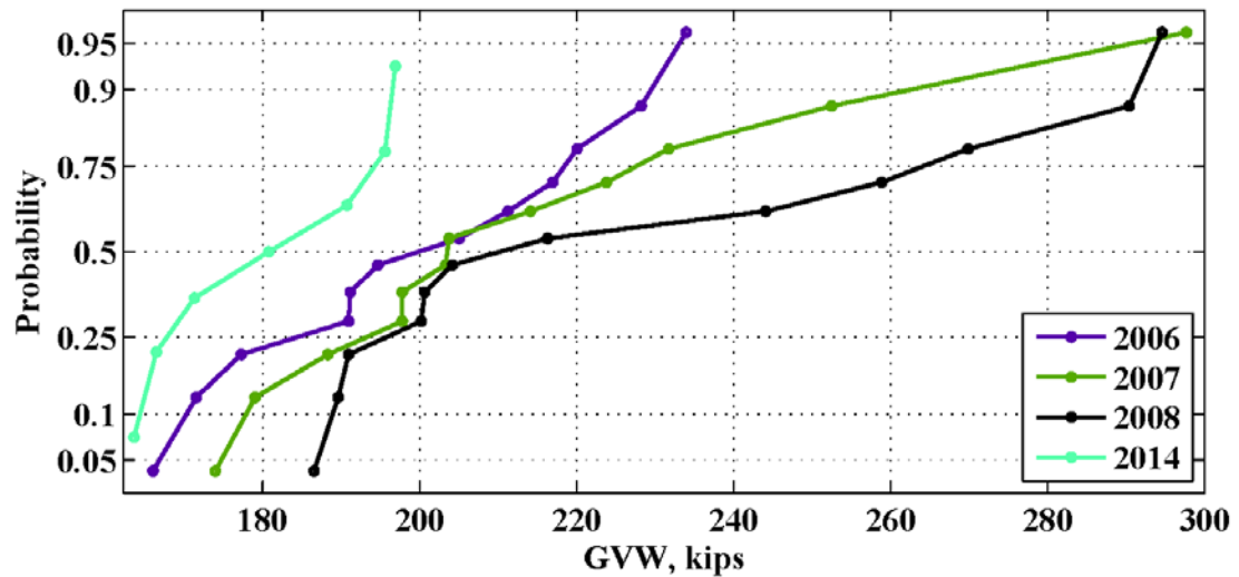
Figure 105: Maximum monthly GVW for the location 965(Shorter)– 2006-2014
