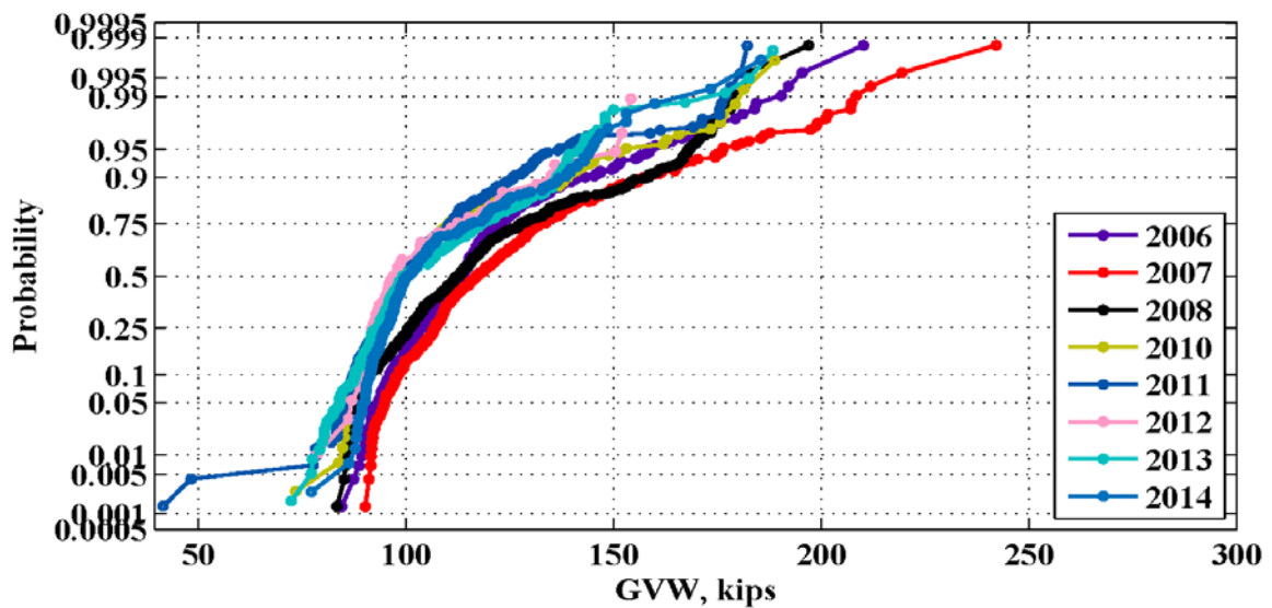
Figure 17: Maximum daily GVW for the location 915(Sunflower) – 2006-2014
