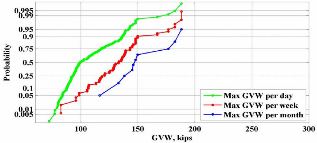
Figure 15: Maximum values of GVW for the location 915(Sunflower) – 2013
