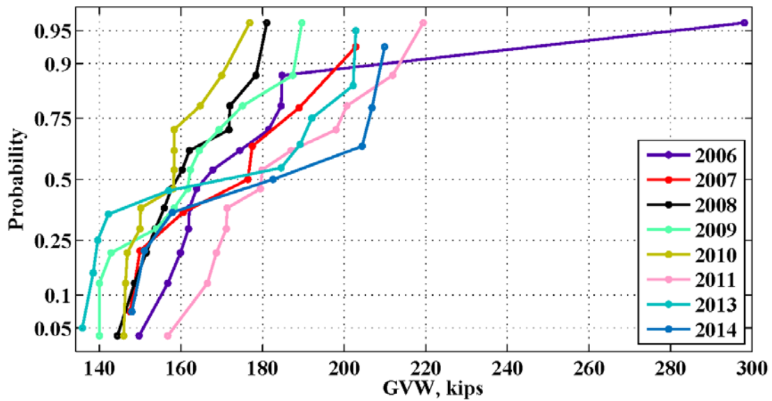
Figure 46: Maximum monthly GVW for the location 933(Muscle Shoals) – 2006-2014
