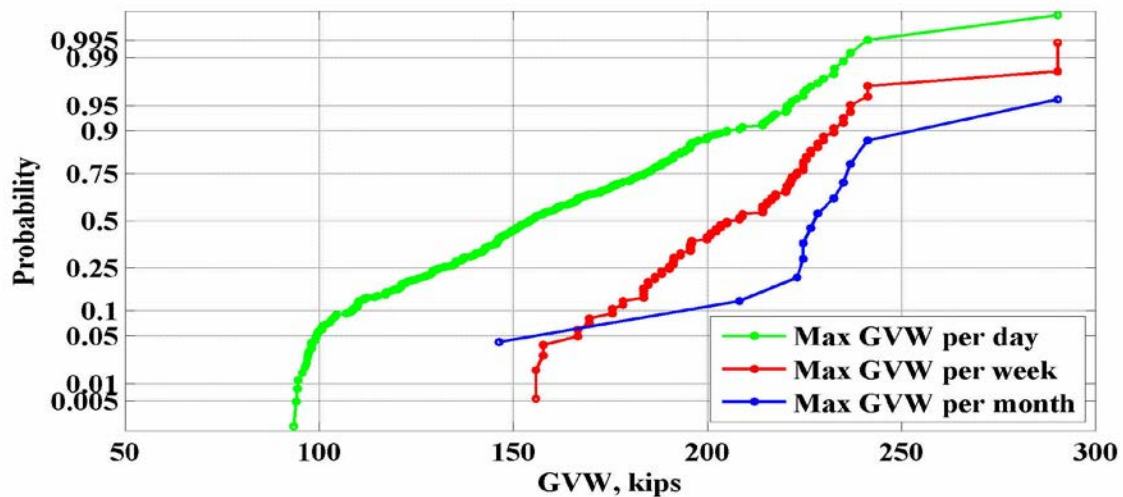
Figure 21: Maximum values of GVW for the location 918(Bucksville) – 2007
