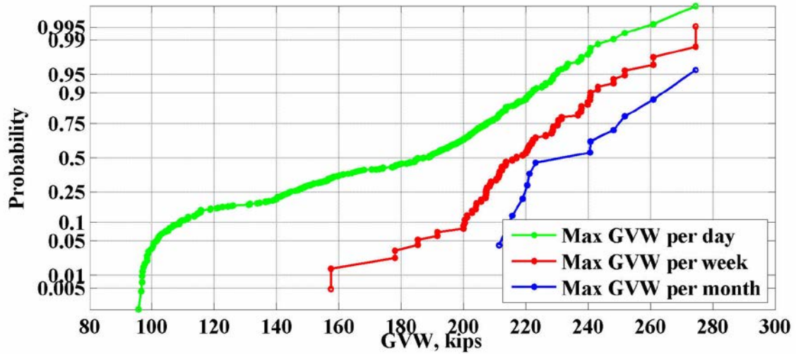
Figure 79: Maximum values of GVW for the location 963(Grand Bay) – 2006
