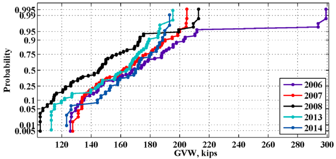
Figure 69: Maximum weekly GVW for the location 960(Whatley) – 2006-2014
