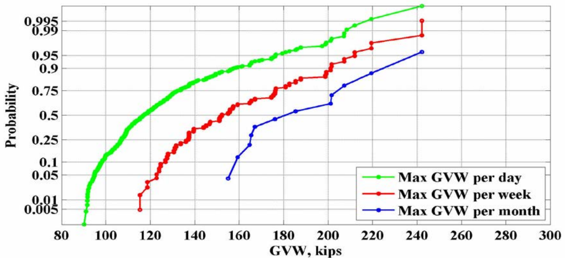
Figure 10: Maximum values of GVW for the location 915(Sunflower) – 2007
