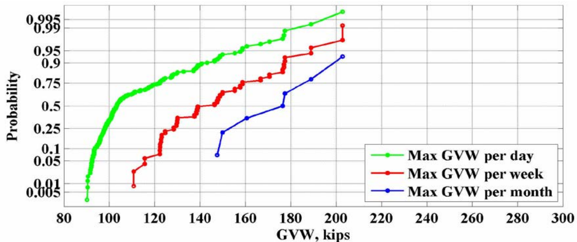
Figure 37: Maximum values of GVW for the location 933(Muscle Shoals) – 2007
