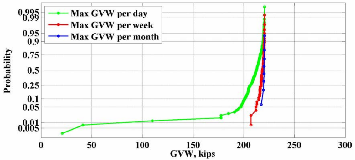
Figure 82: Maximum values of GVW for the location 963(Grand Bay) – 2013
