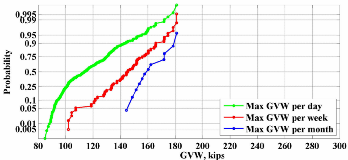
Figure 38: Maximum values of GVW for the location 933(Muscle Shoals) – 2008
