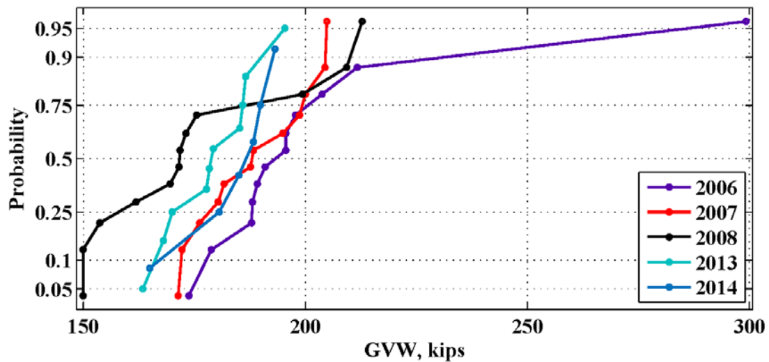
Figure 70: Maximum weekly GVW for the location 960(Whatley) – 2006-2014
