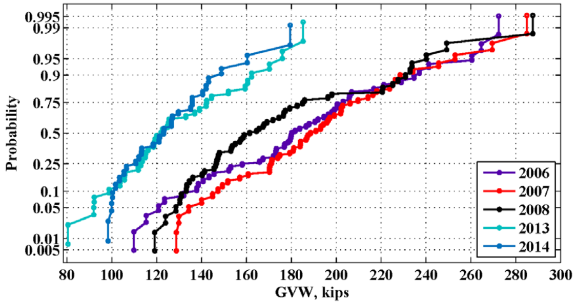
Figure 53: Maximum weekly GVW for the location 934(Sumiton) – 2006-2014
