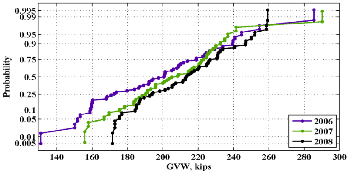
Figure 24: Maximum weekly GVW for the location 915(Sunflower) – 2006-2014
