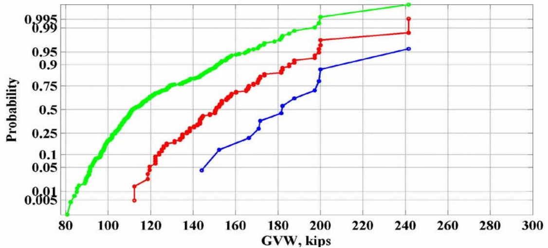
Figure 55: Maximum values of GVW for the location 942(Pine Level) – 2006
