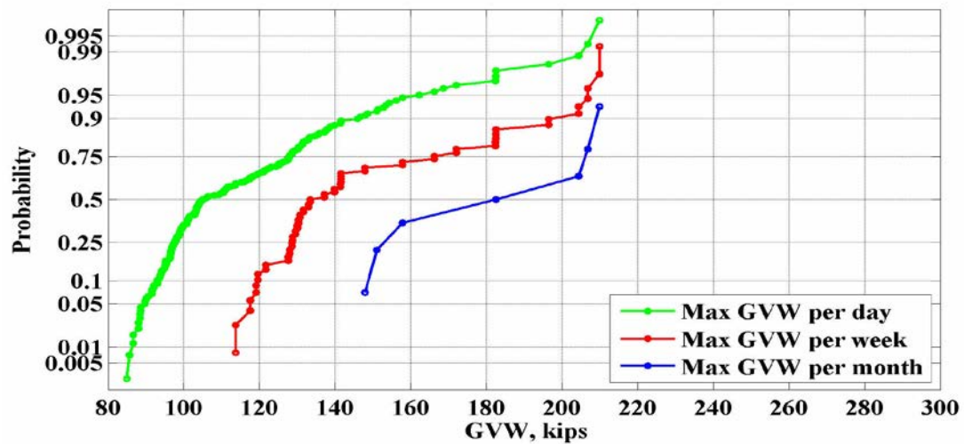
Figure 43: Maximum values of GVW for the location 933(Muscle Shoals)– 2014
