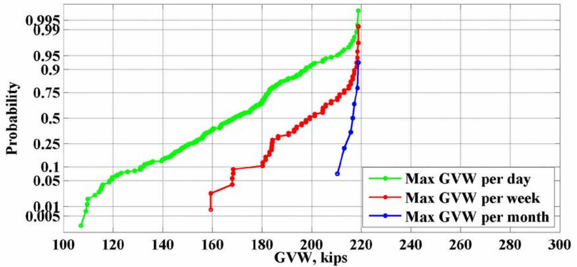
Figure 32: Maximum values of GVW for the location 931(Athens) – 2014
