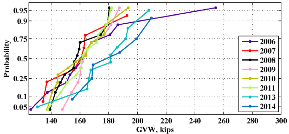
Figure 97: Maximum monthly GVW for the location 964(Ozark) – 2006-2014
