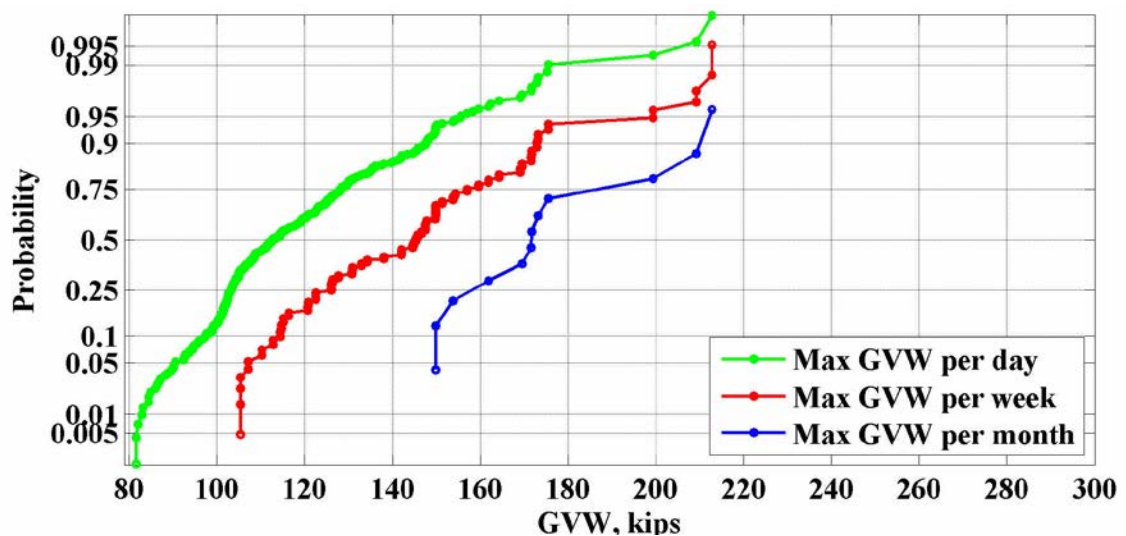
Figure 65: Maximum values of GVW for the location 960(Whatley) – 2008
