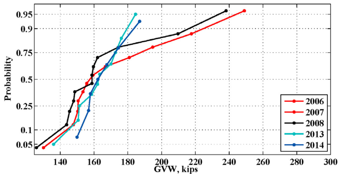
Figure 8: Maximum monthly GVW for the location 911(Alex City) – 2006-2014
