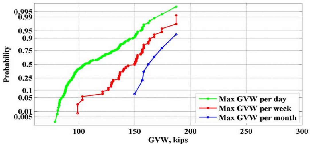
Figure 5: Maximum values of GVW for the location 911(Alex City) – 2014
