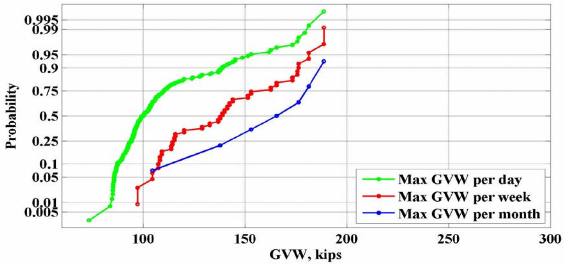
Figure 12: Maximum values of GVW for the location 915(Sunflower) – 2010
