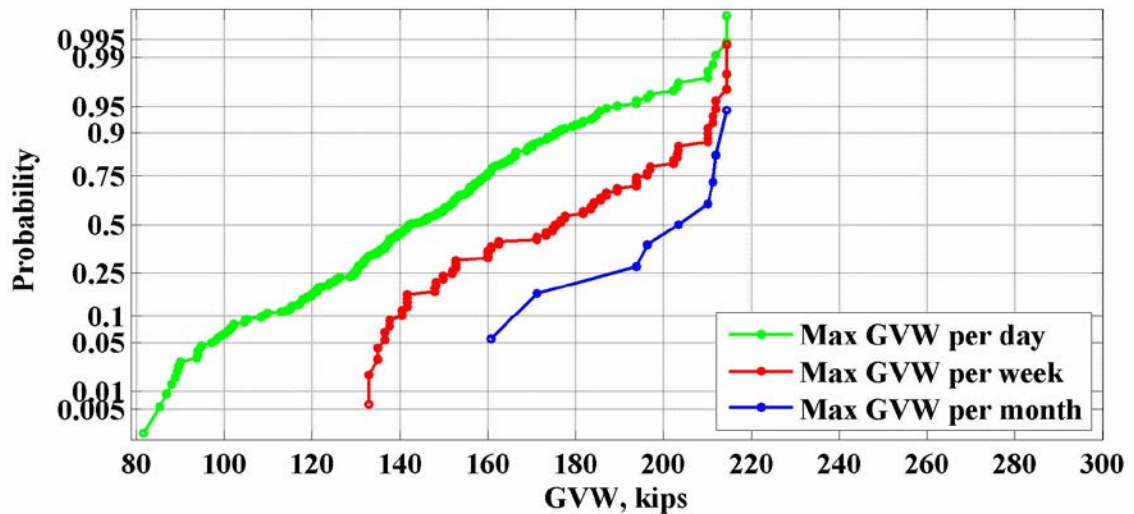
Figure 73: Maximum values of GVW for the location 961(Mobile) – 2008
