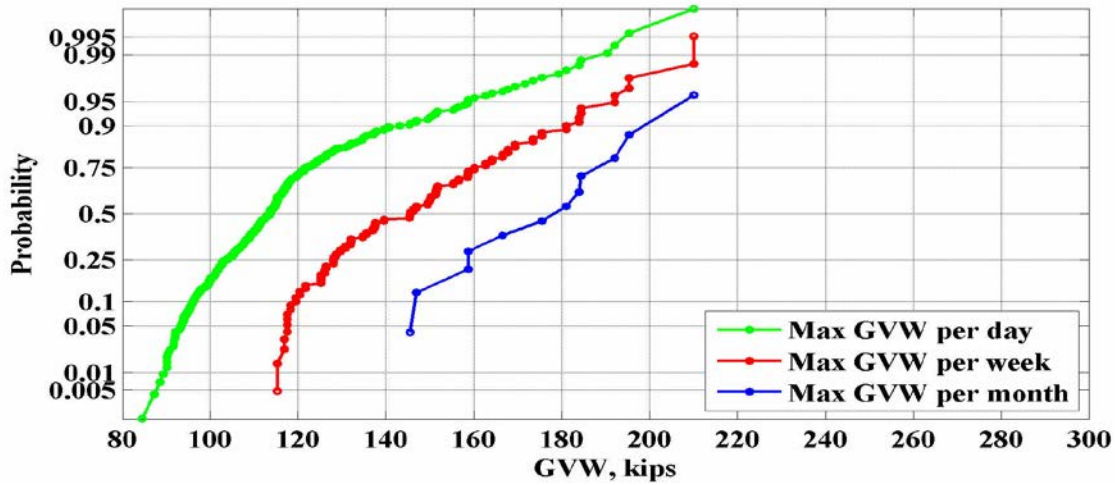
Figure 9: Maximum values of GVW for the location 915(Sunflower) – 2006
