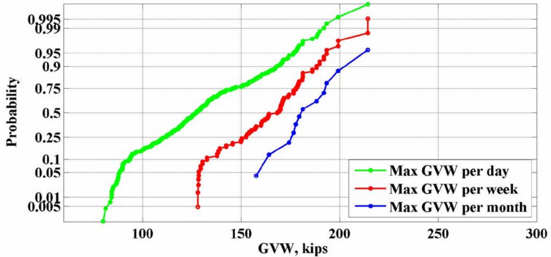
Figure 71: Maximum values of GVW for the location 961(Mobile) – 2006
