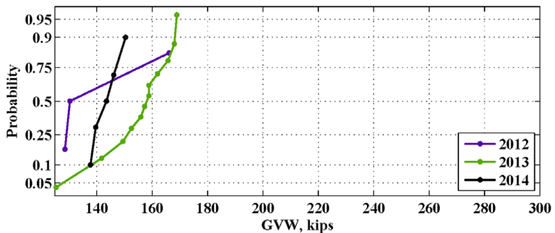
Figure 111: Maximum monthly GVW for the location US-231 – 2012-2014
