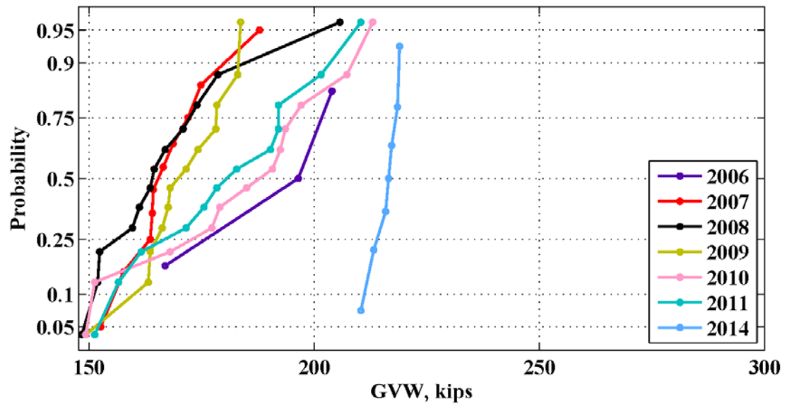
Figure 35: Maximum monthly GVW for the location 931(Athens) – 2006-2014
