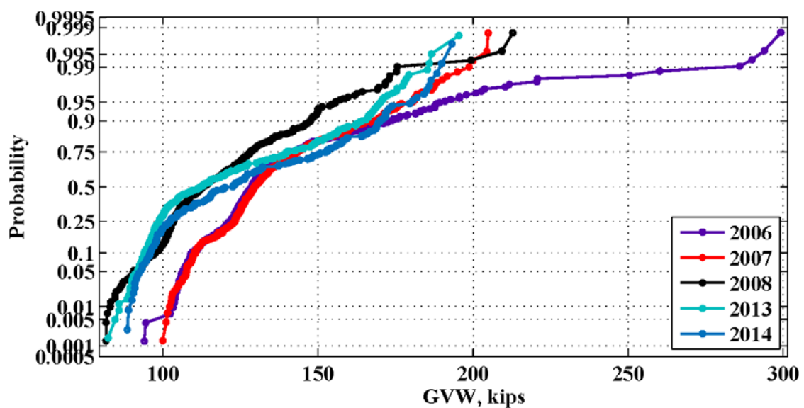
Figure 68: Maximum daily GVW for the location 960(Whatley) – 2006-2014
