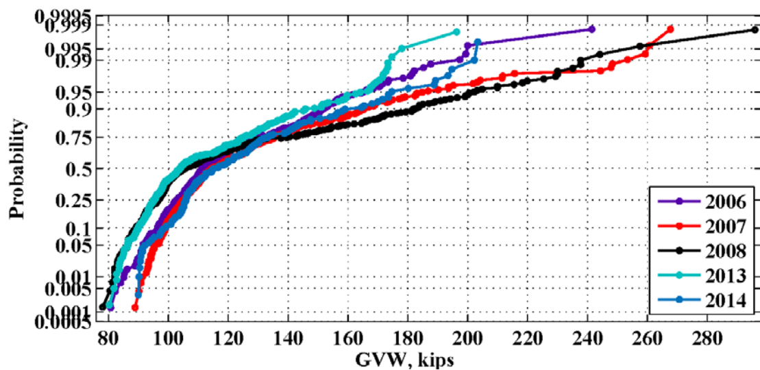
Figure 60: Maximum daily GVW for the location 942(Pine Level) – 2006-2014
