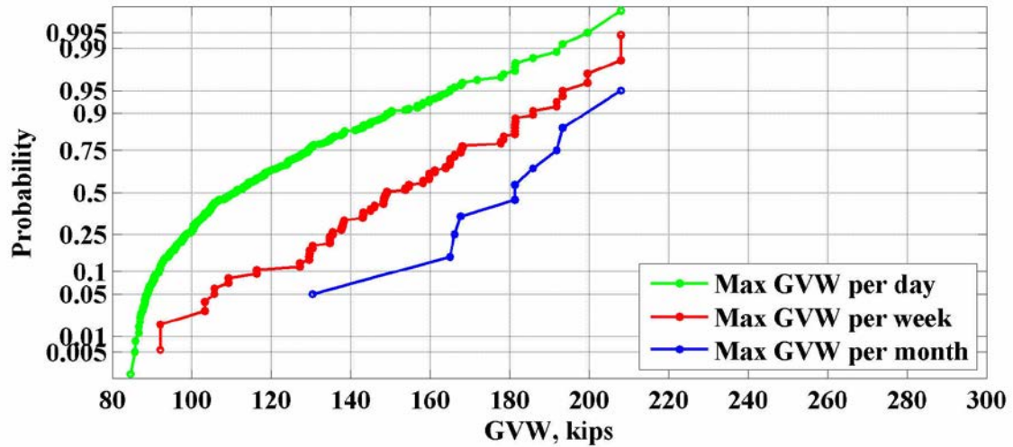
Figure 93: Maximum values of GVW for the location 964(Ozark) – 2013
