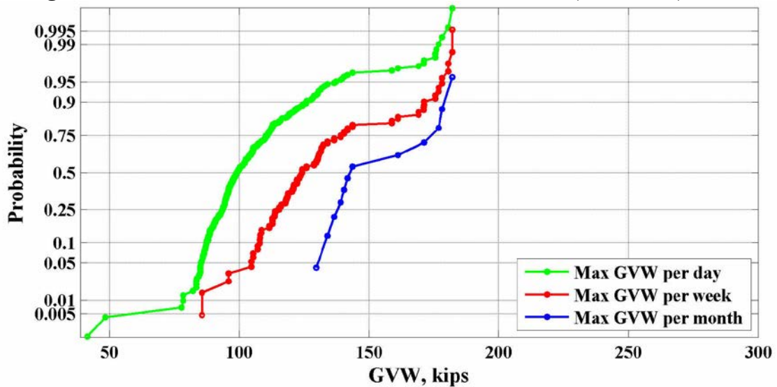
Figure 13: Maximum values of GVW for the location 915(Sunflower) – 2011
