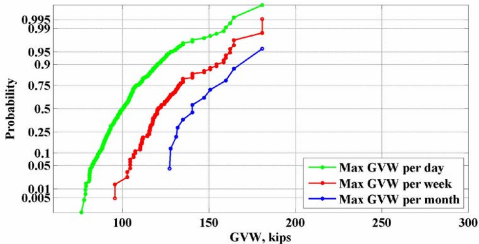
Figure 3: Maximum values of GVW for the location 911(Alex City) – 2008
