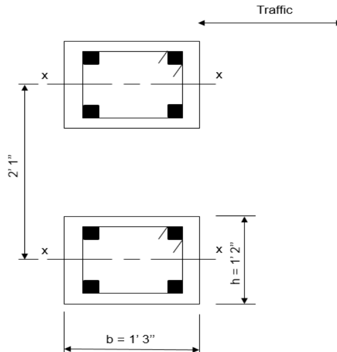
Figure 13: Typical Column 2 Cross Section
