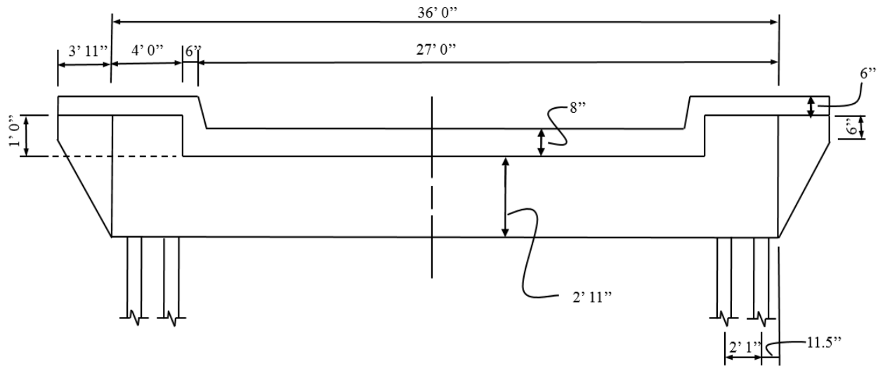
Figure 10: Typical Transverse Beam Dimensions for Spans IV and V
