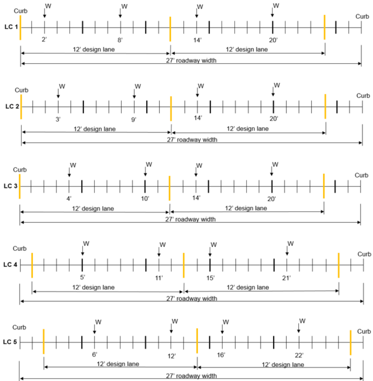
Figure 36: Live Load Cases 1 - 5
