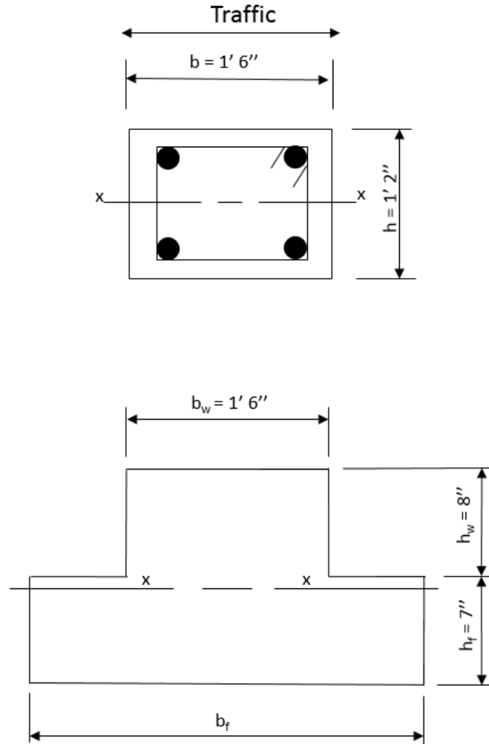
Figure 15: Column 3 Cross Section
