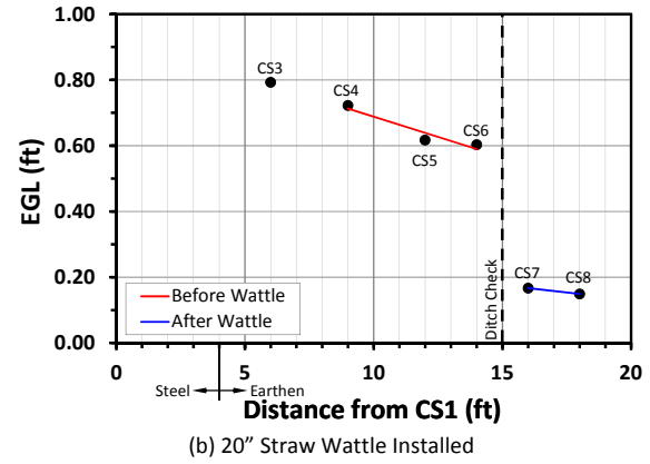
Figure 19: Energy Slope Profiles of Cross Sections.
