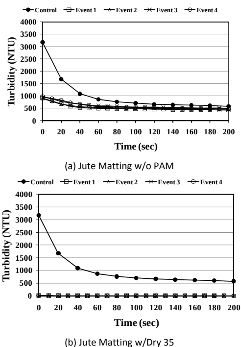
Figure 3: Settling Pattern of Runoff Water.
