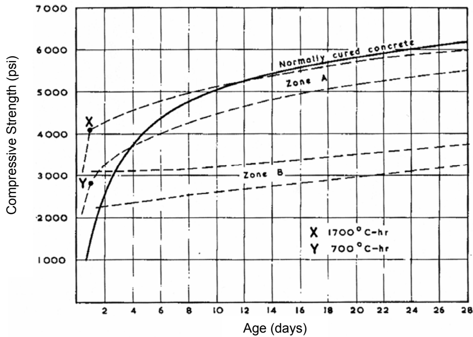
Figure 2.11: Temperature affects on long-term strength (Saul 1951)
