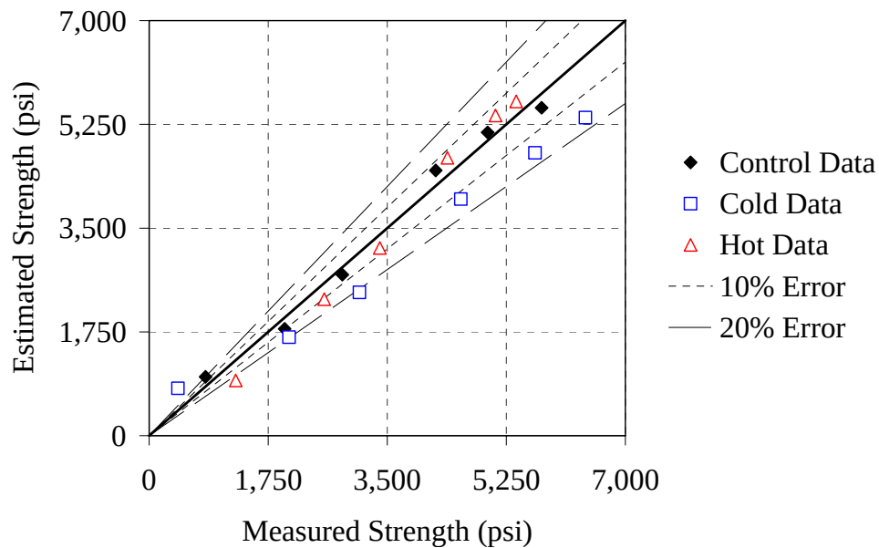
Figure D-1: Estimated strength versus actual strength for Type I - 0.44 mixture
