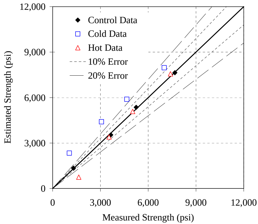
Figure G-17: Error plot for the 70/20/10 - 0.37 mixture, Modified method, NSM
