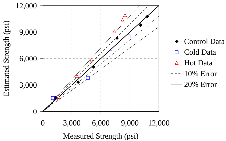
Figure D-9: Estimated strength versus actual strength for 70/20/10 - 0.37 mixture
