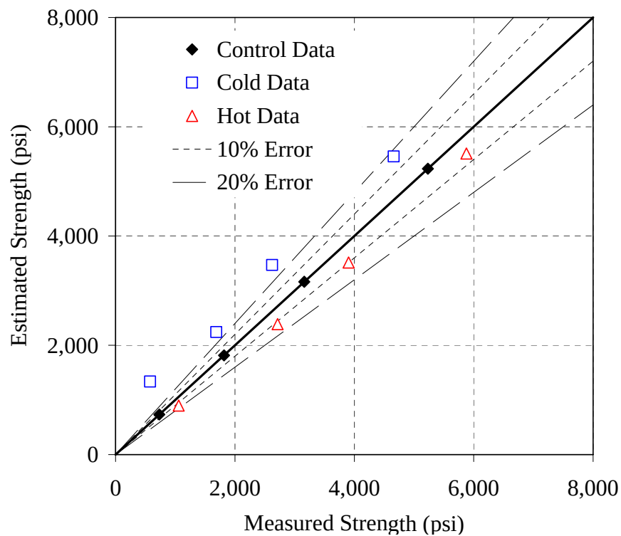
Figure I-10: Error plot for the 30% C mixture, simplified method, E = 25 kJ/mol
