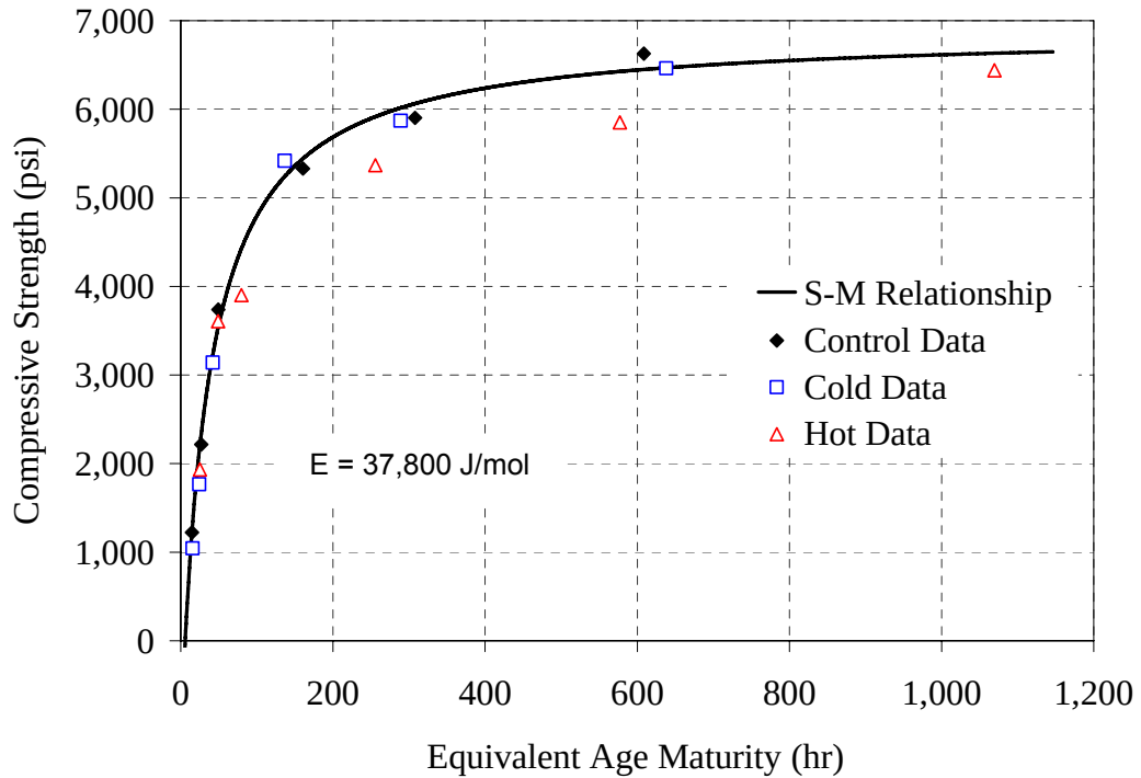
Figure C-4: Strength-maturity plot, ASTM C 1074 method for 20% C mixture
