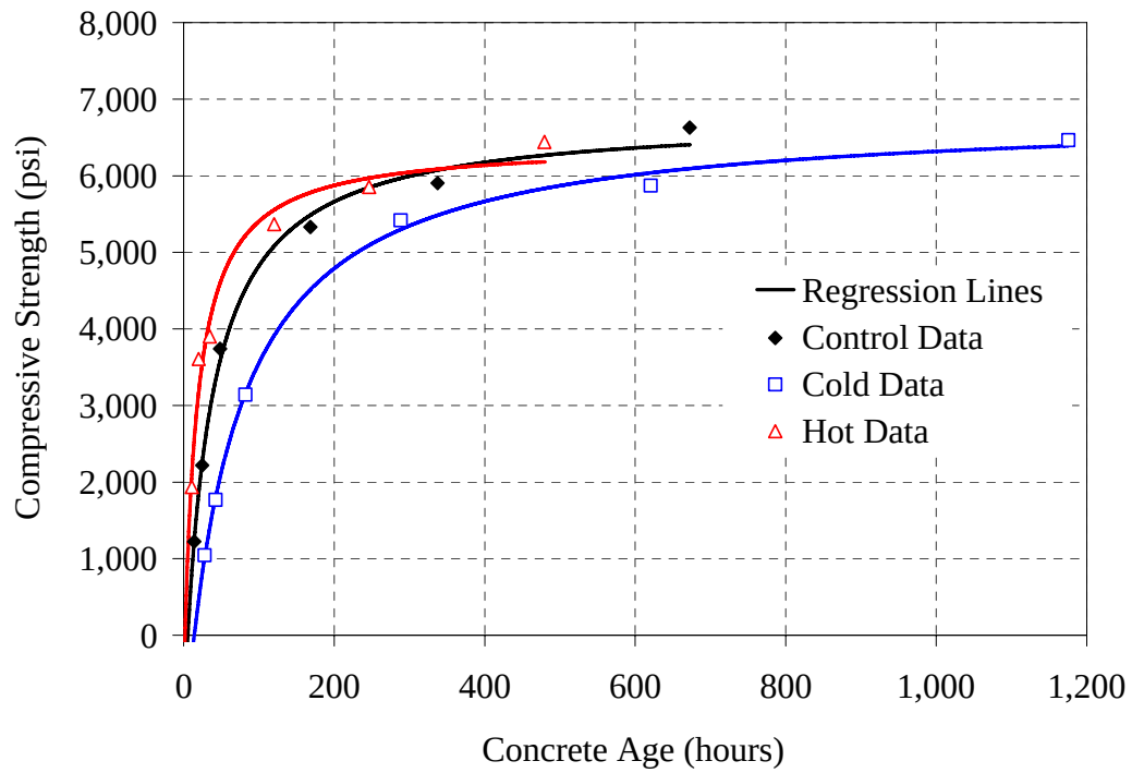
Figure 5.7: Compressive strength versus age results for 20% C mixture
