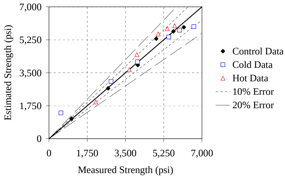
Figure 6.13: Estimated strength versus actual strength for the Type I - 0.41 mixture
