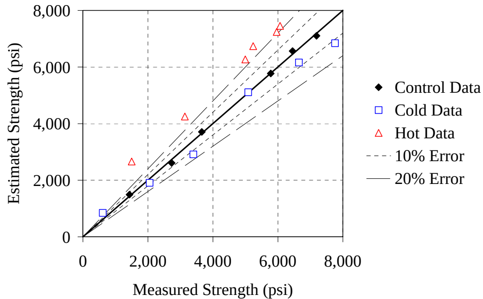
Figure D-16: Estimated strength versus actual strength for 30% Slag mixture
