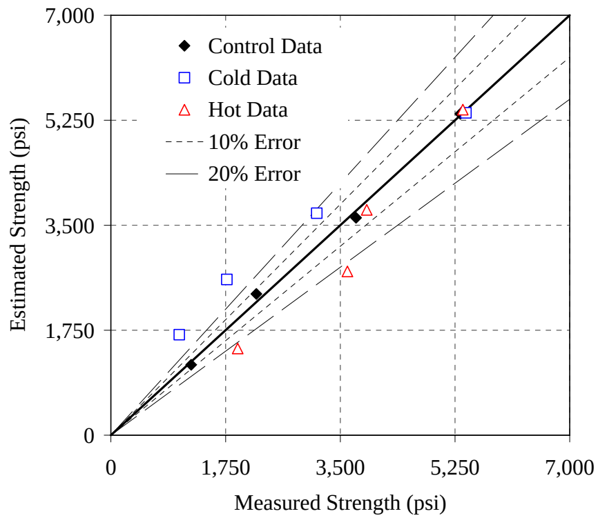
Figure H-7: Error plot for the 20% C mixture, simplified method, T_o = 14^\circ\text{F}
