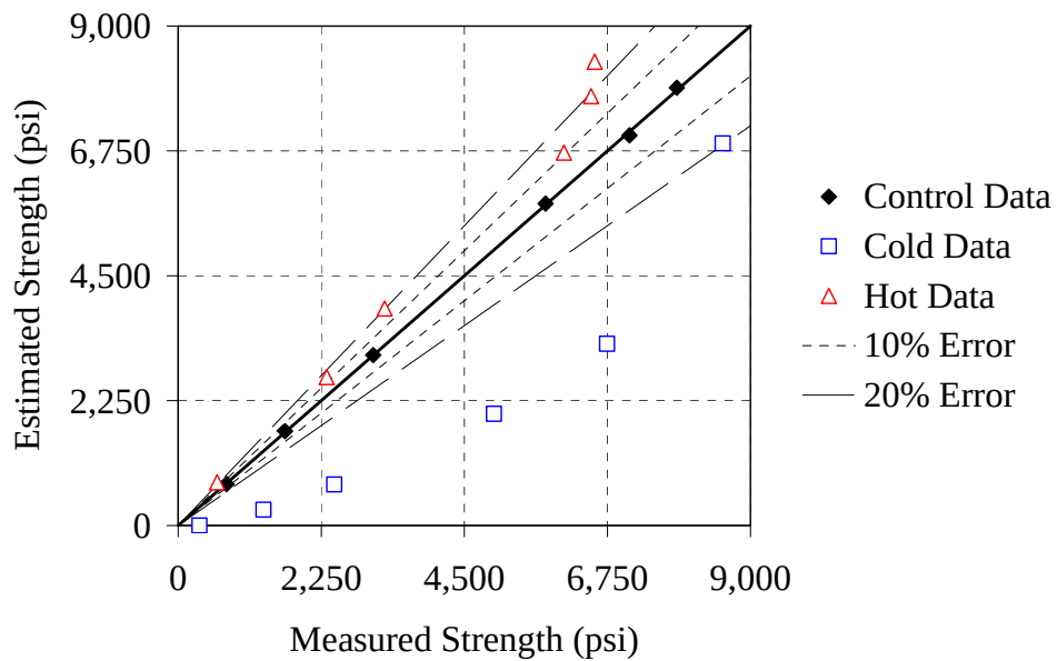
Figure D-7: Estimated strength versus actual strength for 50% Slag mixture
