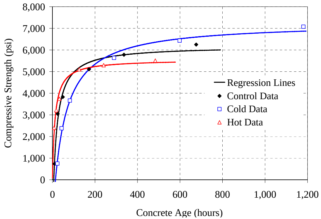
Figure 5.12: Compressive strength versus age results for Type III - 0.44 mixture
