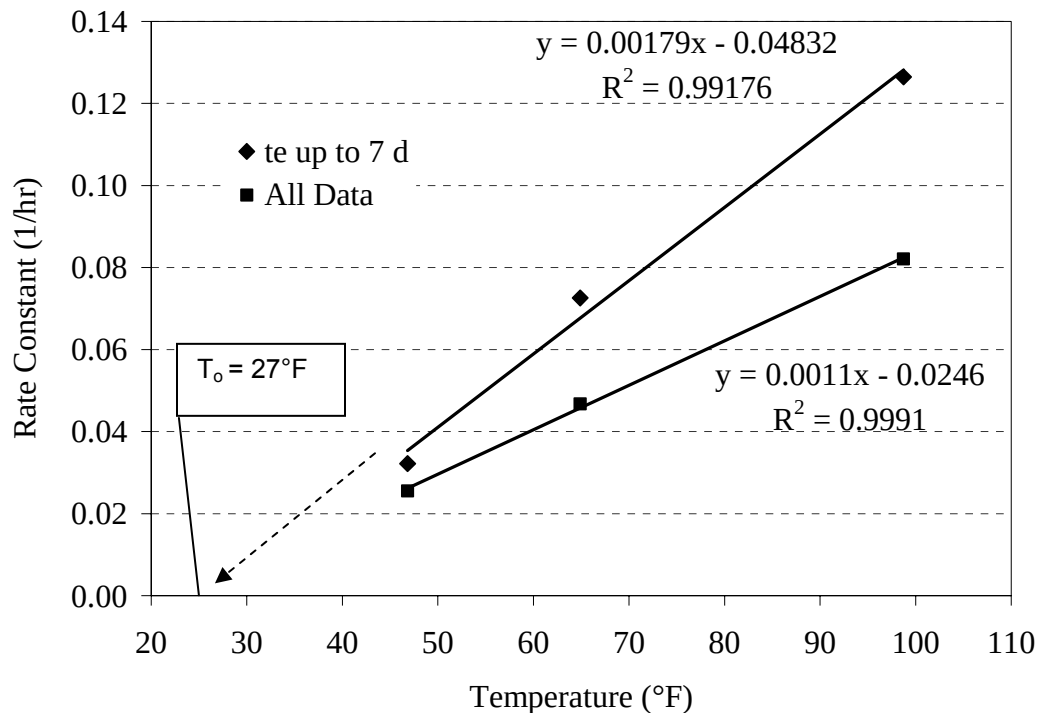
Figure 6.15: Change in rate values and datum temperature for Type I - 0.41 mixture
