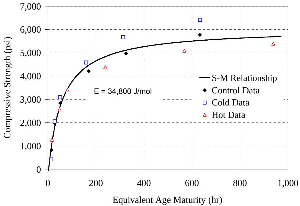
Figure C-1: Strength-maturity plot, ASTM C 1074 method for Type I - 0.44 mixture
