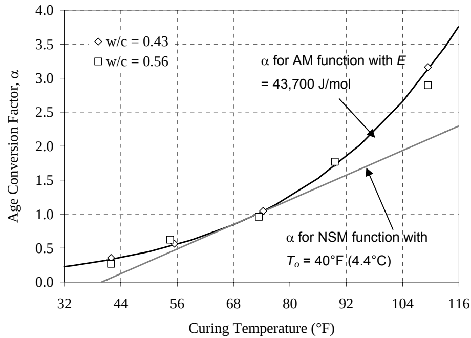
Figure 2.19: Age conversion factors with best-fit Nurse-Saul and Arrhenius age conversion factors (Carino 1991)
