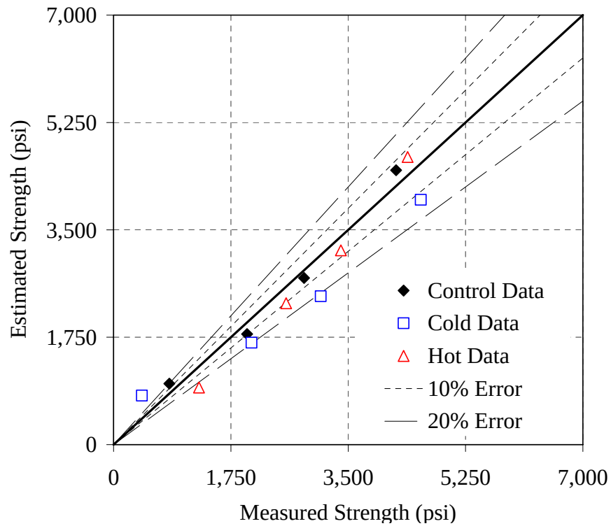
Figure G-2: Error plot for the Type I - 0.44 mixture, ASTM C 1074 method, NSM
