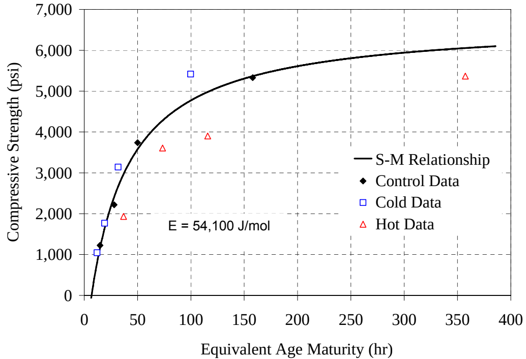
Figure F-4: Strength-maturity plot, Modified ASTM method for 20% C mixture
