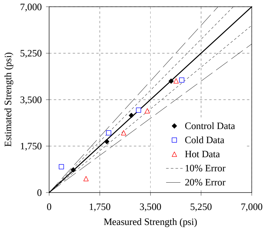
Figure H-1: Error plot for the Type I - 0.44 mixture, simplified method, T_o = 14^\circ\text{F}
