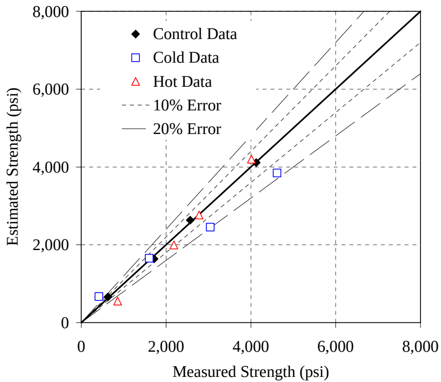
Figure G-3: Error plot for the Type I - 0.48 mixture, Modified method, NSM
