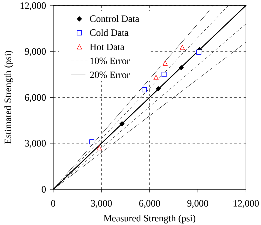
Figure 6.26: Error plot for the Type III - 0.37 mixture, Modified ASTM method, NSM
