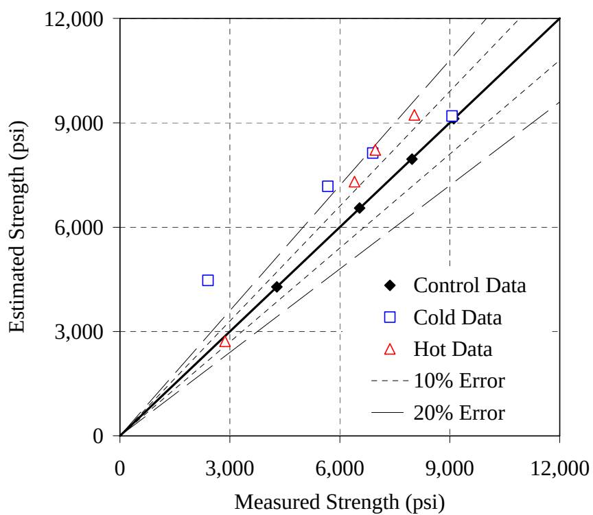
Figure 6.47: Error plot for the Type III - 0.37 mixture, simplified method, E = 25 kJ/mol
