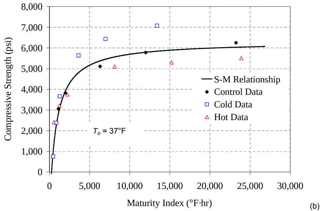
Figure B-8: Type III - 0.44 mixture, (a) compressive strength vs. age, (b) strength-maturity plot, ASTM C 1074 method
