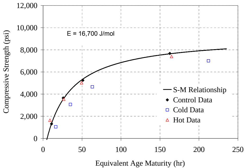
Figure F-9: Strength-maturity plot, Modified ASTM method for 70/20/10 - 0.37 mixture
