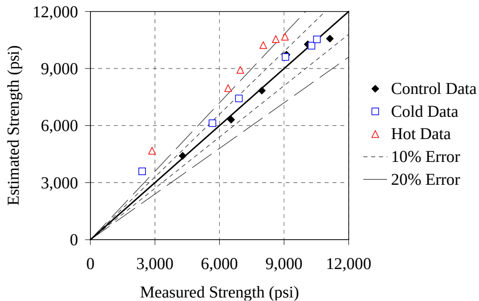
Figure 6.14: Estimated strength versus actual strength for the Type III - 0.37 mixture
