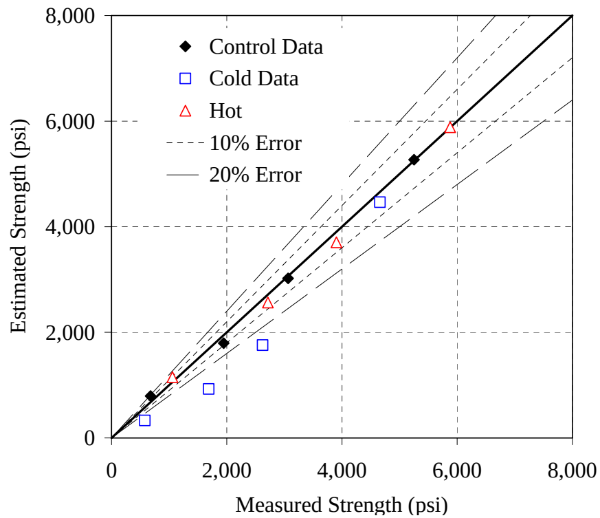
Figure G-10: Error plot for the 30% C mixture, ASTM C 1074 method, NSM
