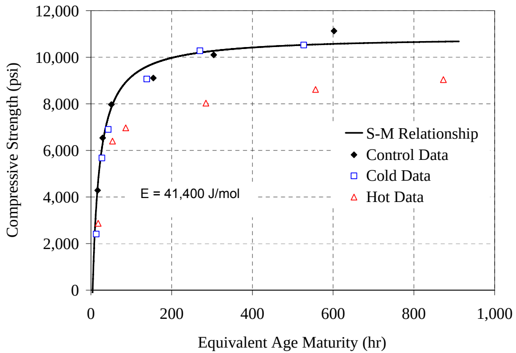
Figure 6.8: Strength-maturity plot, ASTM C 1074 method for Type III - 0.37 mixture
