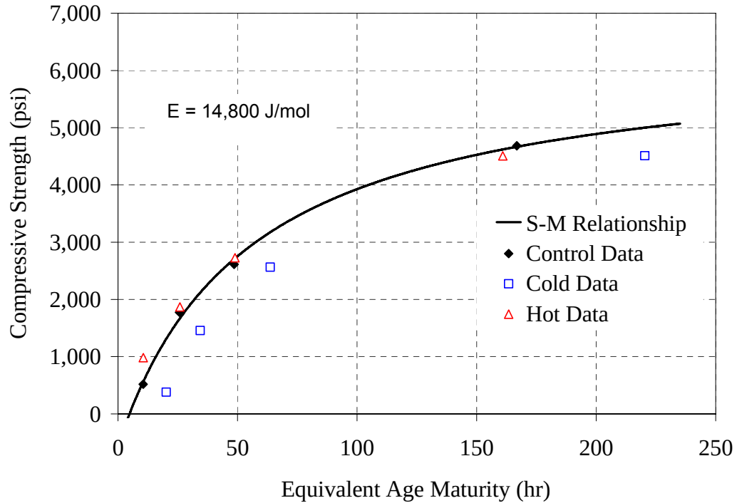
Figure F-10: Strength-maturity plot, Modified ASTM method for 70/20/10-0.44 mixture
