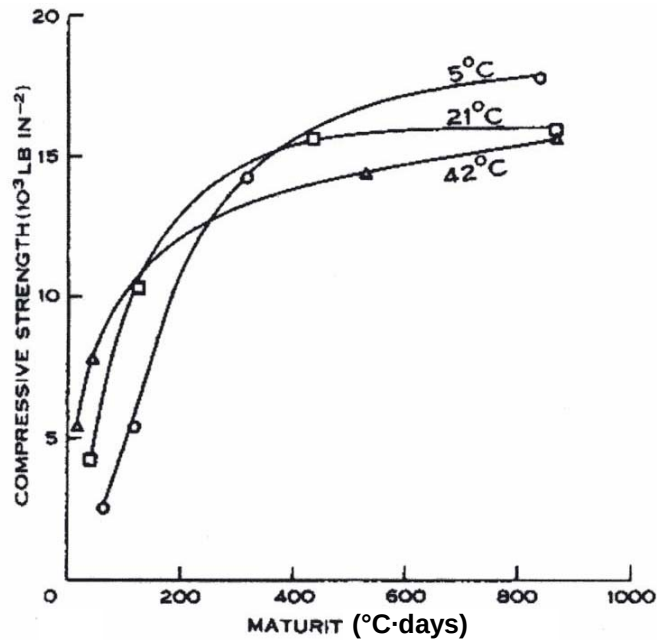
Figure 2.13: Crossover effect due to curing temperatures (Alexander and Taplin 1962)
