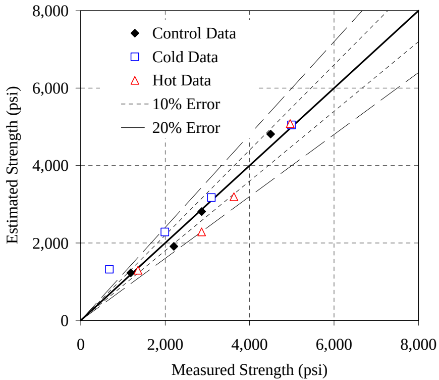
Figure G-26: Error plot for the 30% F mixture, ASTM C 1074 method, AM
