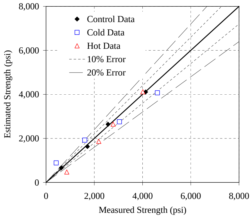
Figure H-3: Error plot for the Type I - 0.48 mixture, simplified method, T_o = 14^\circ\text{F}
