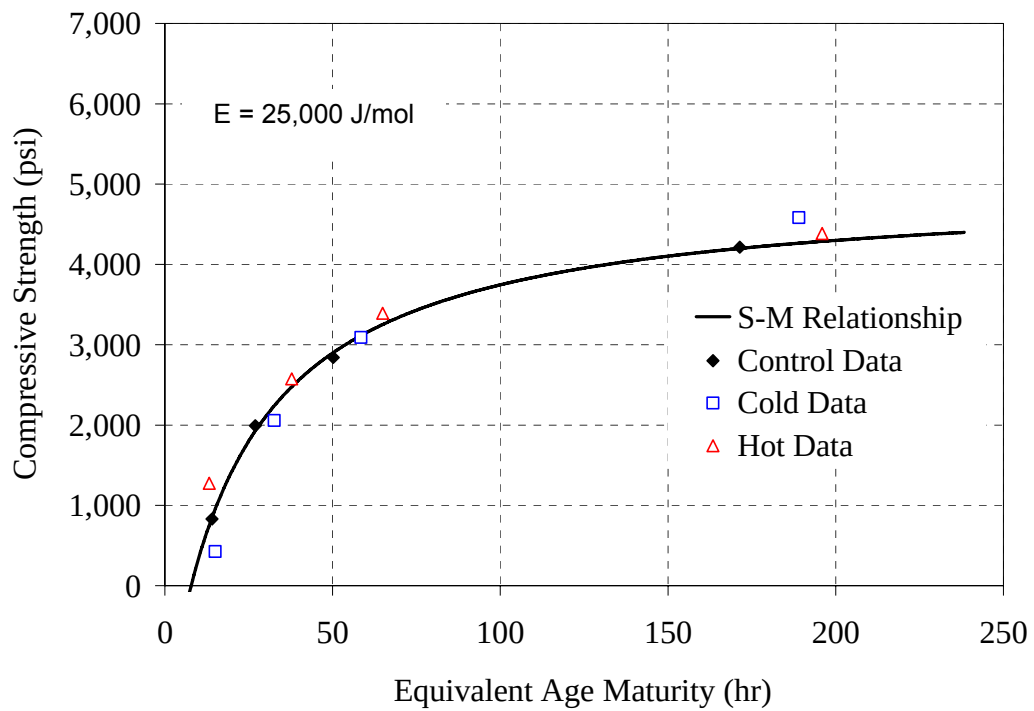
Figure F-1: Strength-maturity plot, Modified ASTM method for Type I - 0.44 mixture
