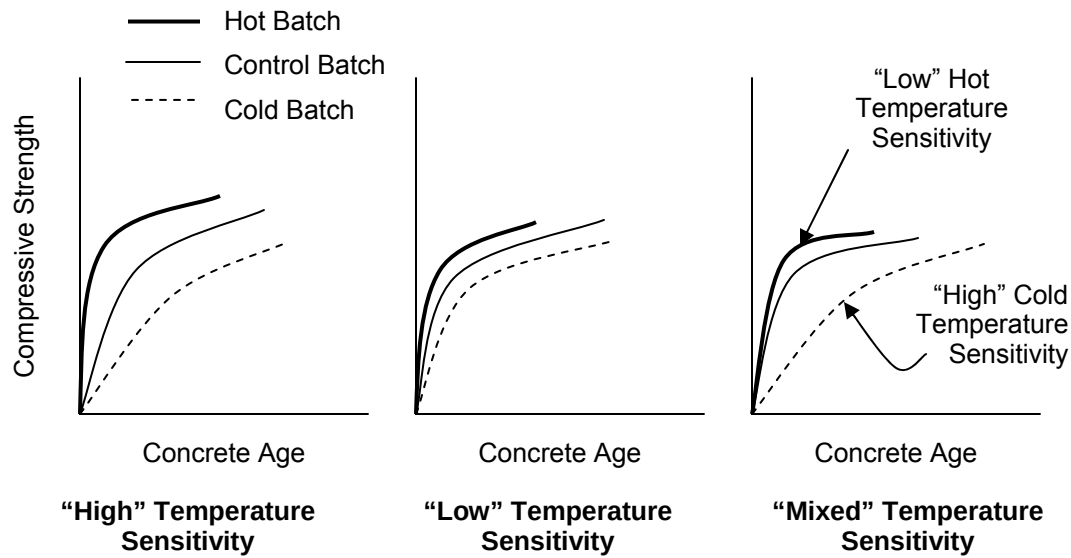
Figure 5.15: Schematic of various degrees of temperature sensitivity
