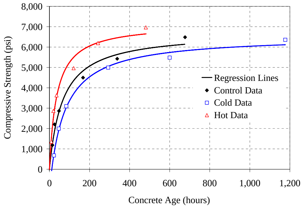
Figure 5.6: Compressive strength versus age results for 30% F mixture
