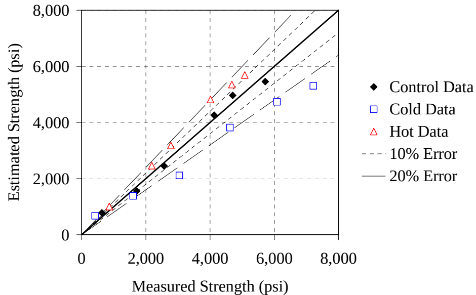
Figure D-12: Estimated strength versus actual strength for Type I - 0.48 mixture
