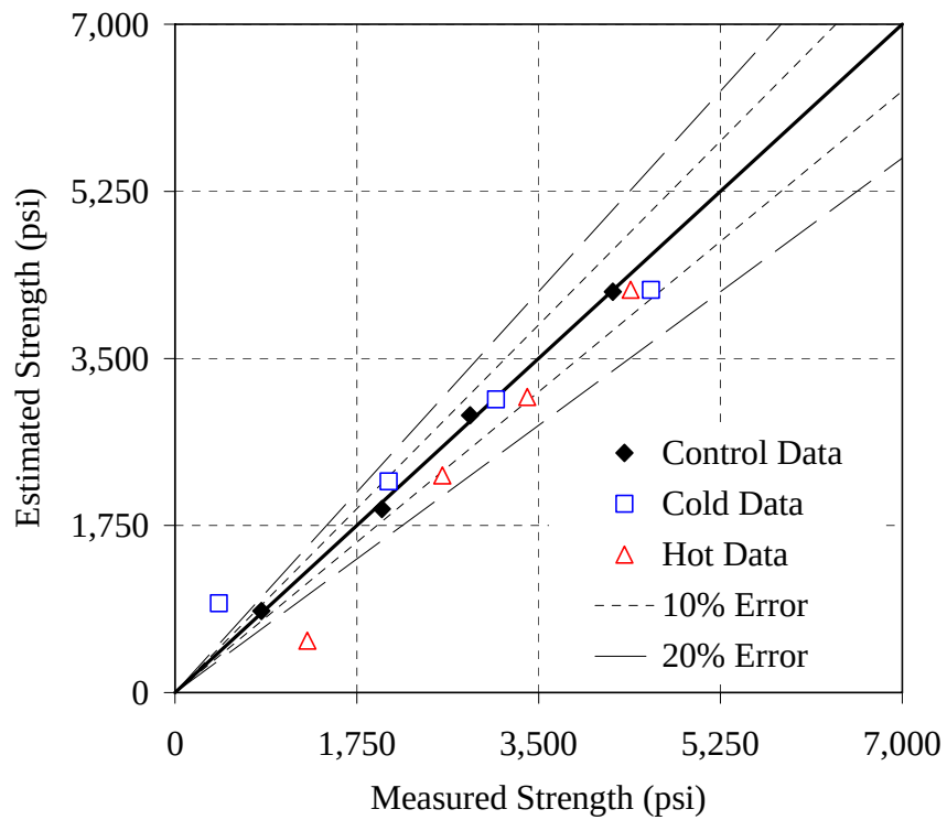
Figure G-1: Error plot for the Type I - 0.44 mixture, Modified method, NSM
