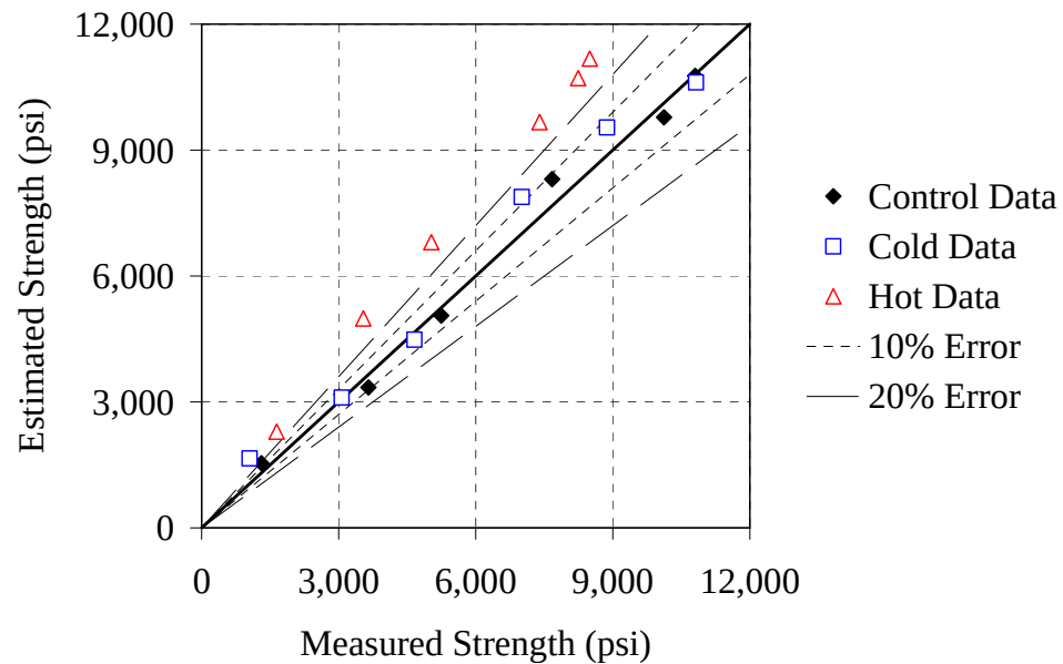
Figure D-19: Estimated strength versus actual strength for 70/20/10 - 0.37 mixture
