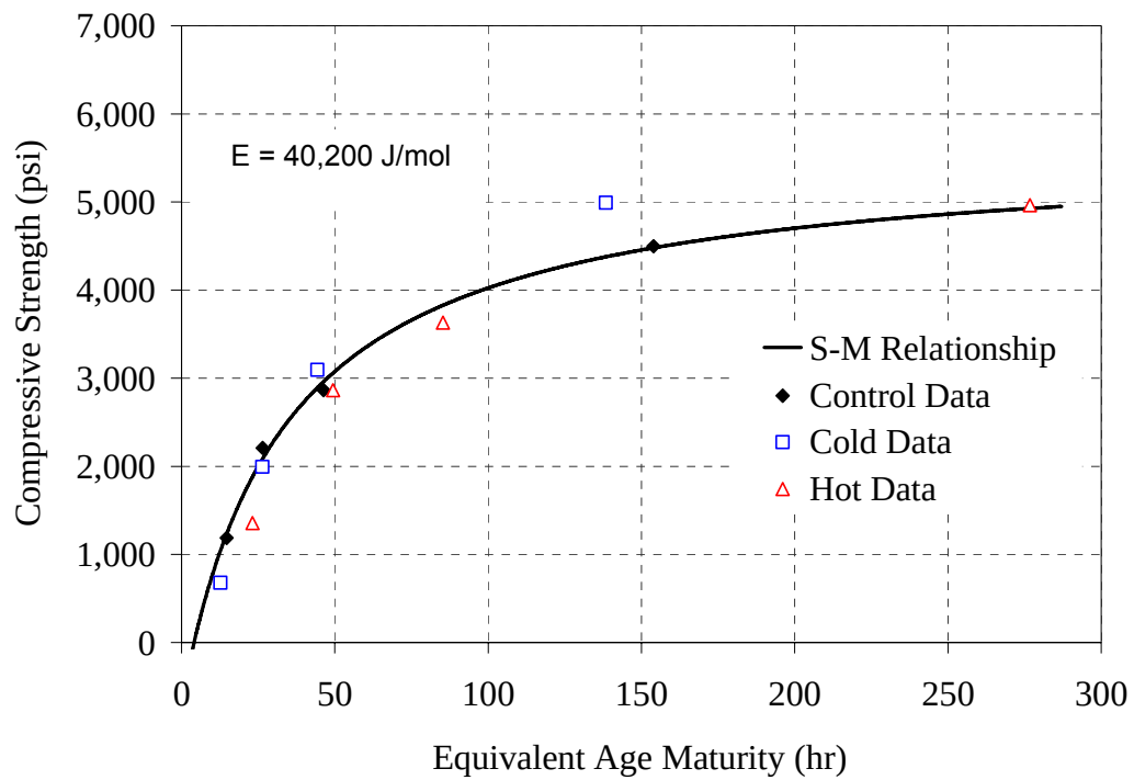
Figure F-3: Strength-maturity plot, Modified ASTM method for 30% F mixture
