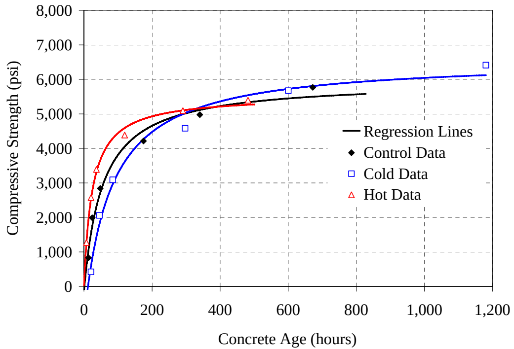
Figure 5.3: Compressive strength versus age results for Type I - 0.44 mixture
