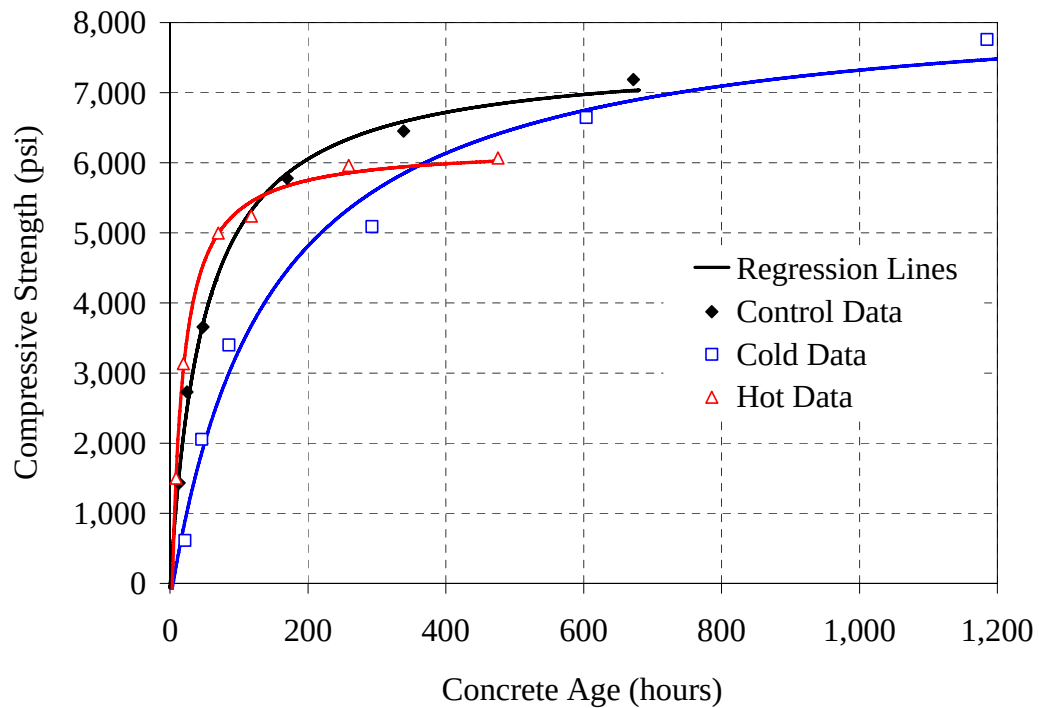
Figure 5.9: Compressive strength versus age results for 30% Slag mixture
