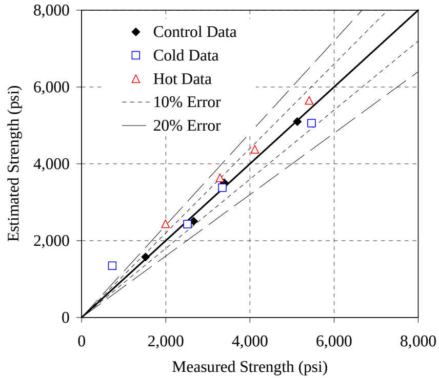
Figure 6.42: Error plot for the 20% F mixture, simplified method, E = 40 kJ/mol
