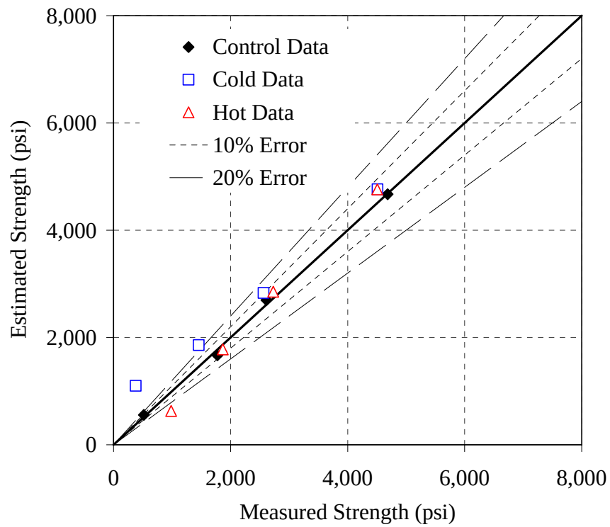
Figure H-19: Error plot for the 70/20/10 - 0.44 mixture, simplified method, T_o = 14^\circ\text{F}
