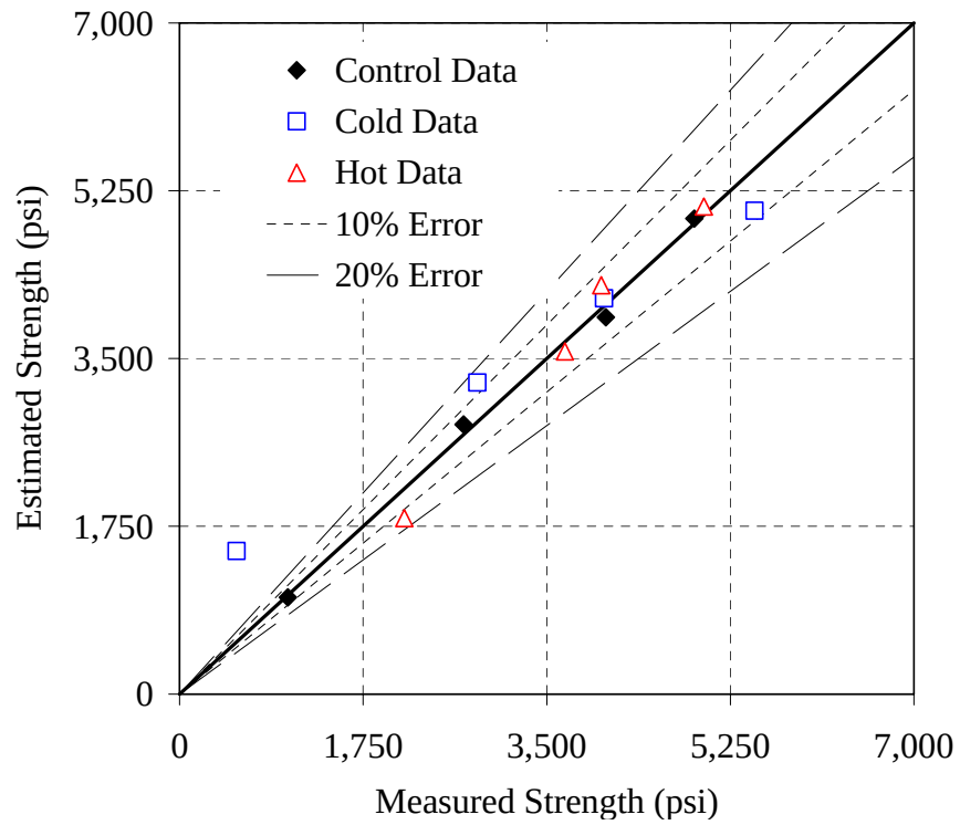
Figure 6.45: Error plot for the Type I - 0.41 mixture, simplified method, E = 25 kJ/mol
