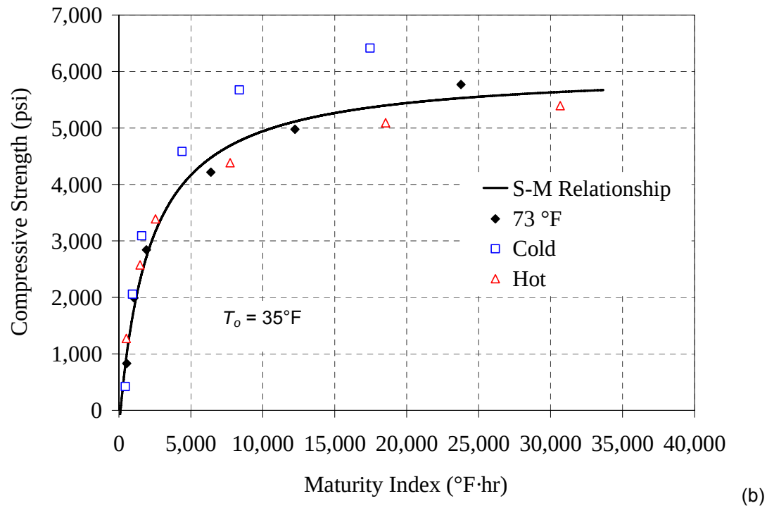
Figure B-1: Type I - 0.44 mixture, (a) compressive strength vs. age, (b) strength-maturity plot, ASTM C 1074 method
