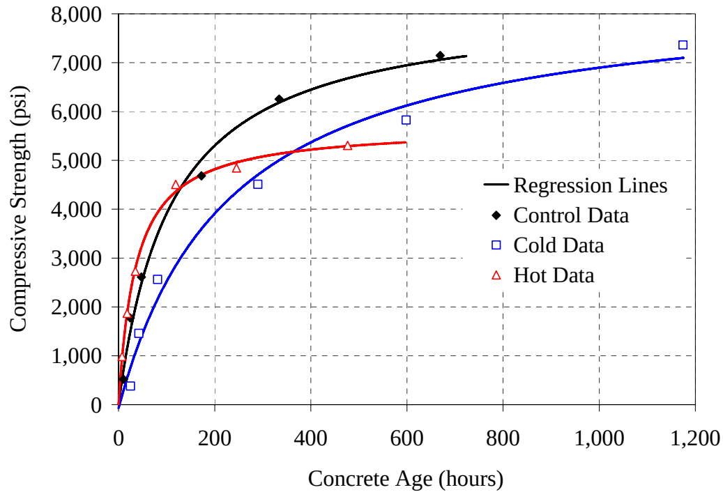
Figure 5.14: Compressive strength versus age results for 70/20/10 - 0.44 mixture
