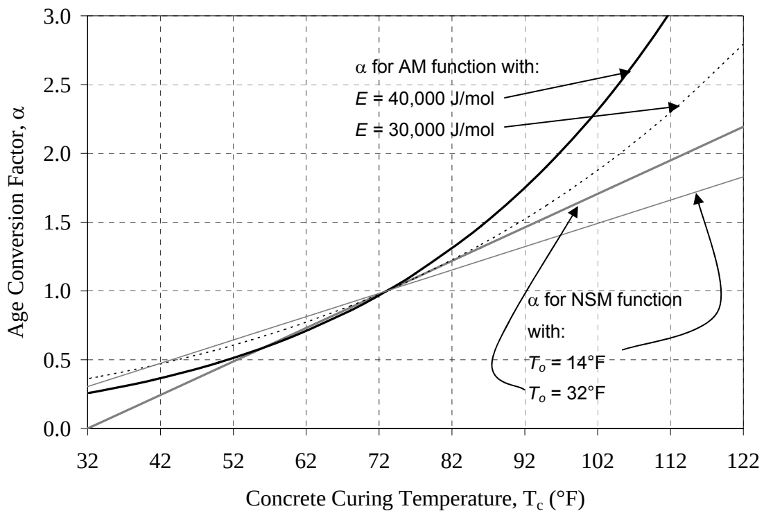
Figure 2.16: Age conversion factors for Nurse-Saul and Arrhenius maturity functions
