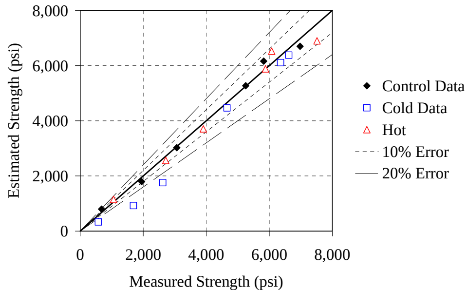
Figure D-5: Estimated strength versus actual strength for 30% C mixture
