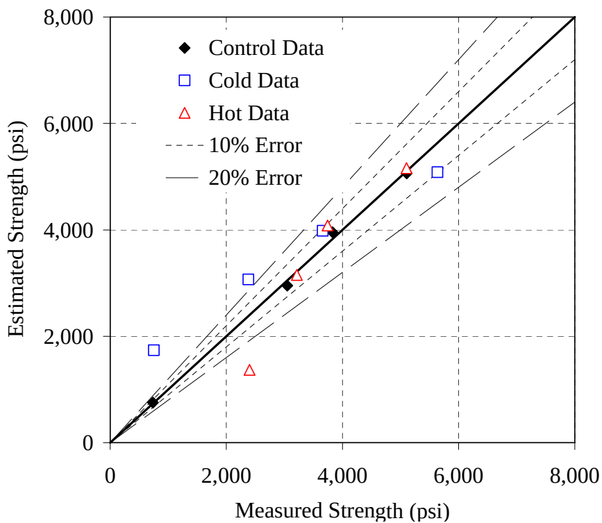
Figure I-16: Error plot for the Type III - 0.44 mixture, simplified method, E = 25 kJ/mol
