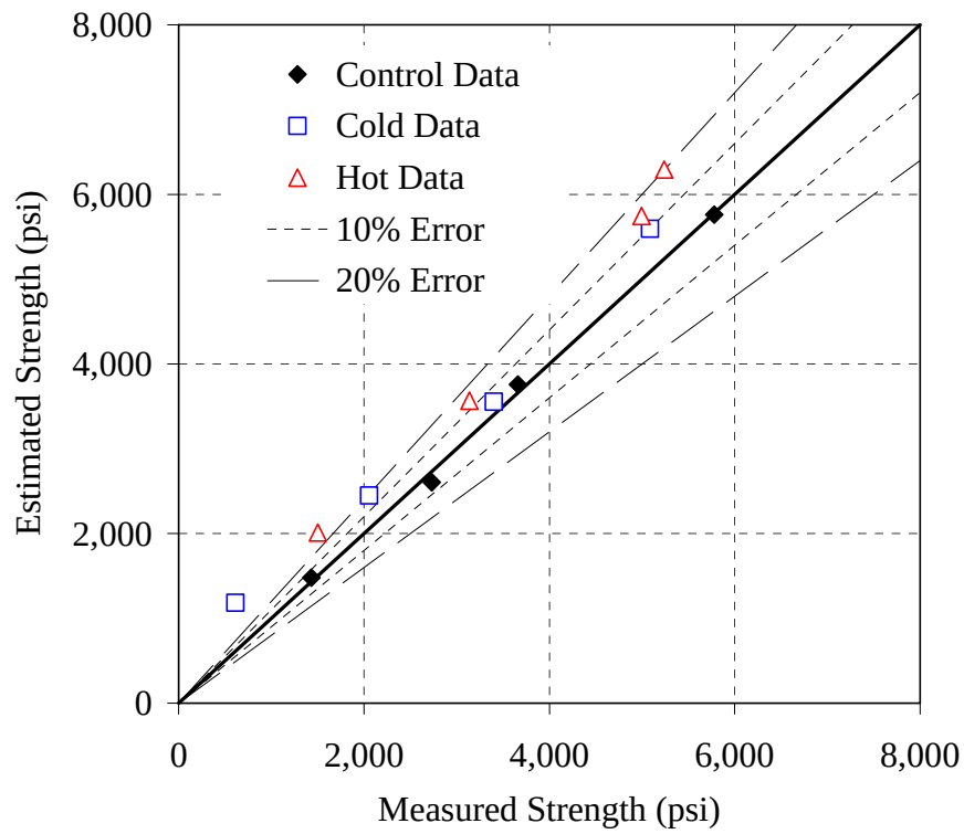
Figure G-31: Error plot for the 30% Slag mixture, Modified method, AM
