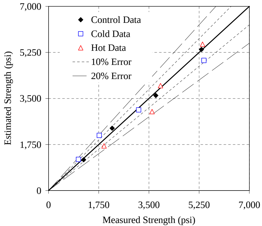
Figure H-8: Error plot for the 20% C mixture, simplified method, T_o = 32^\circ\text{F}
