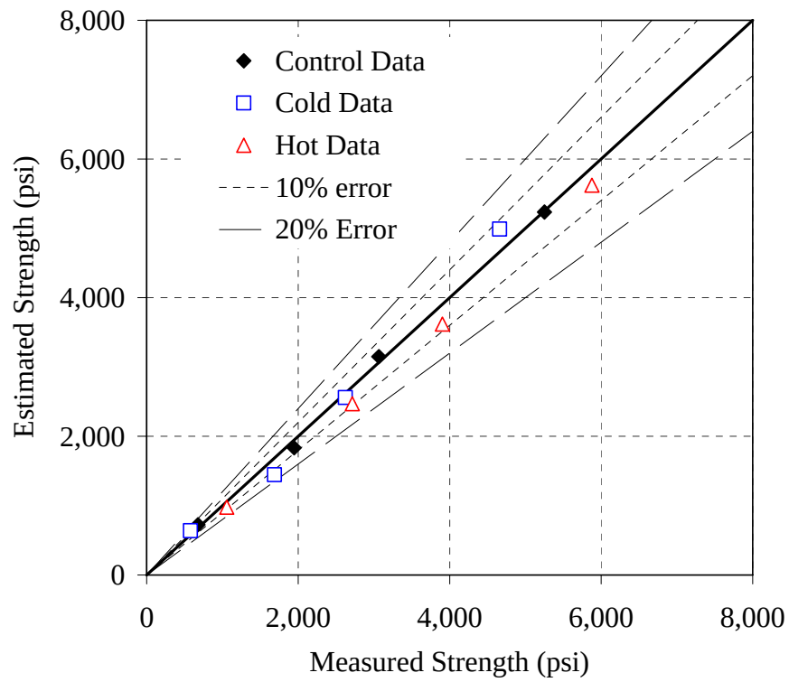
Figure G-9: Error plot for the 30% C mixture, Modified method, NSM
