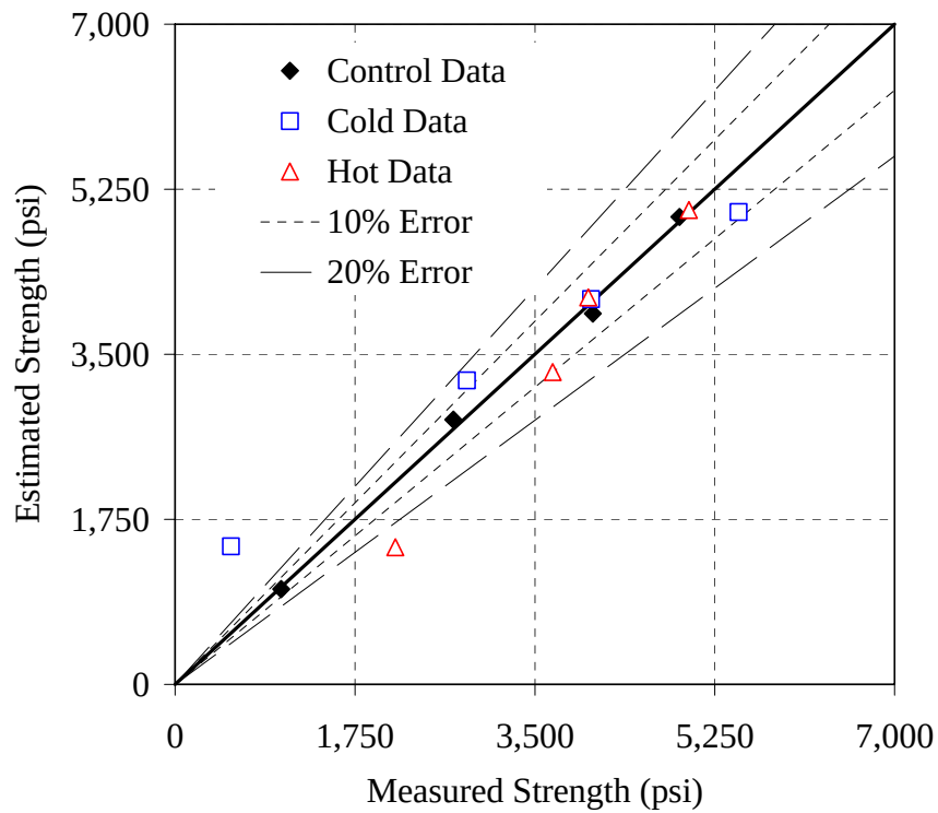
Figure 6.38: Error plot for the Type I - 0.41 mixture, simplified method, T_o = 14^\circ\text{F}
