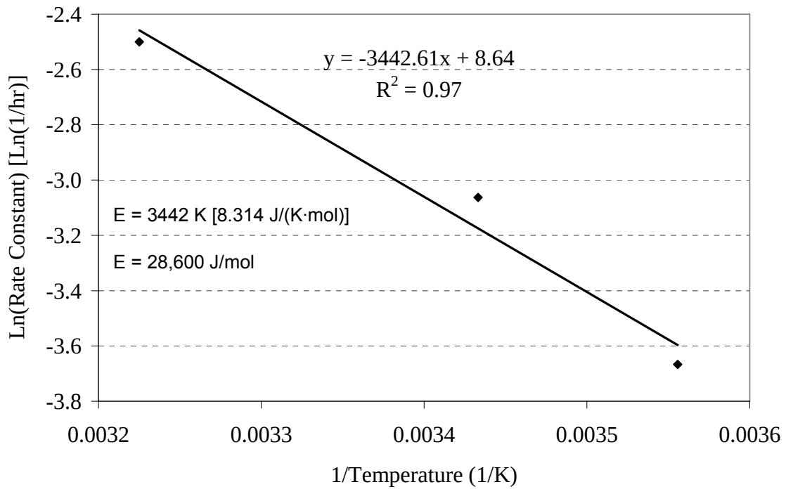
Figure 6.5: Method for computing activation energy based on ASTM C 1074 for the Type I - 0.41 mixture
