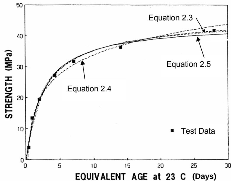
Figure 2.5: Various strength-maturity functions (Carino 1991)
