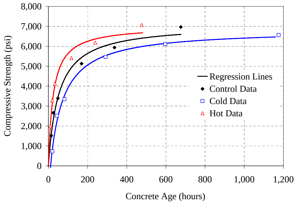
Figure 5.5: Compressive strength versus age results for 20% F mixture
