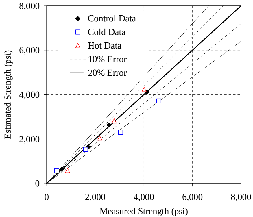
Figure H-4: Error plot for the Type I - 0.48 mixture, simplified method, T_o = 32^\circ\text{F}
