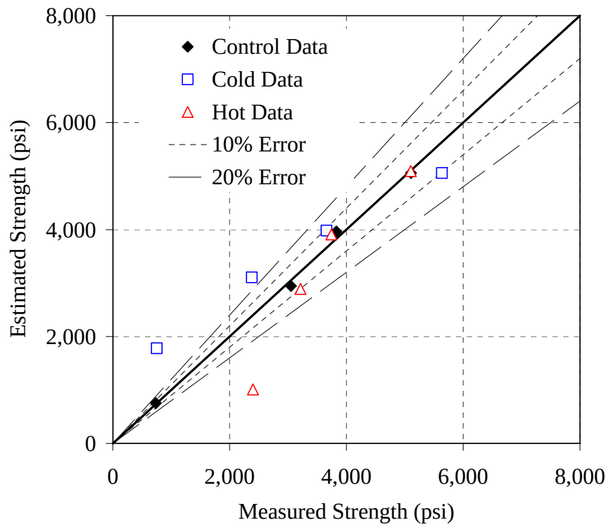
Figure H-15: Error plot for the Type III - 0.44 mixture, simplified method, T_o = 14^\circ\text{F}
