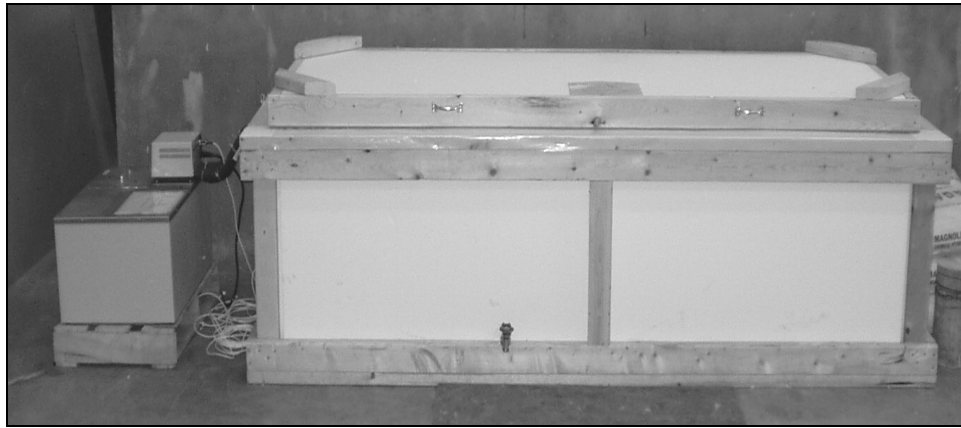
Figure 3.1: Curing tank and programmable heating/cooling circulator
