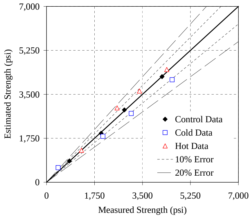
Figure I-1: Error plot for the Type I - 0.44 mixture, simplified method, E = 40 kJ/mol
