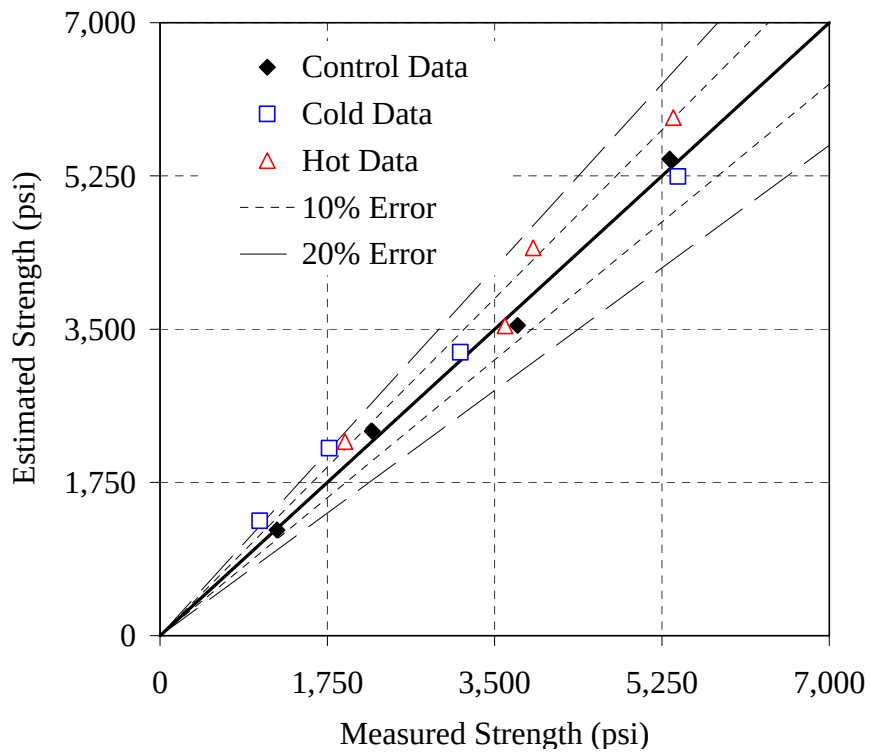
Figure G-28: Error plot for the 20% C mixture, ASTM C 1074 method, AM
