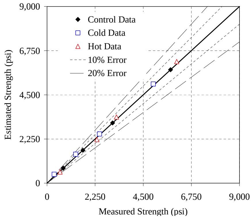
Figure H-14: Error plot for the 50% Slag mixture, simplified method, T_o = 32^\circ\text{F}
