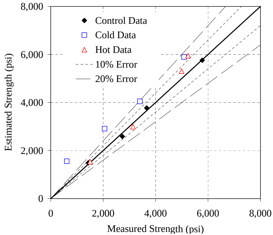
Figure I-12: Error plot for the 30% Slag mixture, simplified method, E = 25 kJ/mol
