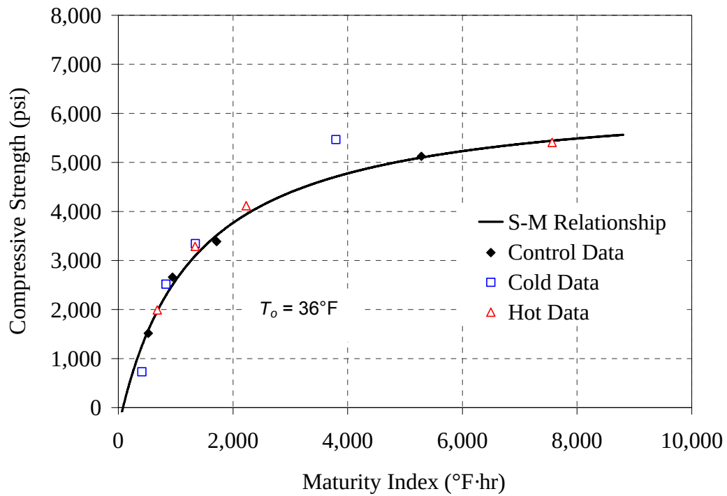
Figure 6.16: Strength-maturity plot, Modified ASTM method for 20% F mixture
