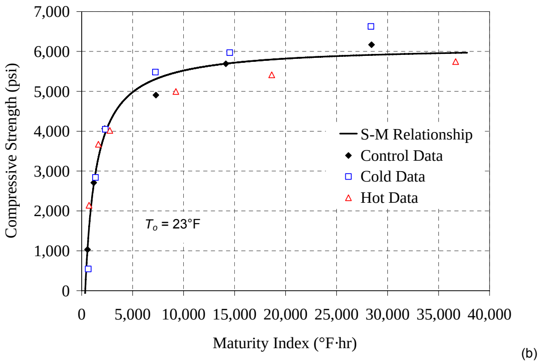
Figure 6.3: Type I - 0.41 mixture, (a) compressive strength versus age, (b) strength-maturity plot, ASTM C 1074 method
