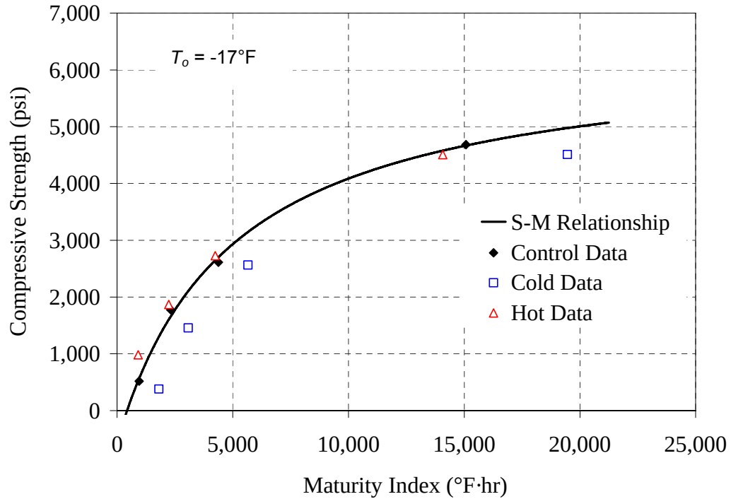
Figure E-10: Strength-maturity plot, Modified ASTM method for 70/20/10-0.44 mixture
