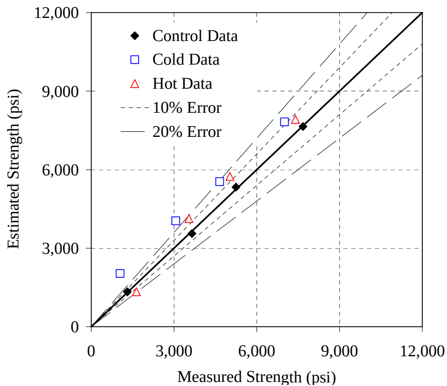
Figure I-18: Error plot for the 70/20/10 - 0.37 mixture, simplified method, E = 25 kJ/mol
