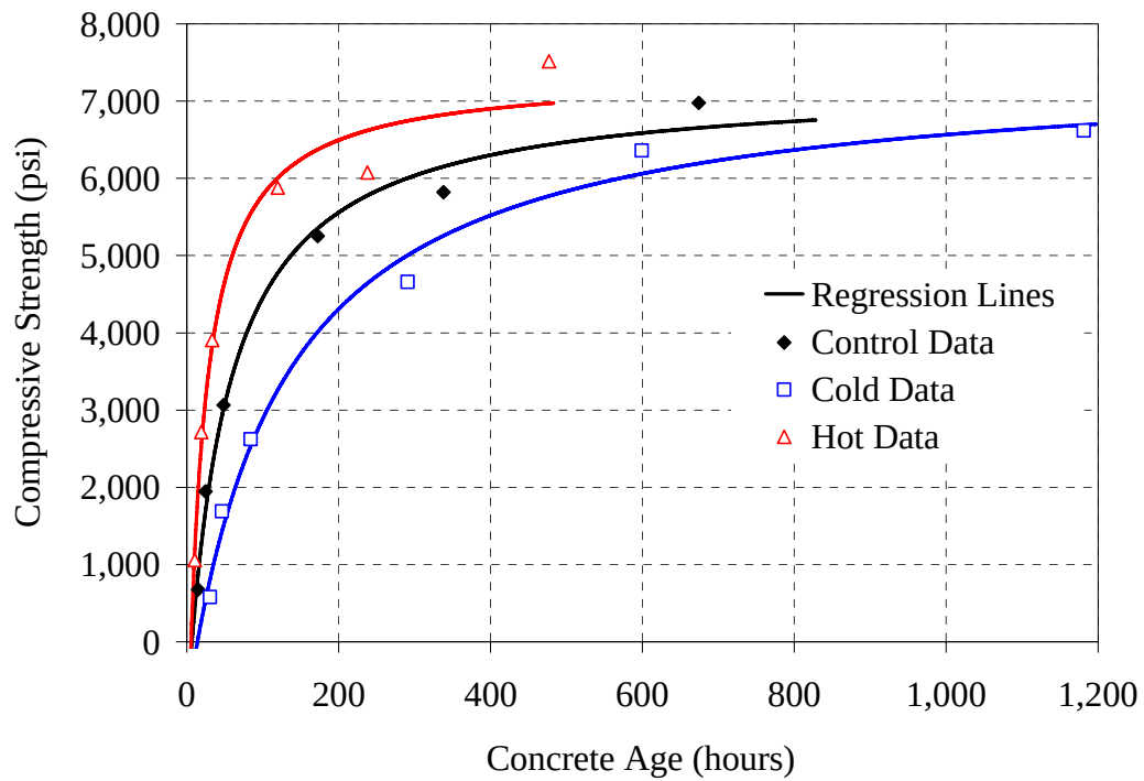
Figure 5.8: Compressive strength versus age results for 30% C mixture
