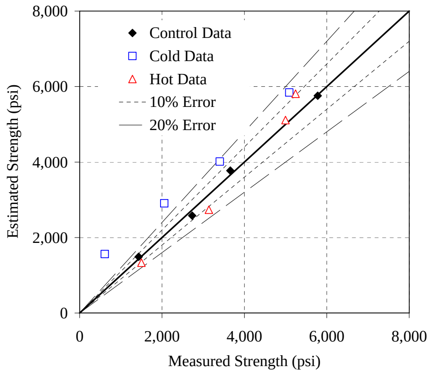
Figure H-11: Error plot for the 30% Slag mixture, simplified method, T_o = 14^\circ\text{F}
