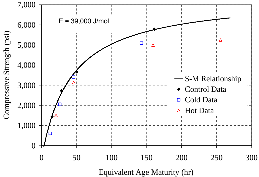
Figure F-6: Strength-maturity plot, Modified ASTM method for 30% Slag mixture
