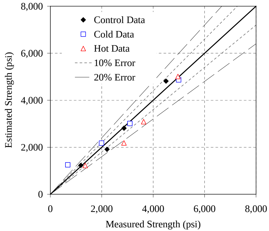
Figure G-6: Error plot for the 30% F mixture, ASTM C 1074 method, NSM
