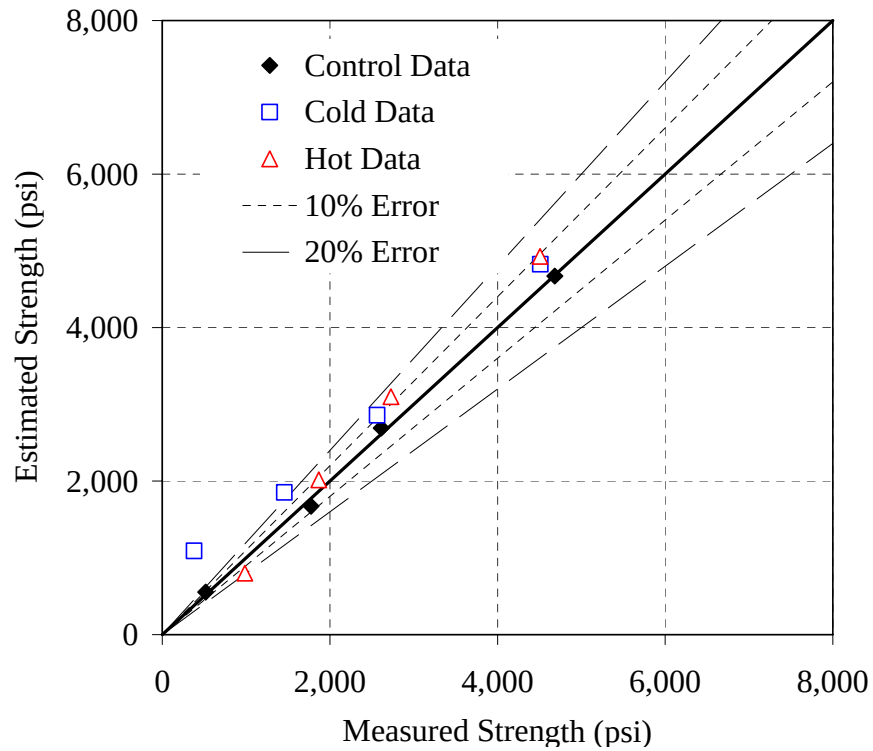
Figure I-20: Error plot for the 70/20/10 - 0.44 mixture, simplified method, E = 25 kJ/mol
