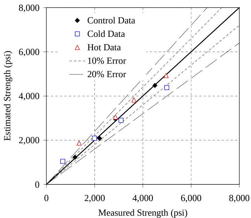
Figure I-5: Error plot for the 30% F mixture, simplified method, E = 40 kJ/mol
