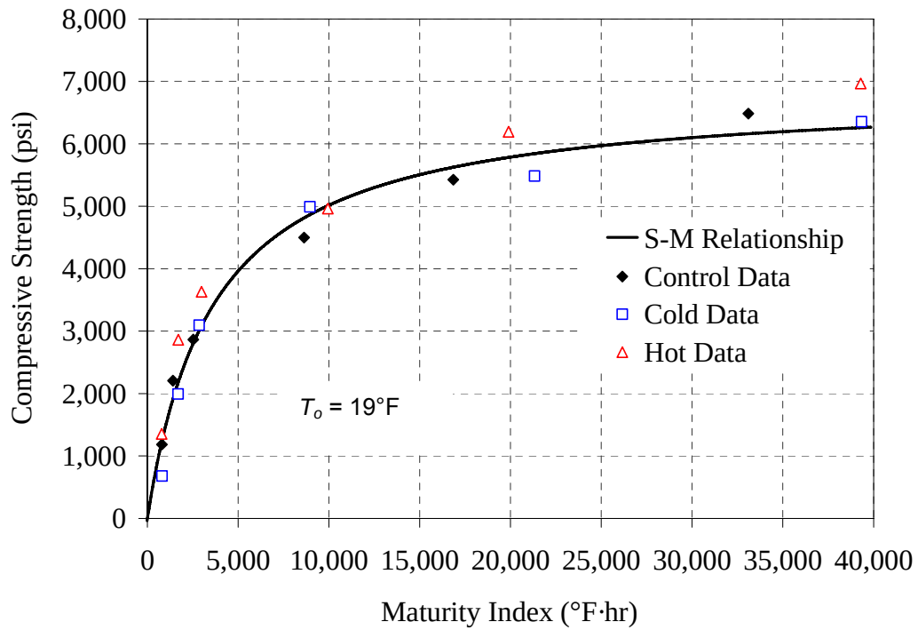
Figure B-3: 30% F mixture, (a) compressive strength vs. age, (b) strength-maturity plot, ASTM C 1074 method
