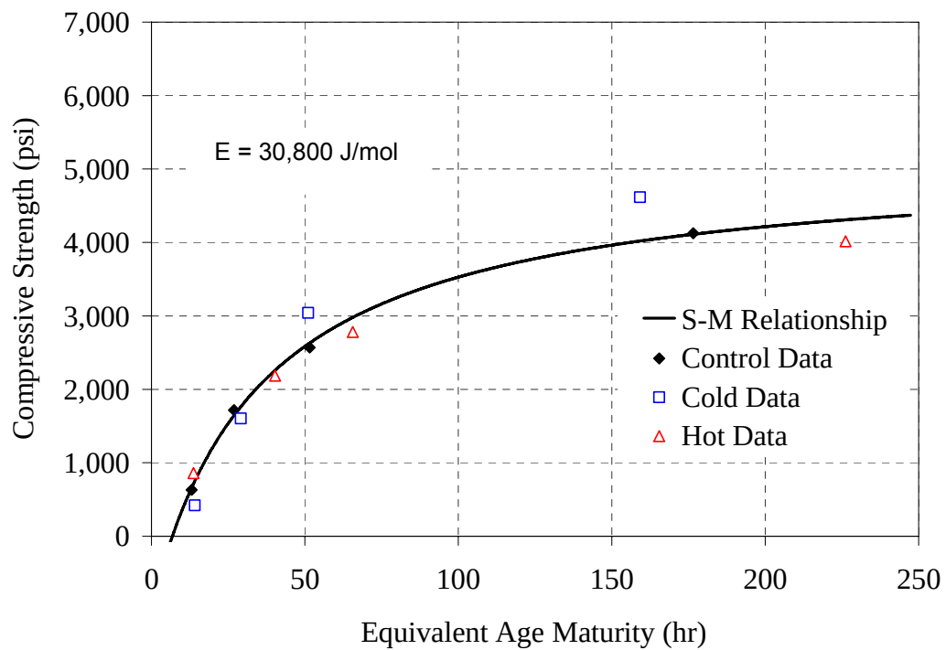
Figure F-2: Strength-maturity plot, Modified ASTM method for Type I - 0.48 mixture
