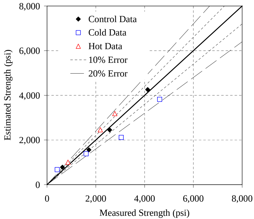
Figure G-24: Error plot for the Type I - 0.48 mixture, ASTM C 1074 method, AM
