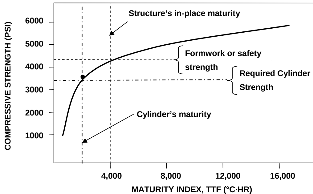
Figure 2.8: Example of verification of safety or formwork strength
