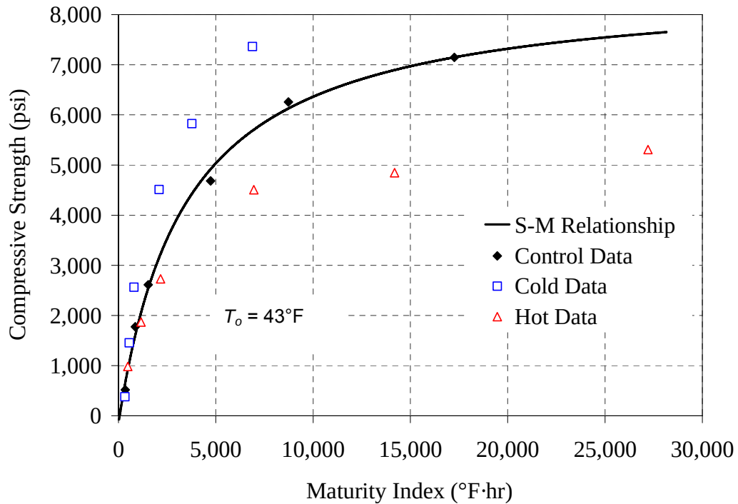
Figure B-10: 70/20/10 - 0.44 mixture, (a) compressive strength vs. age, (b) strength-maturity plot, ASTM C 1074 method
