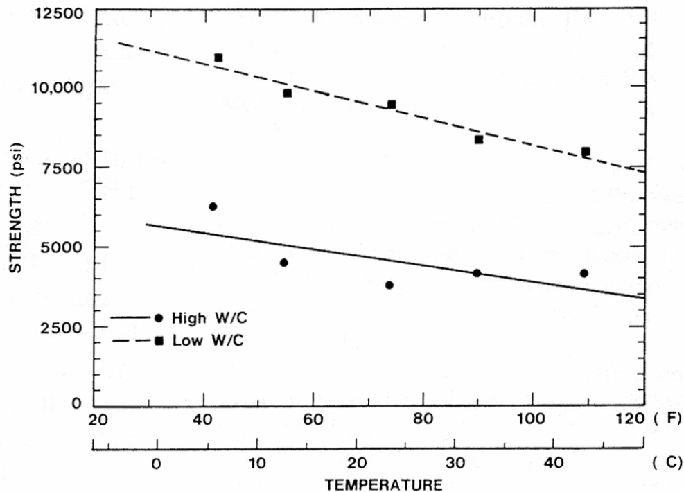
Figure 2.10: Ultimate compressive strength ( S_u ) values for Carino and Lew's experiment (1983)
