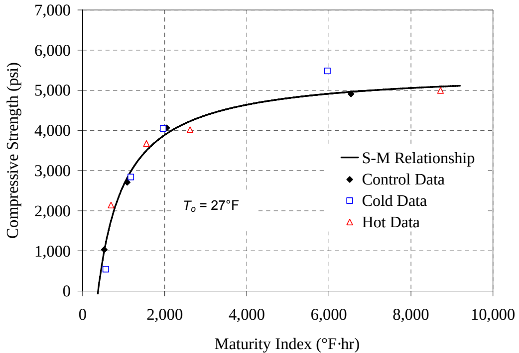
Figure 6.17: Strength-maturity plot, Modified ASTM method for Type I - 0.41
