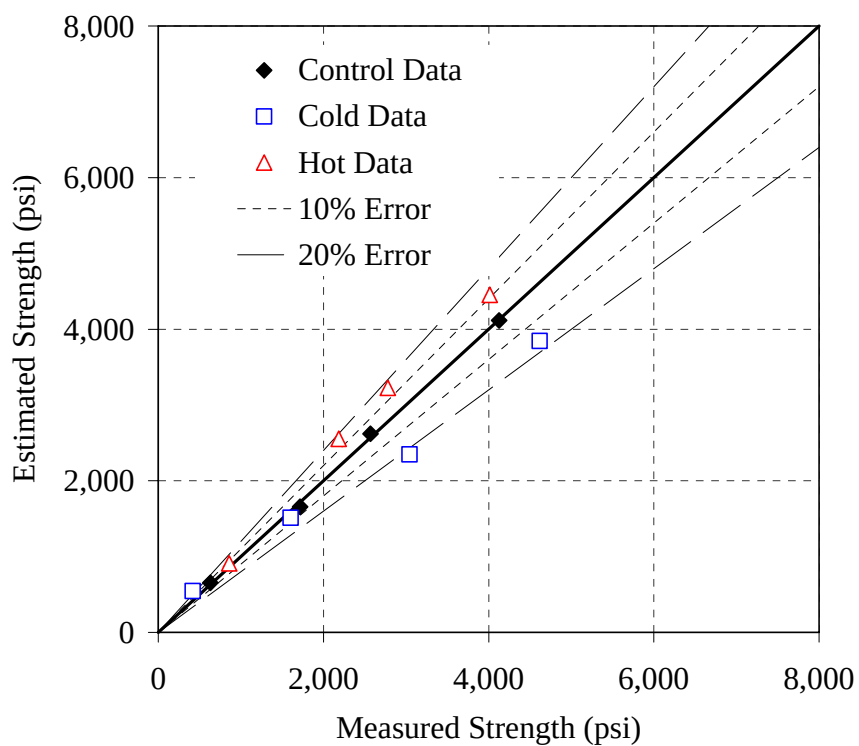
Figure I-3: Error plot for the Type I - 0.48 mixture, simplified method, E = 40 kJ/mol
