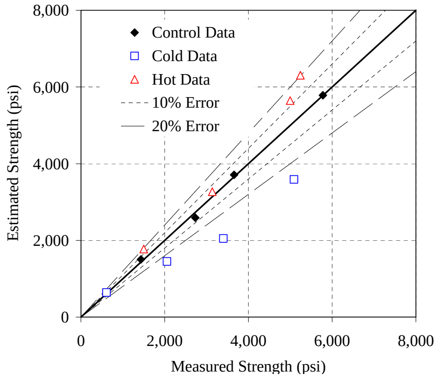
Figure G-12: Error plot for the 30% Slag mixture, ASTM C 1074 method, NSM
