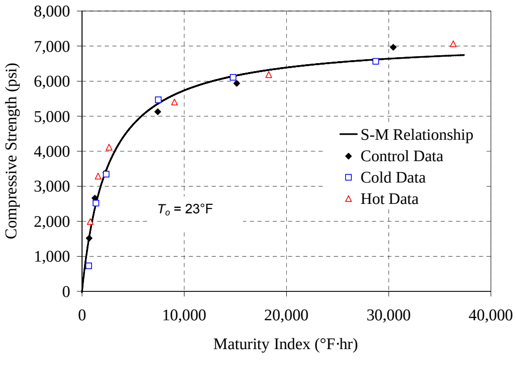
Figure 6.2: 20% F mixture, (a) compressive strength versus age, (b) strength-maturity plot, ASTM C 1074 method
