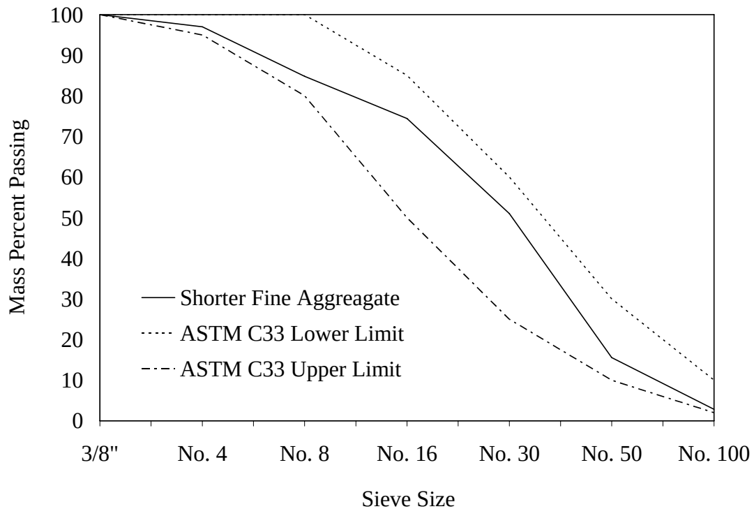
Figure 3.4: Gradation test results for Martin Marietta fine aggregate
