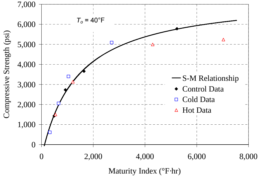
Figure E-6: Strength-maturity plot, Modified ASTM method for 30% Slag mixture
