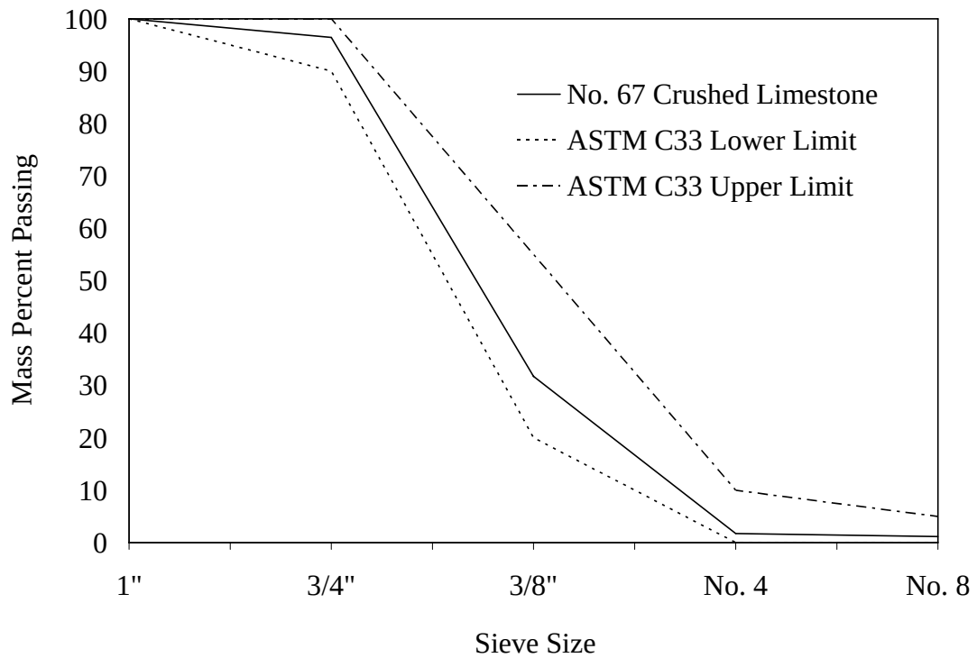
Figure 3.6: Gradation test results for Martin Marietta No. 67 Limestone
