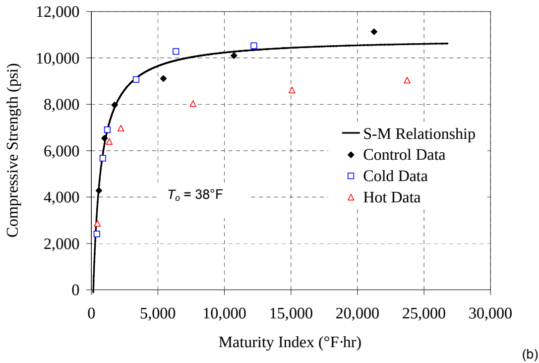
Figure 6.4: Type III - 0.37 mixture, (a) compressive strength versus age, (b) strength-maturity plot, ASTM C 1074 method
