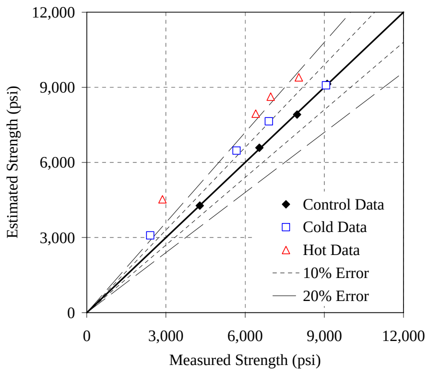
Figure 6.46: Error plot for the Type III - 0.37 mixture, simplified method, E = 40 kJ/mol
