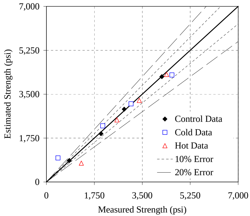
Figure G-21: Error plot for the Type I - 0.44 mixture, Modified method, AM
