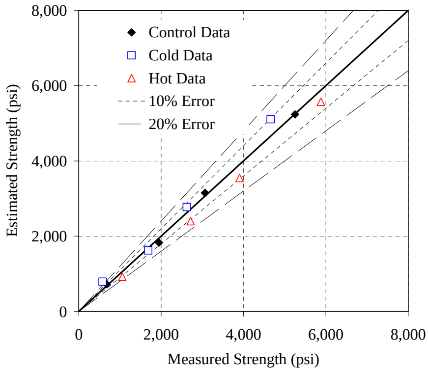
Figure H-10: Error plot for the 30% C mixture, simplified method, T_o = 32^\circ\text{F}
