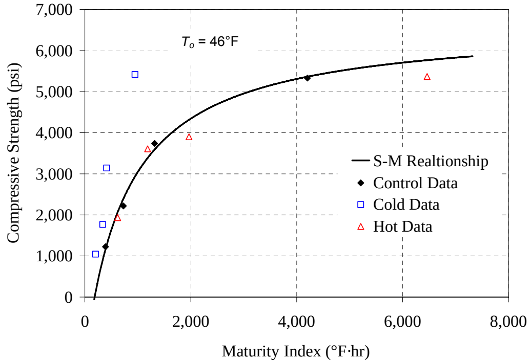
Figure E-4: Strength-maturity plot, Modified ASTM method for 20% C mixture
