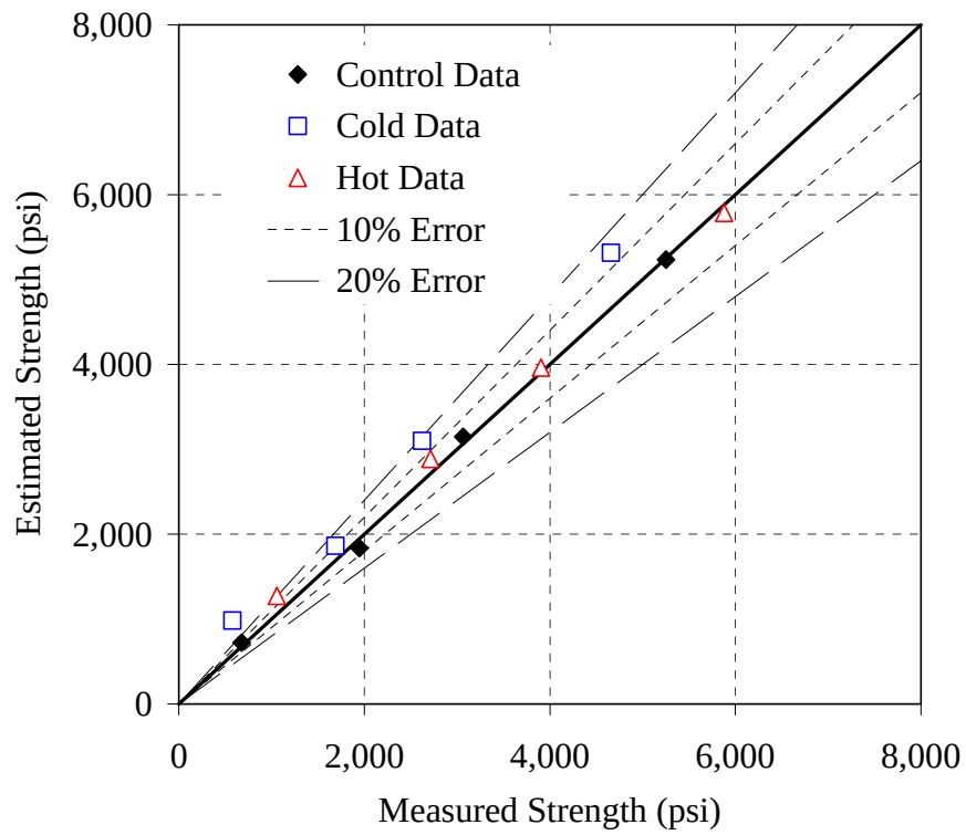
Figure G-29: Error plot for the 30% C mixture, Modified method, AM
