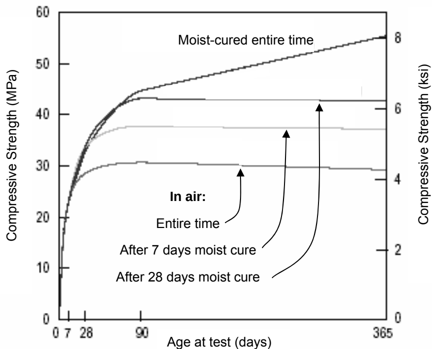
Figure 2.15: Effect of moist-curing time on strength gain of concrete (Gonnerman and Shuman 1928)
