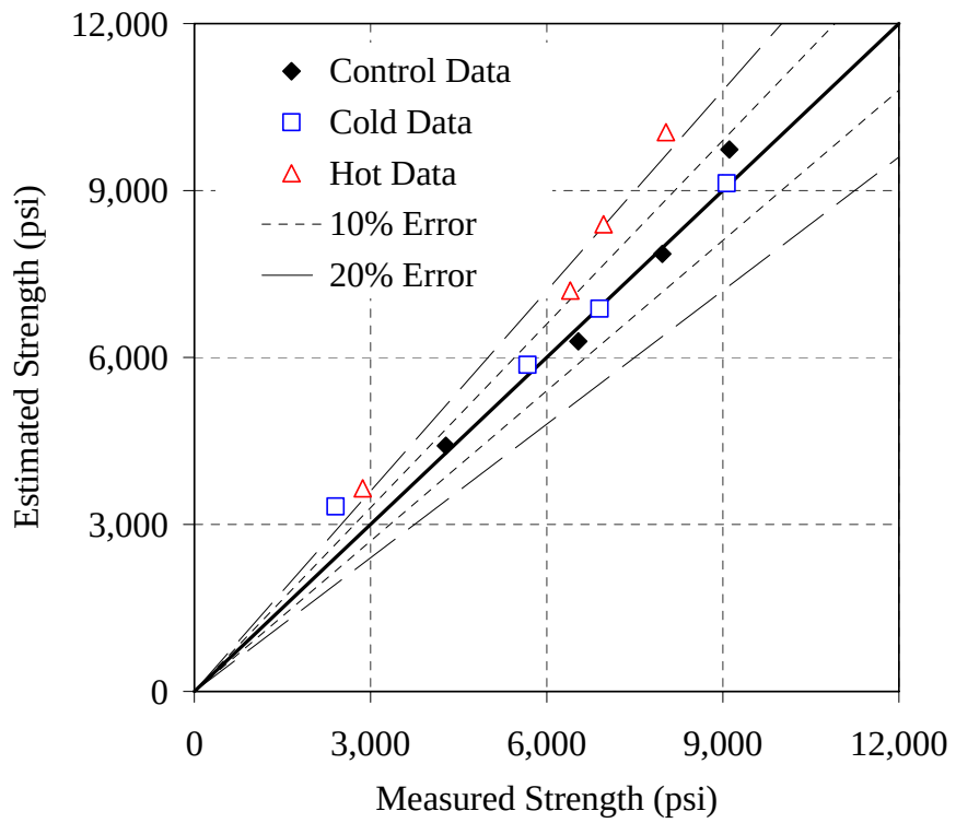
Figure 6.27: Error plot for the Type III - 0.37 mixture, ASTM C 1074 method, NSM
