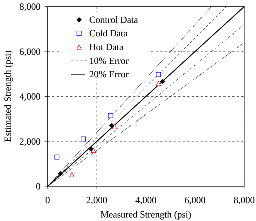
Figure G-19: Error plot for the 70/20/10 - 0.44 mixture, Modified method, NSM
