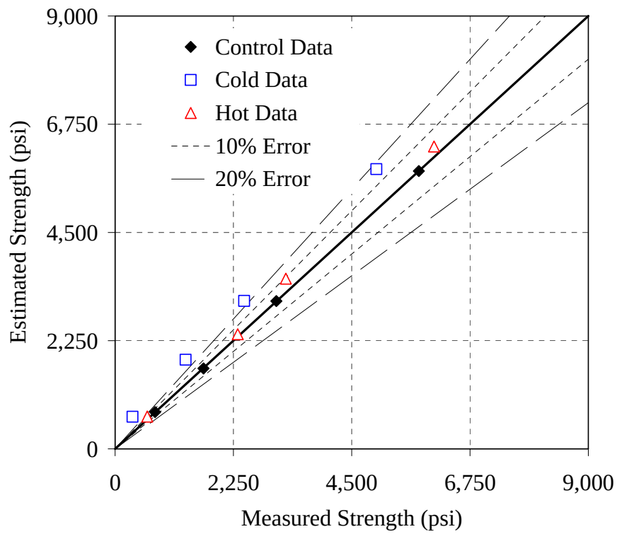
Figure G-33: Error plot for the 50% Slag mixture, Modified method, AM
