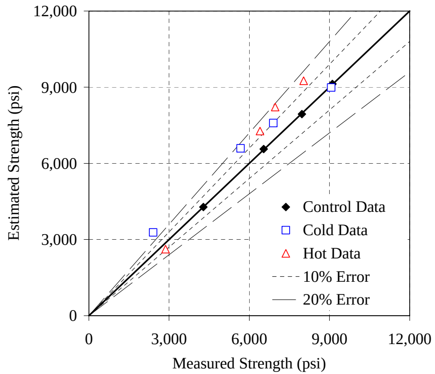
Figure 6.41: Error plot for the Type III - 0.37 mixture, simplified method, T_o = 32^\circ\text{F}
