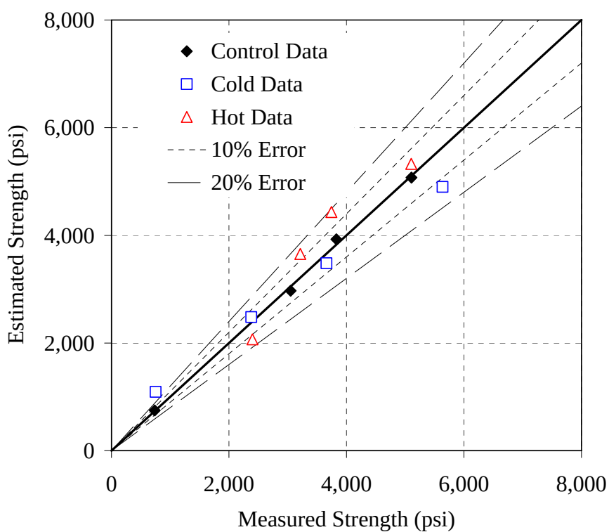
Figure I-15: Error plot for the Type III - 0.44 mixture, simplified method, E = 40 kJ/mol
