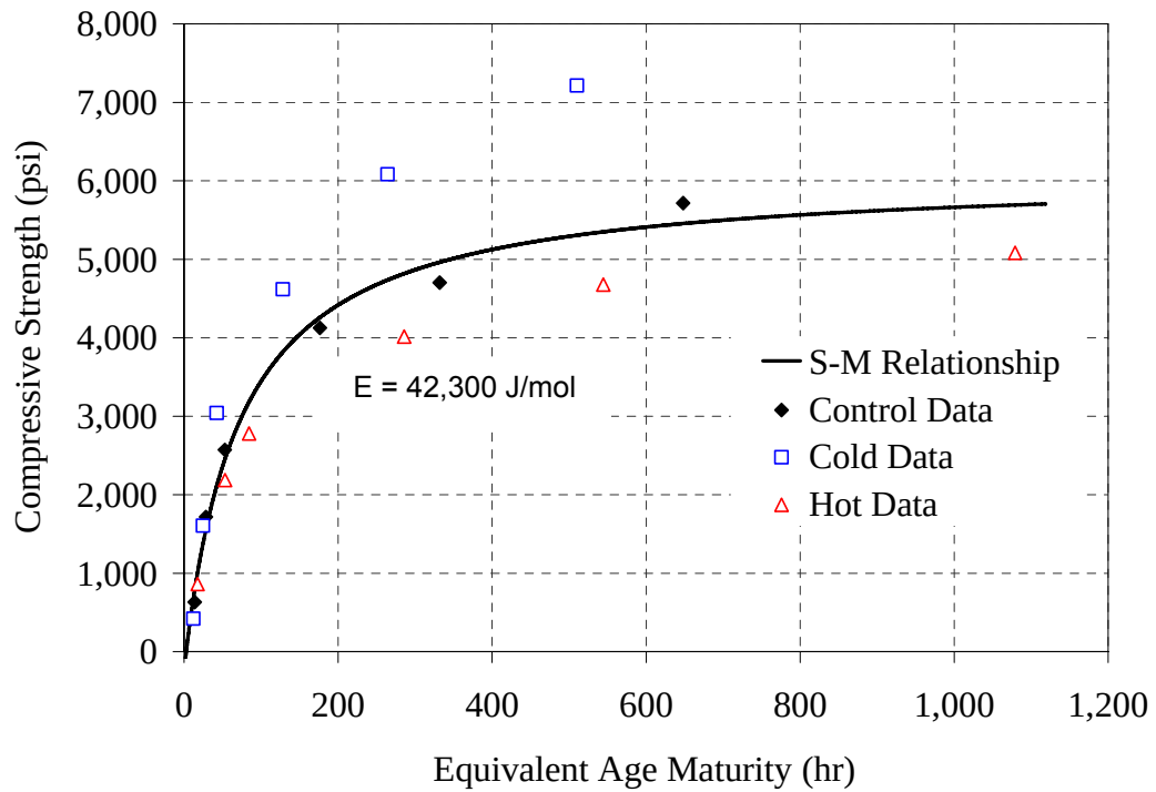
Figure C-2: Strength-maturity plot, ASTM C 1074 method for Type I - 0.48 mixture
