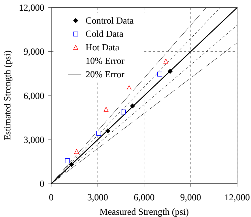
Figure I-17: Error plot for the 70/20/10 - 0.37 mixture, simplified method, E = 40 kJ/mol
