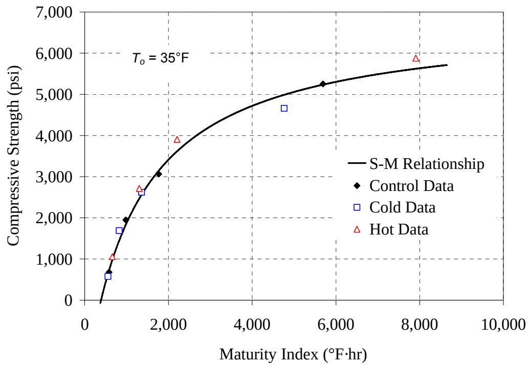
Figure E-5: Strength-maturity plot, Modified ASTM method for 30% C mixture
