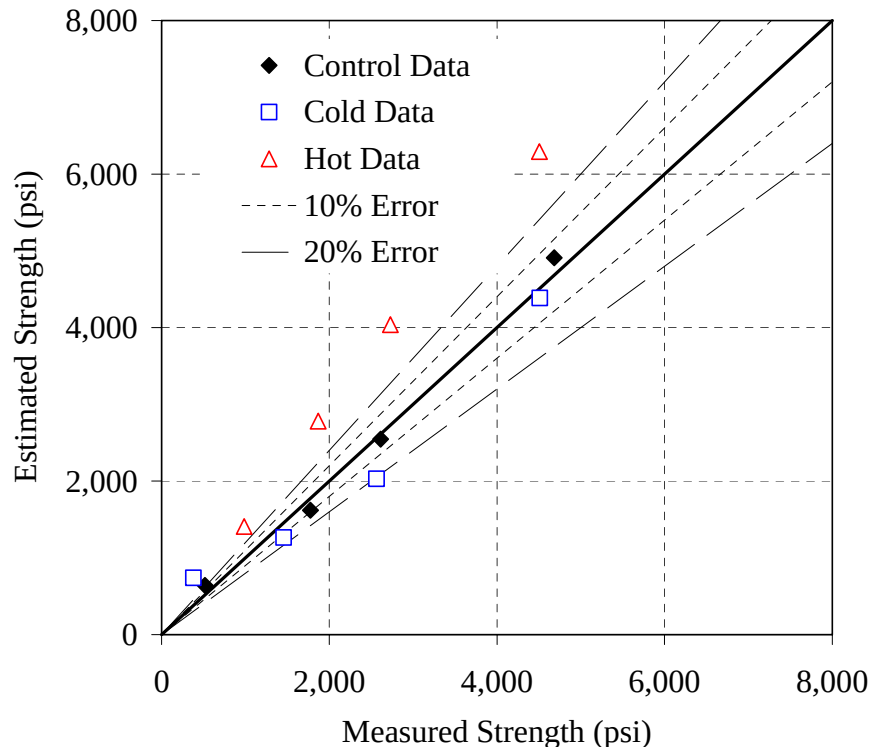
Figure G-40: Error plot for the 70/20/10 - 0.44 mixture, ASTM C 1074 method, AM
