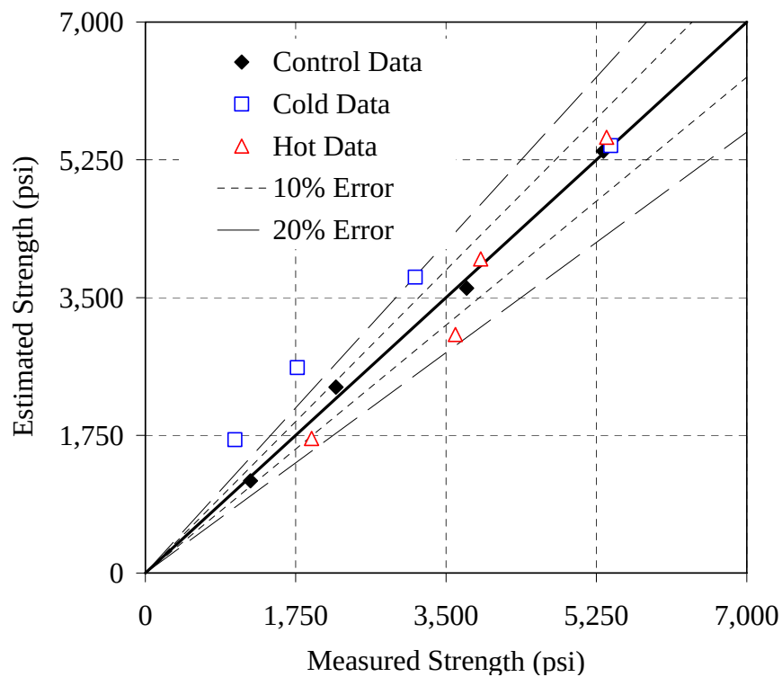
Figure I-8: Error plot for the 20% C mixture, simplified method, E = 25 kJ/mol
