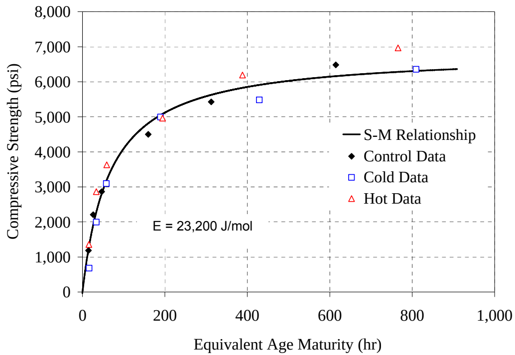
Figure C-3: Strength-maturity plot, ASTM C 1074 method for 30% F mixture
