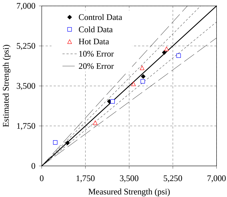
Figure 6.39: Error plot for the Type I - 0.41 mixture, simplified method, T_o = 32^\circ\text{F}
