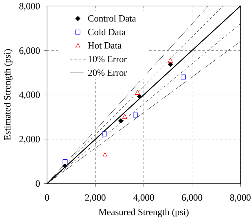
Figure G-16: Error plot for the Type III - 0.44 mixture, ASTM C 1074 method, NSM
