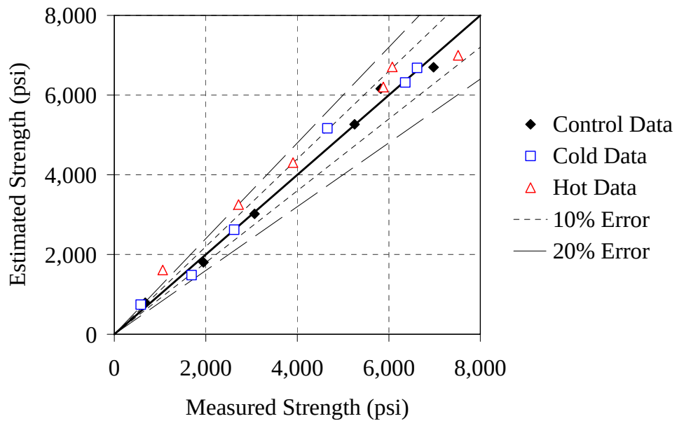
Figure D-15: Estimated strength versus actual strength for 30% C mixture
