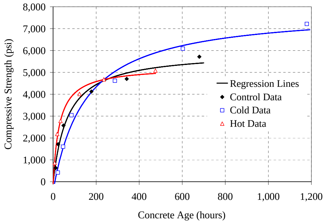
Figure 5.4: Compressive strength versus age results for Type I - 0.48 mixture
