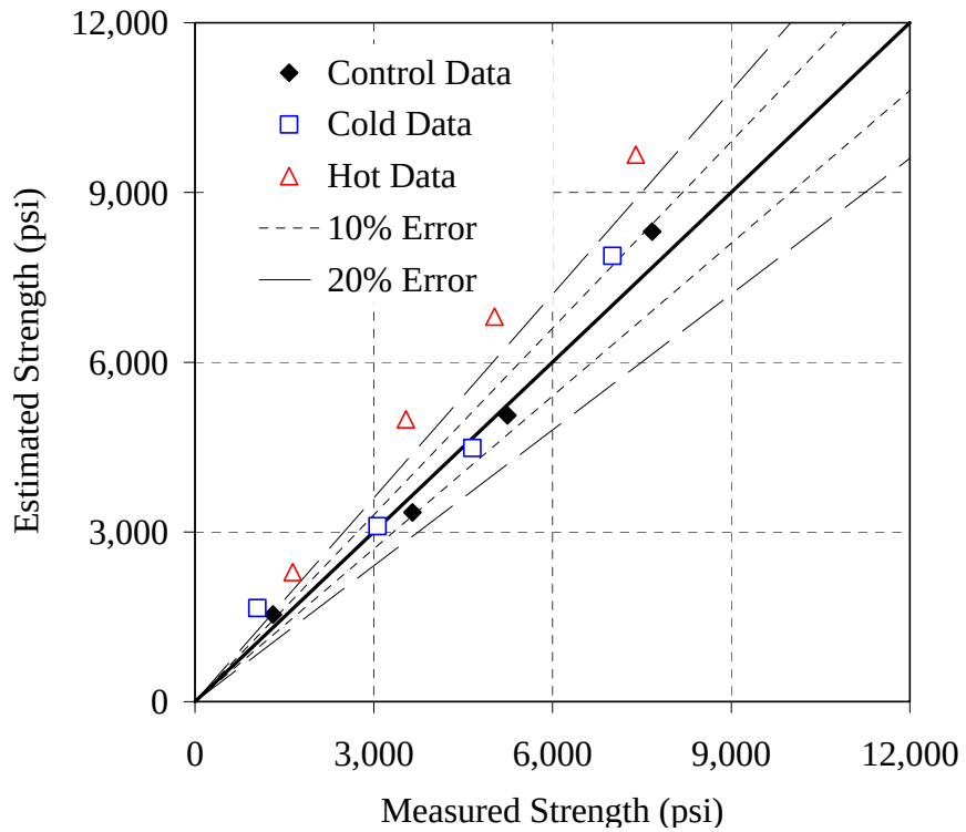
Figure G-38: Error plot for the 70/20/10 - 0.37 mixture, ASTM C 1074 method, AM
