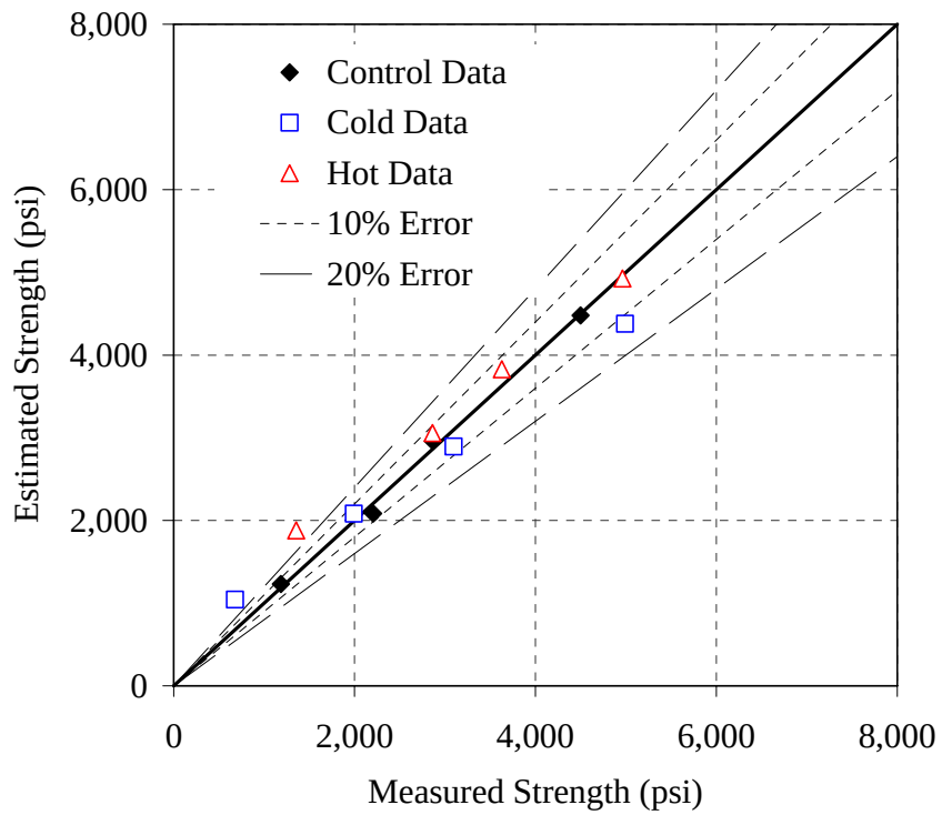
Figure G-25: Error plot for the 30% F mixture, Modified method, AM
