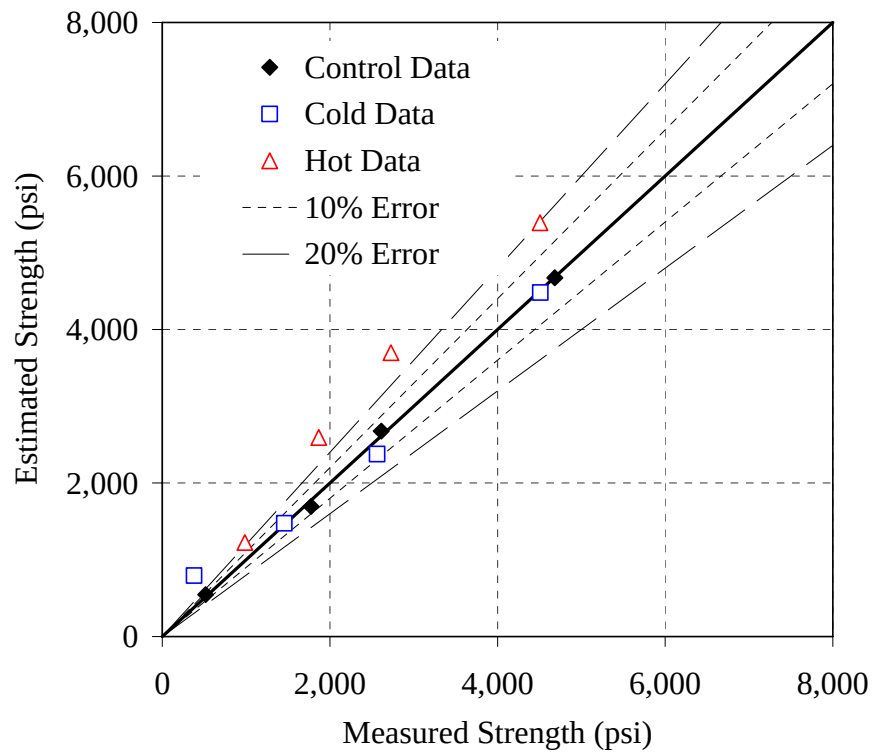
Figure I-19: Error plot for the 70/20/10 - 0.44 mixture, simplified method, E = 40 kJ/mol
