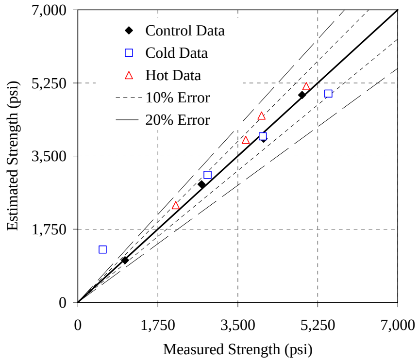
Figure 6.30: Error plot for the Type I - 0.41 mixture, Modified ASTM method, AM
