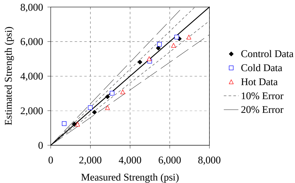
Figure D-3: Estimated strength versus actual strength for 30% F mixture
