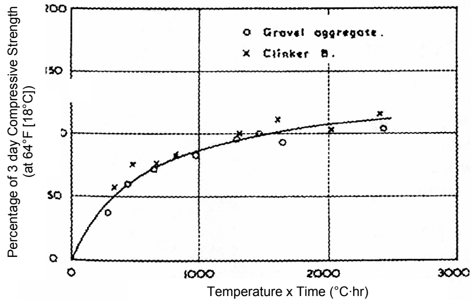
Figure 2.1: Results from experiments performed by Nurse (1949)
