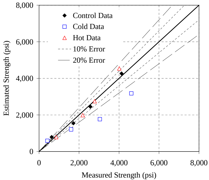
Figure G-4: Error plot for the Type I - 0.48 mixture, ASTM C 1074 method, NSM
