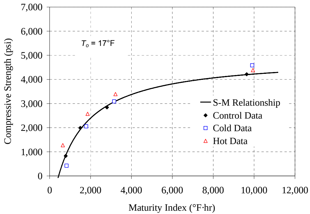
Figure E-1: Strength-maturity plot, Modified ASTM method for Type I - 0.44
