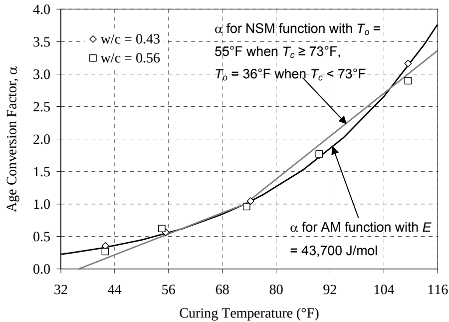
Figure 2.20: Two datum temperature scheme for Nurse-Saul maturity function (Carino 1991)
