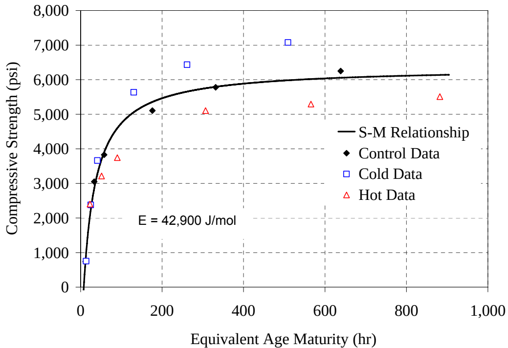
Figure C-8: Strength-maturity plot, ASTM C 1074 method for Type III - 0.44 mixture
