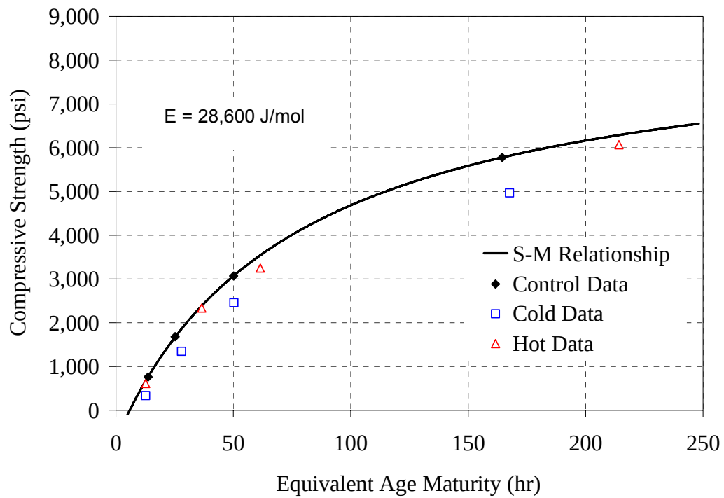
Figure F-7: Strength-maturity plot, Modified ASTM method for 50% Slag mixture
