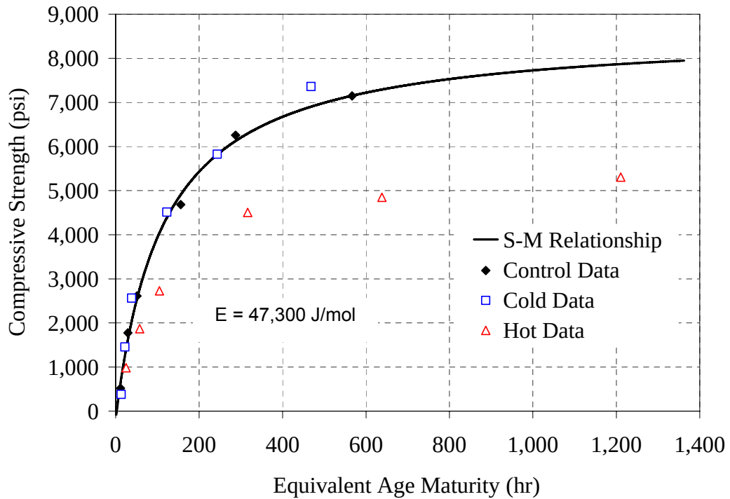
Figure C-10: Strength-maturity plot, ASTM C 1074 method for 70/20/10 - 0.44 mixture
