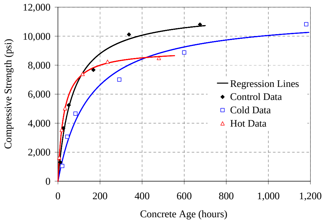
Figure 5.13: Compressive strength versus age results for 70/20/10 - 0.37 mixture
