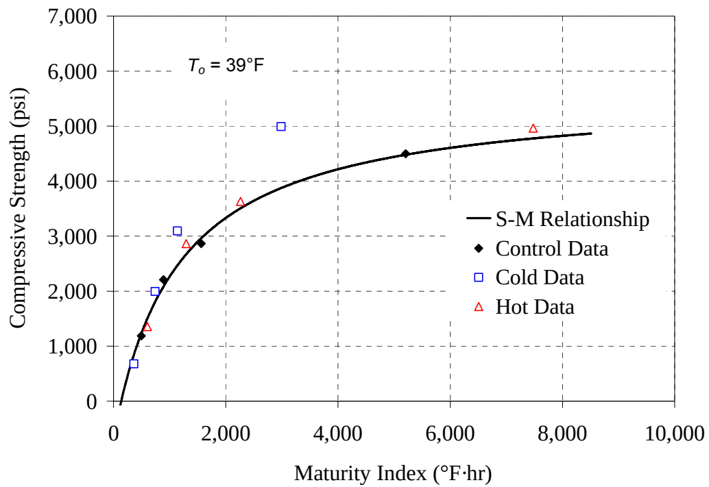
Figure E-3: Strength-maturity plot, Modified ASTM method for 30% F mixture
