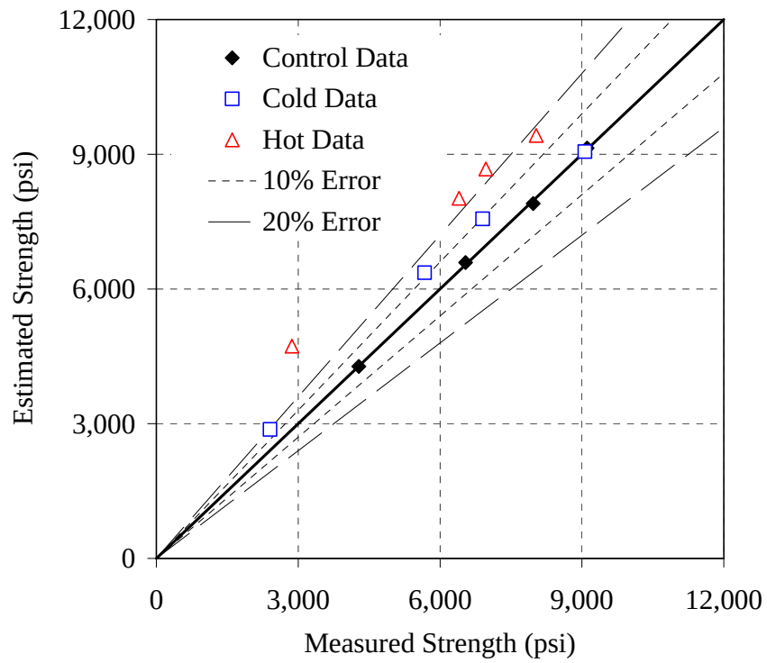
Figure 6.32: Error plot for the Type III - 0.37 mixture, Modified ASTM method, AM
