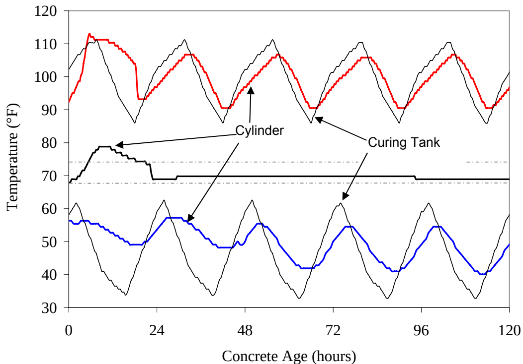
Figure 5.1: Typical temperature history of concrete cylinders
