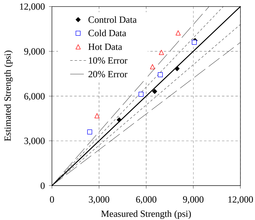
Figure 6.33: Error plot for the Type III - 0.37 mixture, ASTM C 1074 method, AM
