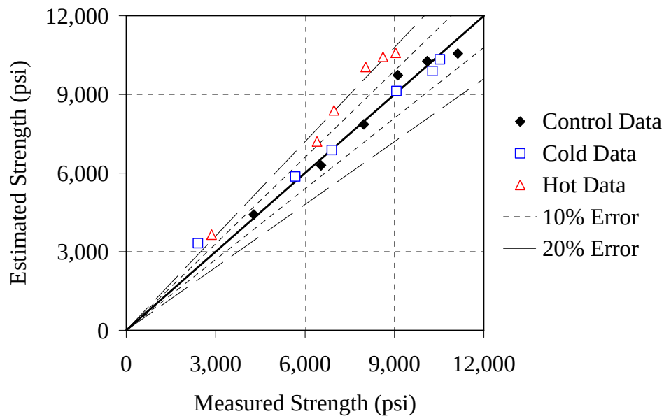
Figure 6.11: Estimated strength versus actual strength for the Type III - 0.37 mixture
