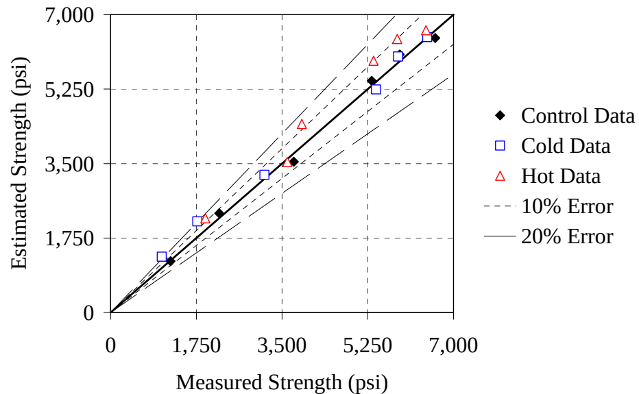
Figure D-14: Estimated strength versus actual strength for 20% C mixture
