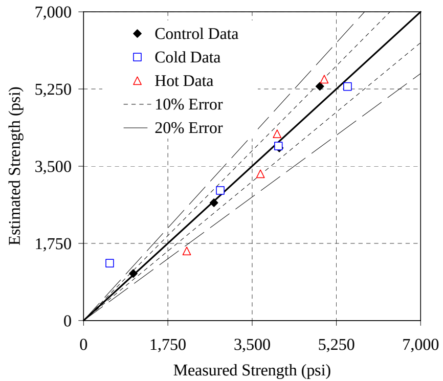
Figure 6.25: Error plot for the Type I - 0.41 mixture, ASTM C 1074 method, NSM
