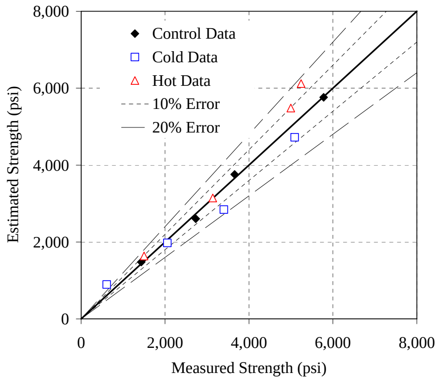
Figure G-11: Error plot for the 30% Slag mixture, Modified method, NSM
