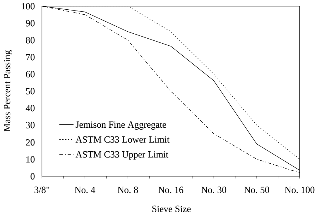
Figure 3.5: Gradation test results for Superior Products fine aggregate
