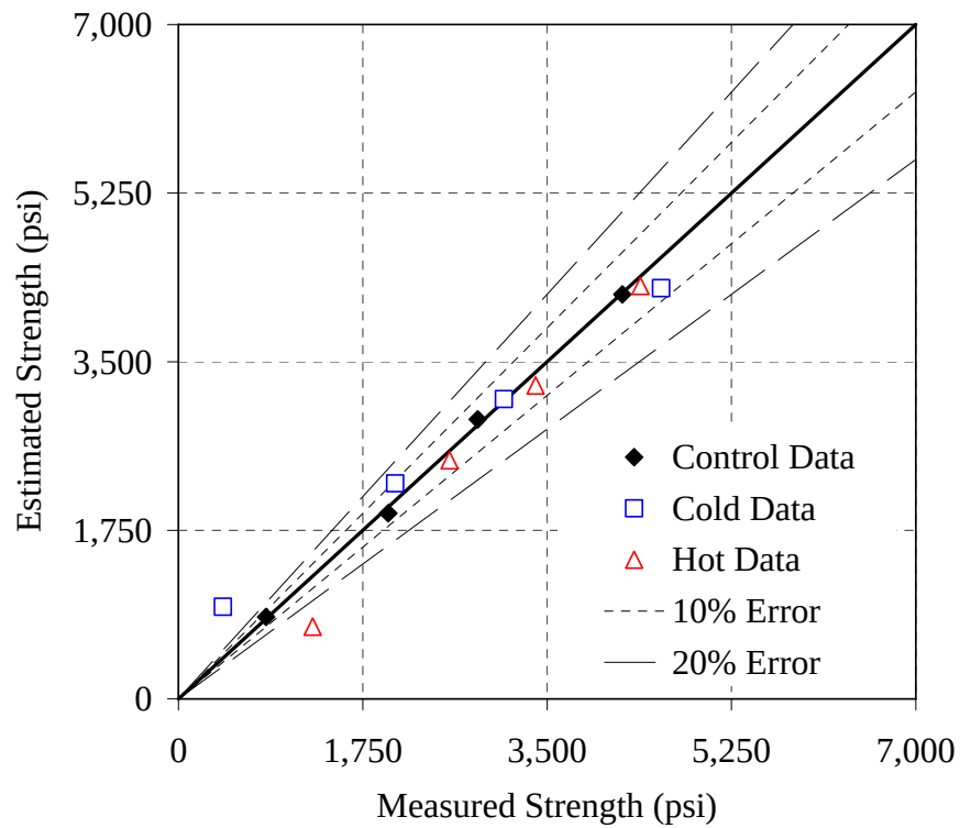
Figure I-2: Error plot for the Type I - 0.44 mixture, simplified method, E = 25 kJ/mol
