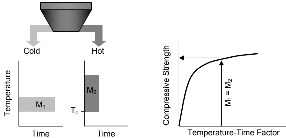
Figure 2.3: Diagram of Saul's maturity rule
