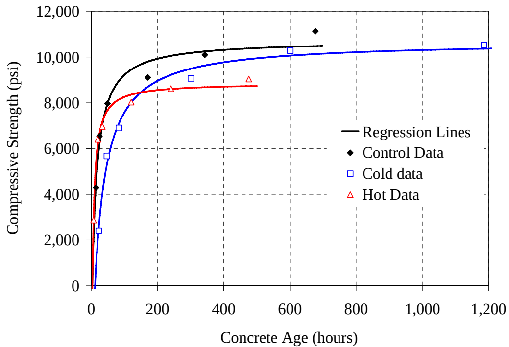
Figure 5.11: Compressive strength versus age results for Type III - 0.37 mixture
