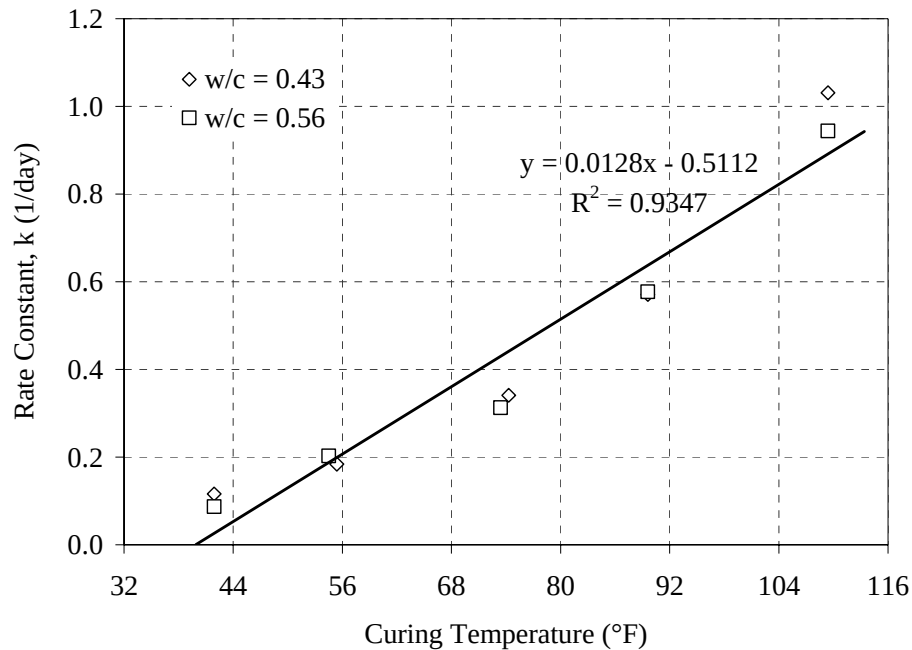
Figure 2.17: Rate constants used to find best-fit datum temperature (Carino 1991)
