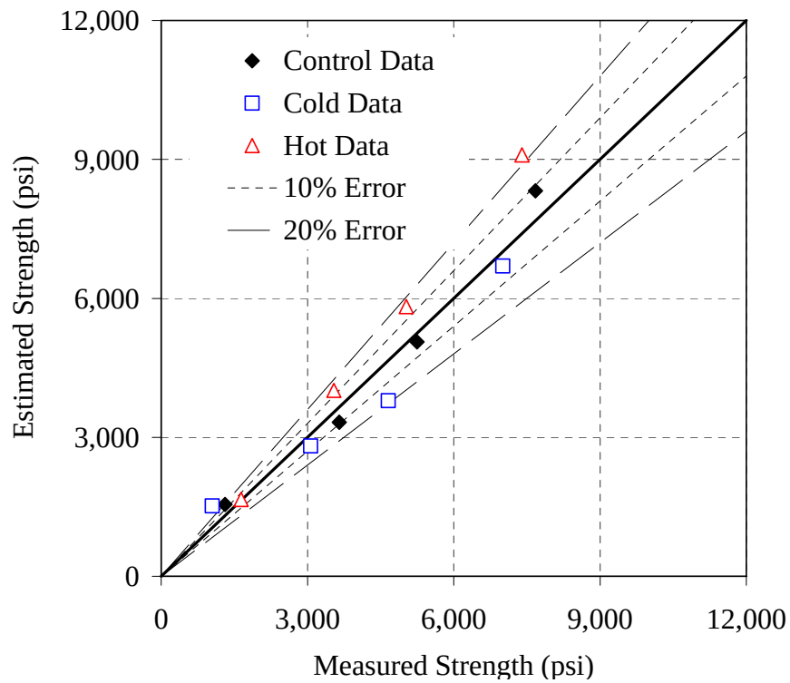
Figure G-18: Error plot for the 70/20/10 - 0.37 mixture, ASTM C 1074 method, NSM
