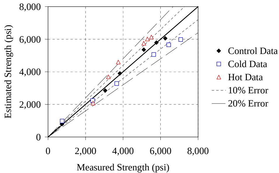
Figure D-18: Estimated strength versus actual strength for Type III - 0.44 mixture
