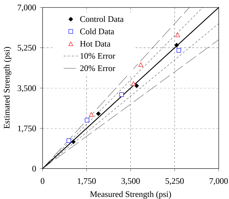
Figure I-7: Error plot for the 20% C mixture, simplified method, E = 40 kJ/mol
