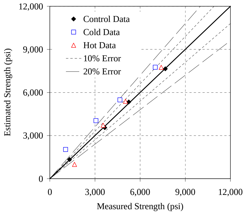
Figure H-17: Error plot for the 70/20/10 - 0.37 mixture, simplified method, T_o = 14^\circ\text{F}
