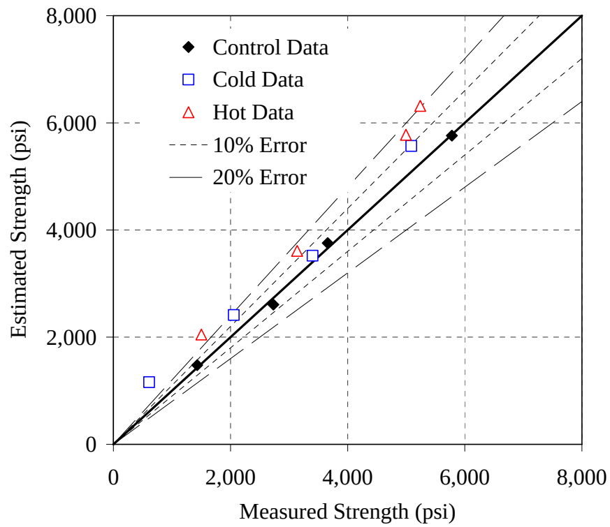
Figure I-11: Error plot for the 30% Slag mixture, simplified method, E = 40 kJ/mol
