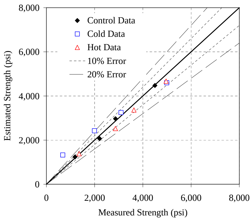
Figure I-6: Error plot for the 30% F mixture, simplified method, E = 25 kJ/mol
