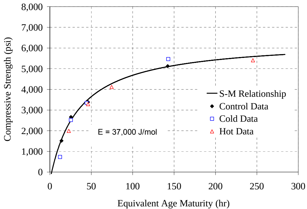
Figure 6.19: Strength-maturity plot, Modified ASTM method for 20% F mixture
