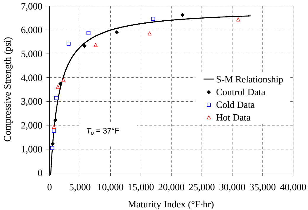
Figure B-4: 20% C mixture, (a) compressive strength vs. age, (b) strength-maturity plot, ASTM C 1074 method
