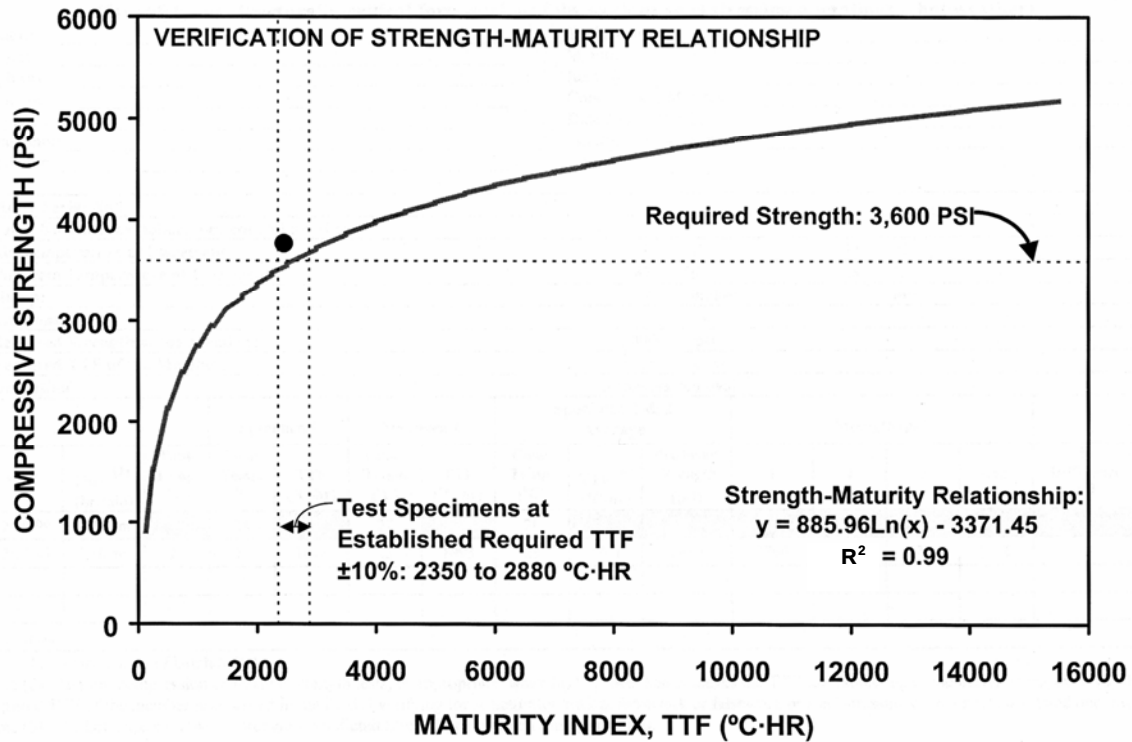
Figure 2.7: Example of verification of design strength (TxDOT 1999)
