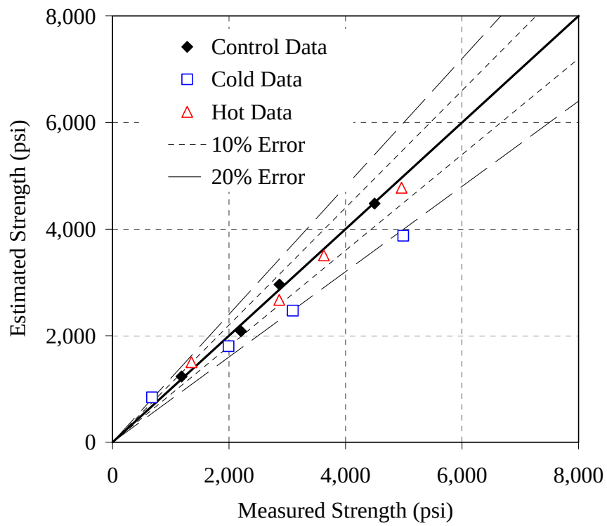
Figure G-5: Error plot for the 30% F mixture, Modified method, NSM
