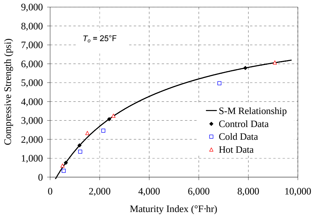
Figure E-7: Strength-maturity plot, Modified ASTM method for 50% Slag mixture
