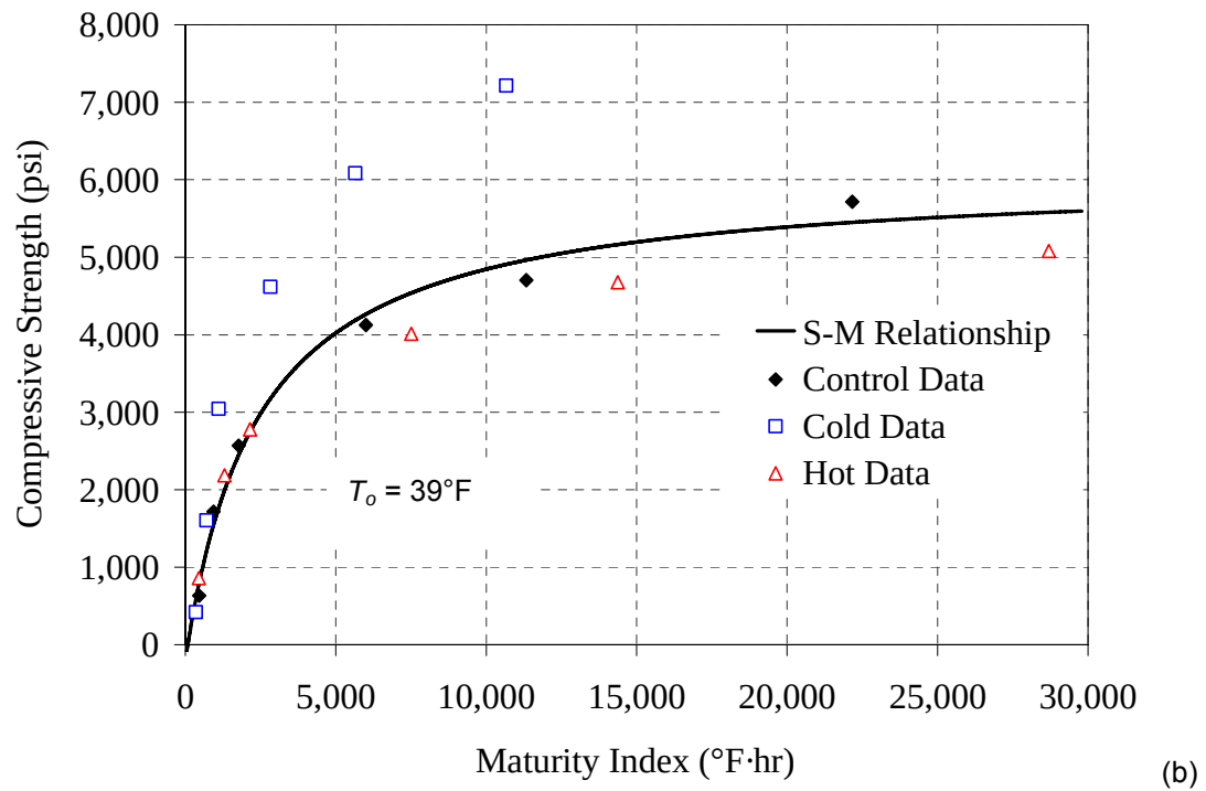
Figure B-2: Type I - 0.48 mixture, (a) compressive strength vs. age, (b) strength-maturity plot, ASTM C 1074 method
