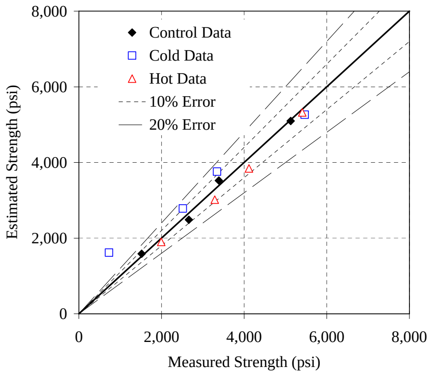
Figure 6.43: Error plot for the 20% F mixture, simplified method, E = 25 kJ/mol
