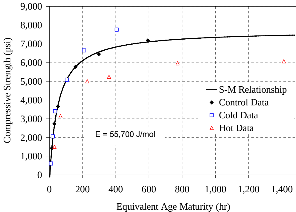
Figure C-6: Strength-maturity plot, ASTM C 1074 method for 30% Slag mixture
