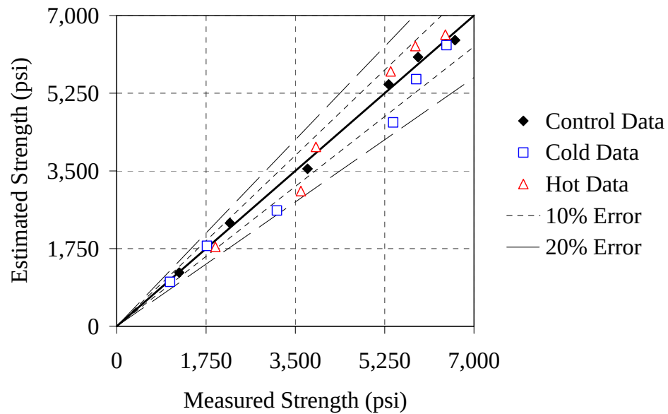
Figure D-4: Estimated strength versus actual strength for 20% C mixture
