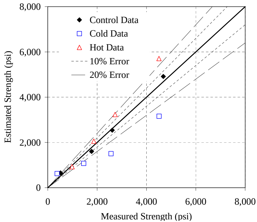
Figure G-20: Error plot for the 70/20/10 - 0.44 mixture, ASTM C 1074 method, NSM
