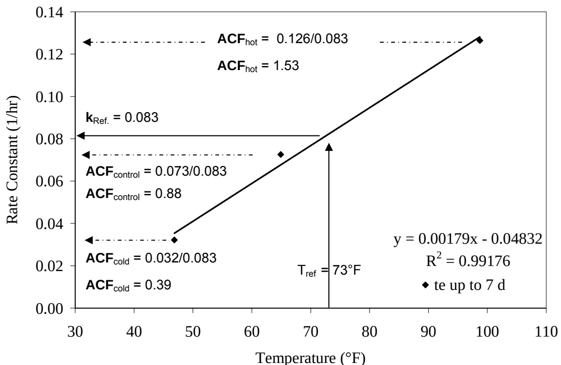
Figure 6.34: Obtaining age conversion factors for Type I - 0.41 mixture
