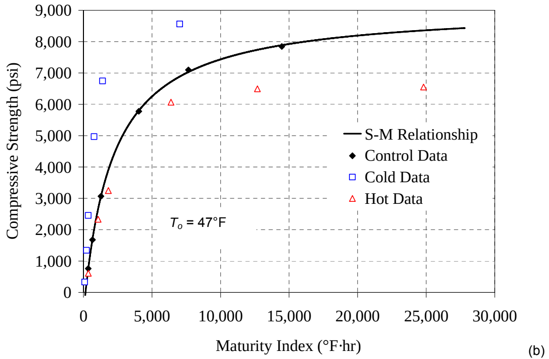
Figure B-7: 50% Slag mixture, (a) compressive strength vs. age, (b) strength-maturity plot, ASTM C 1074 method
