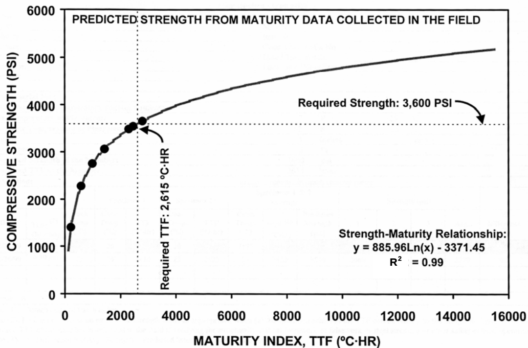
Figure 2.6: Example of estimating strength from strength-maturity relationship (TxDOT 1999)
