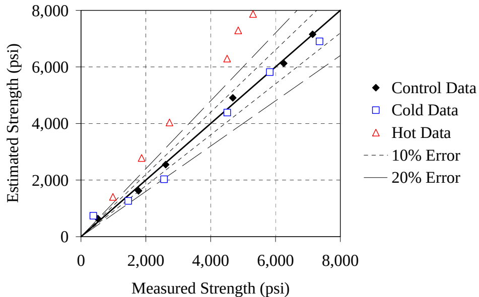
Figure D-20: Estimated strength versus actual strength for 70/20/10 - 0.44 mixture
