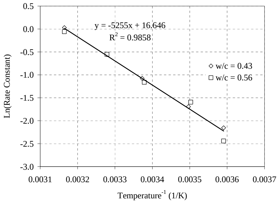
Figure 2.18: Rate constants used to find best-fit activation energy (Carino 1991)
