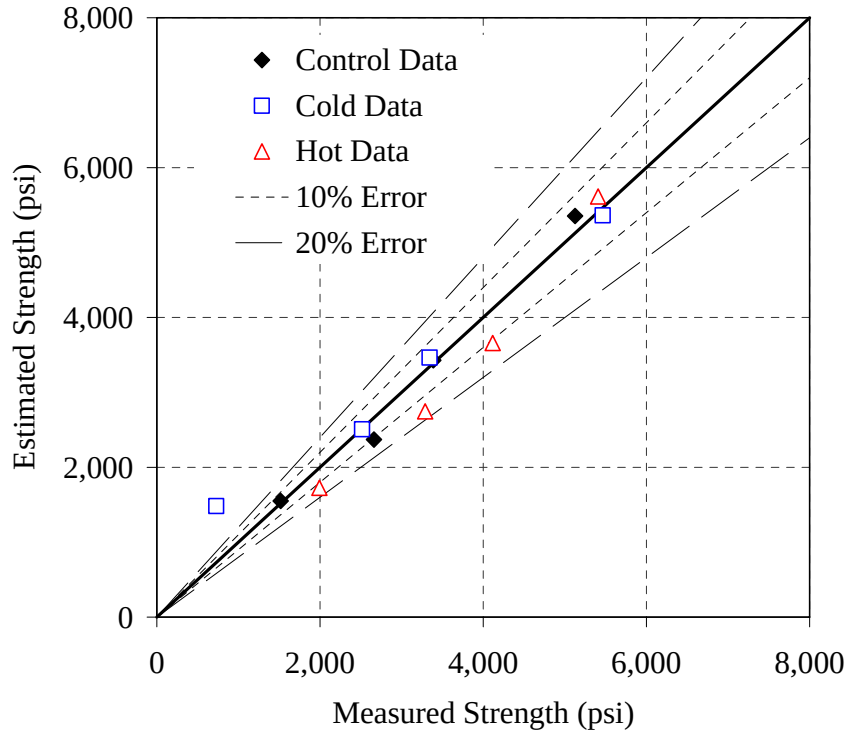
Figure 6.23: Error plot for the 20% F mixture, ASTM C 1074 method, NSM
