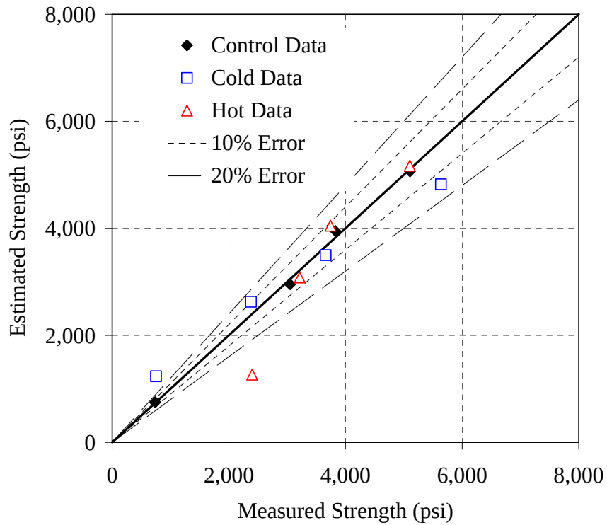
Figure H-16: Error plot for the Type III - 0.44 mixture, simplified method, T_o = 32^\circ\text{F}
