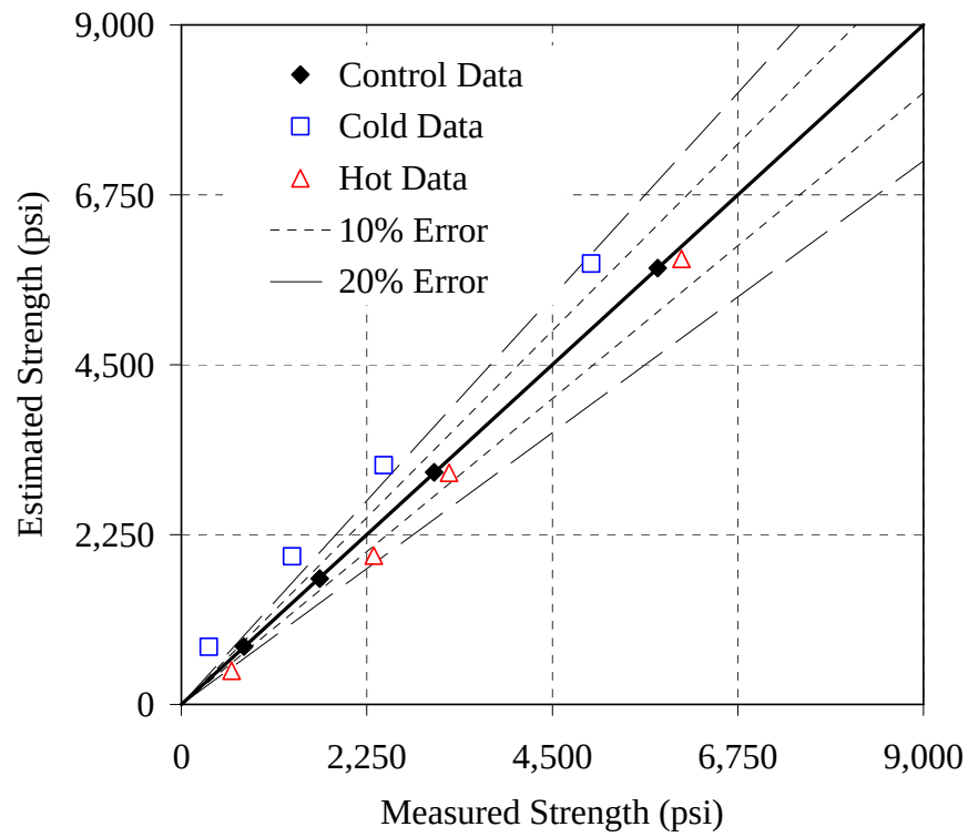
Figure H-13: Error plot for the 50% Slag mixture, simplified method, T_o = 14^\circ\text{F}
