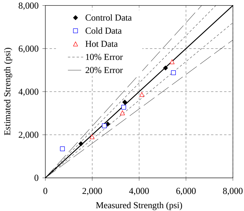
Figure 6.37: Error plot for the 20% F mixture, simplified method, T_o = 32^\circ\text{F}
