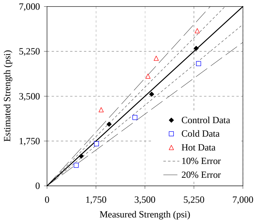
Figure G-27: Error plot for the 20% C mixture, Modified method, AM
