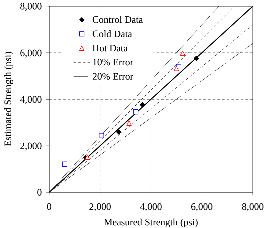
Figure H-12: Error plot for the 30% Slag mixture, simplified method, T_o = 32^\circ\text{F}
