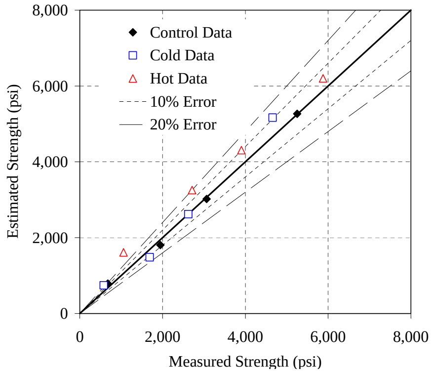
Figure G-30: Error plot for the 30% C mixture, ASTM C 1074 method, AM
