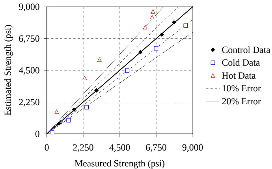
Figure D-17: Estimated strength versus actual strength for 50% Slag mixture
