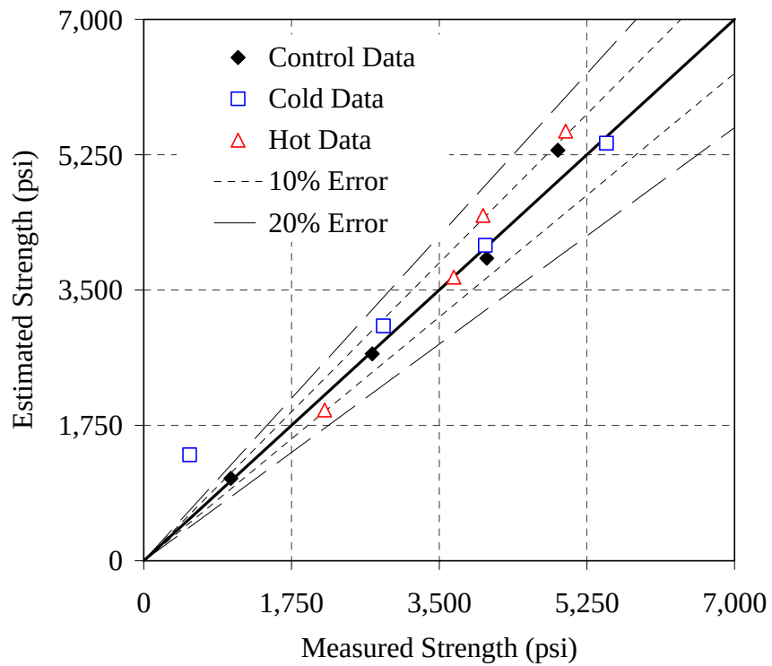
Figure 6.31: Error plot for the Type I - 0.41 mixture, ASTM C 1074 method, AM
