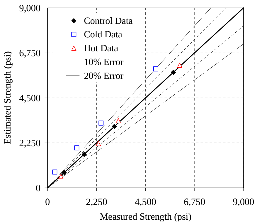
Figure I-14: Error plot for the 50% Slag mixture, simplified method, E = 25 kJ/mol
