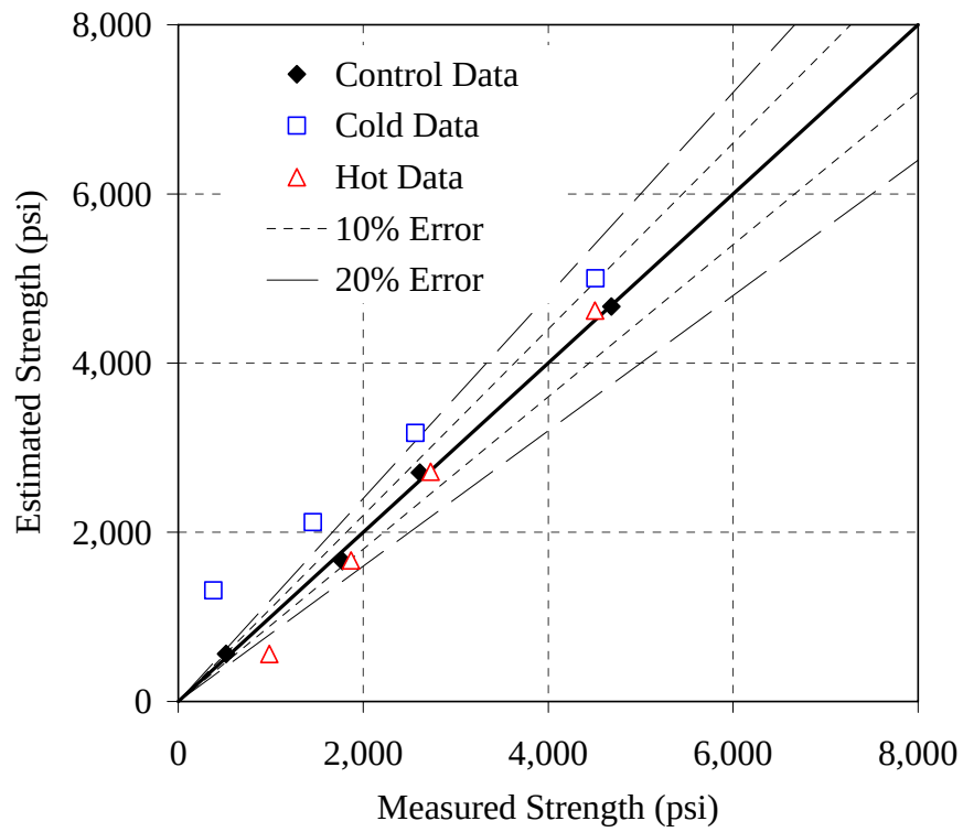
Figure G-39: Error plot for the 70/20/10 - 0.44 mixture, Modified method, AM
