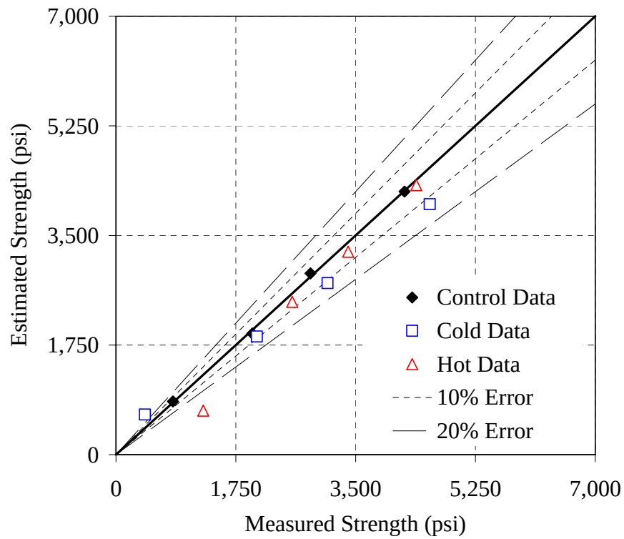
Figure H-2: Error plot for the Type I - 0.44 mixture, simplified method, T_o = 32^\circ\text{F}
