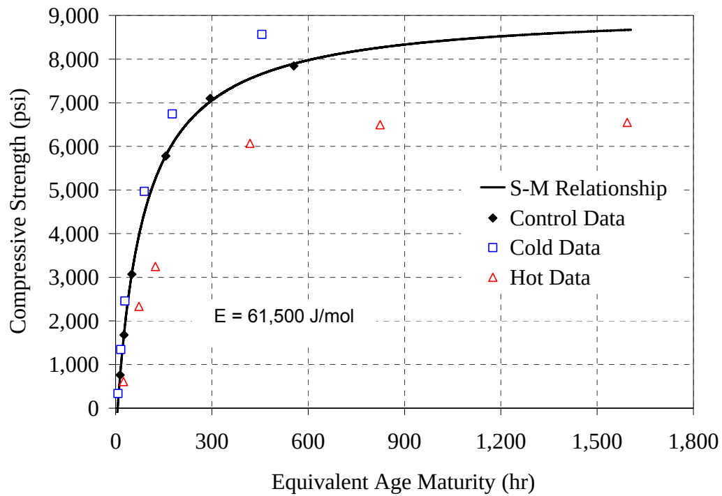
Figure C-7: Strength-maturity plot, ASTM C 1074 method for 50% Slag mixture
