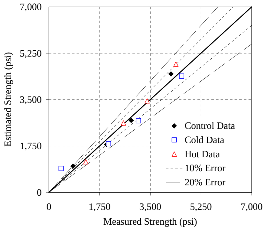
Figure G-22: Error plot for the Type I - 0.44 mixture, ASTM C 1074 method, AM
