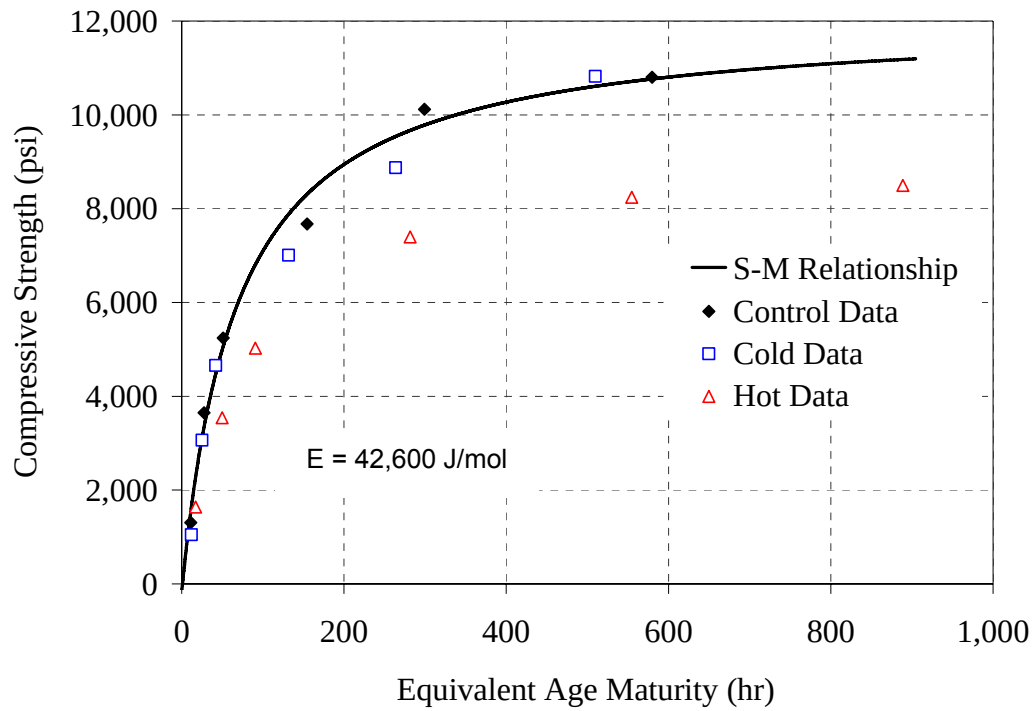
Figure C-9: Strength-maturity plot, ASTM C 1074 method for 70/20/10 - 0.37 mixture
