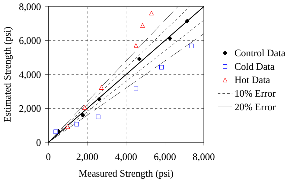
Figure D-10: Estimated strength versus actual strength for 70/20/10 - 0.44 mixture
