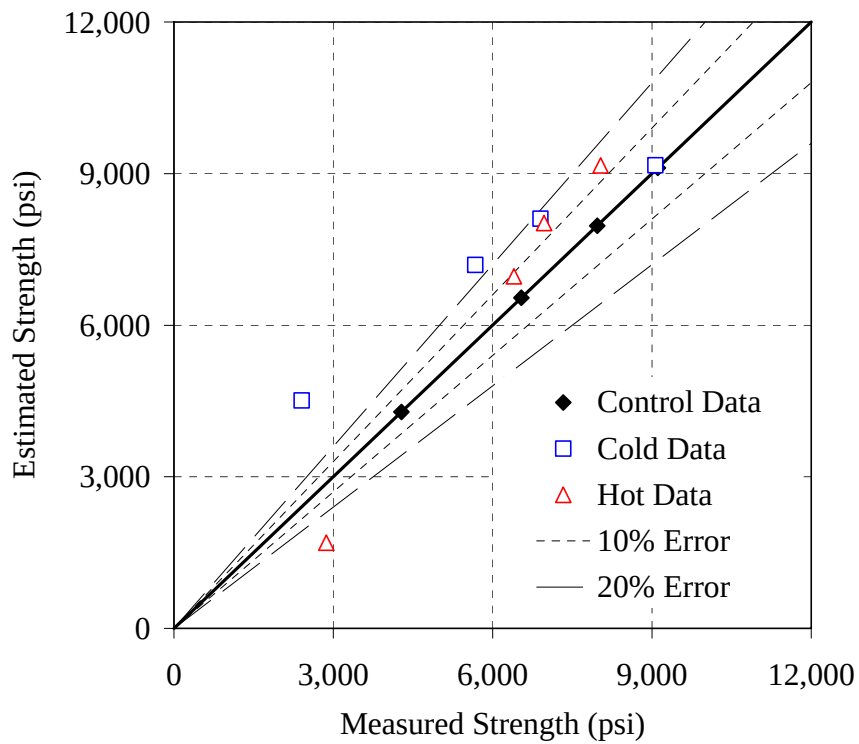
Figure 6.40: Error plot for the Type III - 0.37 mixture, simplified method, T_o = 14^\circ\text{F}
