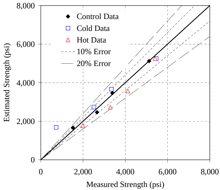
Figure 6.36: Error plot for the 20% F mixture, simplified method, T_o = 14^\circ\text{F}
