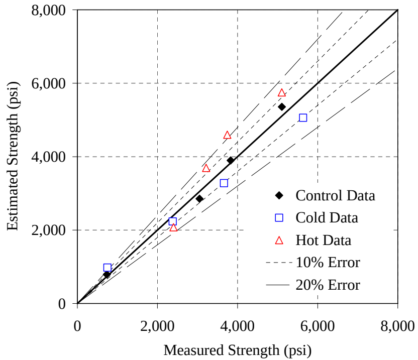
Figure G-36: Error plot for the Type III - 0.44 mixture, ASTM C 1074 method, AM
