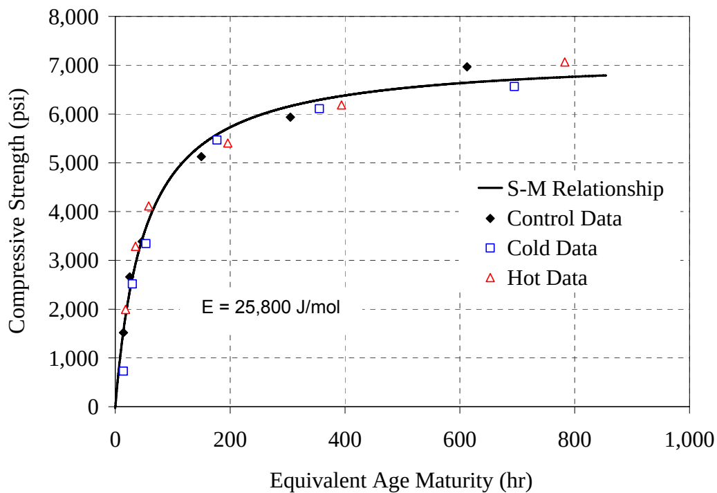
Figure 6.6: Strength-maturity plot, ASTM C 1074 method for 20% F mixture
