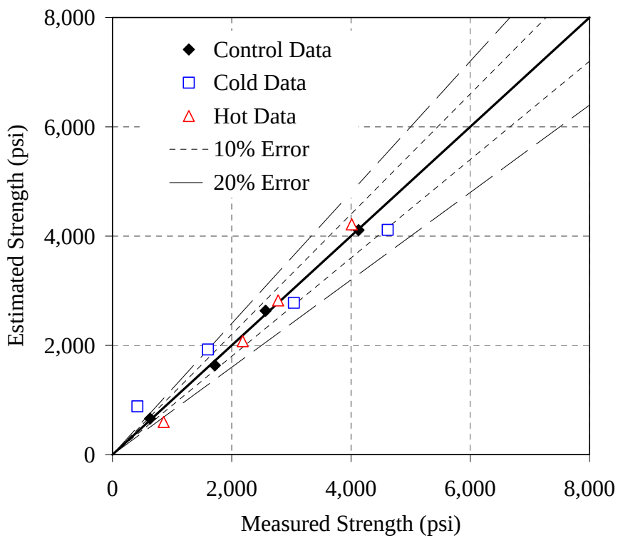
Figure I-4: Error plot for the Type I - 0.48 mixture, simplified method, E = 25 kJ/mol
