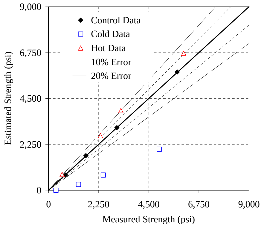
Figure G-14: Error plot for the 50% Slag mixture, ASTM C 1074 method, NSM
