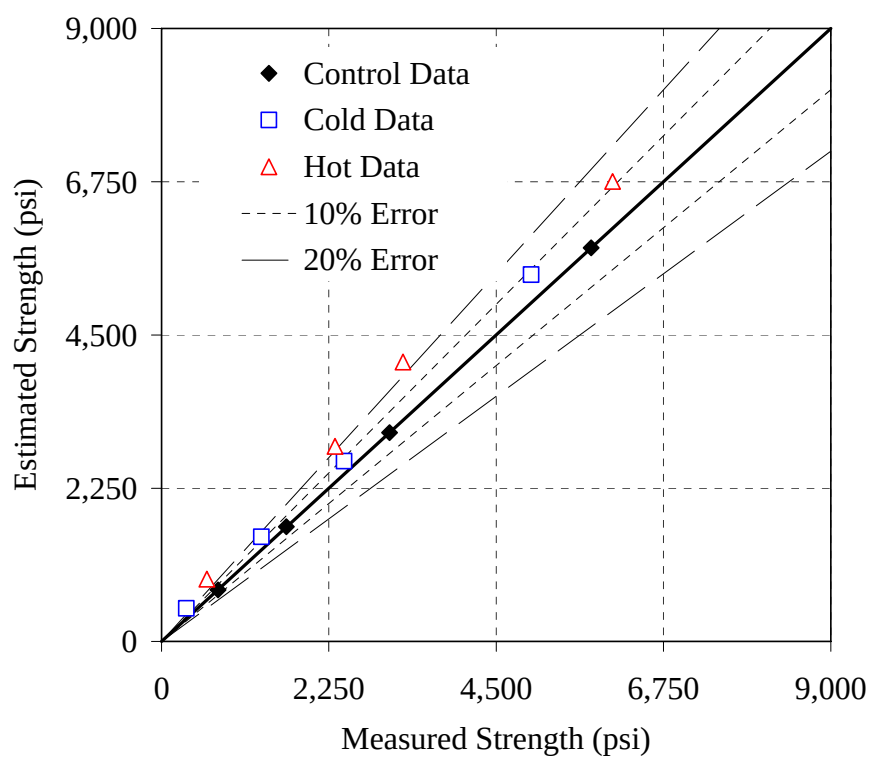
Figure I-13: Error plot for the 50% Slag mixture, simplified method, E = 40 kJ/mol
