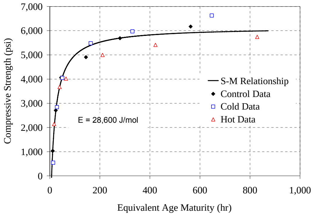
Figure 6.7: Strength-maturity plot, ASTM C 1074 method for Type I - 0.41 mixture
