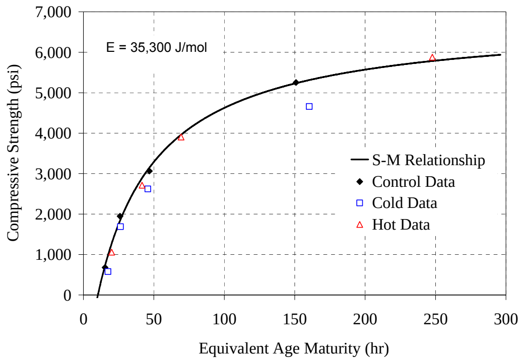
Figure F-5: Strength-maturity plot, Modified ASTM method for 30% C mixture
