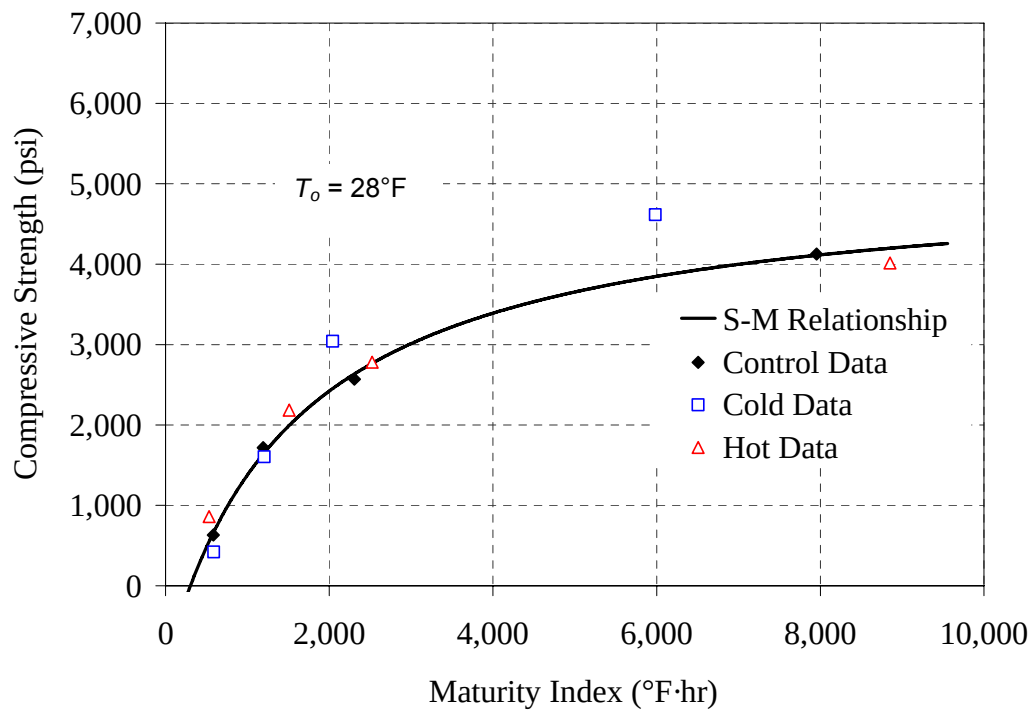
Figure E-2: Strength-maturity plot, Modified ASTM method for Type I - 0.48 mixture
