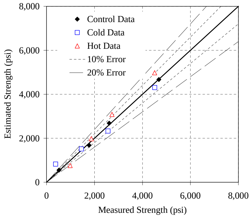
Figure H-20: Error plot for the 70/20/10 - 0.44 mixture, simplified method, T_o = 32^\circ\text{F}
