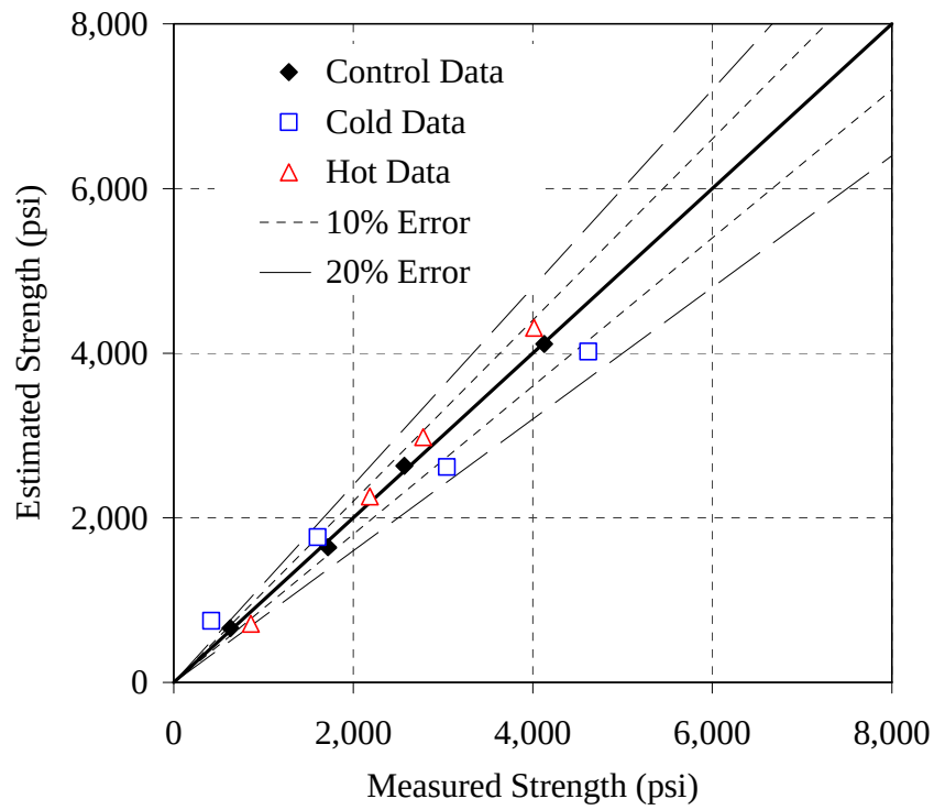
Figure G-23: Error plot for the Type I - 0.48 mixture, Modified method, AM
