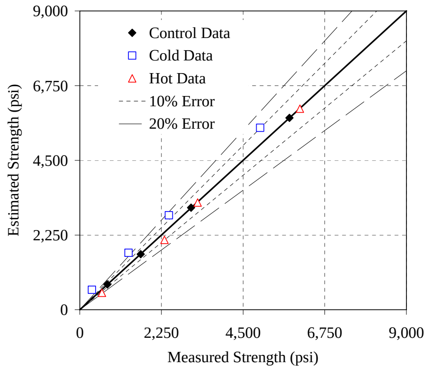
Figure G-13: Error plot for the 50% Slag mixture, Modified method, NSM
