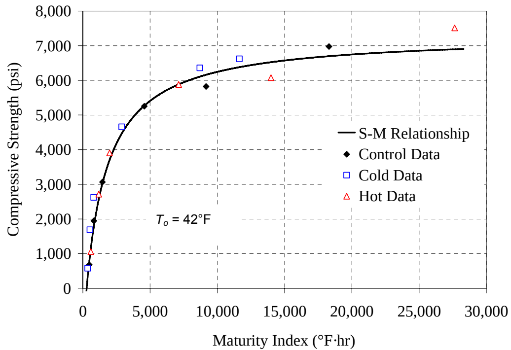
Figure B-5: 30% C mixture, (a) compressive strength vs. age, (b) strength-maturity plot, ASTM C 1074 method
