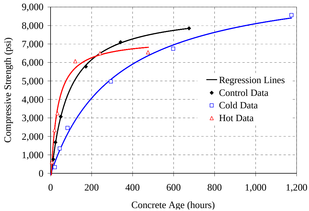
Figure 5.10: Compressive strength versus age results for 50% Slag mixture
