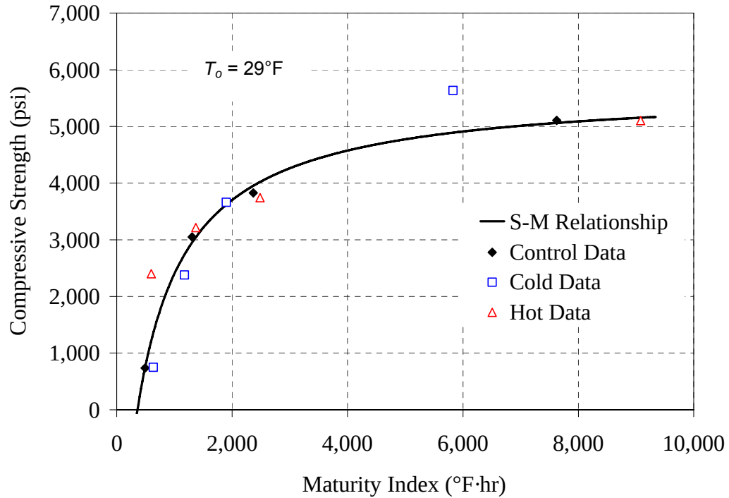
Figure E-8: Strength-maturity plot, Modified ASTM method for Type III - 0.44 mixture
