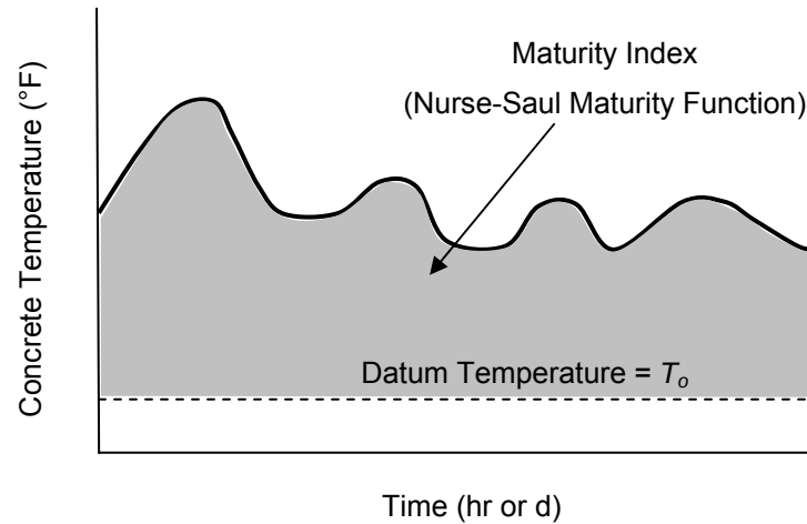
Figure 2.2: Diagram of concrete maturity using Nurse-Saul maturity function
