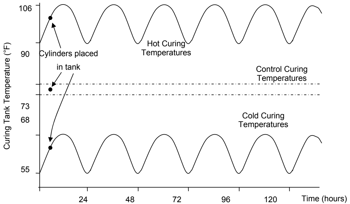
Figure 3.3: Curing tank cycles
