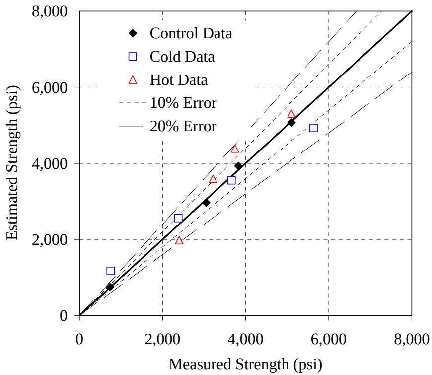
Figure G-35: Error plot for the Type III - 0.44 mixture, Modified method, AM
