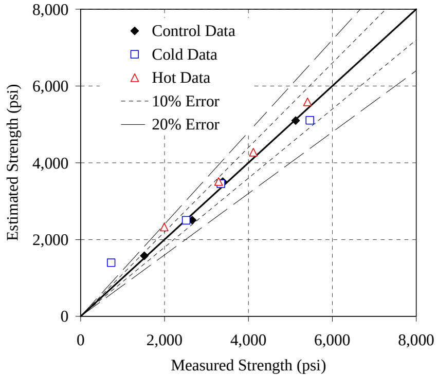
Figure 6.28: Error plot for the 20% F mixture, Modified ASTM method, AM
