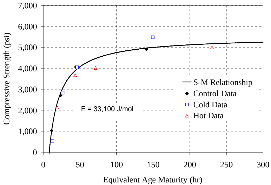
Figure 6.20: Strength-maturity plot, Modified ASTM method for Type I - 0.41 mixture
