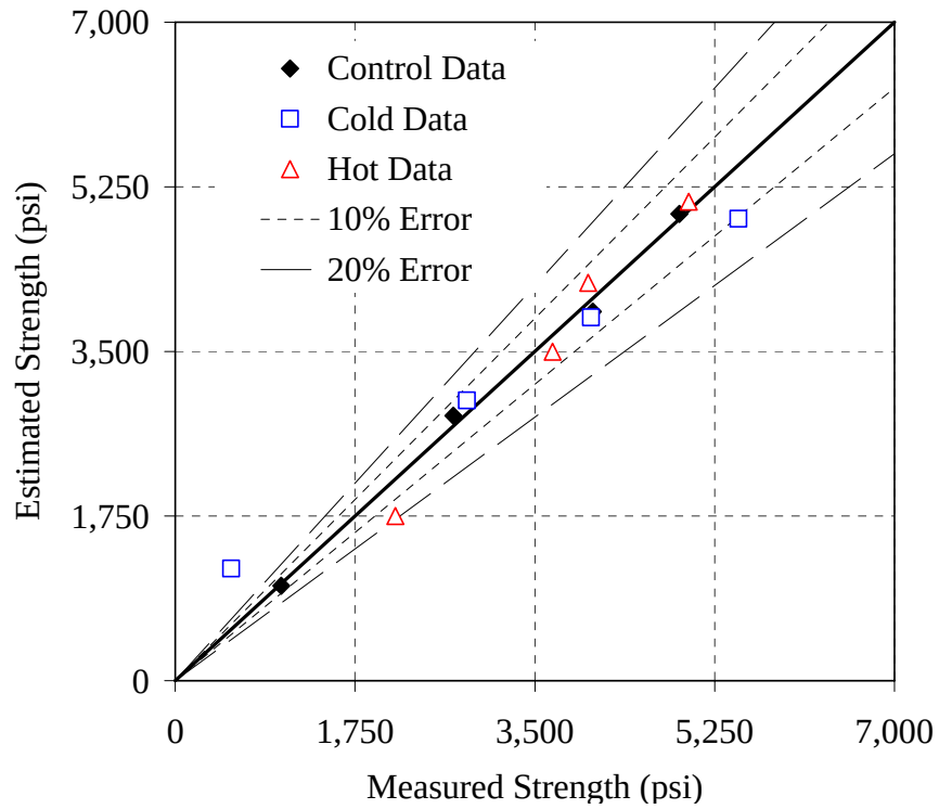
Figure 6.24: Error plot for the Type I - 0.41 mixture, Modified ASTM method, NSM
