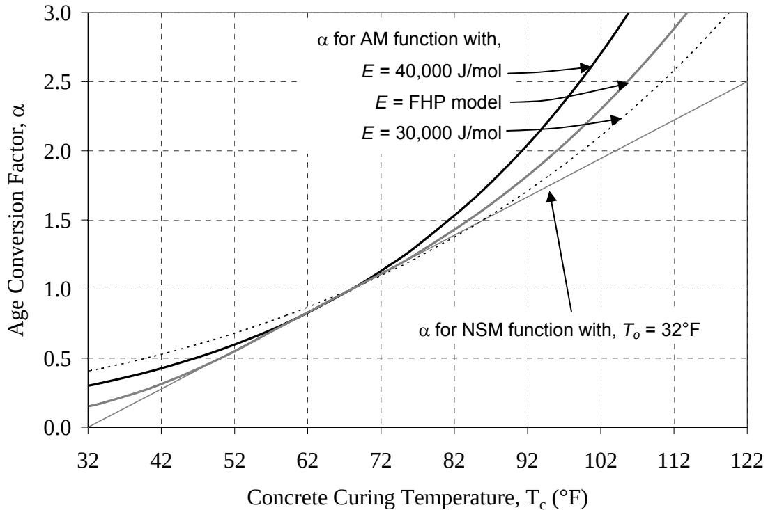
Figure 2.21: Comparing age conversion factors using FHP model to other functions
