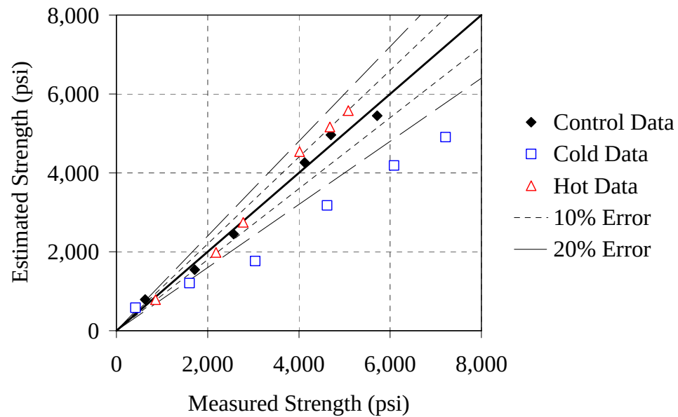
Figure D-2: Estimated strength versus actual strength for Type I - 0.48 mixture
