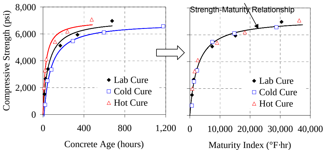
Figure 2.4: Converting strength-age data to strength-maturity data
