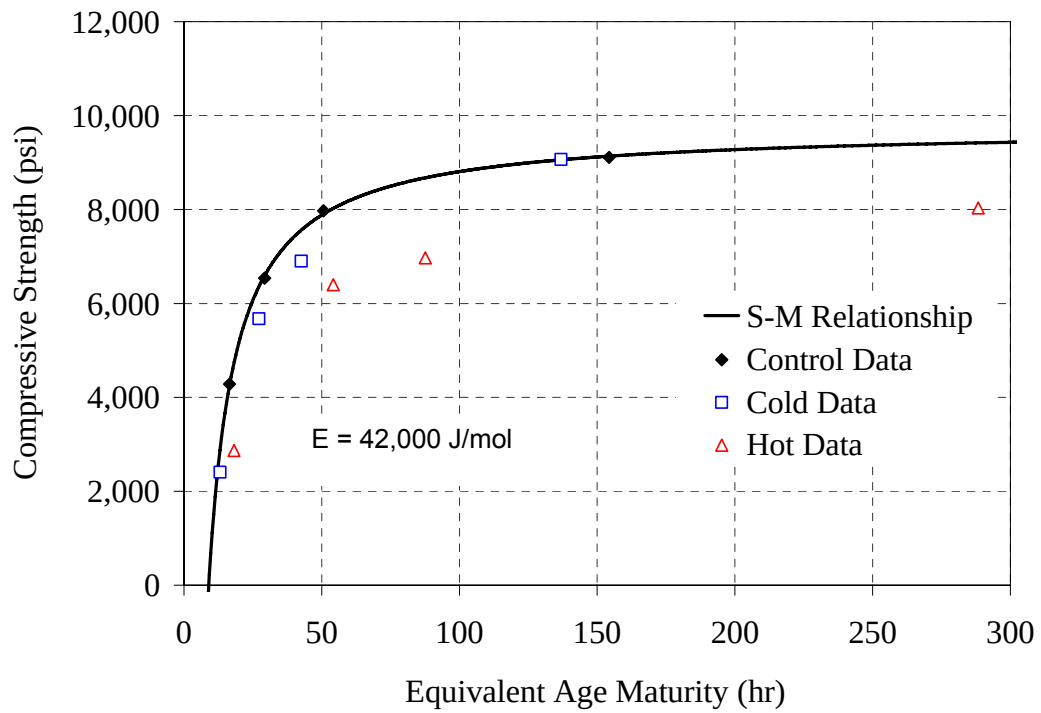
Figure 6.21: Strength-maturity plot, Modified ASTM method for Type III - 0.37 mixture
