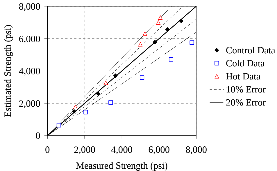
Figure D-6: Estimated strength versus actual strength for 30% Slag mixture
