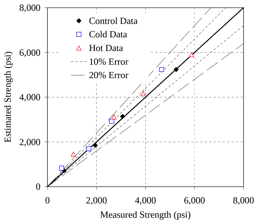
Figure I-9: Error plot for the 30% C mixture, simplified method, E = 40 kJ/mol
