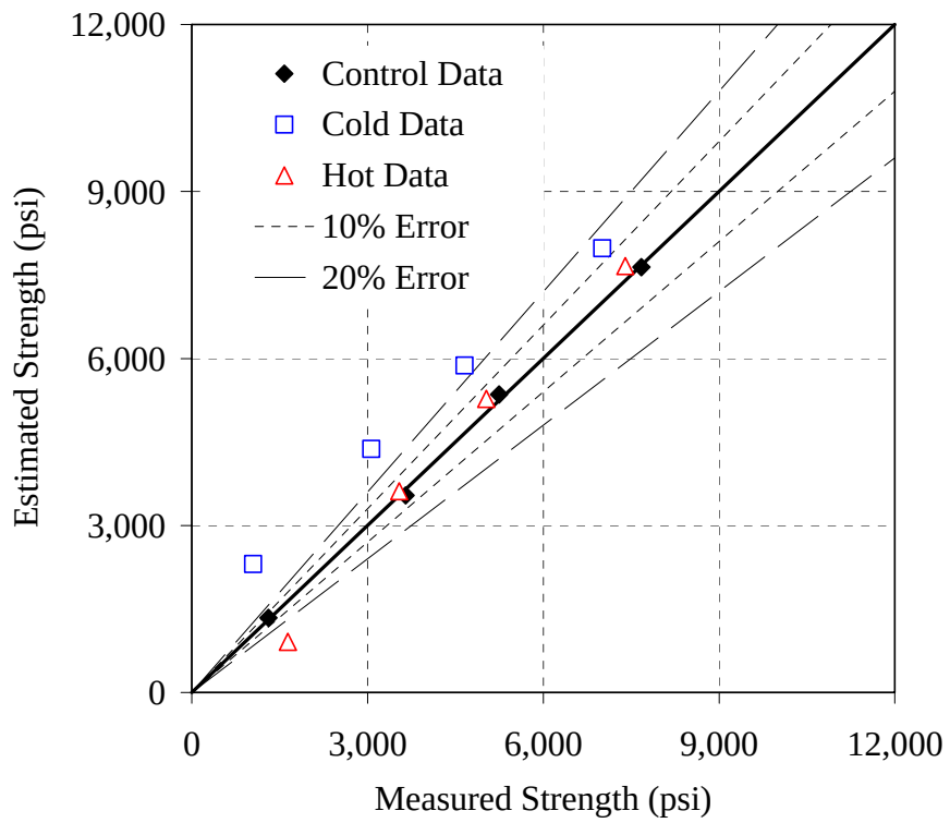
Figure G-37: Error plot for the 70/20/10 - 0.37 mixture, Modified method, AM
