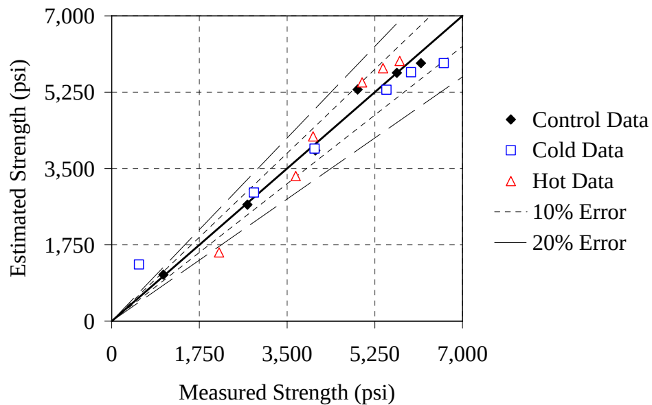
Figure 6.10: Estimated strength versus actual strength for the Type I - 0.41 mixture
