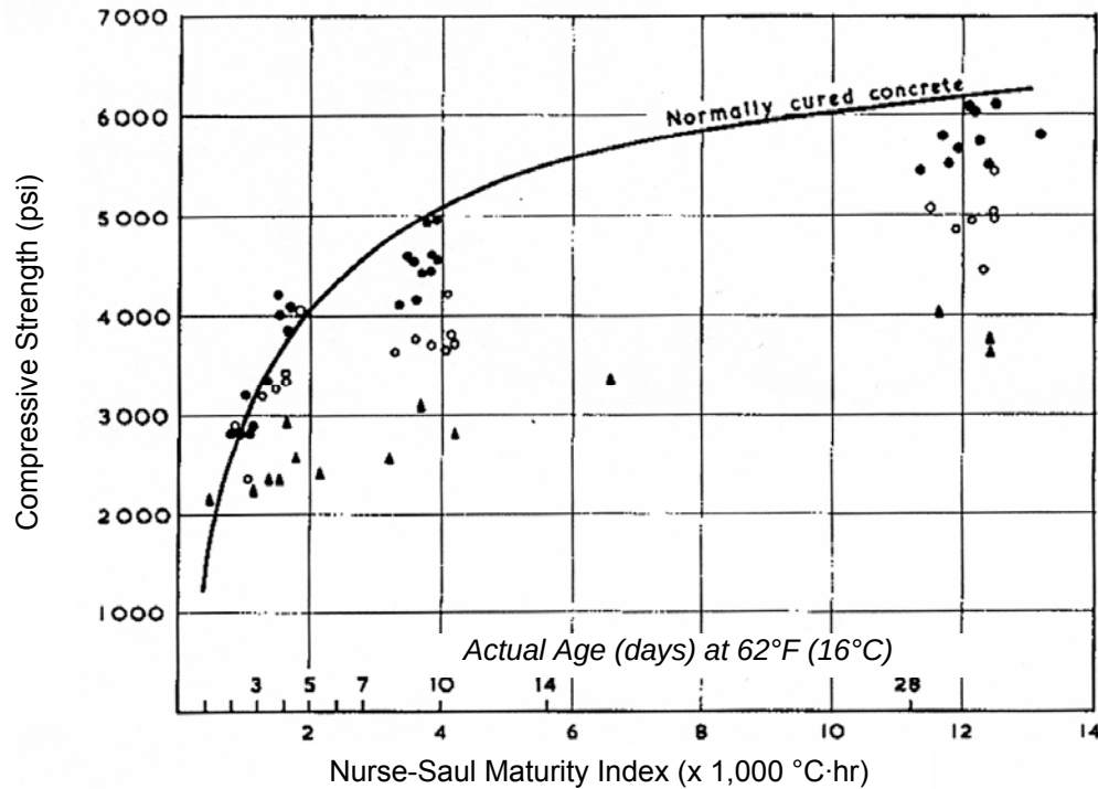
Figure 2.12: Temperature effects on estimating strength using strength-maturity relationship (Saul 1951)
