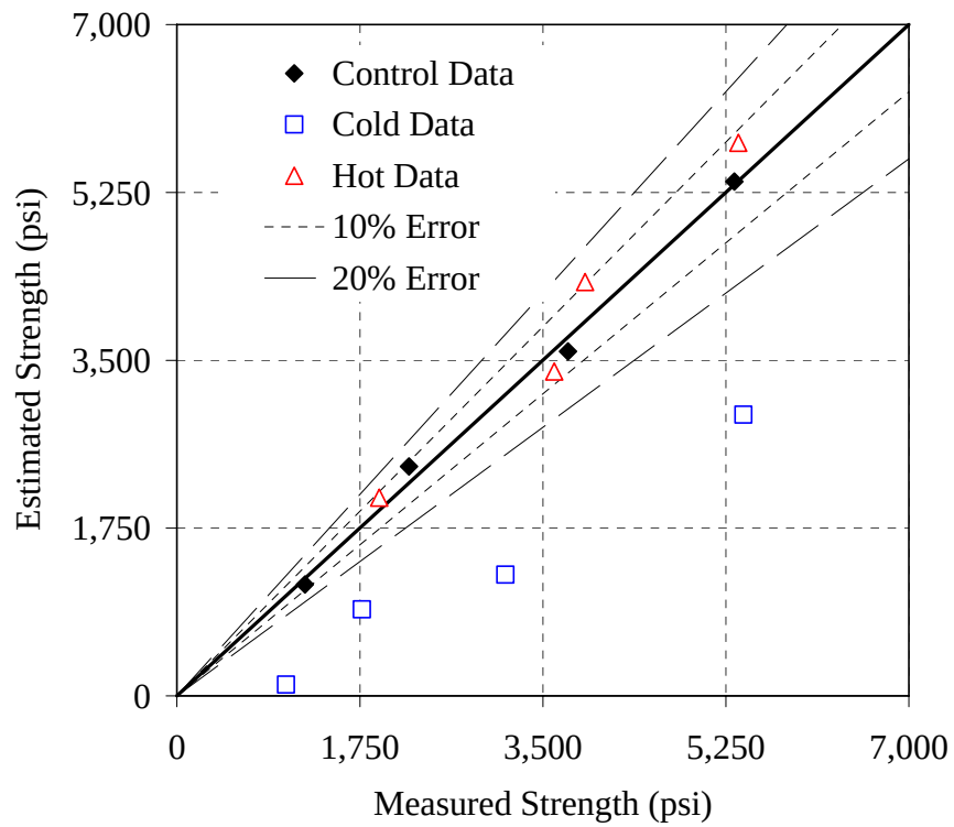
Figure G-7: Error plot for the 20% C mixture, Modified method, NSM
