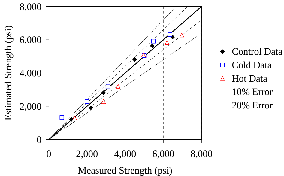
Figure D-13: Estimated strength versus actual strength for 30% F mixture
