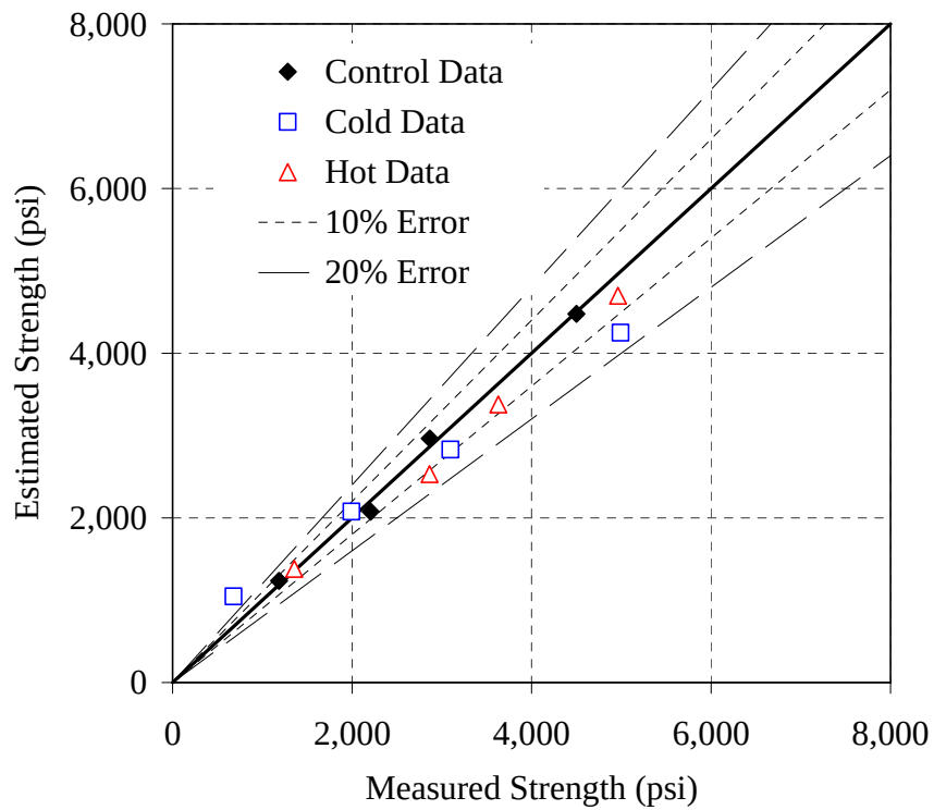
Figure H-6: Error plot for the 30% F mixture, simplified method, T_o = 32^\circ\text{F}
