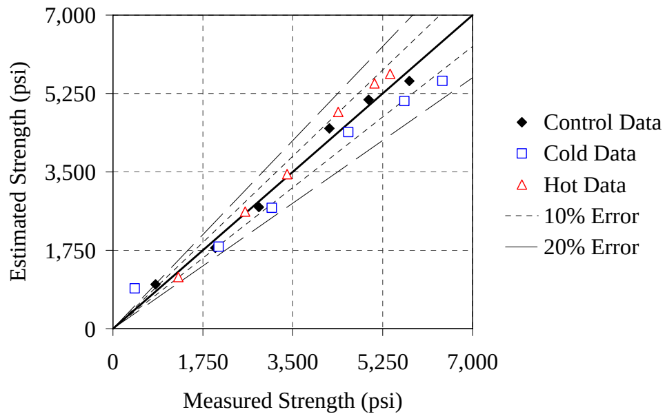
Figure D-11: Estimated strength versus actual strength for Type I - 0.44 mixture
