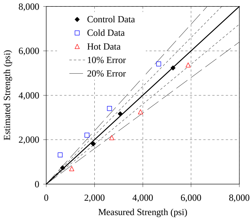
Figure H-9: Error plot for the 30% C mixture, simplified method, T_o = 14^\circ\text{F}
