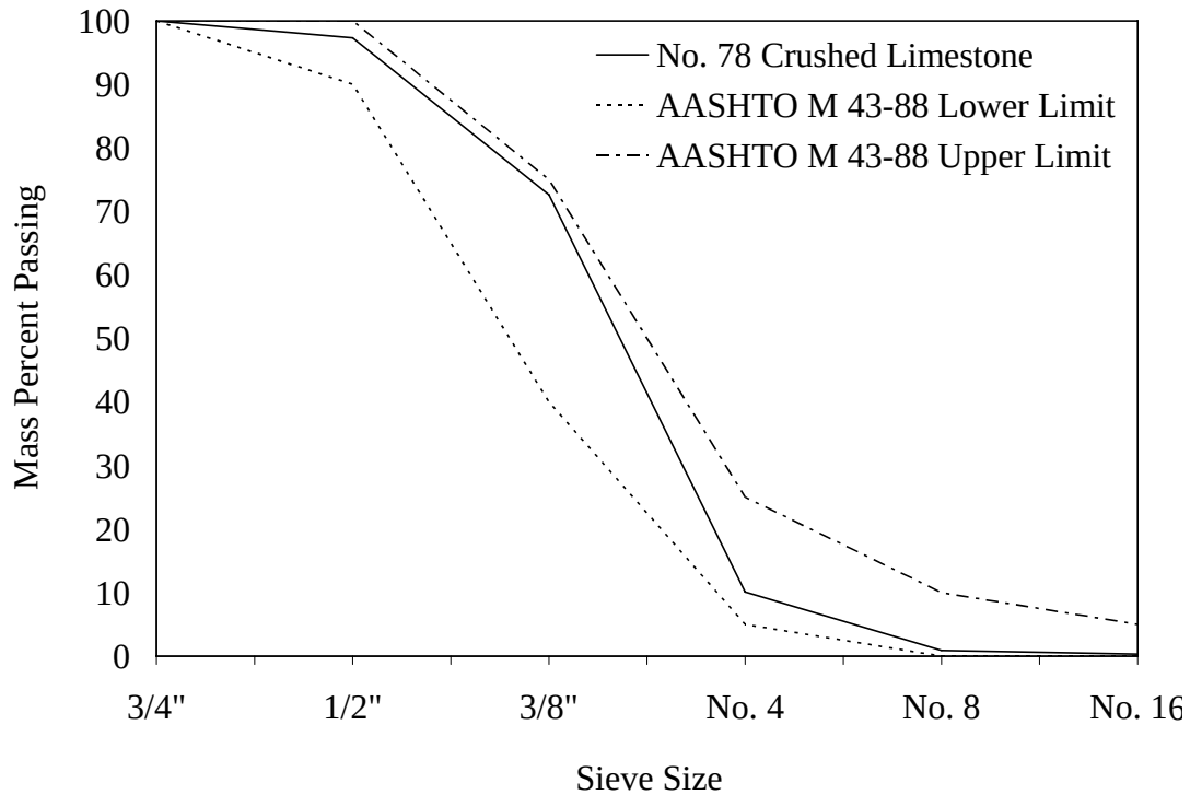
Figure 3.7: Gradation test results for Vulcan Materials No. 78 Limestone
