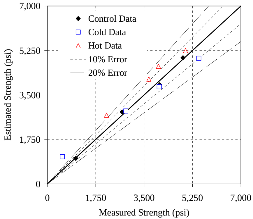
Figure 6.44: Error plot for the Type I - 0.41 mixture, simplified method, E = 40 kJ/mol
