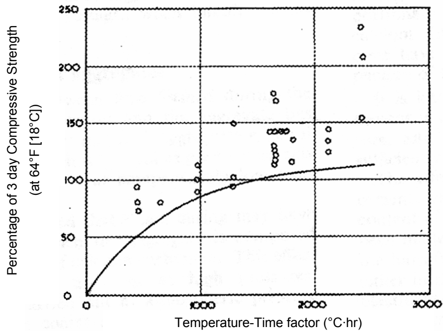
Figure 2.9: Further results from Nurse's experiments (1949)
