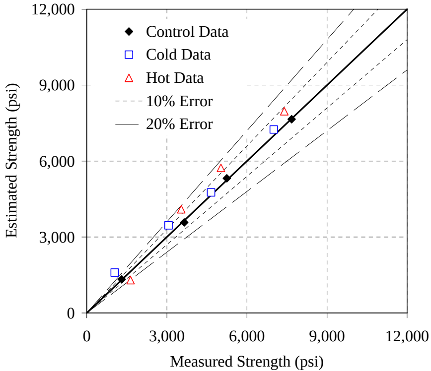
Figure H-18: Error plot for the 70/20/10 - 0.37 mixture, simplified method, T_o = 32^\circ\text{F}
