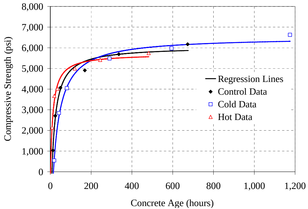
Figure 5.2: Compressive strength versus age results for Type I - 0.41 mixture
