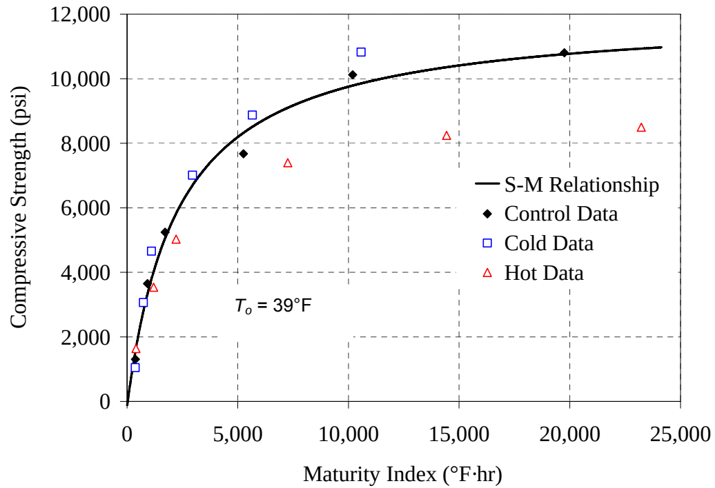
Figure B-9: 70/20/10 - 0.37 mixture, (a) compressive strength vs. age, (b) strength-maturity plot, ASTM C 1074 method
