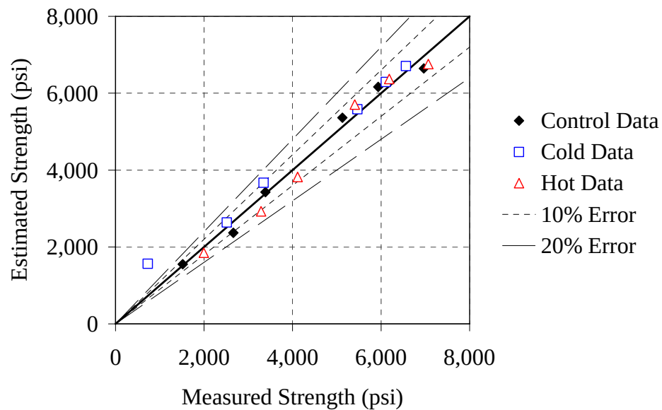
Figure 6.12: Estimated strength versus actual strength for the 20% F mixture
