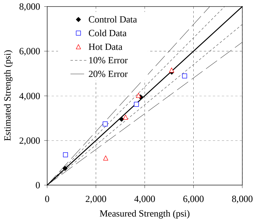
Figure G-15: Error plot for the Type III - 0.44 mixture, Modified method, NSM
