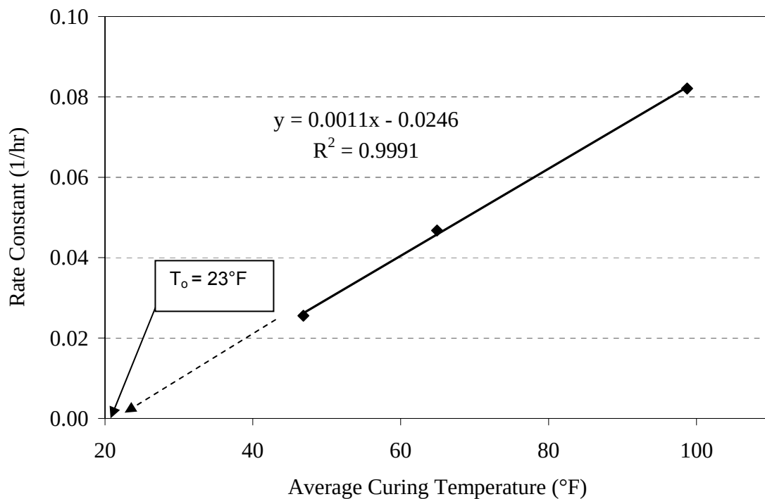
Figure 6.1: Determining the best-fit datum temperature, ASTM C 1074 method (Type I - 0.41 mixture)
