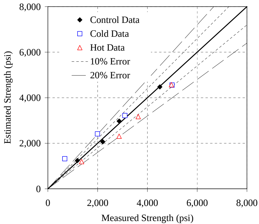
Figure H-5: Error plot for the 30% F mixture, simplified method, T_o = 14^\circ\text{F}
