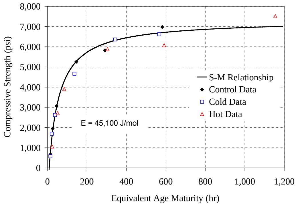
Figure C-5: Strength-maturity plot, ASTM C 1074 method for 30% C mixture
