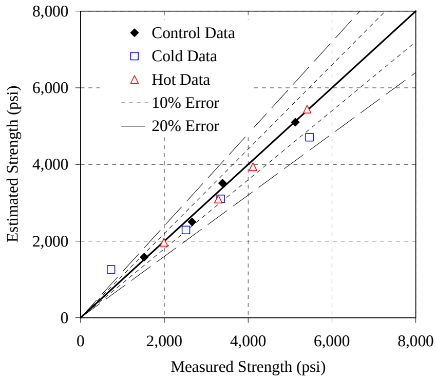
Figure 6.22: Error plot for the 20% F mixture, Modified ASTM method, NSM
