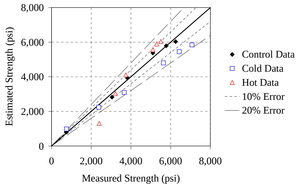
Figure D-8: Estimated strength versus actual strength for Type III - 0.44 mixture
