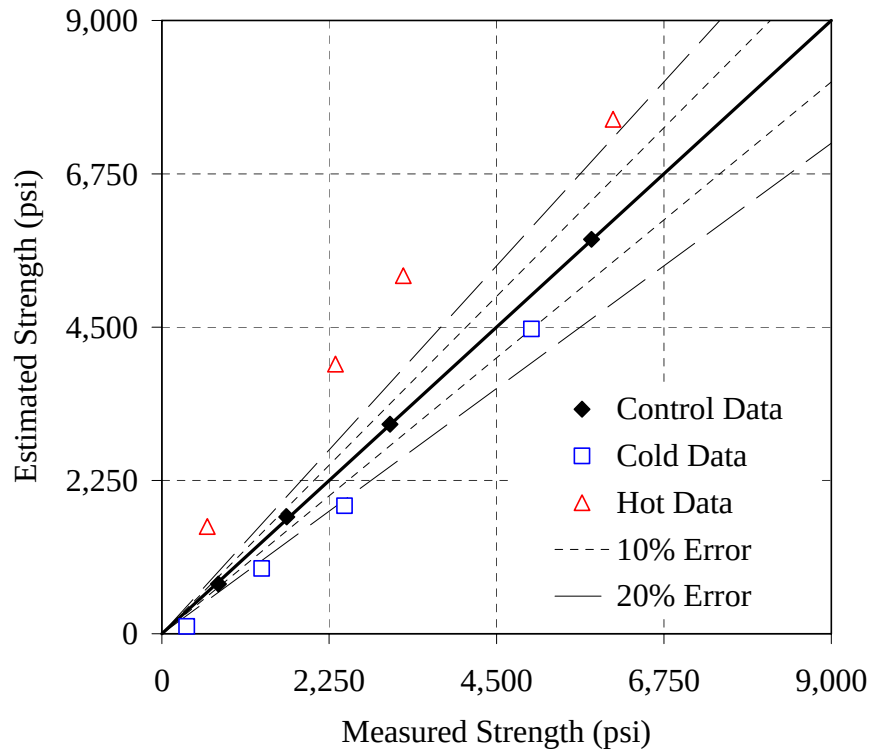
Figure G-34: Error plot for the 50% Slag mixture, ASTM C 1074 method, AM
