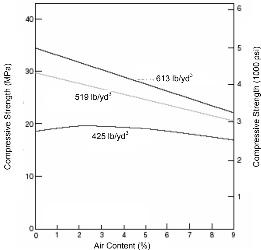
Figure 2.14: Effect of air content on concrete strength (Cordon 1946)
