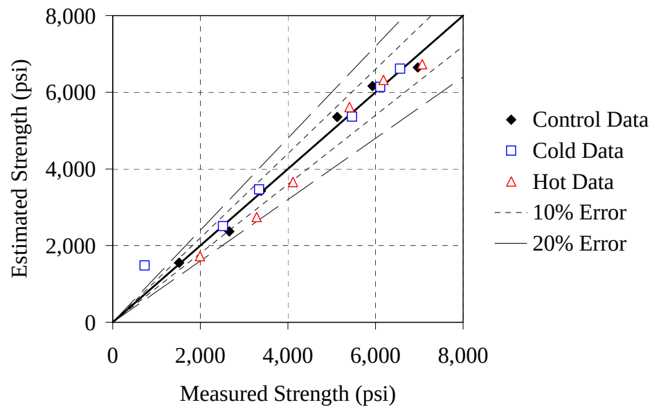
Figure 6.9: Estimated strength versus actual strength for 20% F mixture
