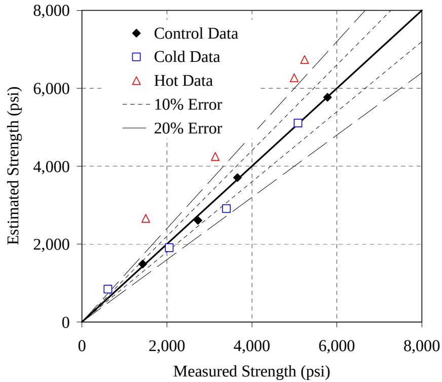
Figure G-32: Error plot for the 30% Slag mixture, ASTM C 1074 method, AM
