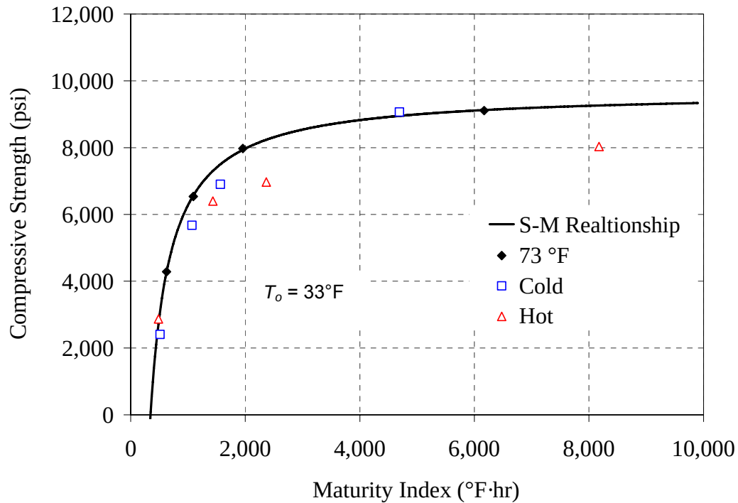
Figure 6.18: Strength-maturity plot, Modified ASTM method for Type III - 0.37 mixture
