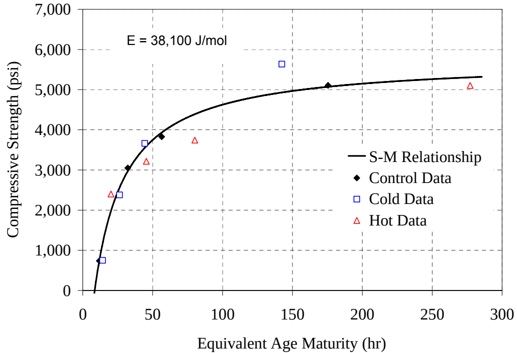
Figure F-8: Strength-maturity plot, Modified ASTM method for Type III - 0.44 mixture
