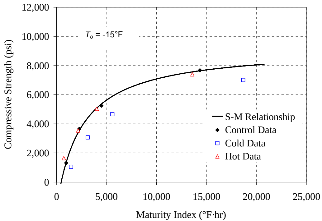
Figure E-9: Strength-maturity plot, Modified ASTM method for 70/20/10 - 0.37 mixture
