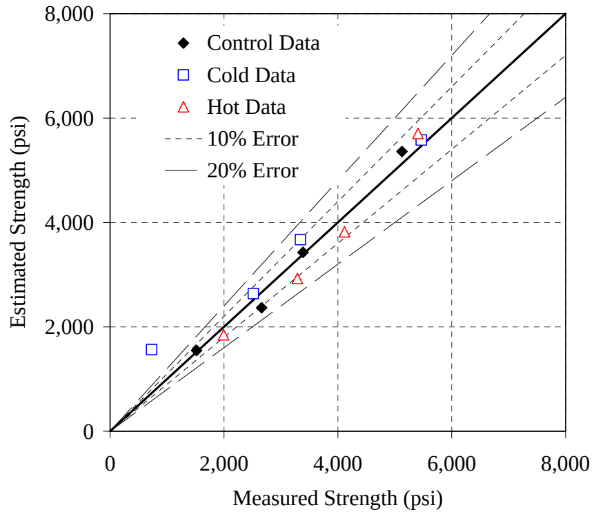
Figure 6.29: Error plot for the 20% F mixture, ASTM C 1074 method, AM
