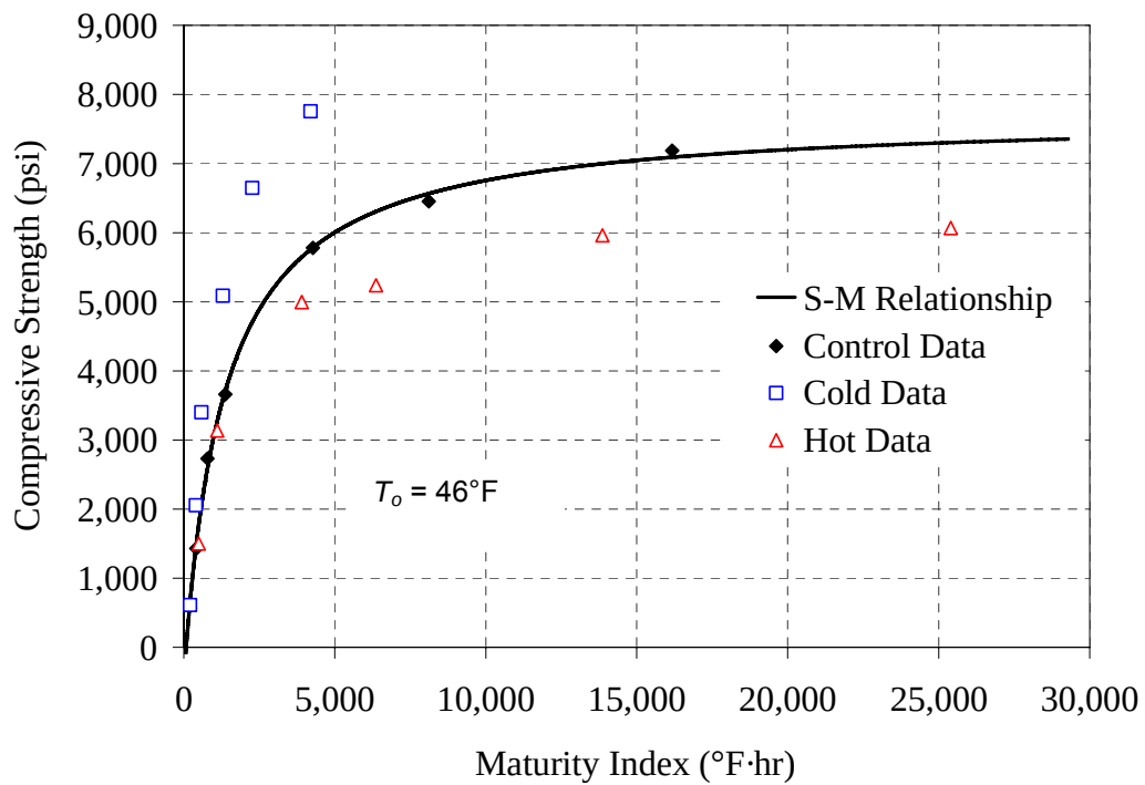
Figure B-6: 30% Slag mixture, (a) compressive strength vs. age, (b) strength-maturity plot, ASTM C 1074 method
