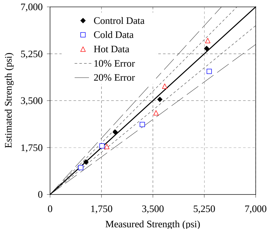
Figure G-8: Error plot for the 20% C mixture, ASTM C 1074 method, NSM
