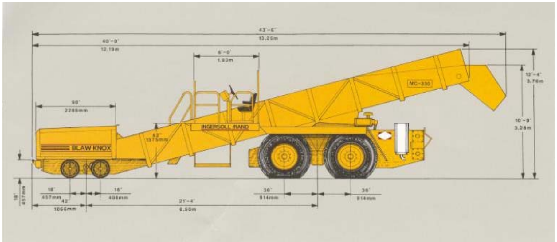
Figure 1. Dimensions of a Blaw-Knox MC-330 (Blaw-Knox 2000).
