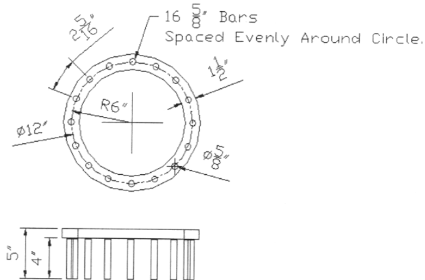
Figure 2.5: J-Ring Testing Apparatus (ASTM J-Ring Draft 2004)
