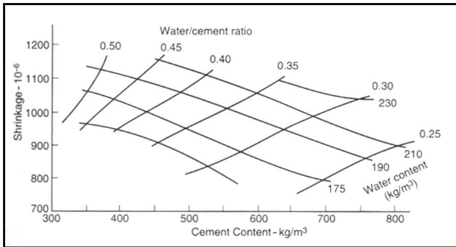
Figure 2.14: Shrinkage versus Cement Content (Neville 1996)
