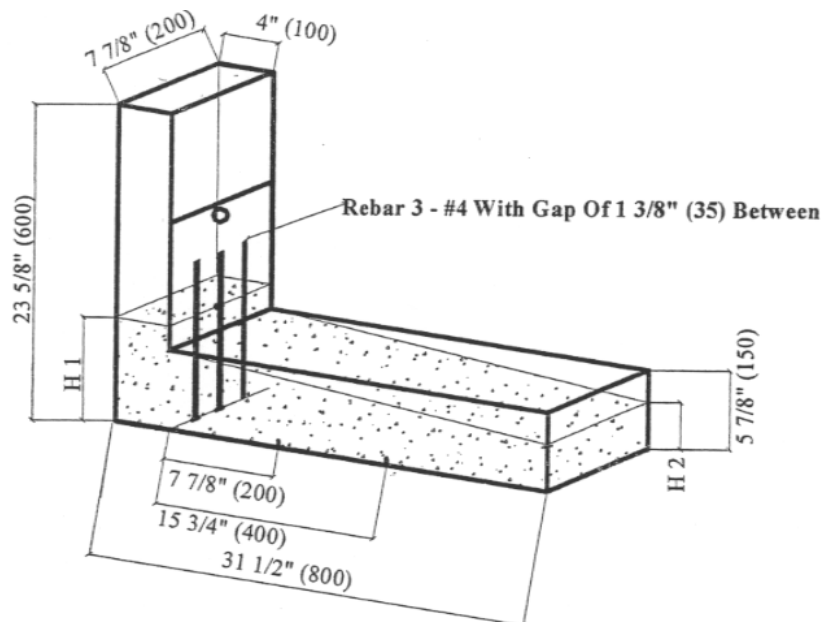
Figure 2.4: L-Box Testing Apparatus (PCI 2003)
