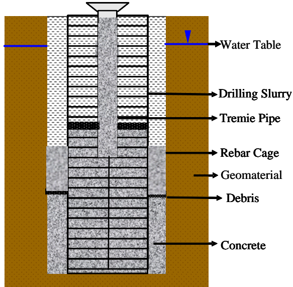
C) Fresh concrete placed in the shaft shaft flows laterally entrapping debris.
