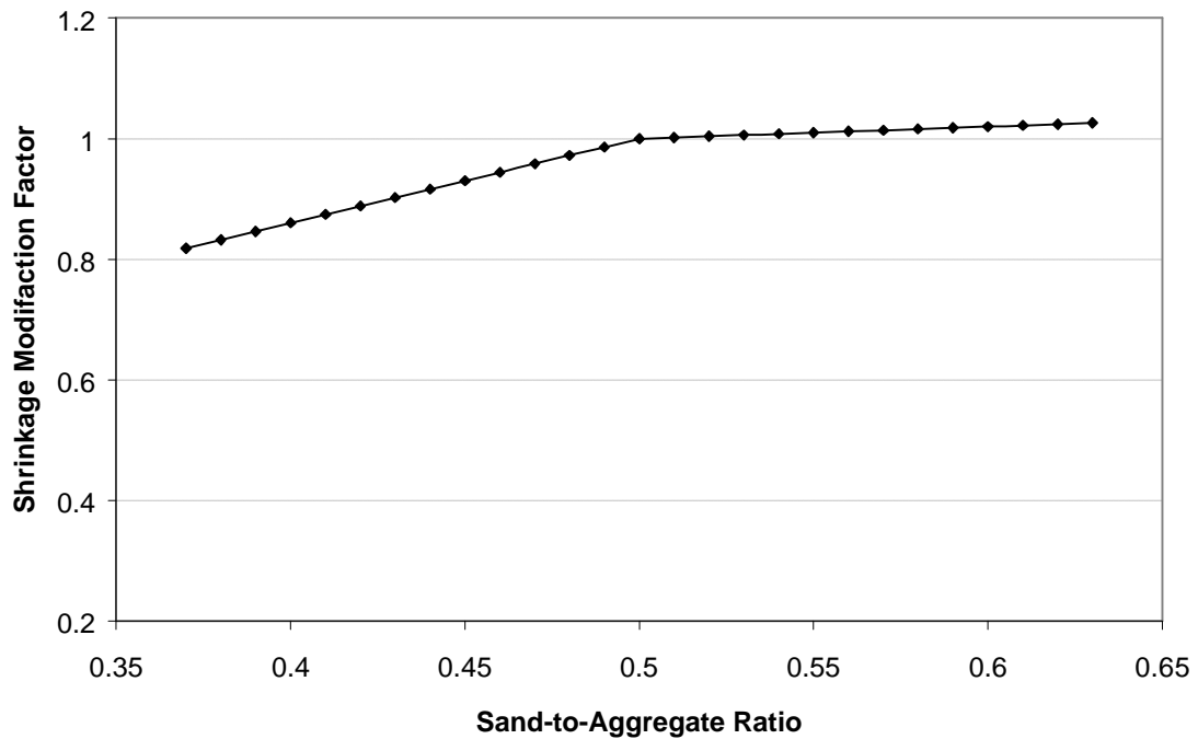
Figure 2.13: Shrinkage Modification Factor for Different Sand-to-Aggregate Ratios (ACI Committee 209 2002)
