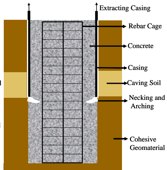
B) Concrete placement is complete, but due to long periods of placement or construction delays the concrete has lost its workability. The casing is extremely difficult to remove which causes arching and necking to occur.
