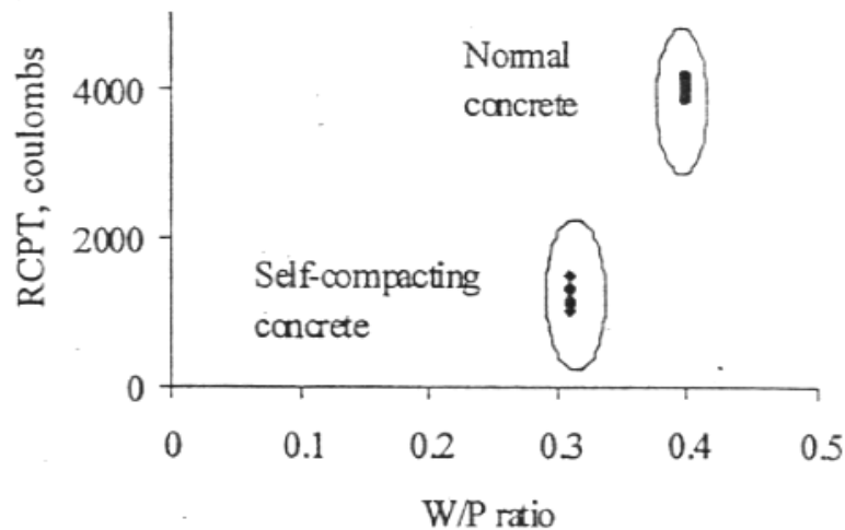
Figure 2.20: RCPT Values of SCC and Normal Concrete (Raghavan et al. 2003)
