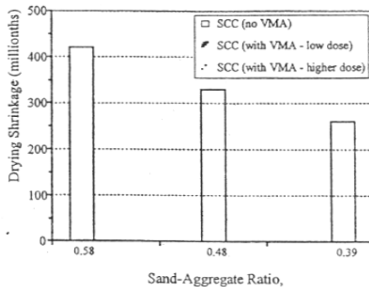
Figure 2.17: Drying Shrinkage versus Sand-to-Aggregate Ratio (Attiogbe et al. 2003)
