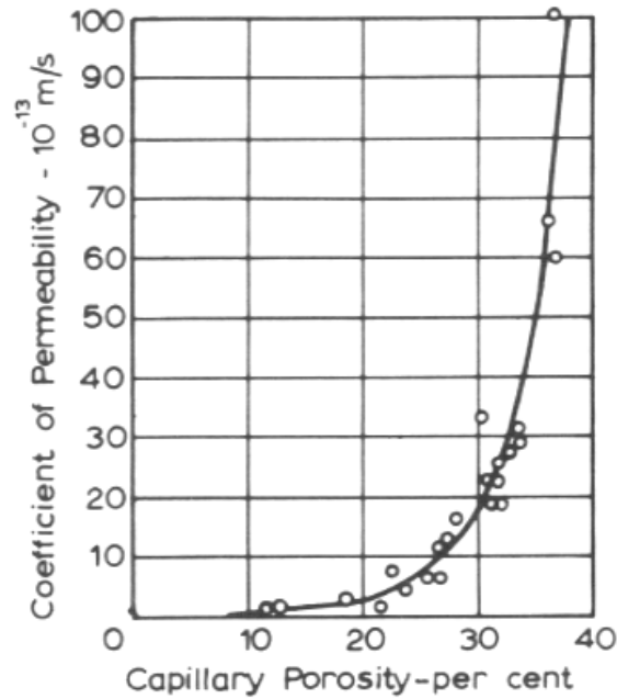
Figure 2.18: Coefficient of Permeability versus Capillary Porosity (Neville 1996)
