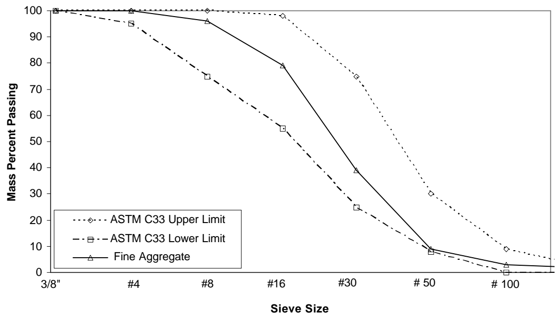
Figure 4.14: Fine Aggregate Gradation for South Carolina Material
