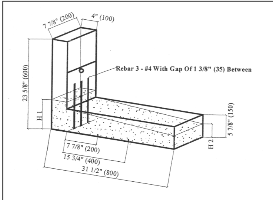
Figure 5.6: L-Box Dimensions (PCI 2003)
