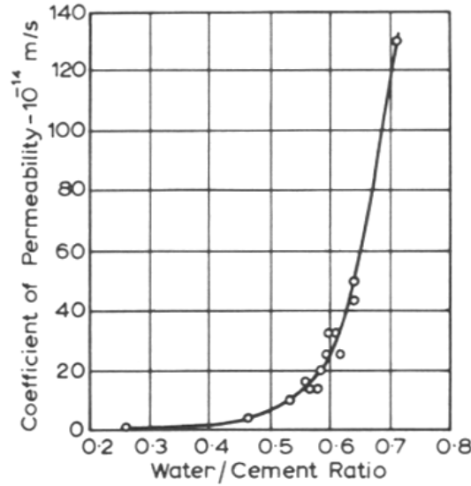
Figure 2.19: Coefficient of Permeability versus Water-to-Cement Ratio (Neville 1996)
