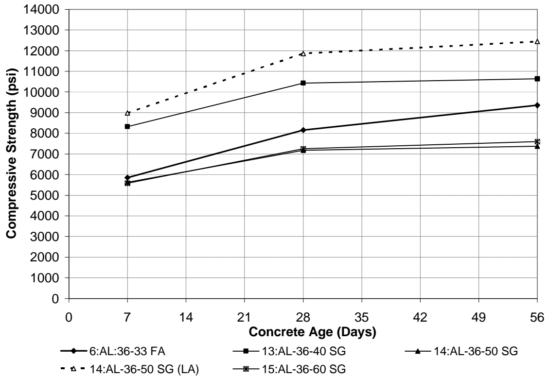
Figure 6.33: Compressive Strength vs. Concrete Age for GGBFS Mixtures
