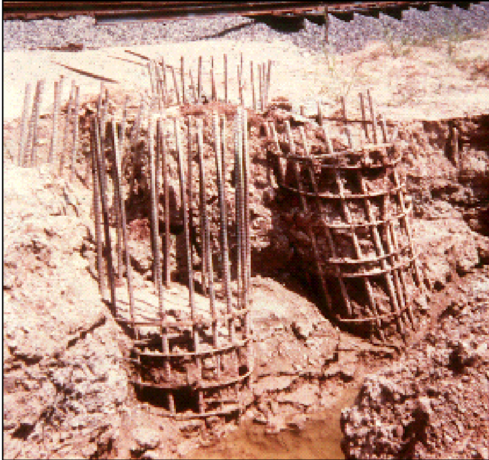
Figure 3.13: Shaft Defects due to the Extraction of the Casing (Annual ADSC Short Course)
