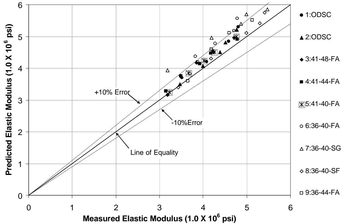
Figure 6.13: Predicted vs. Measured Elastic Modulus according to ACI 318 (2002) (Equation for Phase IV)
