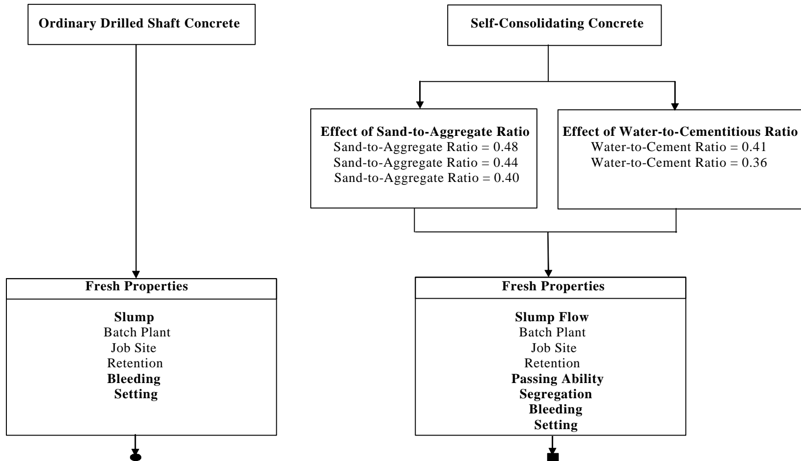
Figure 4.4: Flow Chart for Phase IV (continued on next page)
