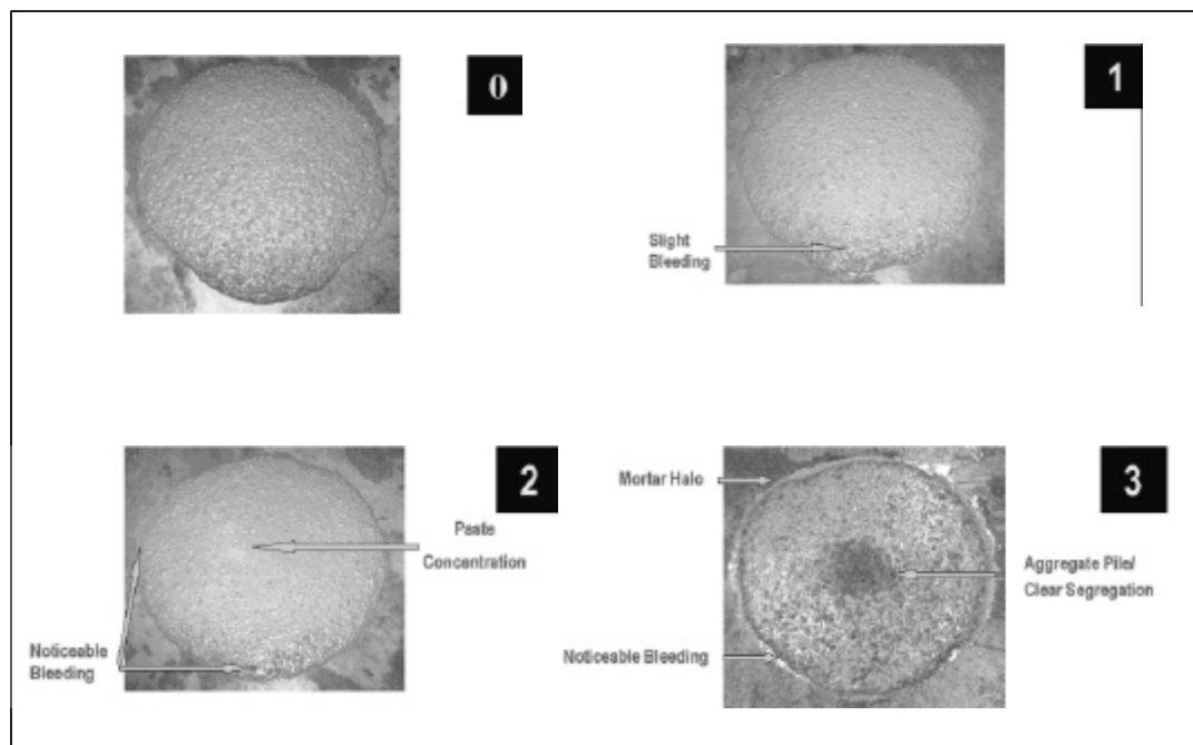
Figure 5.4: Visual Stability Index Rating (Degussa Construction Chemicals 2004)
