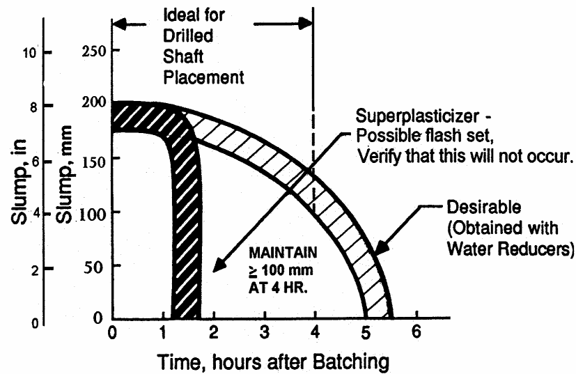
Figure 3.14: Slump Loss versus Time Relationship (O'Neill and Reese 1999)
