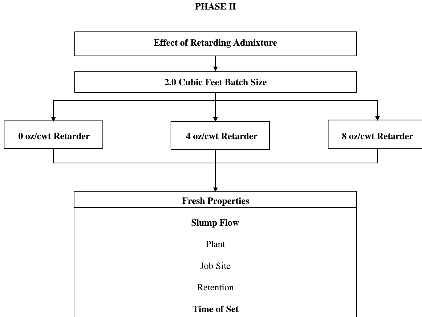
Figure 4.2: Flow chart for Phase II
