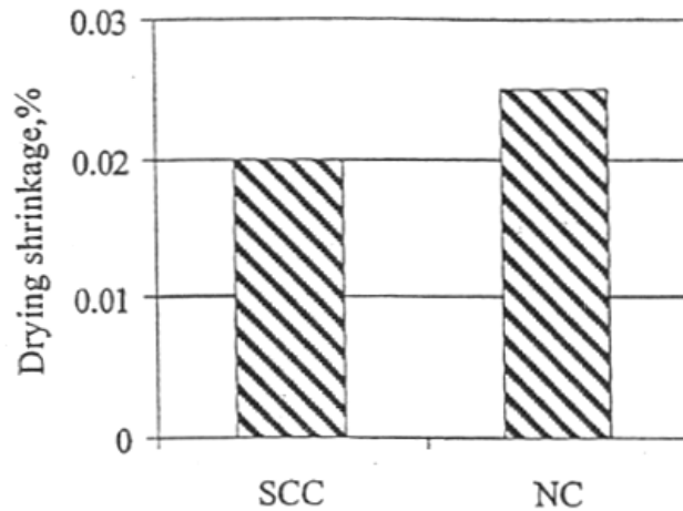
Figure 2.16: SCC versus Normal Concrete (Raghavan et al. 2003)
