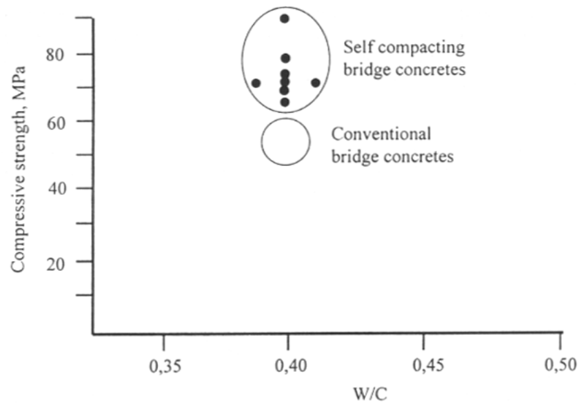
Figure 2.10: Average Compressive Strengths of SCC and Conventional Bridge Concretes with w/c of 0.40 (Tragardh 1999)
