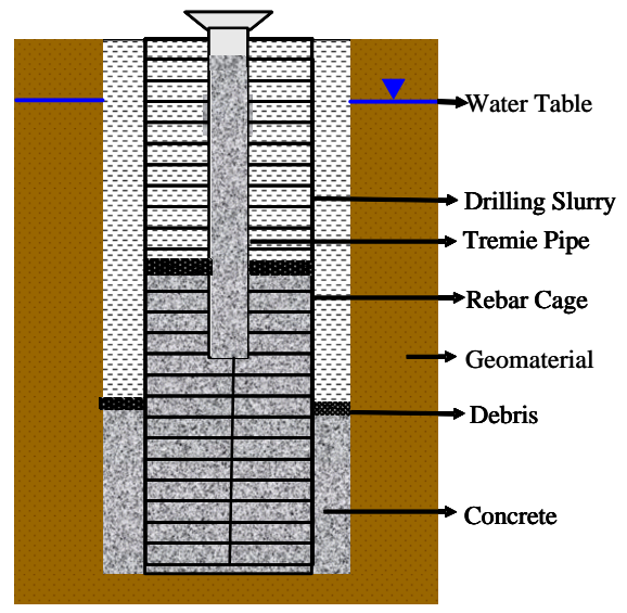
B) Heavily congested rebar cage begins to screen the concrete causing an elevation difference between the inside and outside rebar cage.
