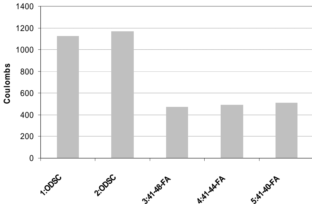
Figure 6.16: 91-Day Permeability Results
