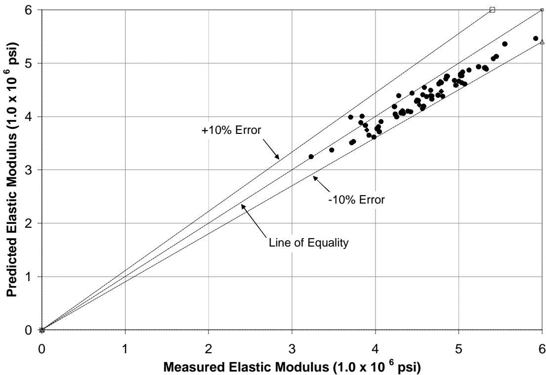
Figure 6.40: Predicted vs. Measured Elastic Modulus According to ACI 363 (2002) - (Phase V)
