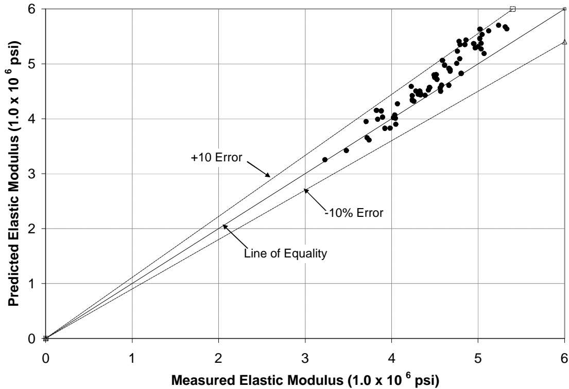
Figure 6.39: Predicted vs. Measured Elastic Modulus According to ACI 318 (2002) - (Phase V)
