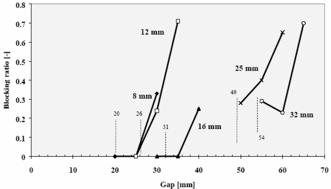
Figure 2.9: Blocking Ratios versus Reinforcement Spacing for Different Size Aggregate (Petersson 1999)
