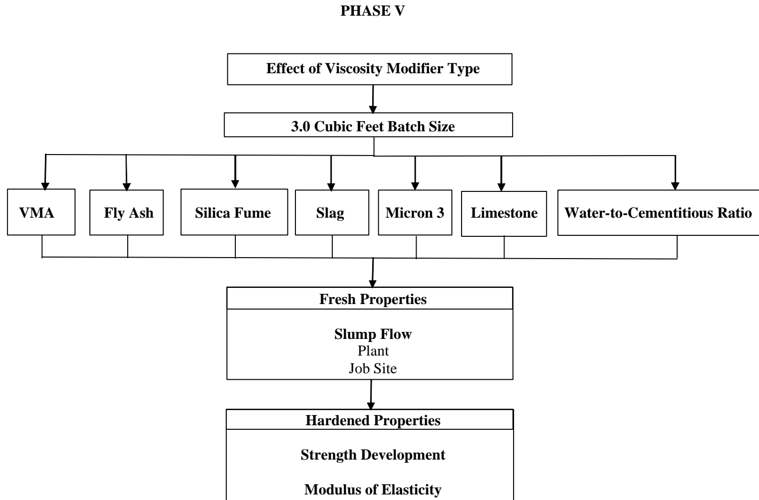
Figure 4.8: Flow Chart for Phase V
