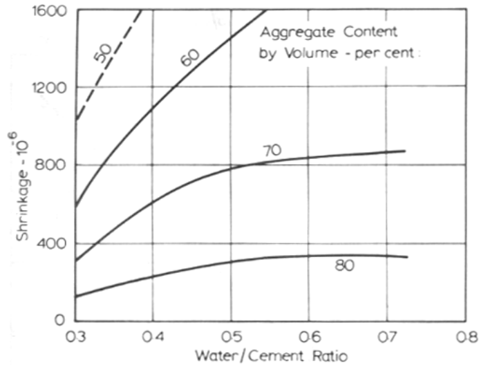
Figure 2.12: Aggregate Content versus Water-to-Cement Ratio (Neville 1996)
