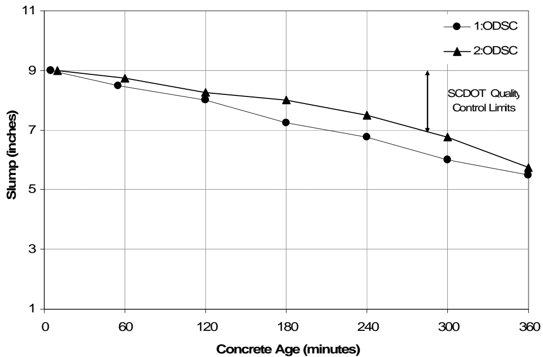
Figure 6.7: Slump vs. Concrete Age
