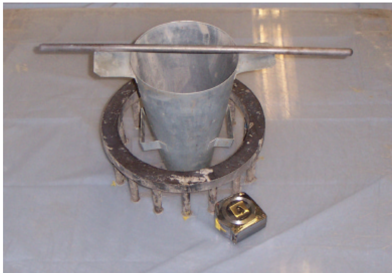
Figure 5.5: Testing Equipment for J-Ring Test
