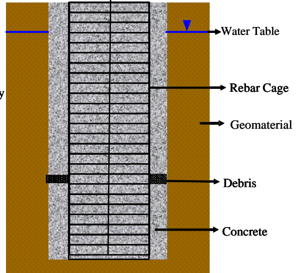
D) Completed shaft may contain entrapped debris due to heavily congested rebar cage.
