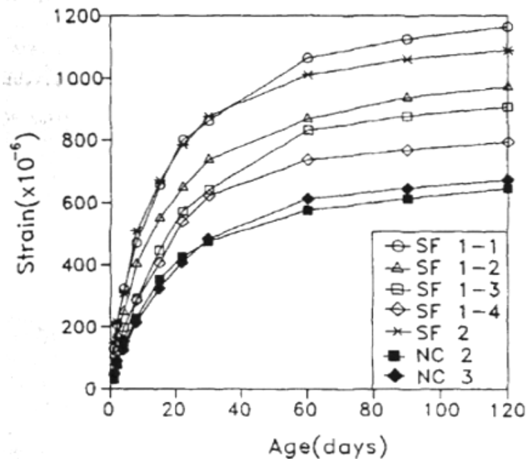
Figure 2.15: Drying Shrinkage versus Age (Kim et al. 1998)
