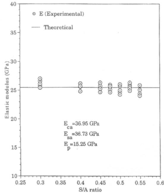
Figure 2.11: Elastic Modulus versus Sand-to-Aggregate Ratio (Su et al. 2002)
