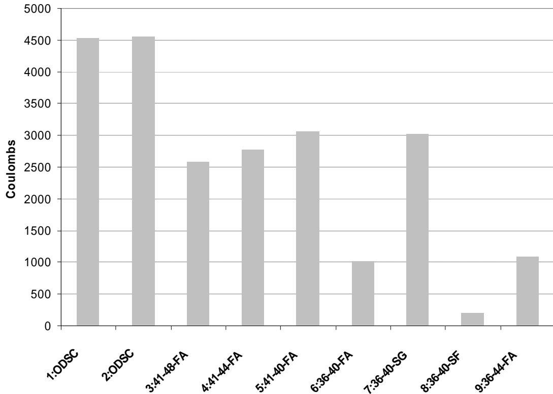
Figure 6.17: 365-Day Permeability Results
