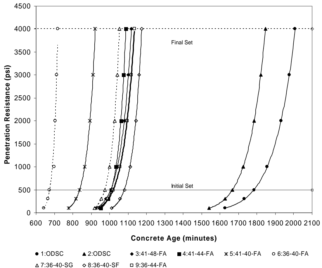
Figure 6.10: Penetration Resistance vs. Concrete Age
