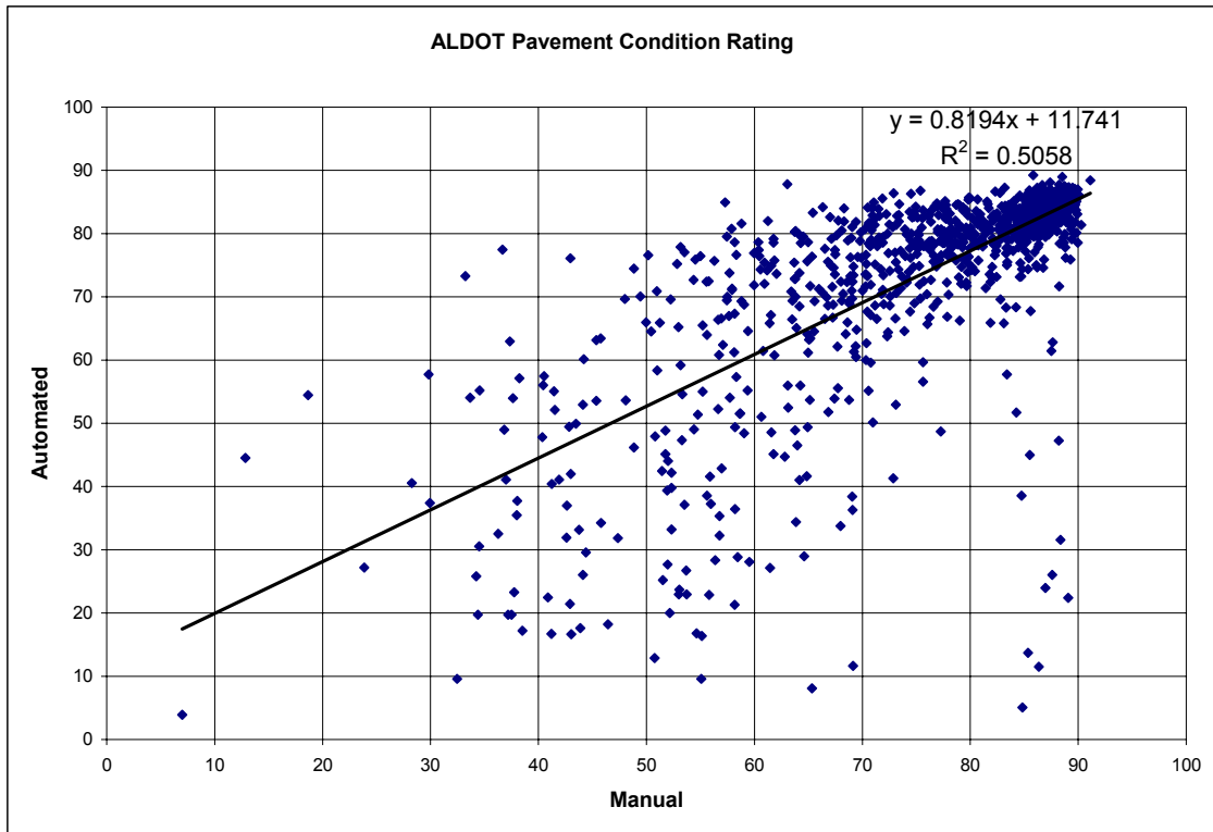
Figure C.1 ALDOT Pavement Condition Rating (Eq. 3.3) Regression Plot
