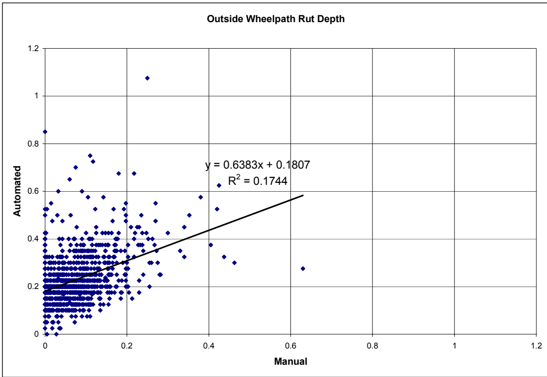
Figure C.3 Outside Wheelpath Rut Depth Regression Plot
