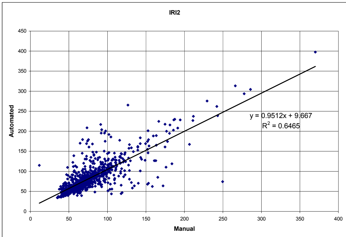
Figure C.2 International Roughness Index 2 Regression Plot
