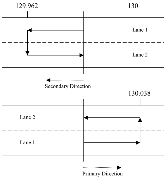
Figure 4.2 Schematic of ALDOT's Manual Survey for a Multilane Section.
