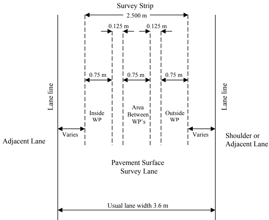
Figure 2.8 Cross Section of Survey Lane Showing Survey Area (AASHTO, 2001).
