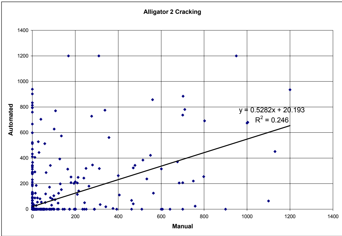
Figure C.5 Alligator 2 Cracking Regression Plot
