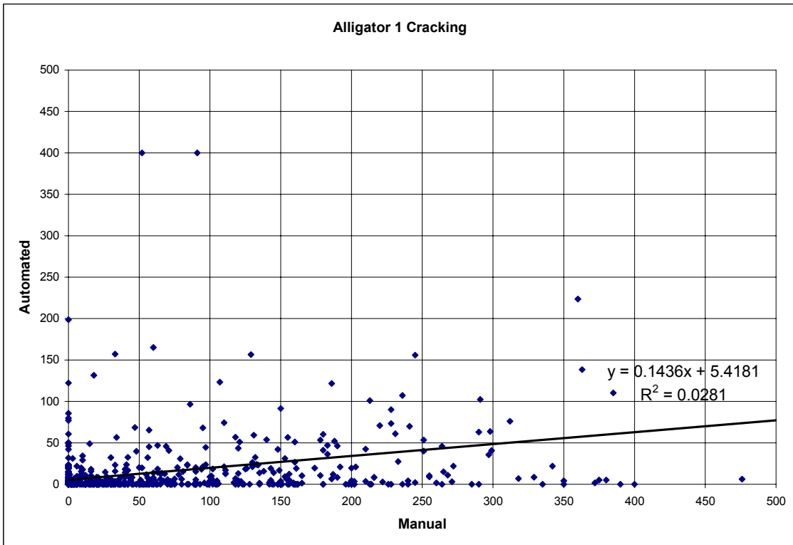
Figure C.4 Alligator 1 Cracking Regression Plot
