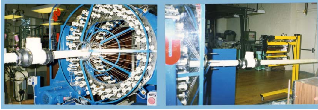
Fig. 1 The novel formation and curing center developed at Auburn University, Department of Textile Engineering
